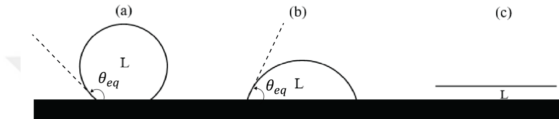
Figure 1.1: Liquids on a solid substrate, (a) hydrophobic ( 180^\circ > \theta_{eq} > 90^\circ ) and (b) hydrophilic ( \theta_{eq} < 90^\circ ) systems show the partial wetting; the wetting is stronger in (b) than (a), (c) shows the complete wetting ( \theta_{eq} = 0^\circ ).
