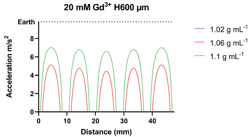
Figure 29. Configuration of the reduced gravitational acceleration of Earth in different densities of cells (1.02, 1.06, and 1.1 g mL -1 ) when using 20 mM Gd 3+ solution at 600 \mu m height from Halbach array.
