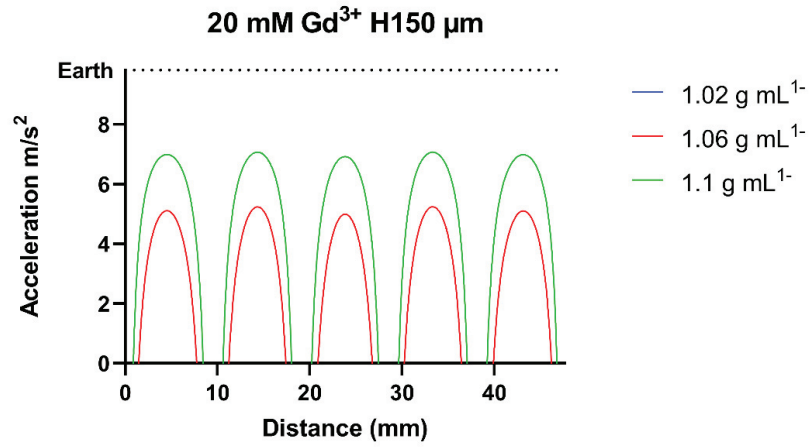
Figure 20. Configuration of the reduced gravitational acceleration of Earth in different densities of cells (1.02, 1.06, and 1.1 g mL -1 ) when using 20 mM Gd 3+ solution at 150 \mu m height from Halbach array.
