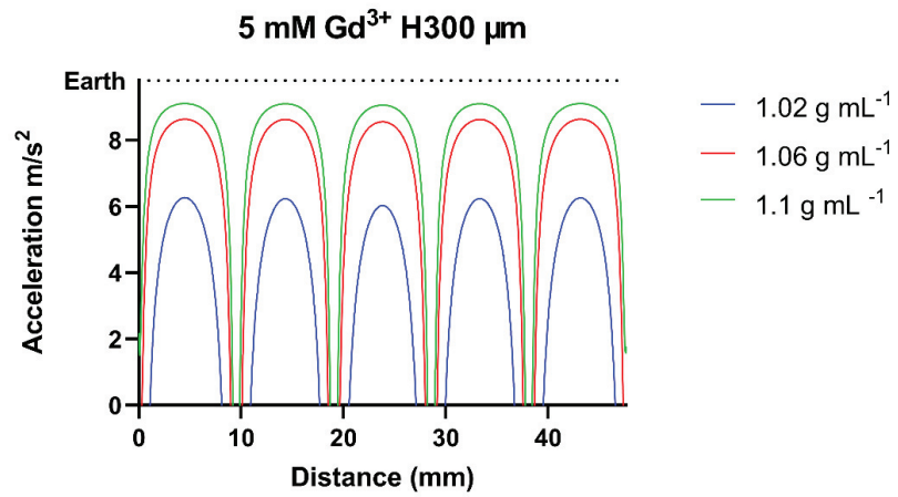
Figure 21. Configuration of the reduced gravitational acceleration of Earth in different densities of cells (1.02, 1.06, and 1.1 g mL -1 ) when using 5 mM Gd 3+ solution at 300 \mu m height from Halbach array.
