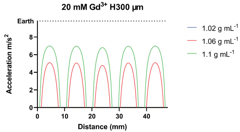
Figure 23. Configuration of the reduced gravitational acceleration of Earth in different densities of cells (1.02, 1.06, and 1.1 g mL -1 ) when using 20 mM Gd 3+ solution at 300 \mu m height from Halbach array.
