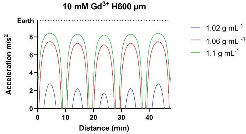
Figure 28. Configuration of the reduced gravitational acceleration of Earth in different densities of cells (1.02, 1.06, and 1.1 g mL -1 ) when using 10 mM Gd 3+ solution at 600 \mu m height from Halbach array.
