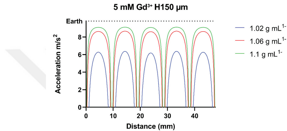
Figure 18. Configuration of the reduced gravitational acceleration of Earth in different densities of cells ( 1.02 , 1.06 , and 1.1 \text{ g mL}^{-1} ) when using 5 \text{ mM Gd}^{3+} solution at 150 \mu\text{m} height from Halbach array.
