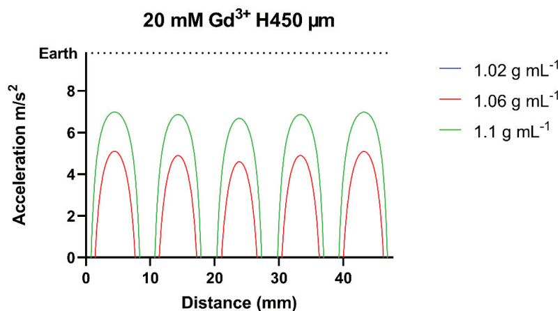
Figure 26. Configuration of the reduced gravitational acceleration of Earth in different densities of cells (1.02, 1.06, and 1.1 g mL -1 ) when using 20 mM Gd 3+ solution at 450 \mu m height from Halbach array.
