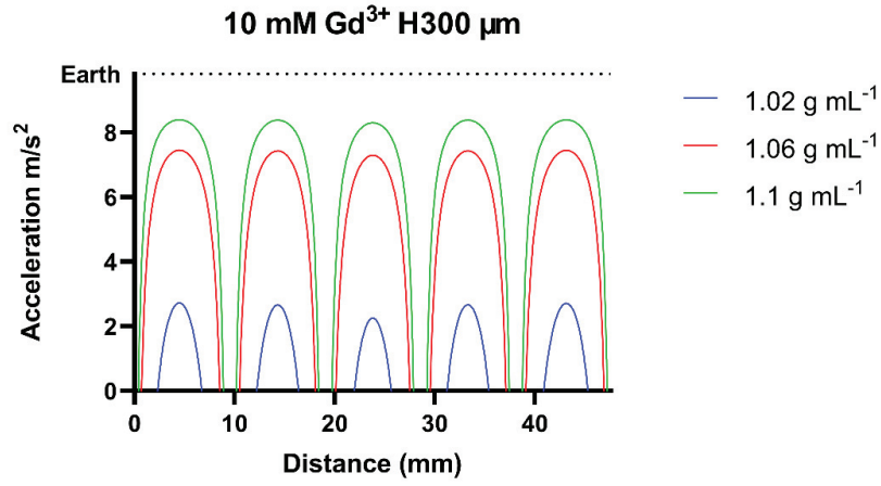
Figure 22. Configuration of the reduced gravitational acceleration of Earth in different densities of cells (1.02, 1.06, and 1.1 g mL -1 ) when using 10 mM Gd 3+ solution at 300 \mu m height from Halbach array.
