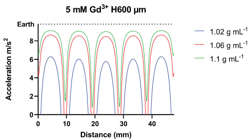
Figure 27. Configuration of the reduced gravitational acceleration of Earth in different densities of cells (1.02, 1.06, and 1.1 g mL -1 ) when using 5 mM Gd 3+ solution at 600 \mu m height from Halbach array.
