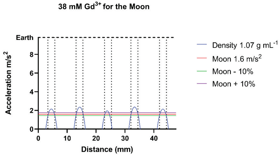
Figure 32. The graph shows that when the density of the cells is 1.07 \text{ g mL}^{-1} and the \text{Gd}^{3+} concentration is 38 \text{ mM} , the gravity of the Earth ( 9.81 \text{ m/s}^2 ) is approximately reduced to that of the Moon's gravity ( 1.6 \text{ m/s}^2 ).
