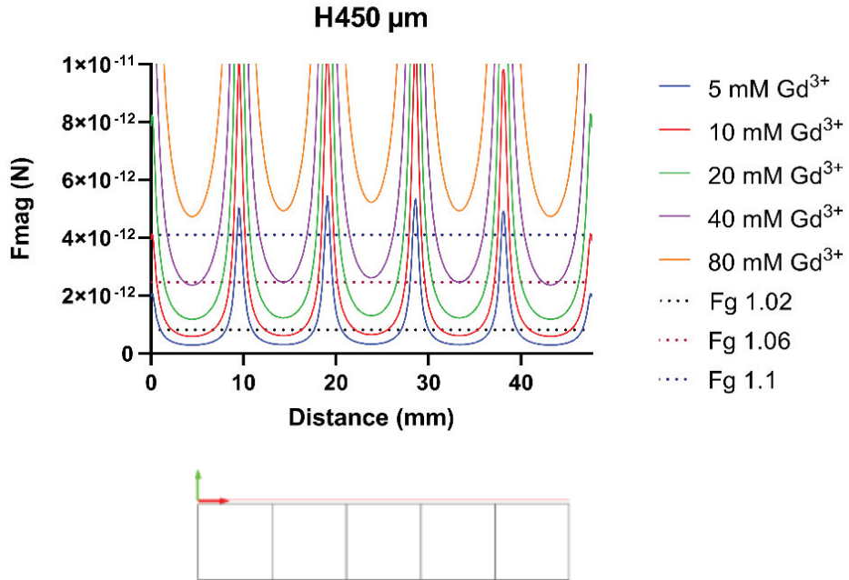
Figure 16. The configuration of the relationship between magnetic force and gravitational force (at different densities of cells 1.02 \text{ g mL}^{-1} , 1.06 \text{ g mL}^{-1} , and 1.1 \text{ g mL}^{-1}
