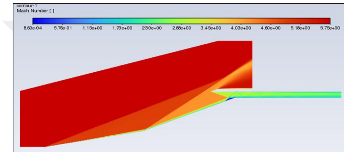
Figure 5.3. Off-Design Mach Contour of M=5.75
