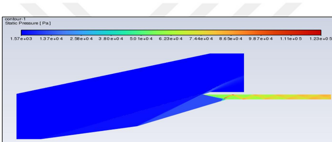
Figure 4.10. Static Pressure Contour of Viscous CFD Result
