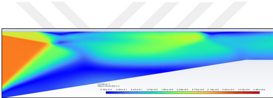
Figure 5.5. Off-Design Disturbed Mach Contour of M=4.5
