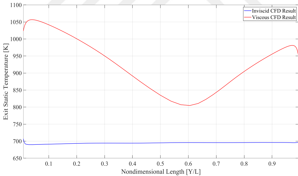
Figure 4.20. Comparison of Isolator Exit Static Temperature Profiles along Isolator Y-Axis
