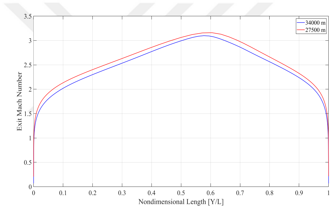
Figure 5.7. Effect of Flight Altitudes on Isolator Exit Mach Number
