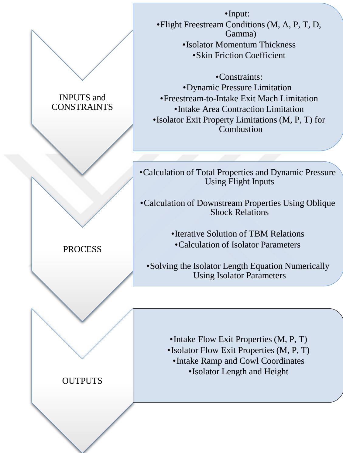
Figure 2.1: Flowchart of Simple Design Tool
