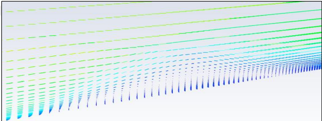
Figure 4.14. Zoomed View of Velocity Vector Profile around Shoulder Bubble
