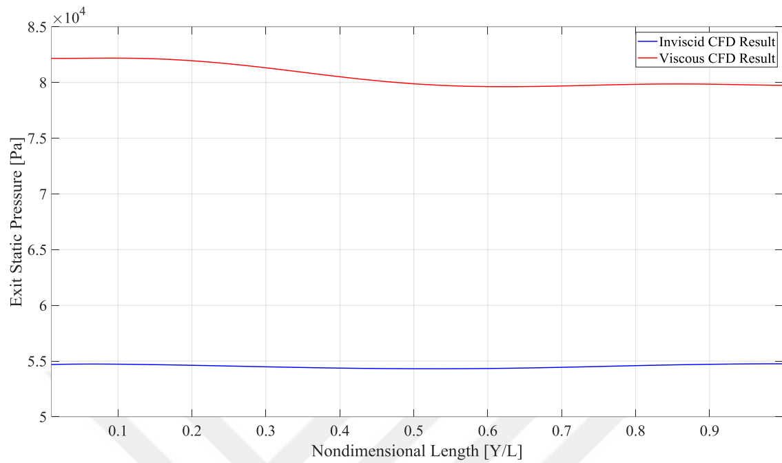
Figure 4.19. Comparison of Isolator Exit Static Pressure Profiles along Isolator Y-Axis
