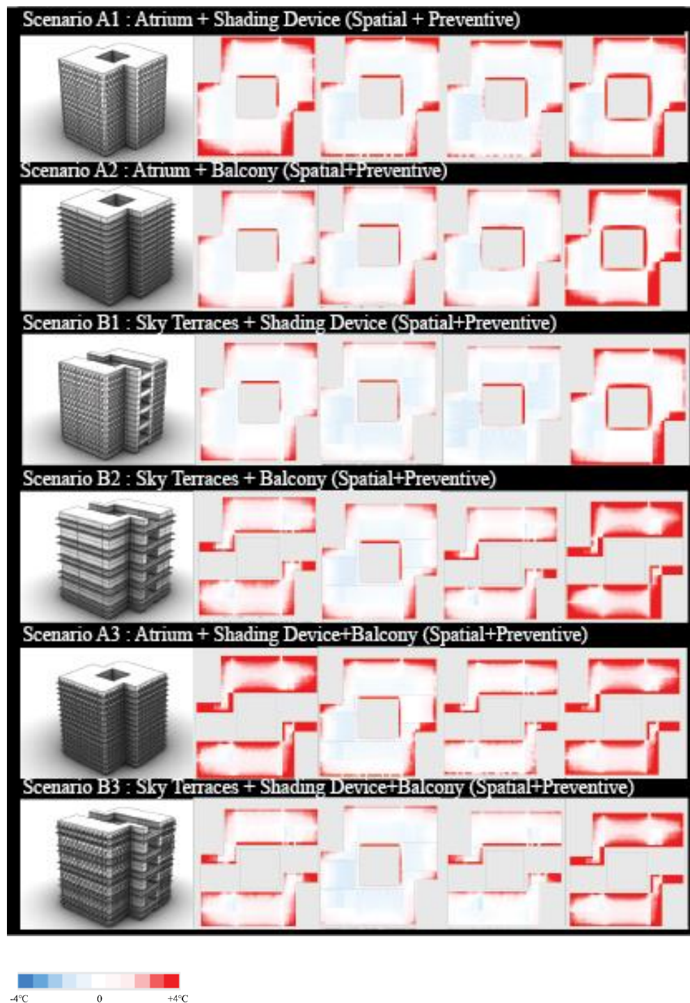
Figure 5.22. ATC thermal comfort degree difference values for each scenario
