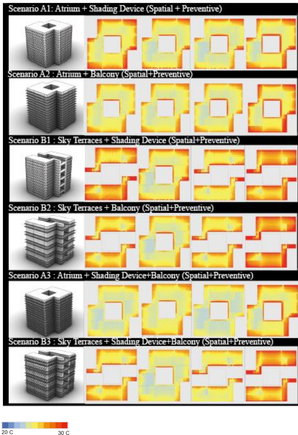
Figure 5.17. ATC thermal comfort Operative Temperature values for each scenario
