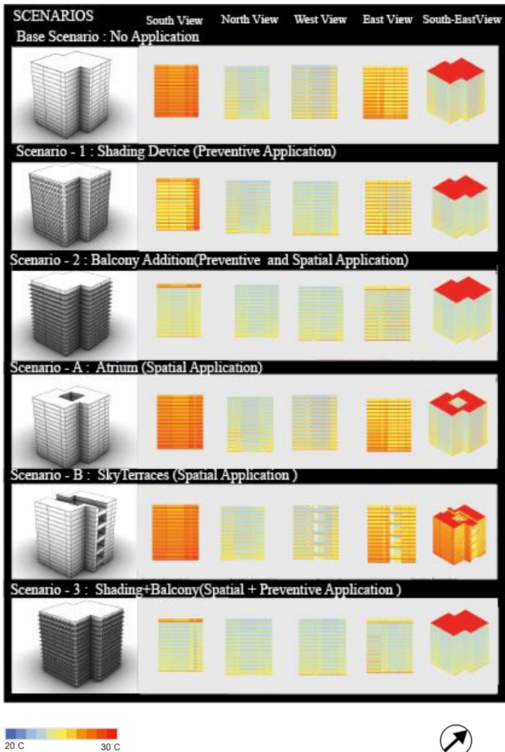
Figure 4.19. Outdoor surface temperature analysis results obtained from EnergyPlus analysis for scenarios
