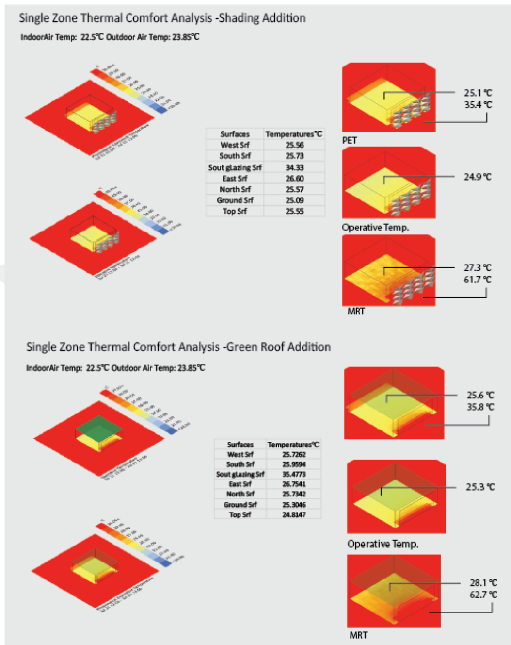
Figure 4.10. Single Zone PET and ATC thermal comfort analysis shading device and green façade application analysis
