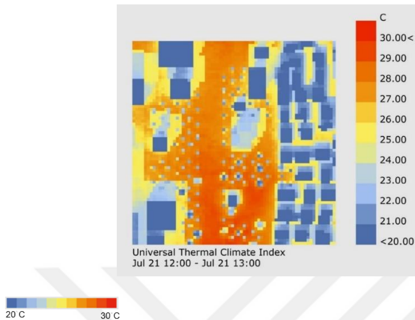
Figure 5.3. UTCI analysis results in neighborhood scale – With tree canopy and without CFD analysis result. 123.045-m 2
