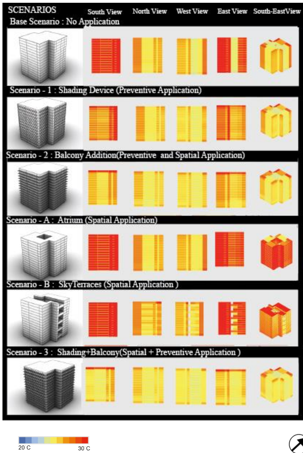
Figure 4.16. Indoor surface temperature analysis results obtained from EnergyPlus analysis for scenarios
