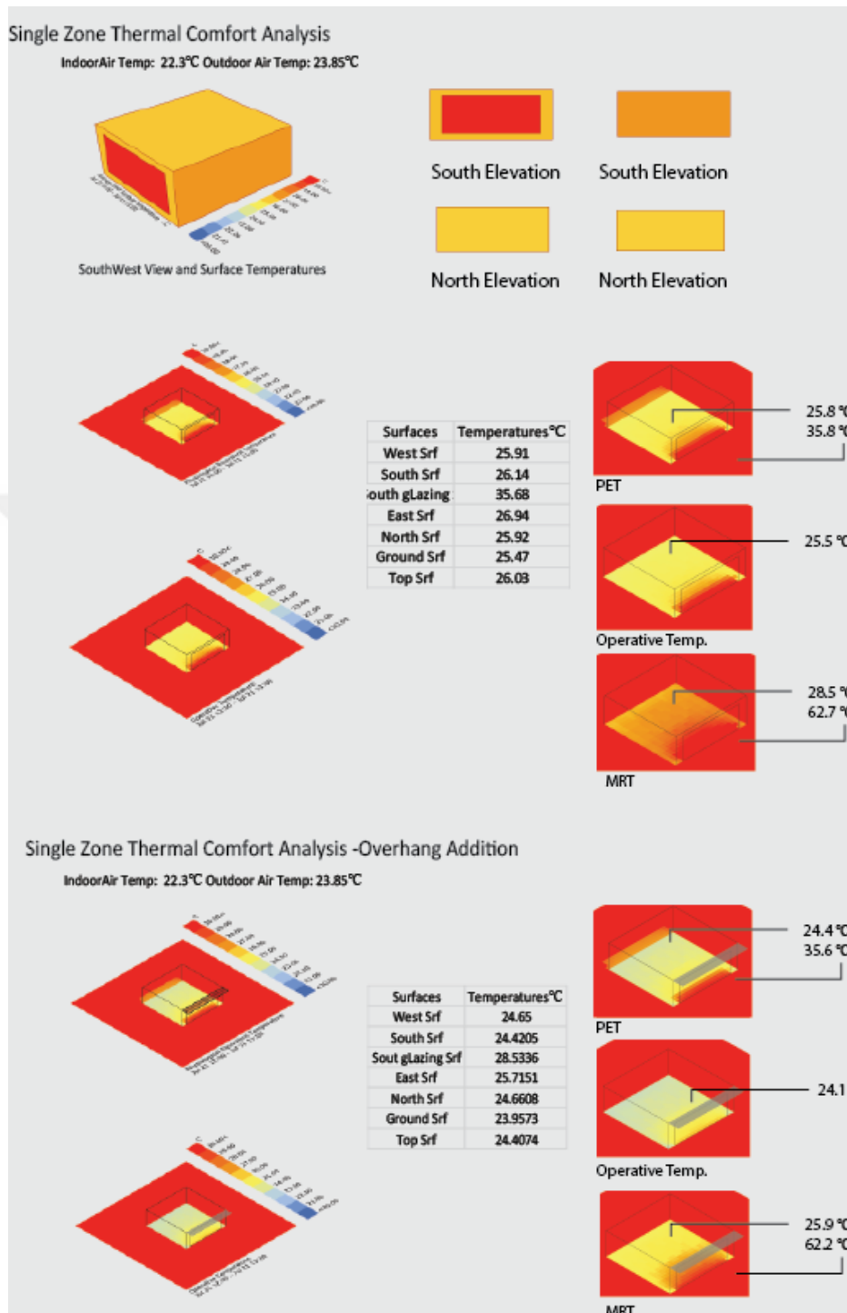
Figure 4.9. Single Zone PET and ATC thermal comfort analysis and overhang addition
