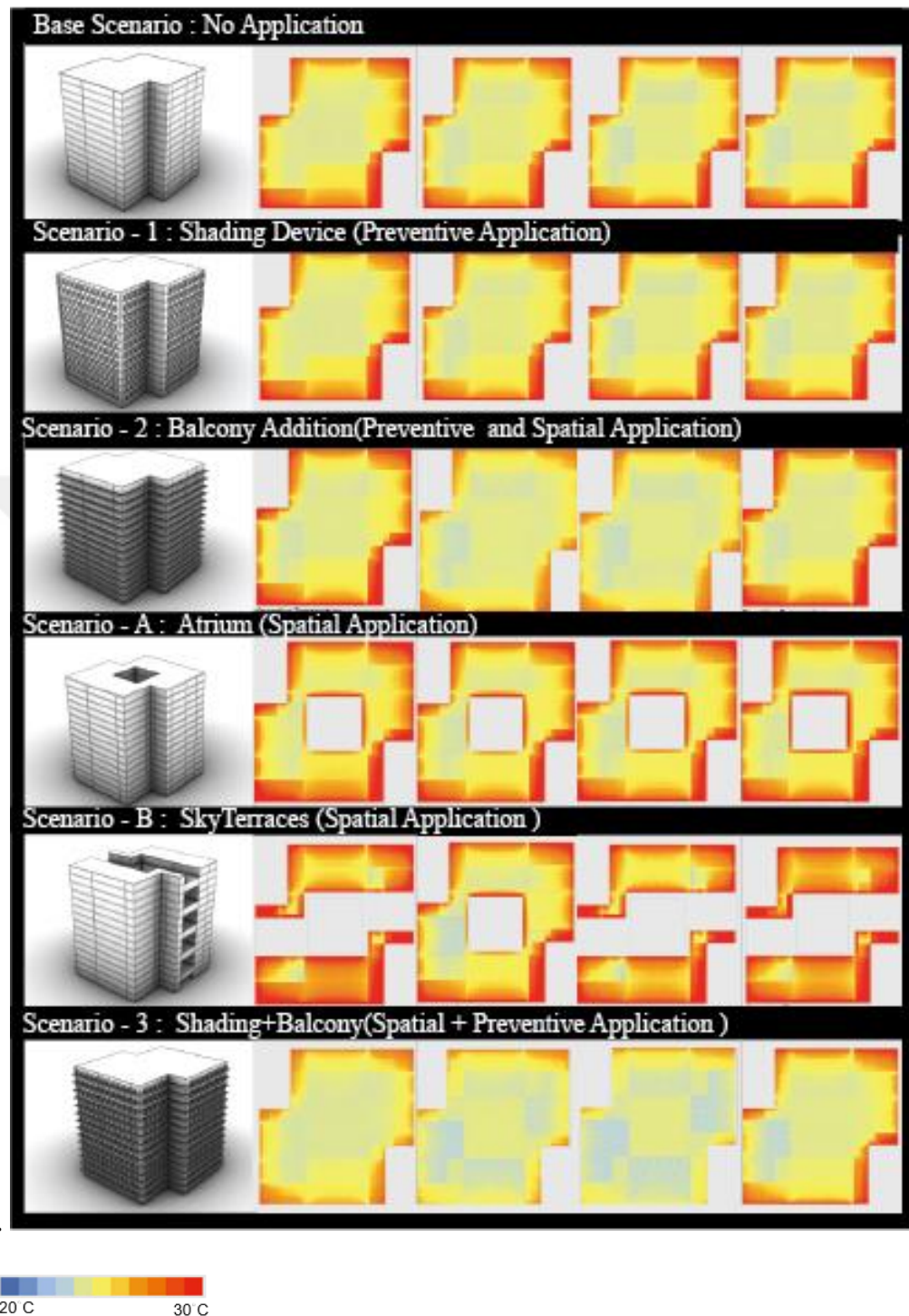
Figure 5.16. ATC thermal comfort Operative Temperature values for each scenario
