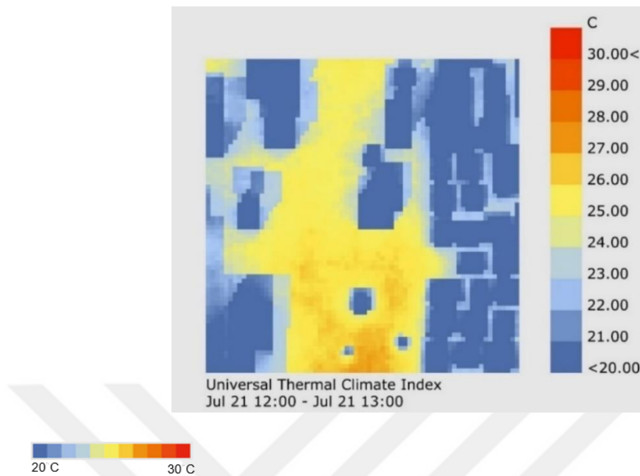
Figure 5.4. UTCI analysis result in neighborhood scale – Without tree Canopy and with Wind Speed Data included
