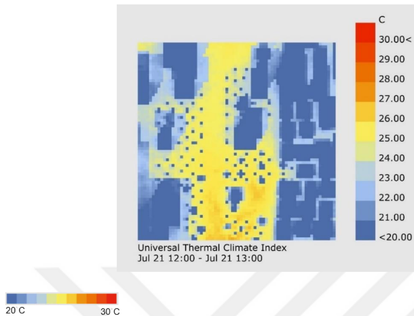
Figure 5.5. UTCI analysis result in neighborhood scale – Tree Canopy and Wind Speed Data included
