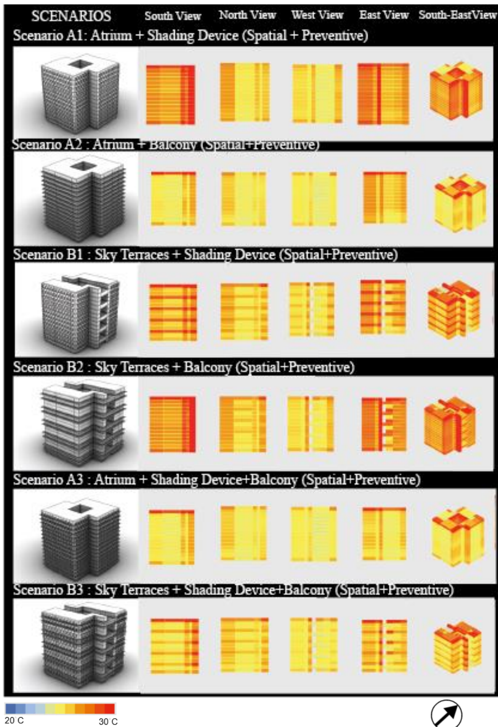
Figure 4.17. Indoor surface temperature analysis results obtained from EnergyPlus analysis for scenarios
