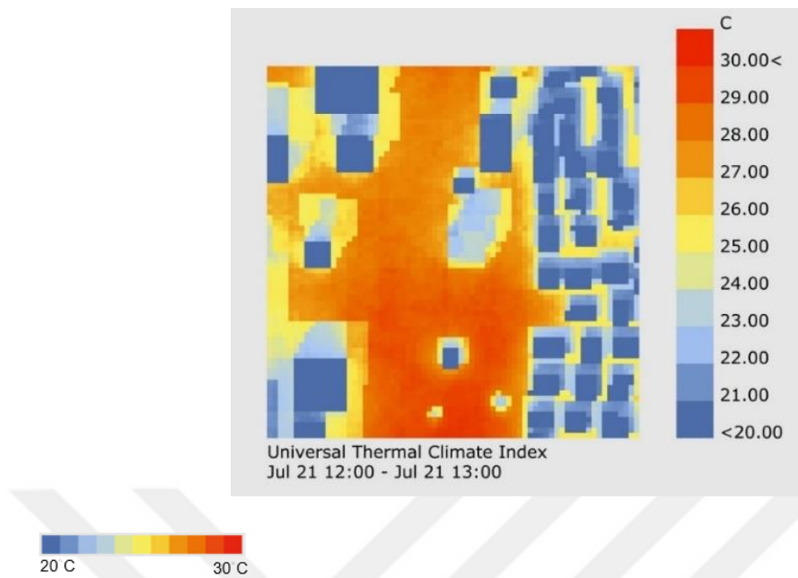
Figure 5.2. UTCI analysis results in neighborhood scale – Without tree canopy and CFD analysis result. 123045-m 2
