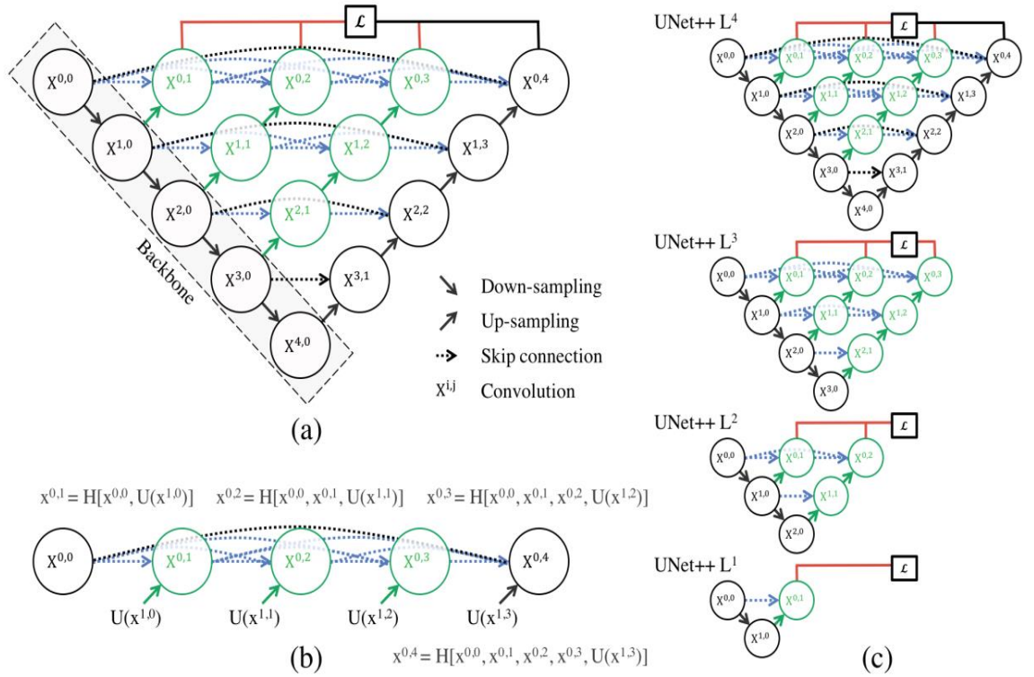
Figure 3.3 Overview of the UNet++ architecture (Zhou et al. 2018)
