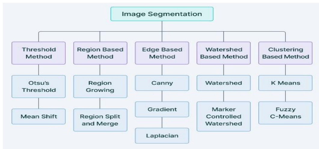
Figure 2.1 Traditional Image Segmentation techniques (Bandyopadhyay 2022)
