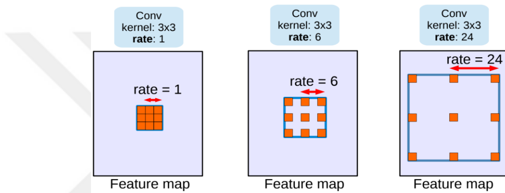
Figure 3.6 Atrous convolution with a 3 \times 3 kernel and various rates (Chen et al. 2017b)
