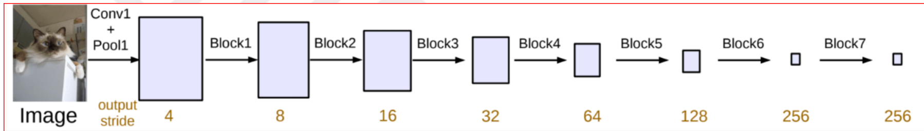
Figure 3.7 Going deeper without atrous convolution (Chen et al. 2017b)
