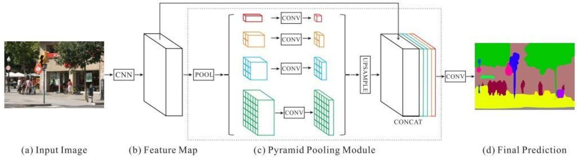
Figure 3.4 Overview of the PSPNet architecture (Zhao et al. 2017)
