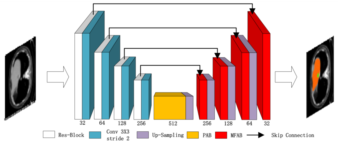
Figure 3.16 The architecture of MA-Net (Li et al. 2022)
