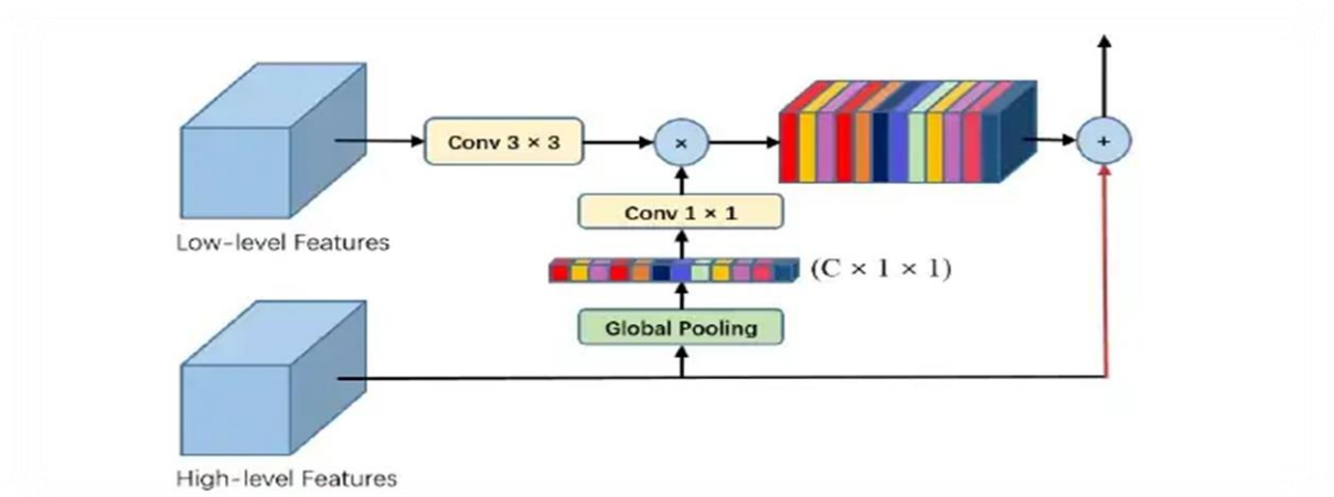
Figure 3.15 Global Attention Upsample module structure (Chaurasia and Culurciello 2017).
