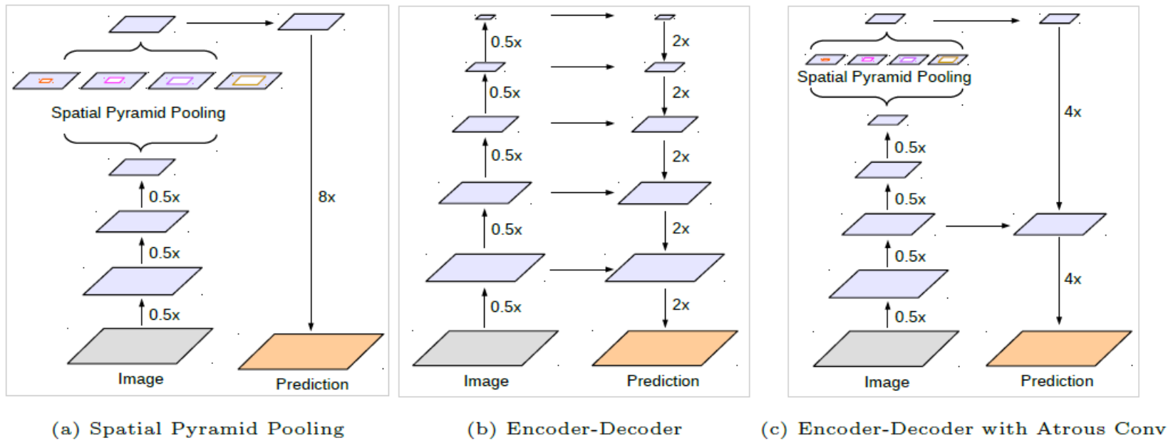
Figure 3.10 Spatial Pyramid Pooling, and Encoder-Decoder structure (Chen et al. 2018)
