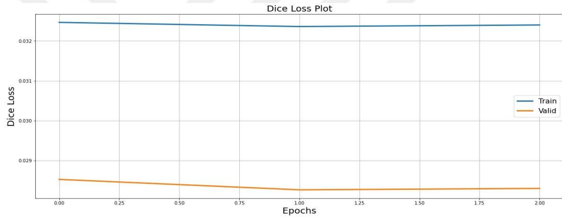
Figure 4.2 Training and validation Dice Loss for 3 epochs using UNet model on DeepGlobe data set
