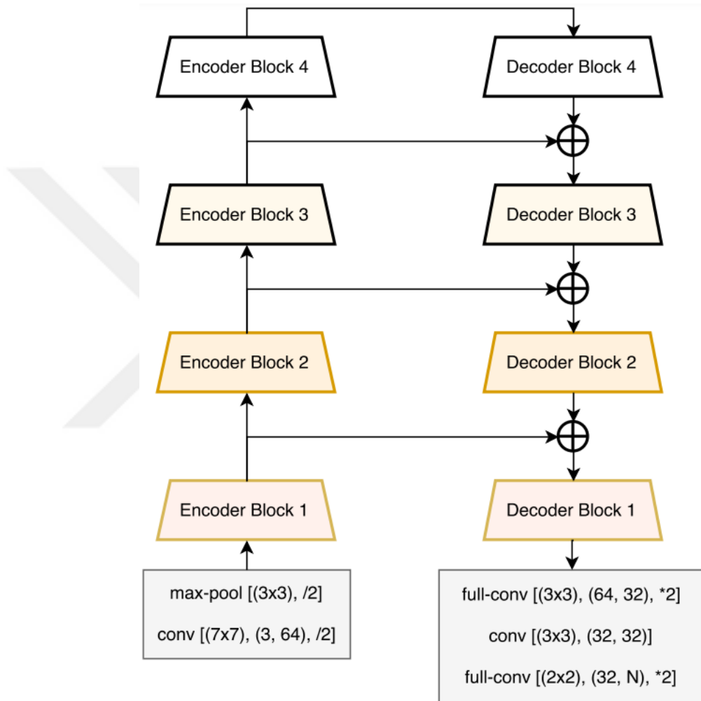
Figure 3.5 Overview of LinkNet architecture (Chaurasia and Culurciello 2017)
