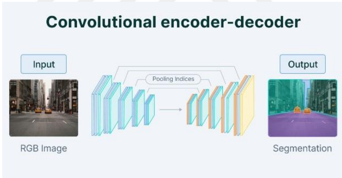
Figure 2.2 Encoder-Decoder base architecture (Bandyopadhyay 2022)
