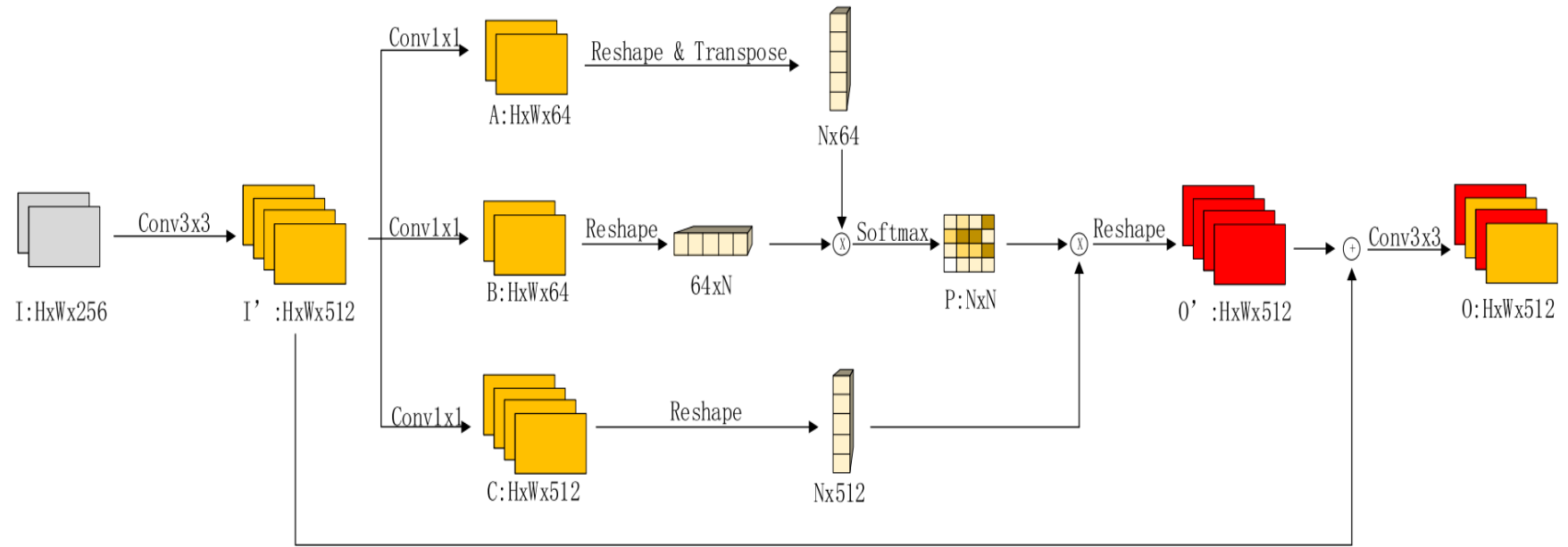
Figure 3.17 Position-wise Attention Block (PAB). While the input image is H \times W \times 256 , the final image is H \times W \times 512 . Finally, the attention feature map is obtained using the softmax function (Fan et al. 2020)
