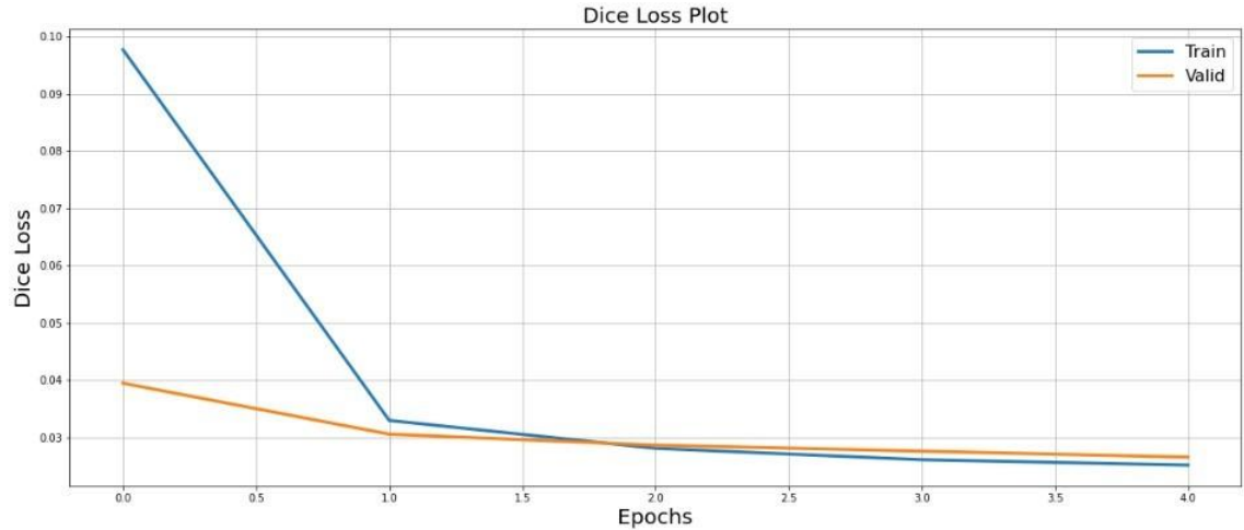
Figure 4.8 Training and validation Dice Loss for 5 epochs using UNet model on DeepGlobe data set and with [-90:90] rotation angles
