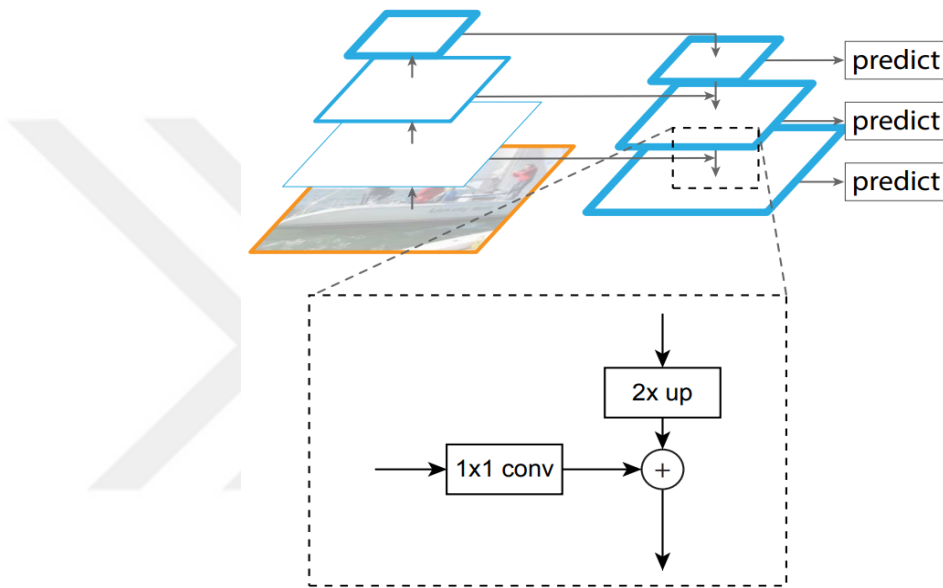
Figure 3.12 A construction block that, by addition, demonstrates both the top-down pathway and the lateral link (Lin et al. 2017)
