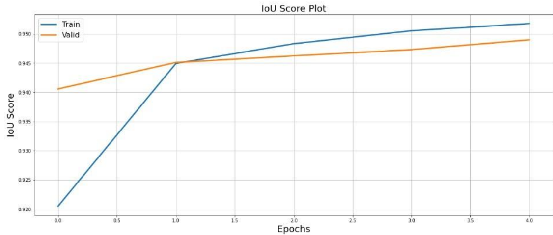
Figure 4.7 Training and validation IoU for 5 epochs using UNet model on DeepGlobe data set and with [-90:90] rotation angles
