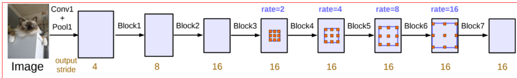
Figure 3.8 Atrous convolution for deeper exploration. When the output stride equals 16, atrous convolution with a rate larger than 1 is used after block 3. Without and with atrousal convolution, cascaded modules (Chen et al. 2017b)
