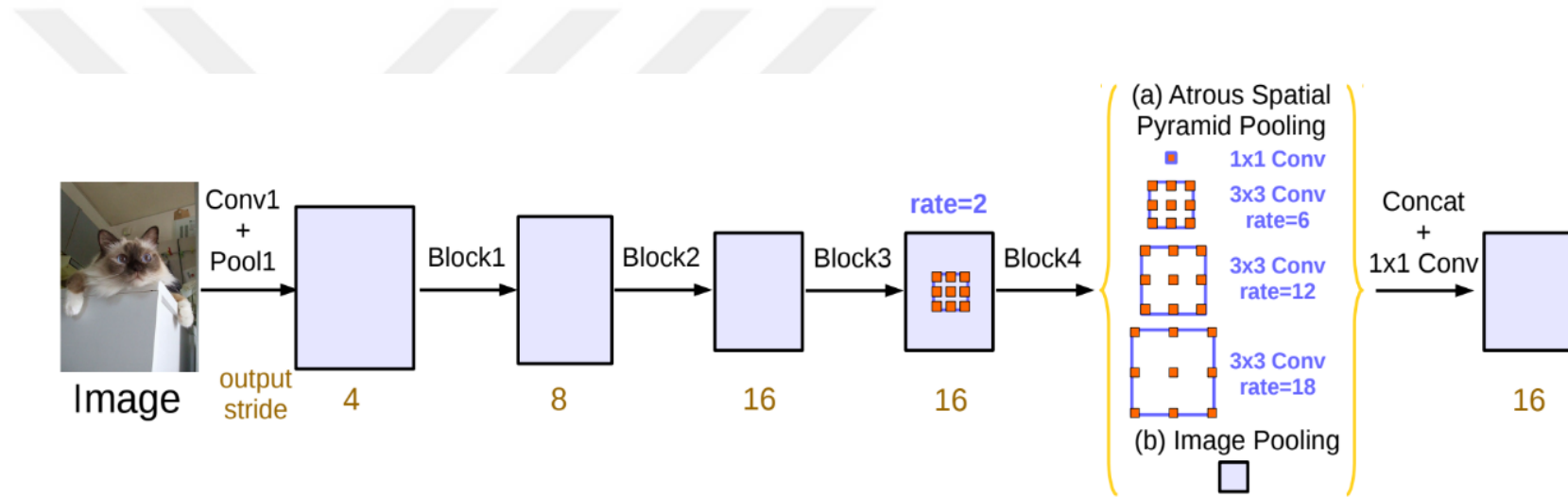
Figure 3.9 Parallel modules with atrous convolution (ASPP), augmented with image-level features (Chen et al. 2017b)
