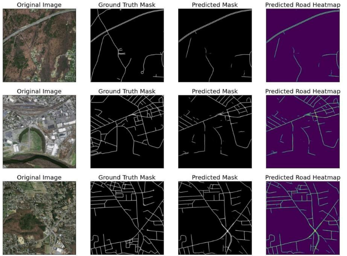
Figure 4.6 Some predicted samples from Massachusetts data set using Pan model
