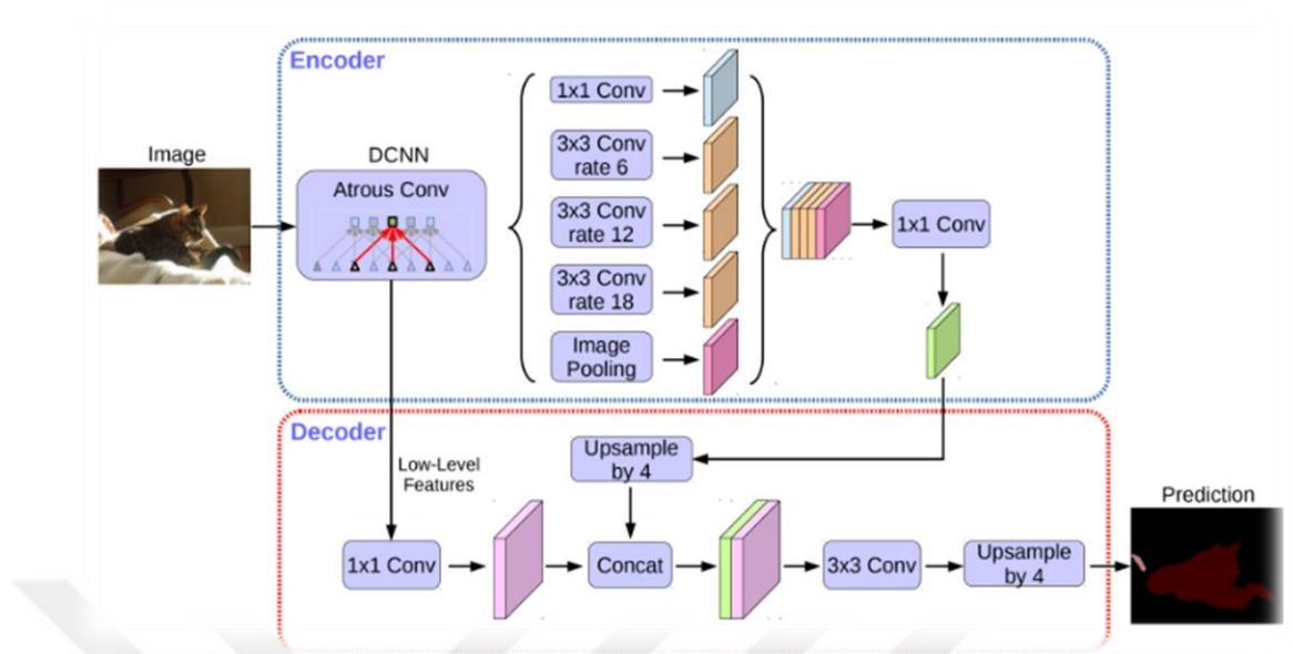
Figure 3.11 The architecture of DeepLab-v3+ segmentation model (Chen et al. 2014)
