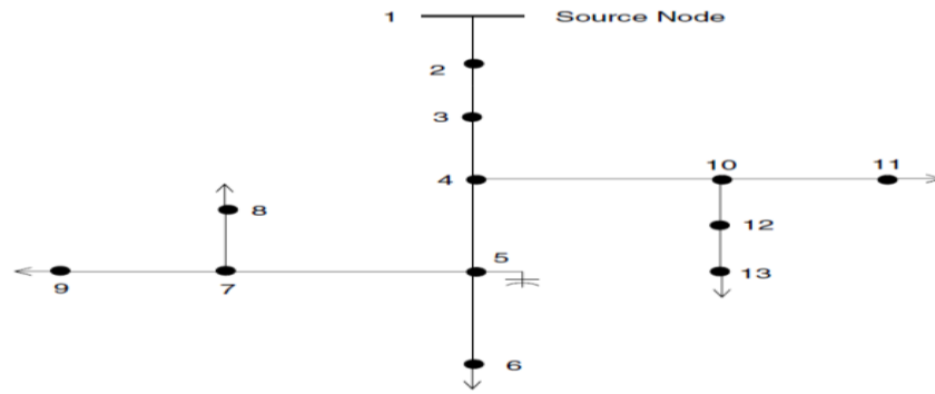
Figure 2.5 Typical feeder
