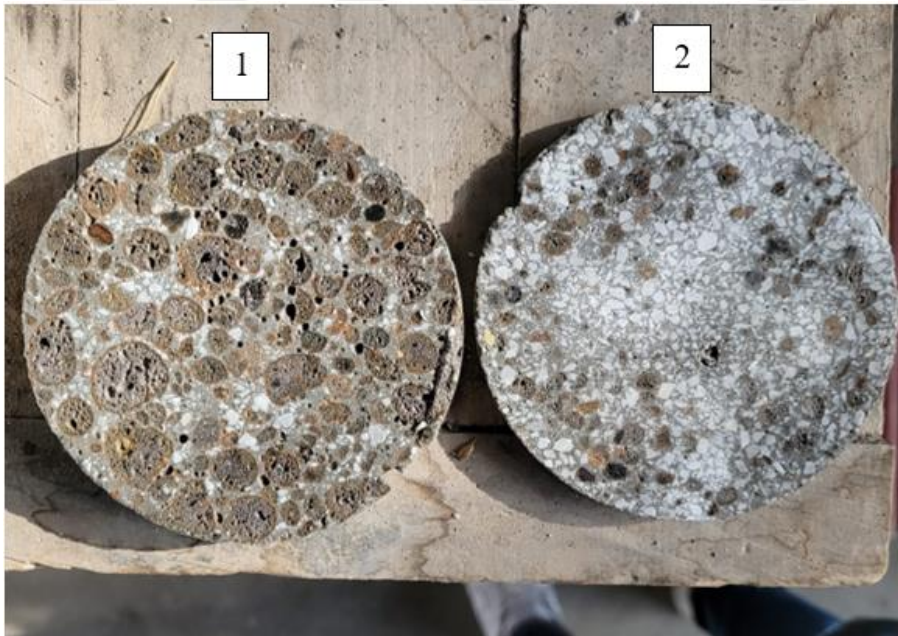
Figure 4.9 Cross Section of Mix #5
