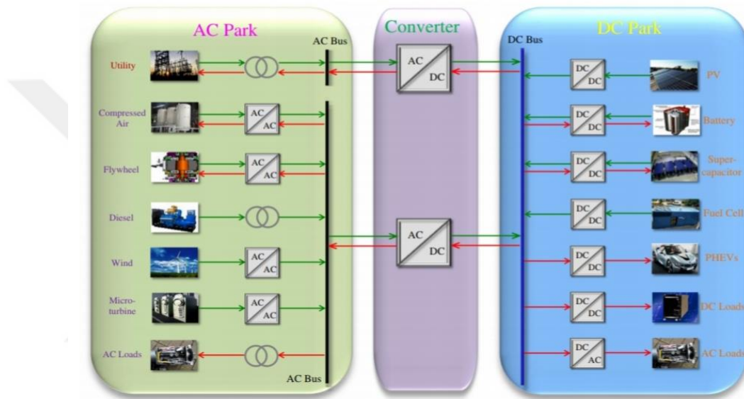
Figure 2.2. Hybrid microgrid typical system structure
