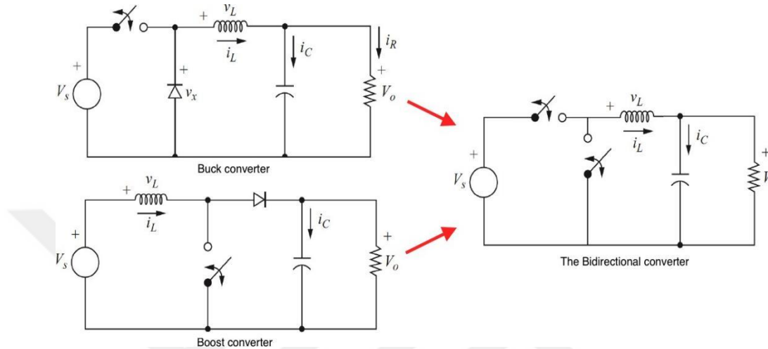
Figure 3.13. Bidirectional converter.
