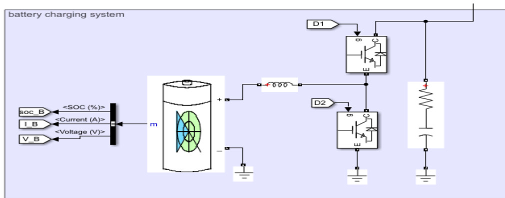
Figure 3.11. Energy storage system.
