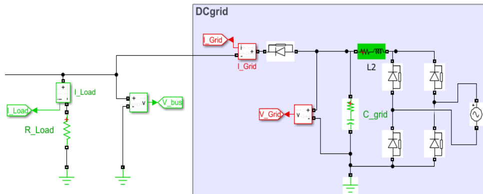
Figure 3.14. DC microgrid.
