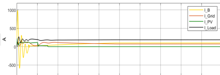
Figure 4.60. System current curves in case of idle PV and full load.
