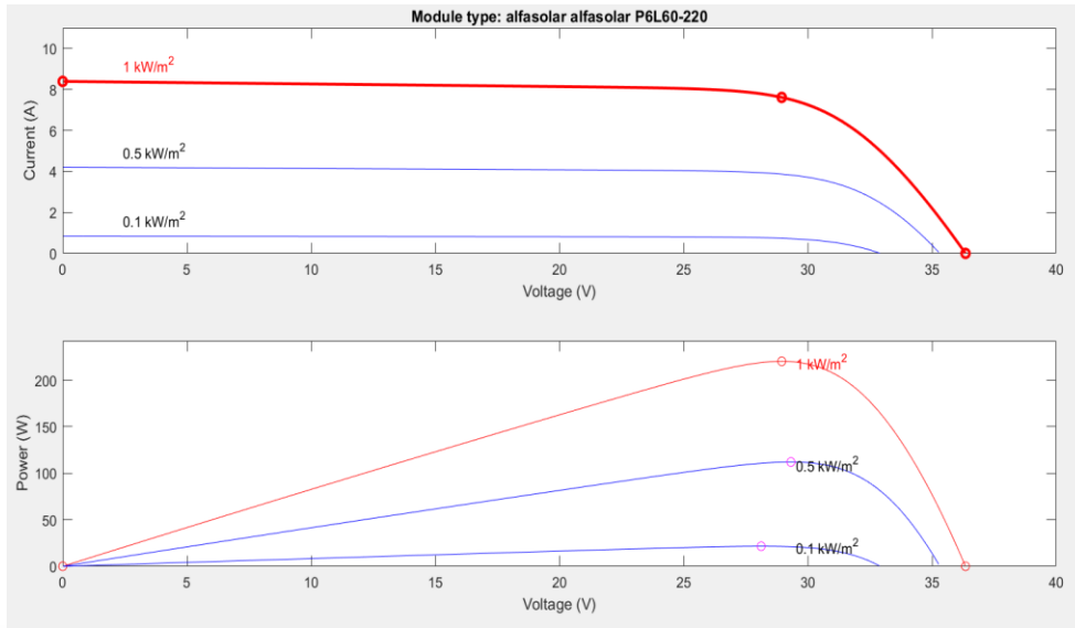
Figure 3.4. P-V & I-V Curves for single module.
