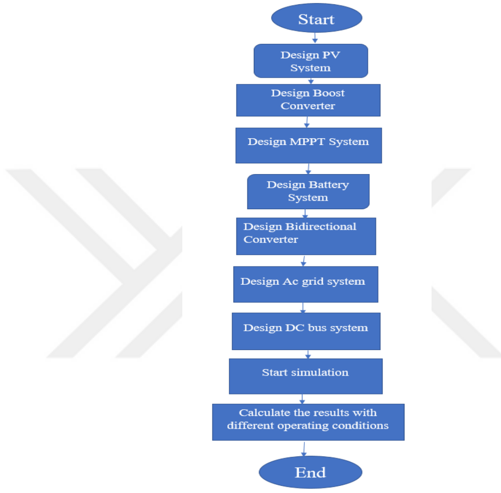
Figure 1.2. Methodology flowchart.
