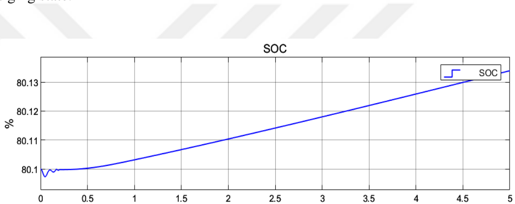
Figure 4.19. Battery SOC curve in case of 500 W/m 2 and 25% full load.
