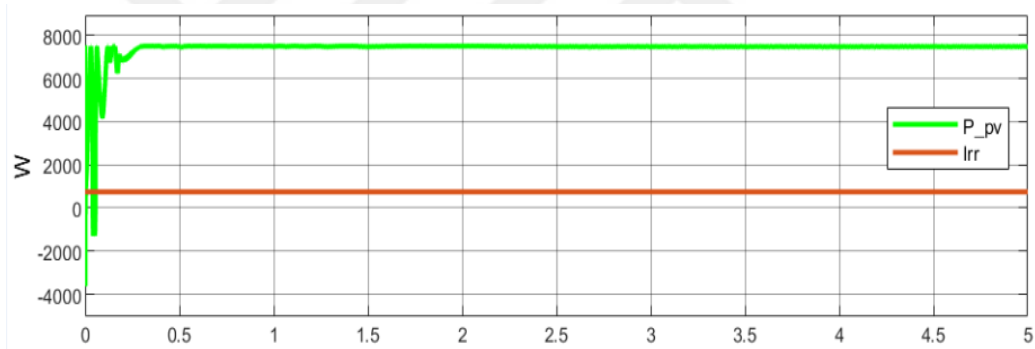
Figure 4.32. MPPT performance in case of 750 w/m 2 and 25% full load.
