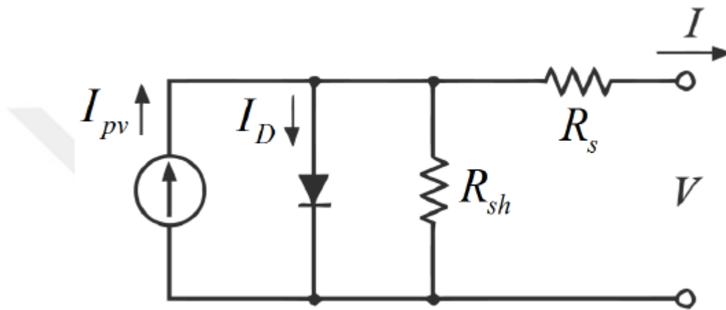
Figure 3.2. Equivalent model of single-diode photovoltaic cell.
