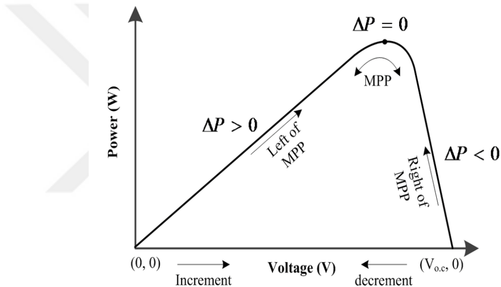
Figure 3.7. P&O MPPT working curve
