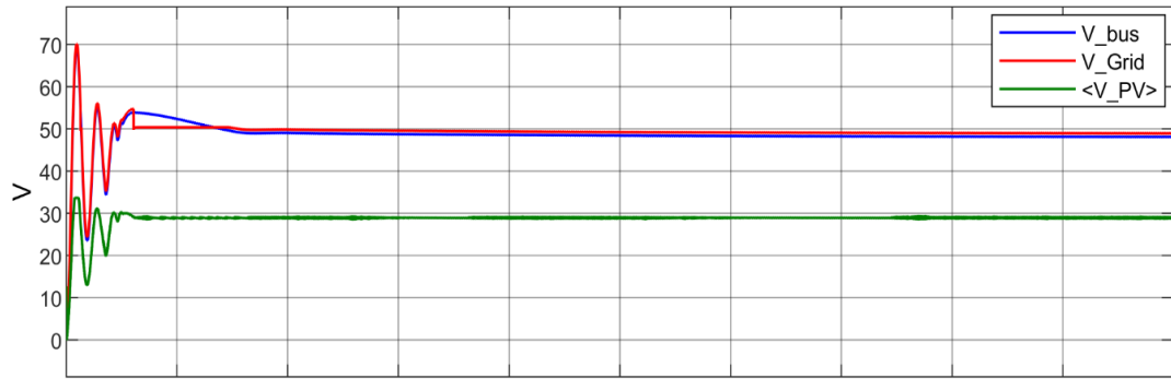
Figure 4.1. System voltages in case of 250 W/m 2 radiation level and 25% full load.
