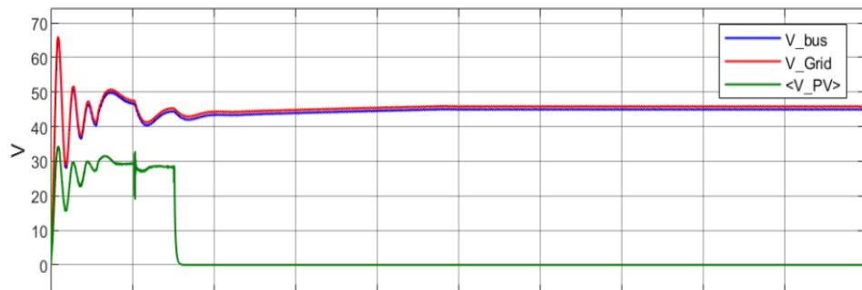
Figure 4.59. System voltage curves in case of idle PV and full load
