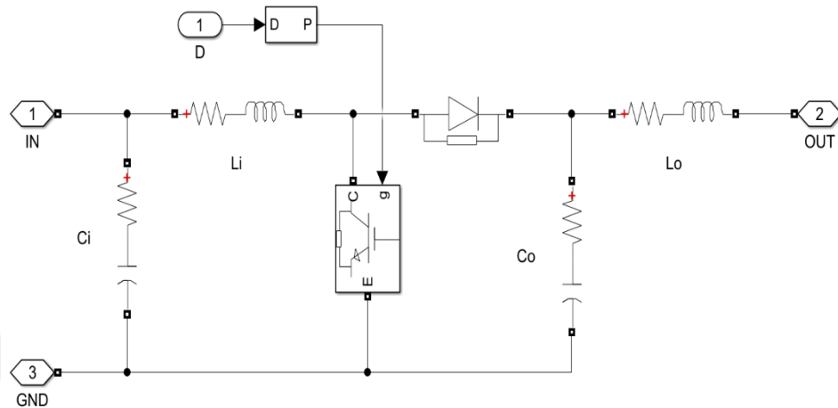
Figure 3.9. Boost converter.
