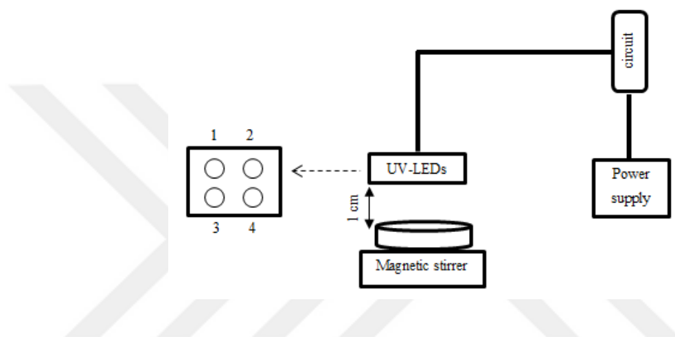
Figure 3.3. Static UV-LED unit
