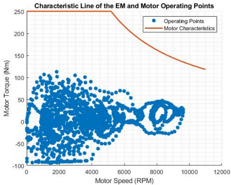
Figure 3.4: Simulation output of motor operating points.
