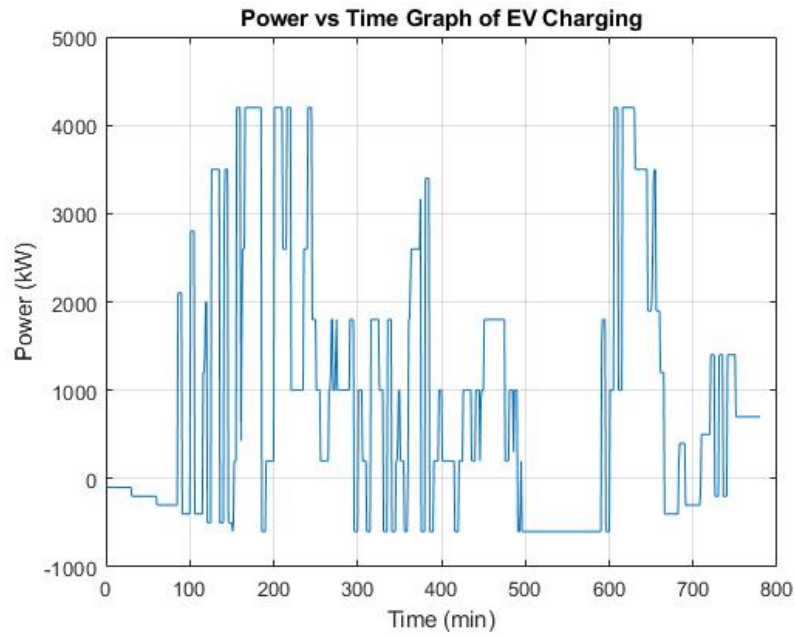
Figure 4.13: EV charging power vs time graph with optimization (V2G introduced).
