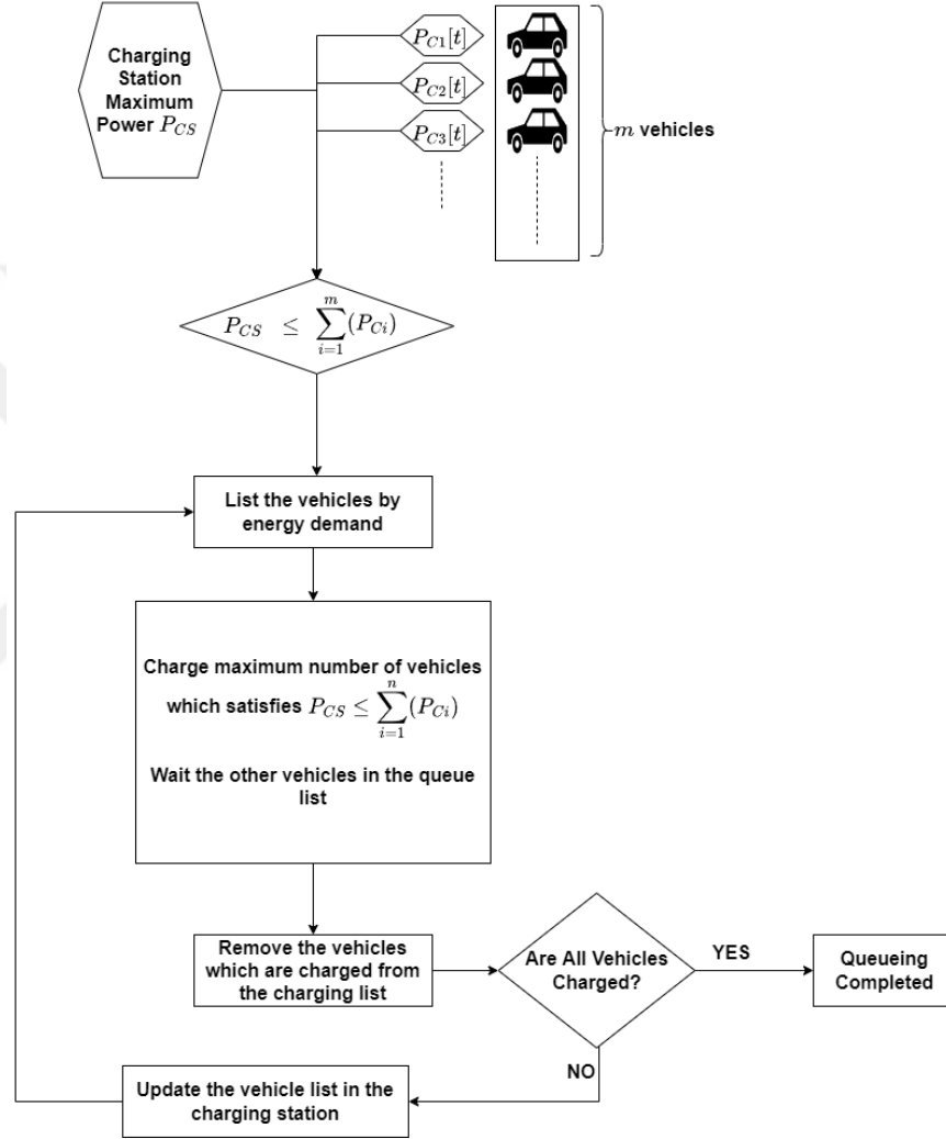
Figure 4.1: Overall Flowchart of the Proposed Queueing Algorithm
