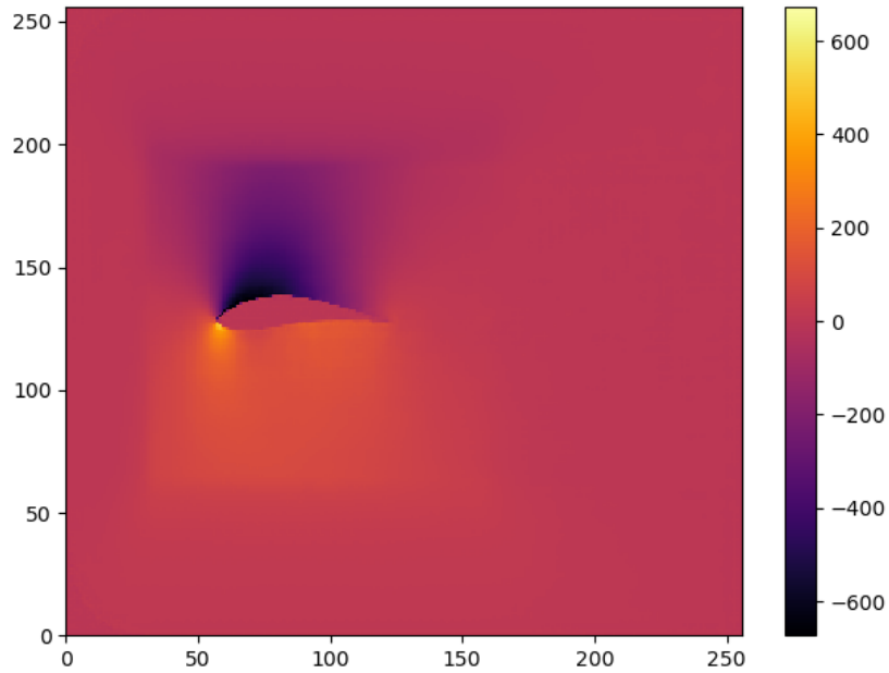
Figure A.3: P ; Pressure component of the predicted field.
