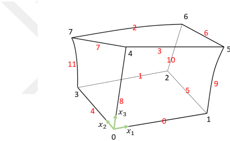
Figure 3.2: Ordering for mapping from a hexagon to a blockMesh block. The Black integers represent vertex numbering and the Red integers show the edge numbers. A block is represented in the code by ordering the vertices in accordance with the numbering presented above. The edges then are automatically assigned between the vertices in the presented order. Note that the edges represent curves rather than straight lines and thus are arc-length parameterized.
