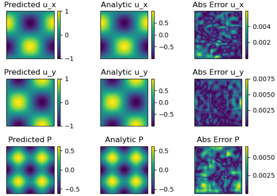
Parametric PINN results at time 0.6 s.
