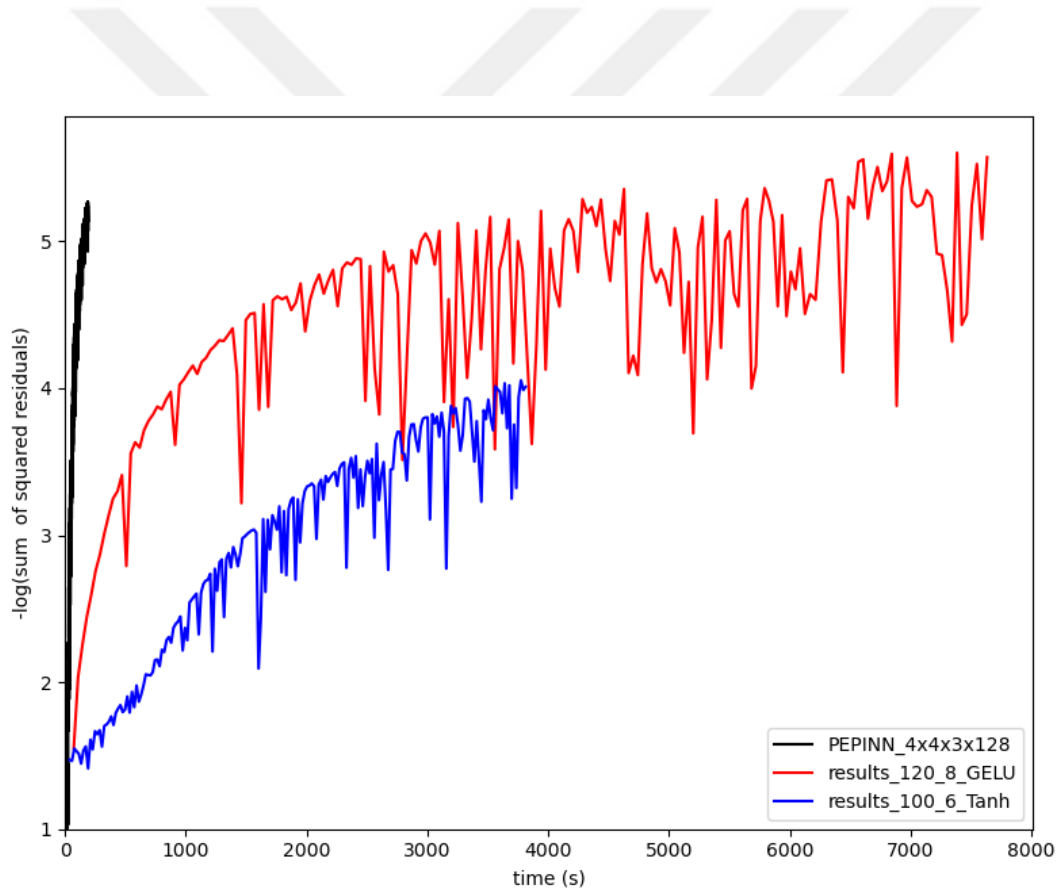
Figure 2.7: Comparison of the PEPINN with signature 4 \times 4 \times 3 \times 128 with baseline model and the model used in [62] when a query points permutation of size 16 \times 32 \times 32 is provided to baseline models and maximum query points permutation of size 16 \times 32 \times 32 is provided for the PEPINN model during 20000 iterations.
