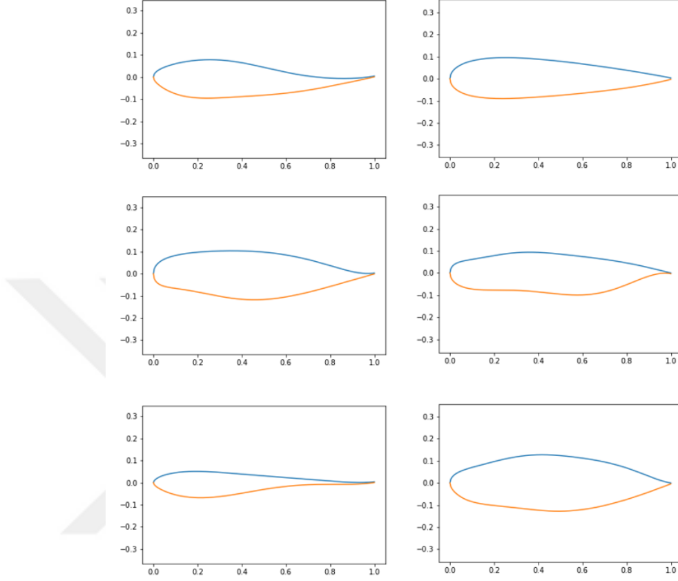
Figure 3.1: First 6 airfoils out of 1000 generated airfoils using CST method. It can be observed that even in this small subset of the generated airfoils some are similar to the airfoils used in practical applications while others are just airfoil-like shapes that might be impractical to use in engineering applications. Yet even in this limited number of cases a large range of variations in shape is present.
