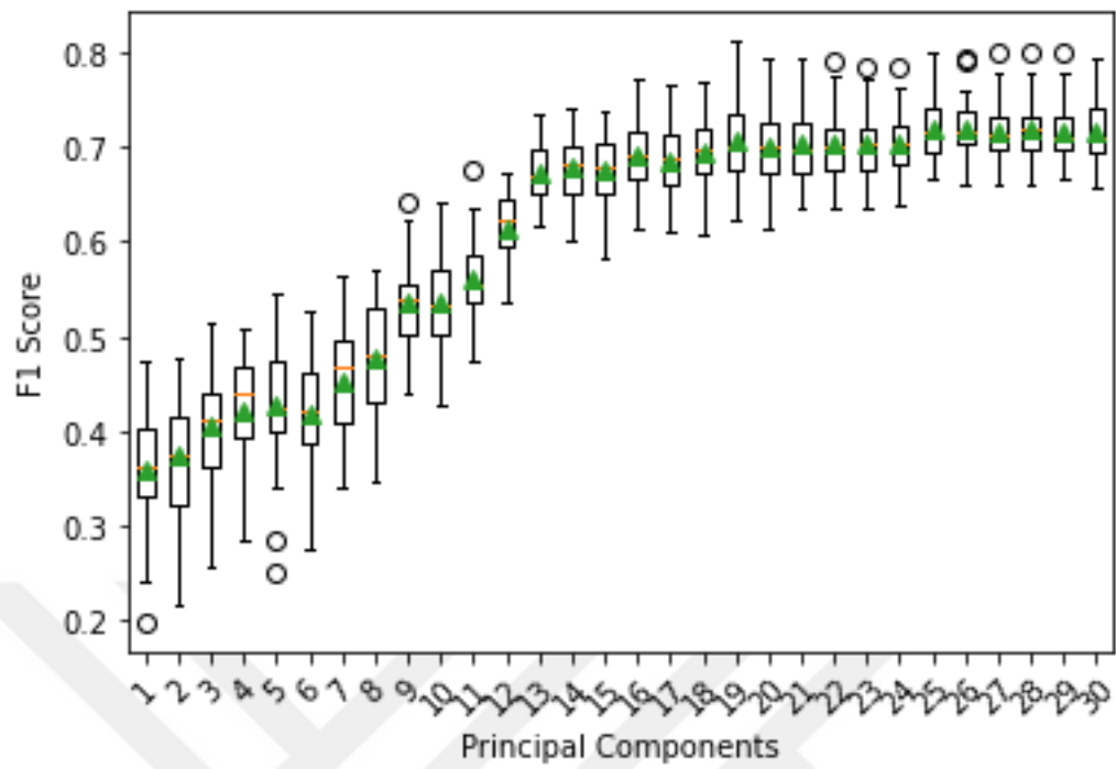
Figure 4.3 Box Plot of the Grid Search Results for the Number of Components That Yields the Best F1 Score
