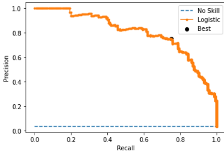
Figure 5.1 Precision - Recall Curve for Model 1
