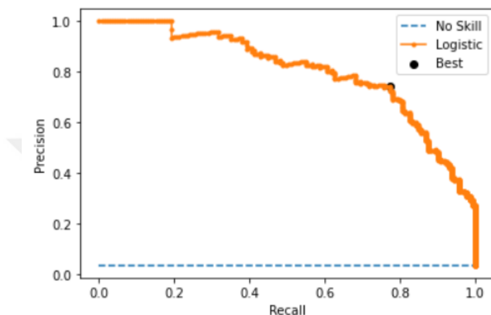
Figure 5.9 Precision – Recall Curve for Model 5
