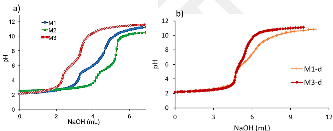
Figure 3.5. Titration curves of macromers.
