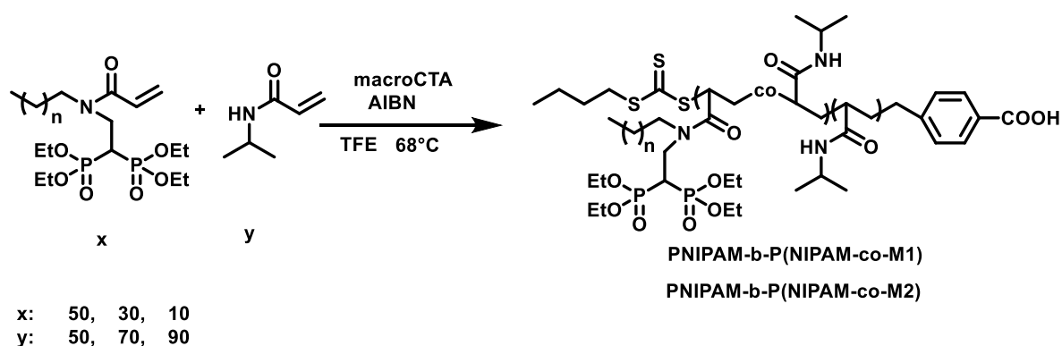
Figure 5.12. Synthesis of block copolymers (PNIPAM-b-P(NIPAM-co-M x )).
