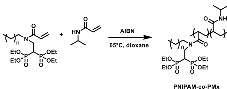
Figure 5.6. Synthesis of P(NIPAM-co-Mx) by FRP.
