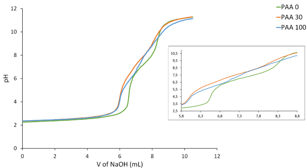
Figure 4.5. Acid–base titration curves of the 1 mg/mL aqueous solutions of PAA0, PAA30, and PAA100.
