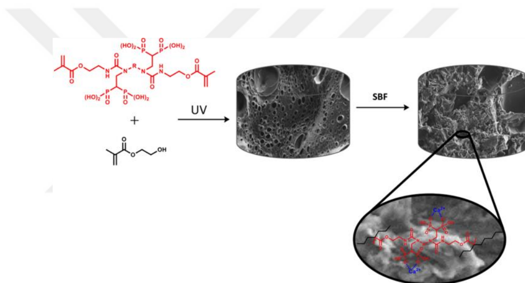
Figure 1.17. SEM images of bisphosphonic acid-functionalized dimethacrylate crosslinked HEMA hydrogels. Reprinted from [163]. (Further permission related to figure excerpted should be directed to ACS).
