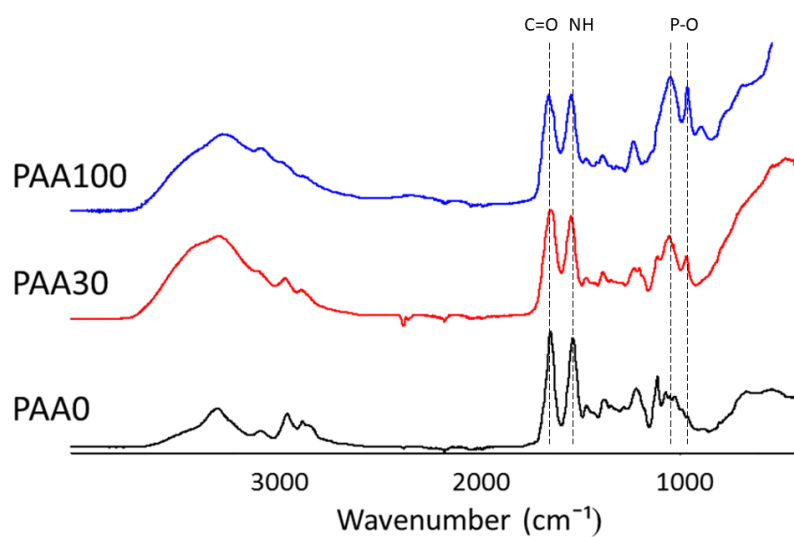
Figure 4.3. FTIR spectra of PAA0, PAA30 and PAA100.
