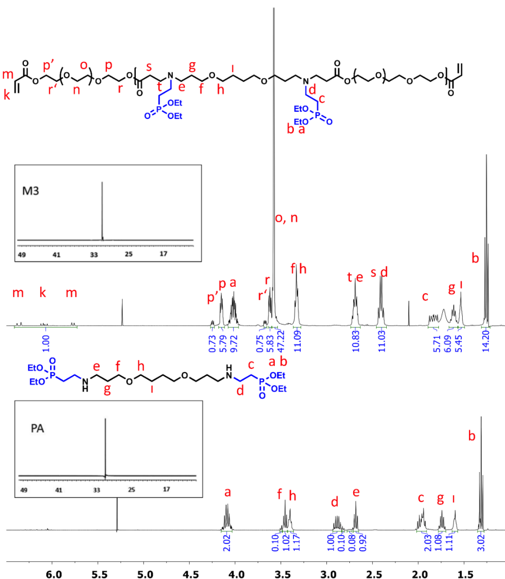
Figure 3.2. ^1\text{H} NMR spectra of PA and M3 (PEGDA:PA mol ratio of 1.1:1).
