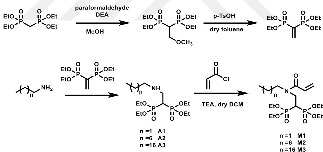
Figure 5.3. Synthesis of bisphosphonate functionalized amines (Ax) and acrylamides (Mx).
