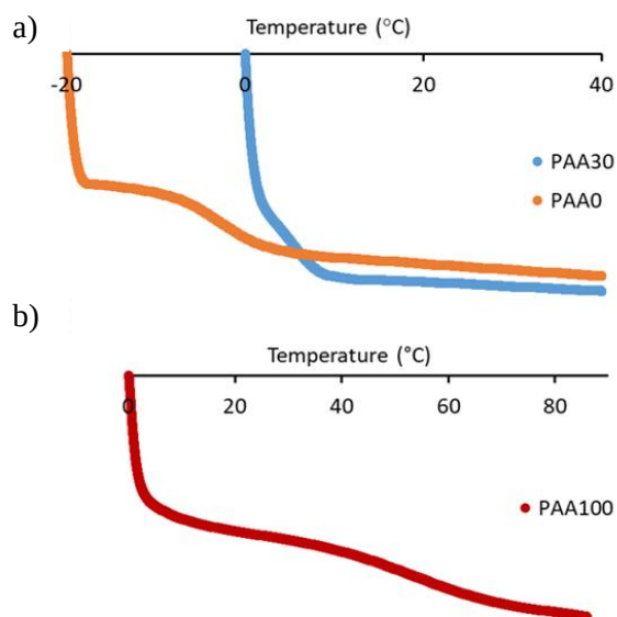
Figure 4.4. DSC curves of PAA macromers (a) PAA30 and PAA0 and (b) PAA100.
