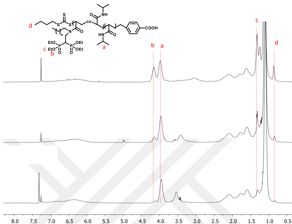
Figure 5.13. ^1\text{H} NMR spectra of the copolymers \text{PNIPAM}_{200}\text{-b-(NIPAM}_y\text{-co-M2}_x) y:x 45:5, 35:15, 50:50 respectively from bottom to top.
