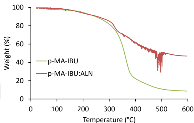
Figure 6.4. TGA thermogram of p-MA-IBU p-MA-IBU:ALN.
