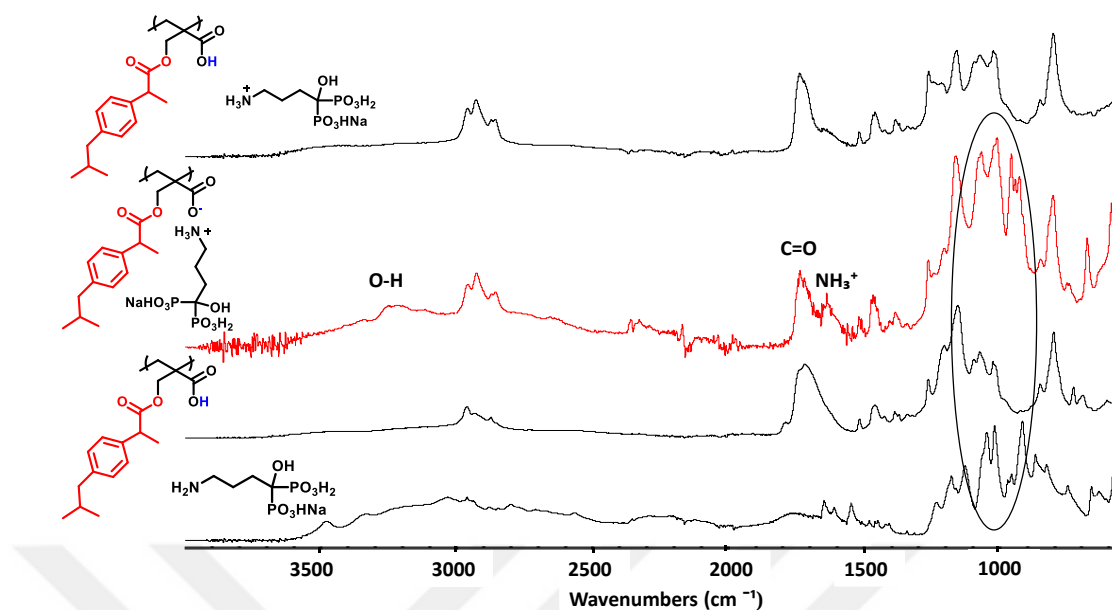
Figure 6.2. FT-IR spectra of p-MA-IBU:ALN at pH 3, p-MA-IBU:ALN, ALN (top to bottom).
