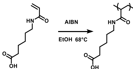
Figure 6.7. Synthesis of PAHA.
