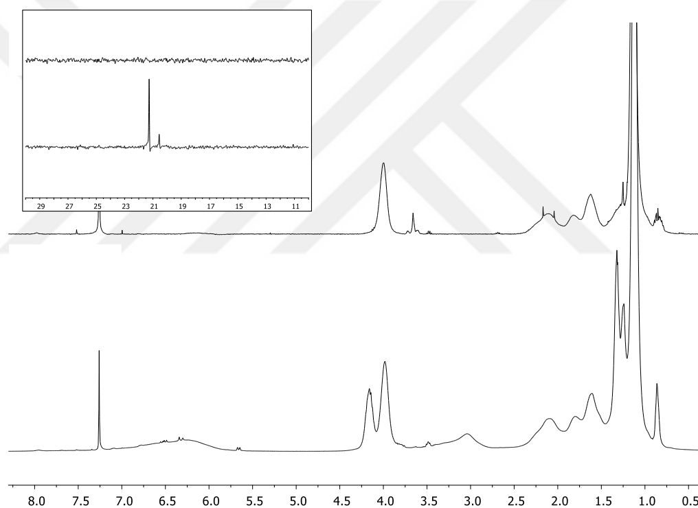
Figure 5.15. ^1\text{H} NMR and ^{31}\text{P} NMR spectra of the polymer before (below) and after (above) dealkylation.
