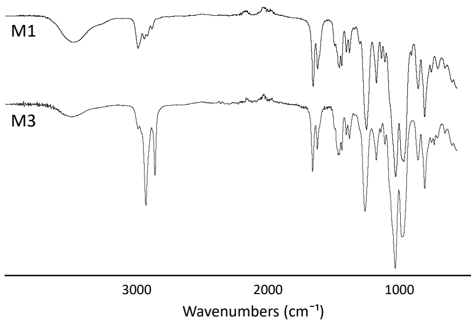
Figure A.6. FTIR spectra of acrylamide monomers M1 and M3.
