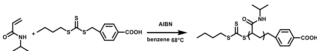
Figure 5.8. Synthesis of PNIPAM by RAFT polymerization.
