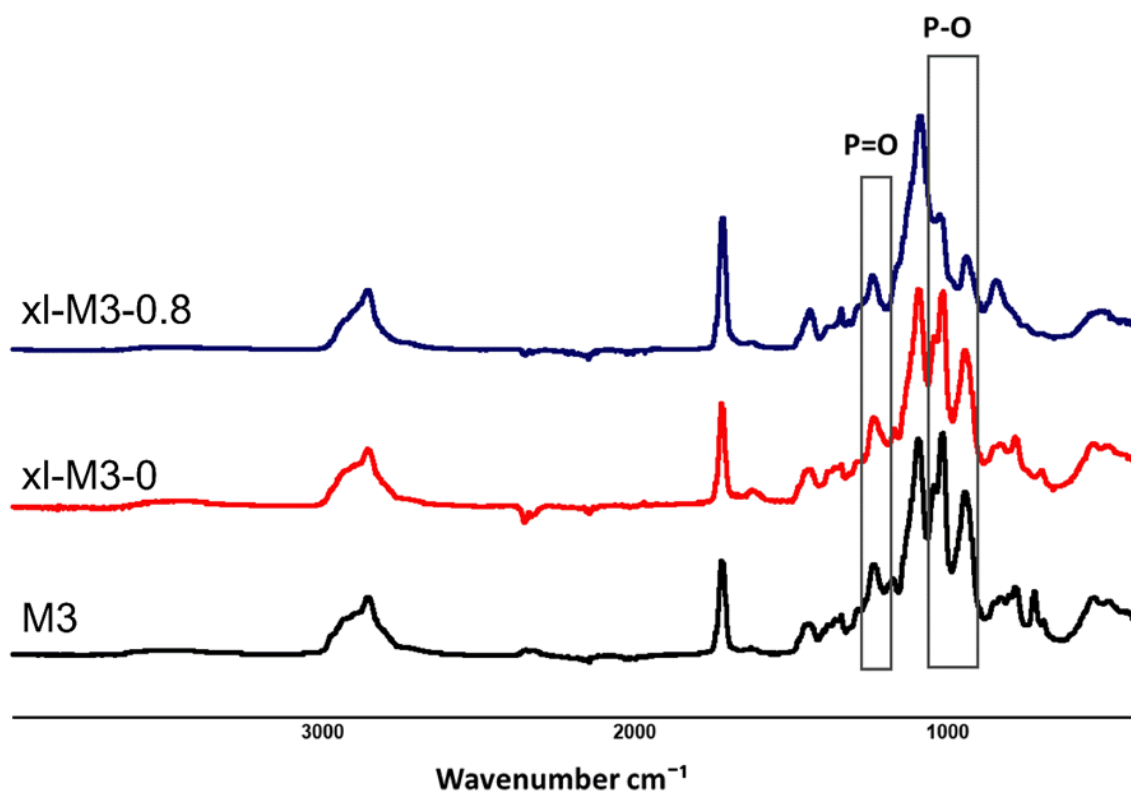
Figure 3.3. FTIR spectra of M3, xl-M3-0 and xl-M3-0.8.
