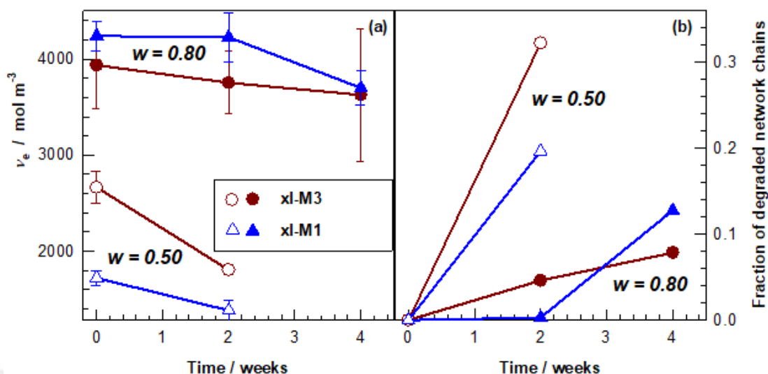
Figure 3.13. The cross-link density \nu_e of the hydrogels (a) and the fraction of degraded network chains, 1 - \nu_e / \nu_{e,0} , (b) both plotted against the degradation time. Empty symbols: w = 0.5 , filled symbols: w = 0.8 .
