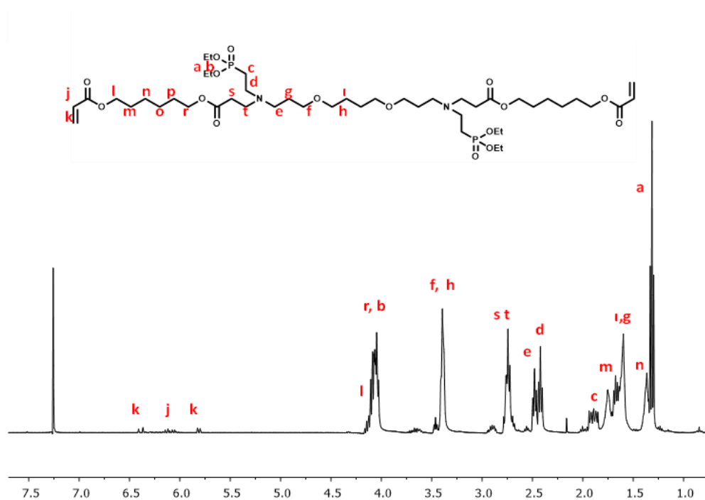
Figure A.2. ^1\text{H} NMR spectrum of macromer M1.
