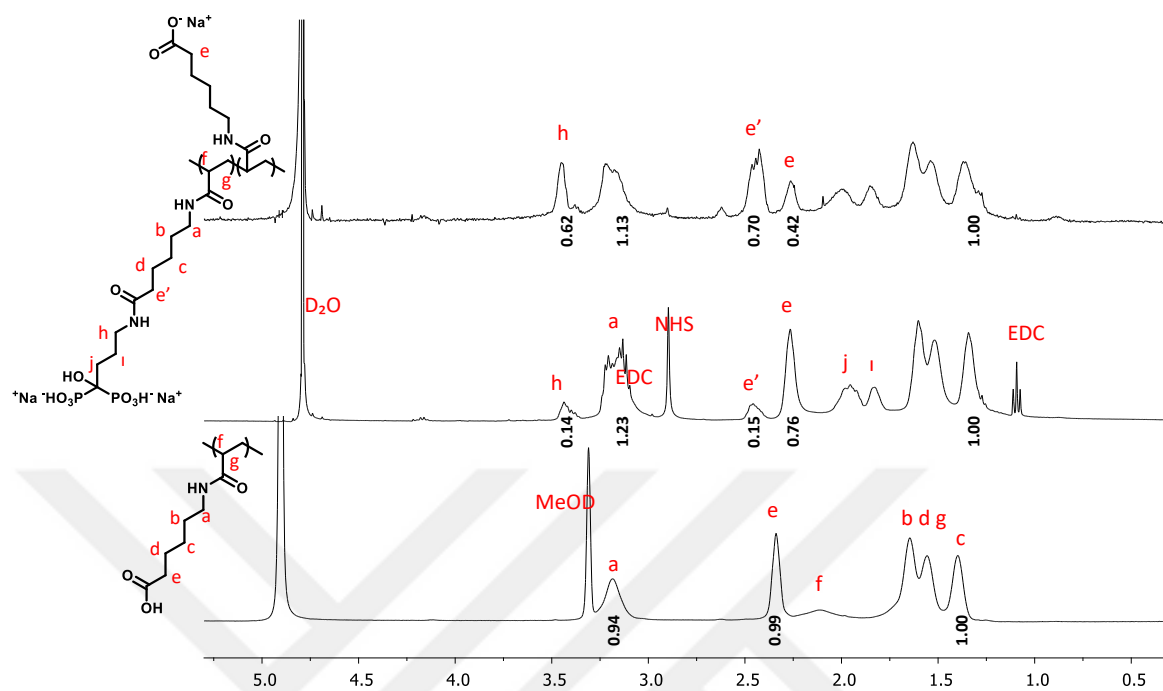
Figure 6.8. ^1\text{H} NMR spectra of PAHA and ALN-PAHA.
