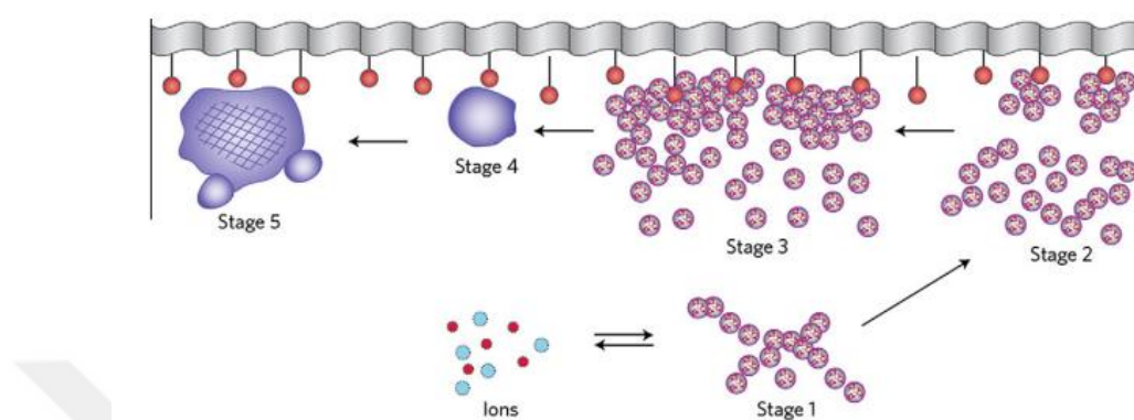
Figure 1.16. Representation of calcium phosphate nucleation and growth on anionic group functionalized surfaces. Reprinted from [144].
