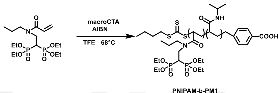
Figure 5.10. Synthesis of diblock copolymer of NIPAM and M1.
