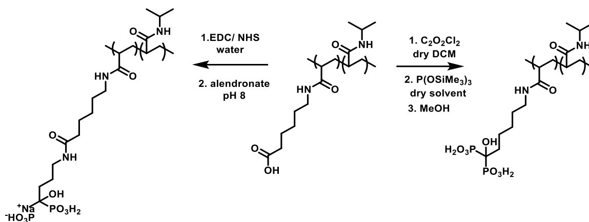
Figure 5.18. Synthesis of tmsp-P(NIPAM-co-AHA) and ale-P(NIPAM-co-AHA).
