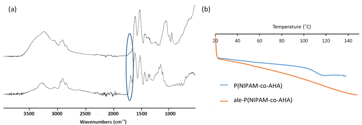
Figure 5.20. (a) FTIR spectra of ale-P(NIPAM-co-AHA) (above) and P(NIPAM-co-AHA) (below) (b) DSC curves of copolymers.
