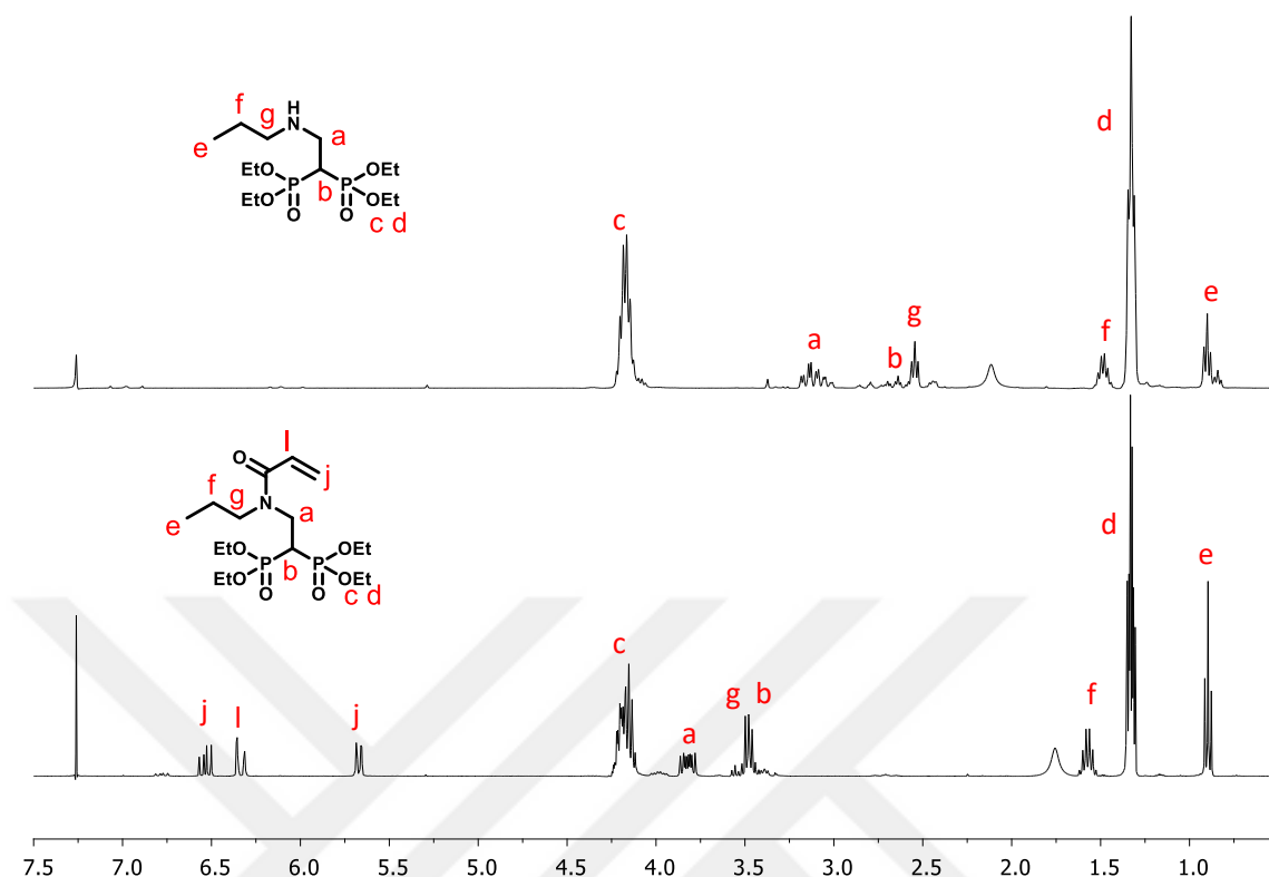
Figure 5.4. ^1\text{H} NMR of A1 and M1.
