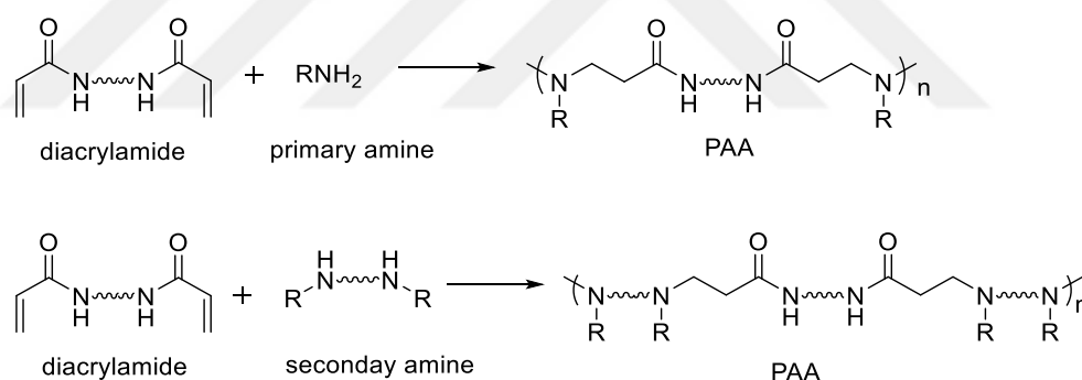
Figure 1.4. Synthesis of PAAs.
