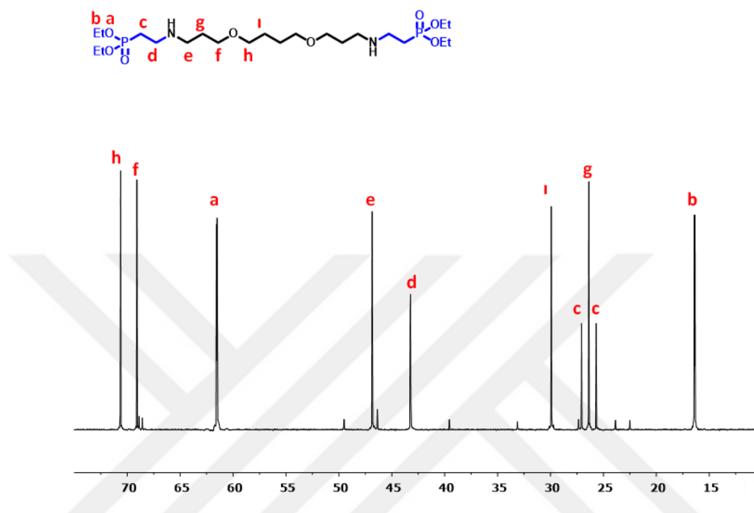
Figure A.1. ^{13}\text{C} NMR spectrum of PA.
