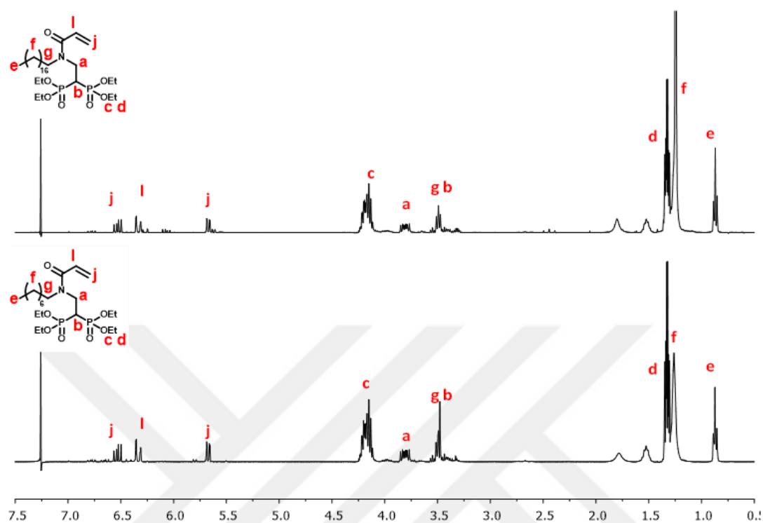
Figure A.5. ^1\text{H} NMR spectra of acrylamide monomers M2 and M3.
