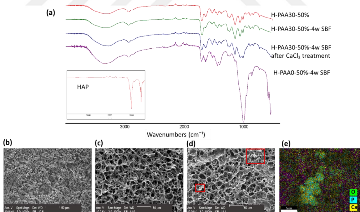
Figure 4.8. (a) FTIR spectra of H-PAA30-50% before (top); and H-PAA30-50% and H-PAA0-50%, treated as labeled, with HAP inset, (b–d) SEM micrographs of the top three cases listed in (a), in order, (e) \times 8000 and mapped image of (d).
