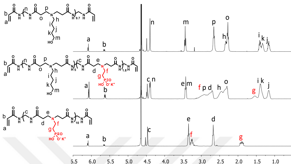
Figure 4.2. ^1\text{H} -NMR spectra of PAA0, PAA30 and PAA100.
