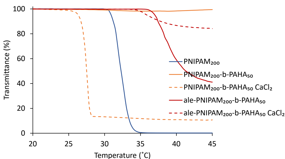
Figure 5.22. Turbidimetry studies of \text{PNIPAM-b-PAHA} .
