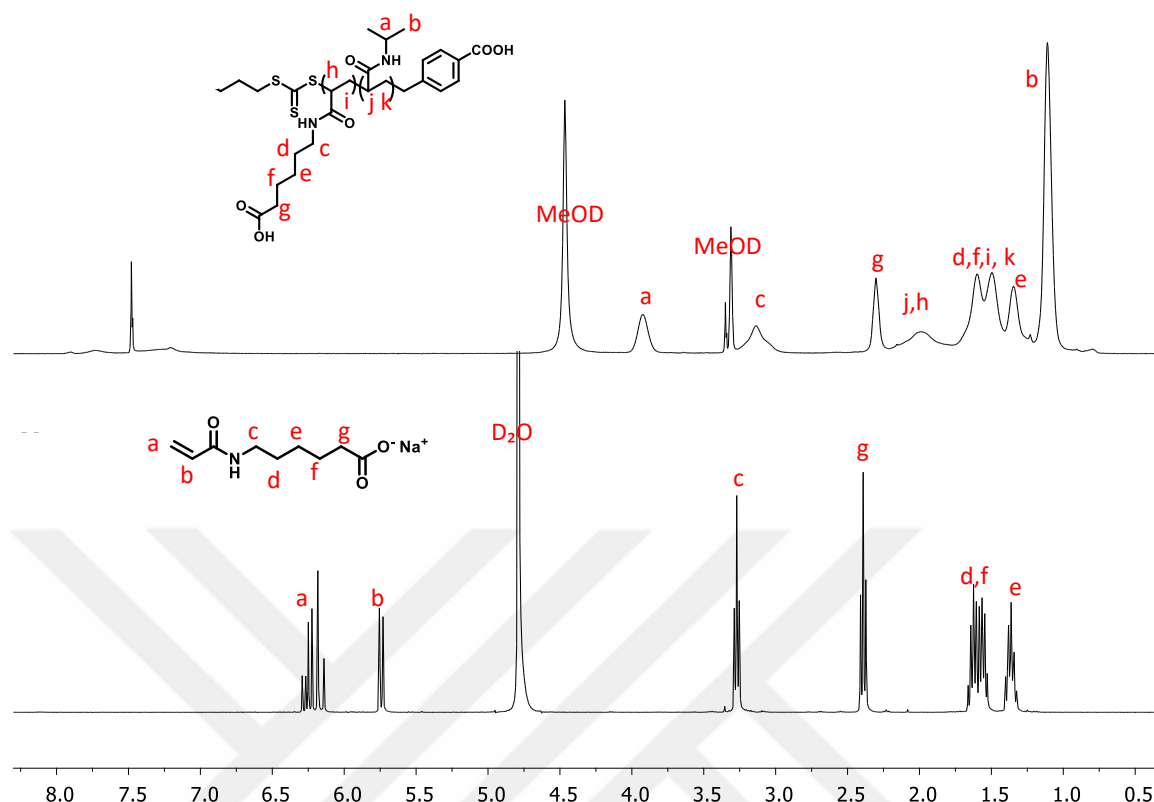
Figure 5.17. ^1\text{H} NMR spectra of AHA monomer and PNIPAM-b-PAHA.
