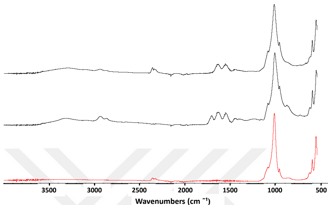
Figure 6.13. FTIR spectra of ALN-PAHA:HAP, PAHA:HAP and HAP (from top to bottom).
