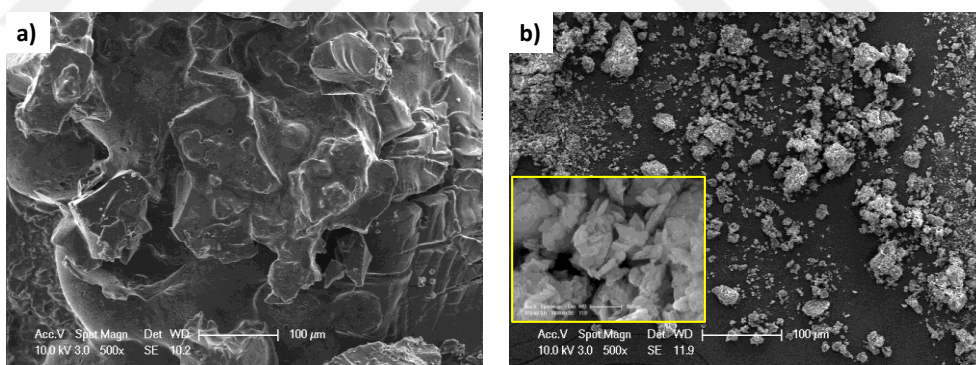
Figure 6.3. SEM micrographs of (a) p-MA-IBU and (b) p-MA-IBU:ALN.
