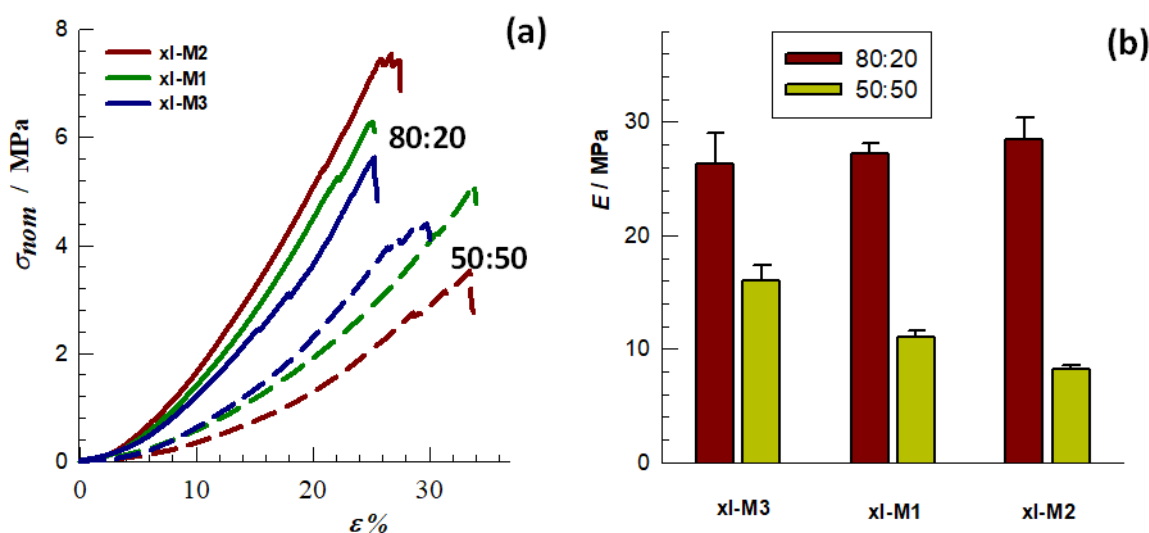
Figure 3.11. (a) Stress-strain curves of the gels at w = 0.80 (solid curves) and 0.50 (dashed curves). (b) Young's moduli E of the gels formed at w = 0.80 (dark red) and 0.50 (dark yellow).
