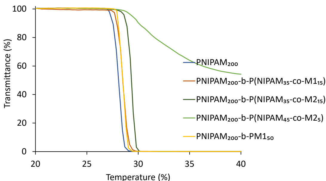
Figure 5.21. Turbidimetry studies of block copolymers of NIPAM and Mx.
