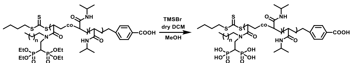
Figure 5.14. TMSBr dealkylation of block copolymers.
