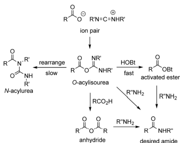
Figure 6.10. Mechanism of amidation via activated esters.
