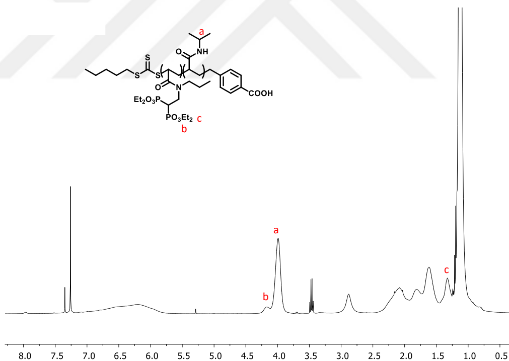
Figure 5.11. ^1\text{H} NMR spectrum of PNIPAM-b-PM1.
