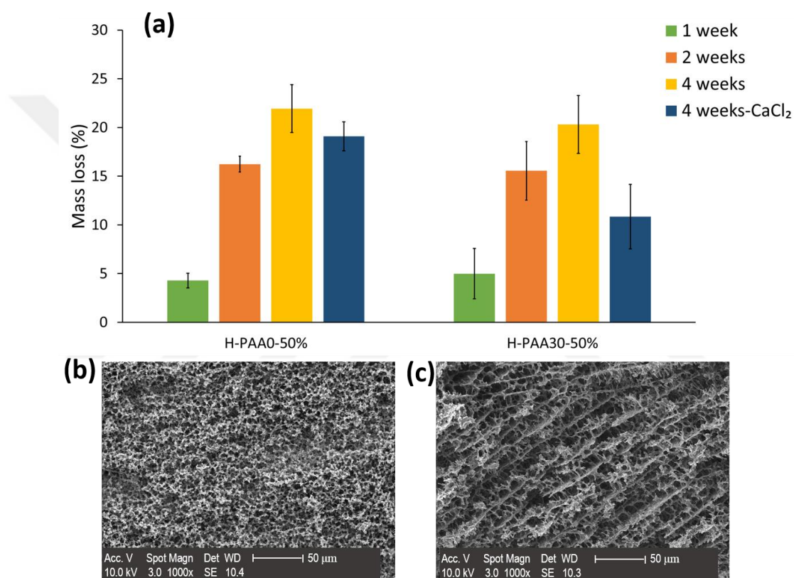
Figure 4.7. (a) The degradation of H-PAA0-50% and H-PAA30-50% hydrogels in pH 7.4; (b) SEM micrographs of H-PAA30-50%, (b) before and (c) after 4 weeks degradation.
