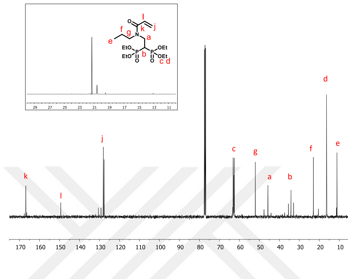
Figure 5.5. ^{13}\text{C} and ^{31}\text{P} NMR of M1.
