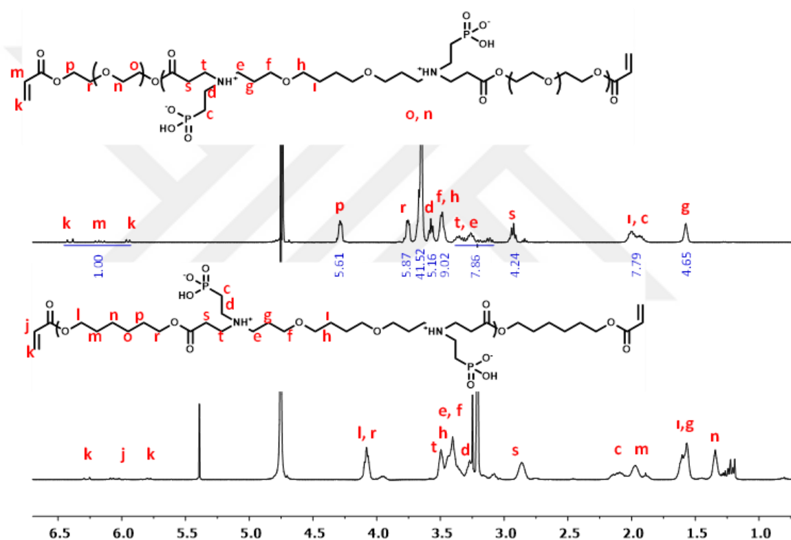
Figure 3.4. ^1\text{H} NMR spectra of M1-d and M3-d.
