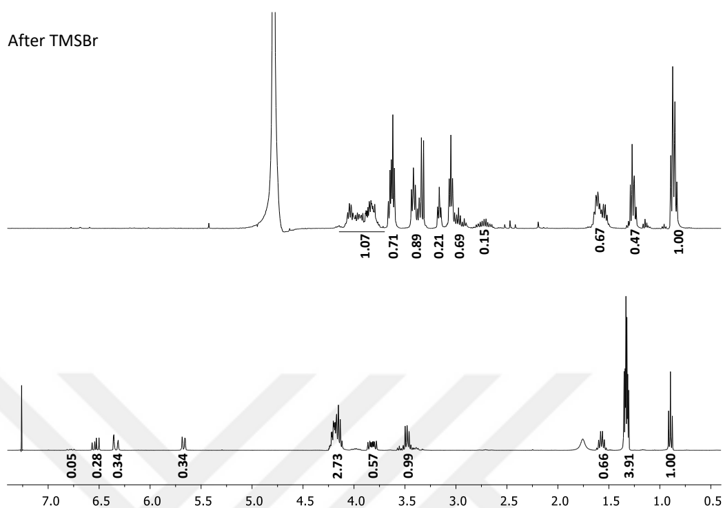
Figure A.7. ^1\text{H} NMR and integrals of M1 before and after TMSBr dealkylation.
