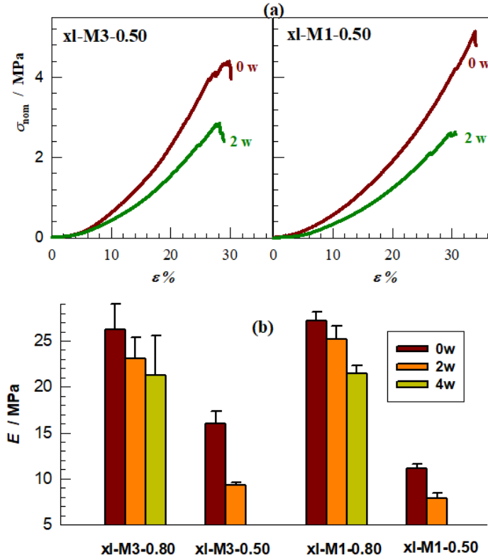
Figure 3.12. (a) Typical stress-strain curves of virgin and 2 weeks-degraded xl-M3 and xl-M1 gels formed from PEGDA and HDDA, respectively. w = 0.50 . (b) The modulus E of gels at various degradation times.
