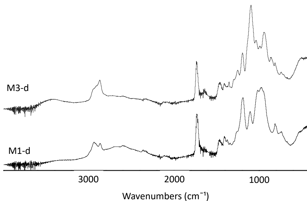
Figure A.4. FTIR spectra of dealkylated macromers M1-d and M3-d.
