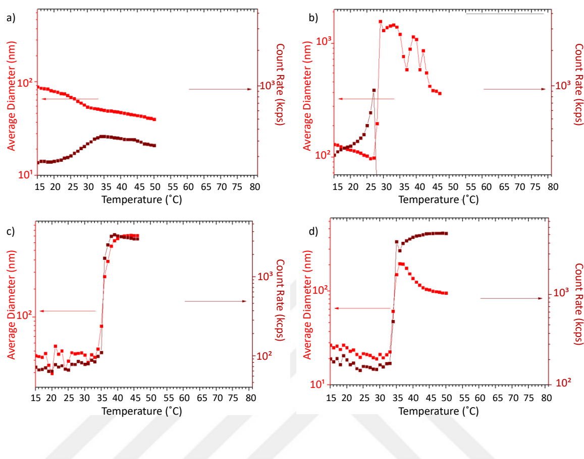
Figure 5.23. Average diameter and count rate vs temperature graphs of 10 g/L solutions of PNIPAM 200 -b-PAHA 100 (above) and ale-PNIPAM 200 -b-PAHA 100 (below) (a,c) in water and (b, d) in 0.02 M CaCl 2 solution.
