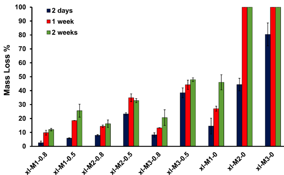
Figure 3.7. The mass loss of PBAE gels and PEGDA-PBAE copolymers in 2 days, 1 week and 2 weeks in PBS.
