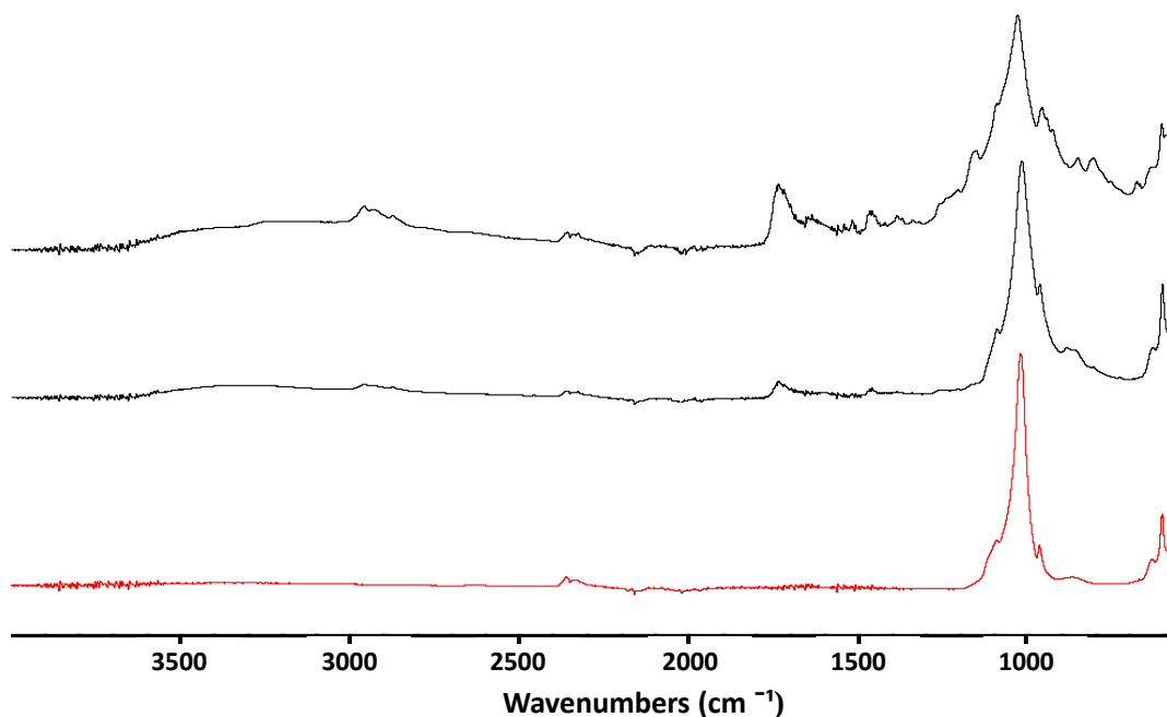
Figure 6.5. FTIR spectra of p-MA-IBU:ALN:HAP, p-MA-IBU:HAP and HAP (from top to bottom).
