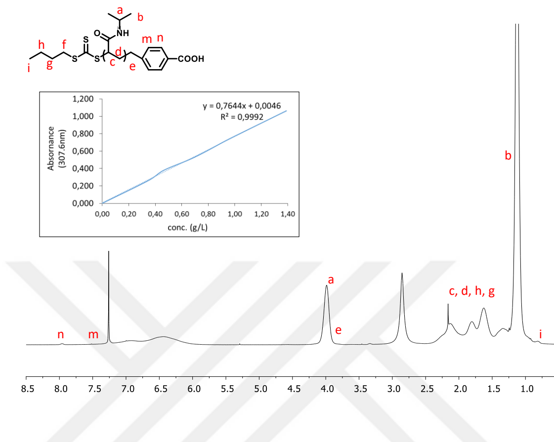
Figure 5.9. ^1\text{H} NMR spectrum and UV-vis measurements of PNIPAM.
