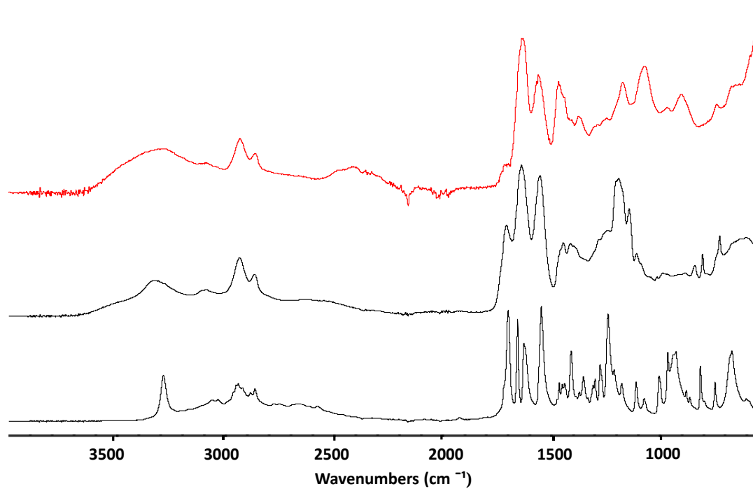
Figure 6.9. FTIR spectra of ALN-PAHA, PAHA and AHA (from top to bottom).
