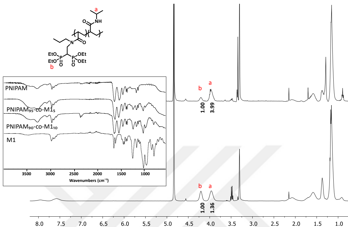
Figure 5.7. ^1\text{H} NMR spectra of \text{P}(\text{NIPAM}_{90}\text{-co-M1}_{10}) and \text{P}(\text{NIPAM}_{95}\text{-co-M1}_5) . FTIR spectra of copolymers and M1.
