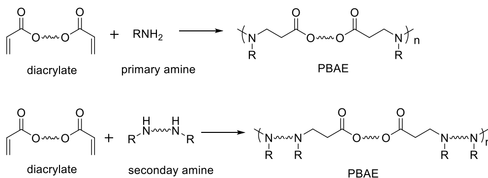
Figure 1.3. Synthesis of PBAEs.
