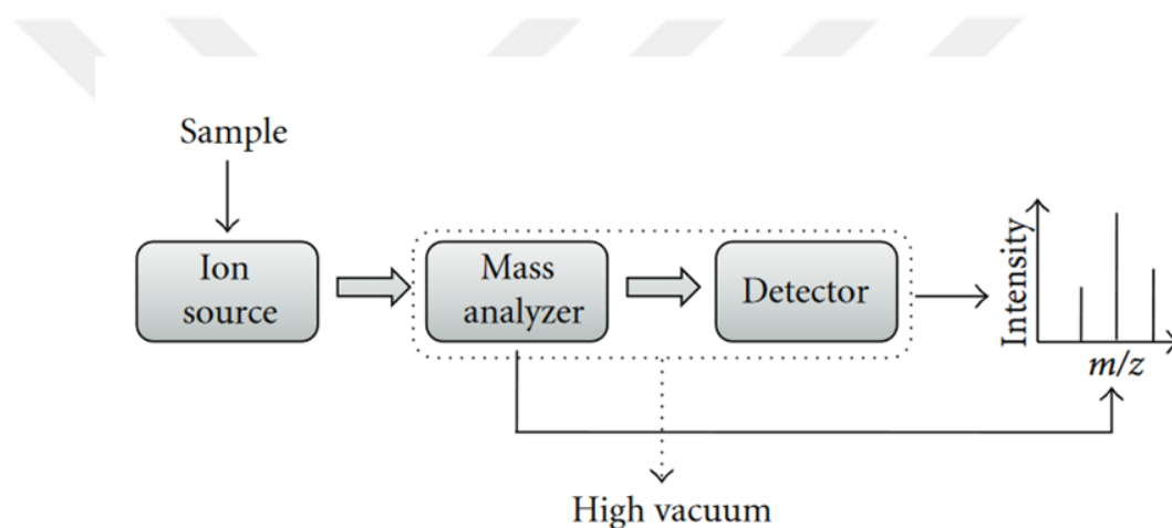
Figure 2.7. The basic components of the ESI-mass spectrometer [24].
