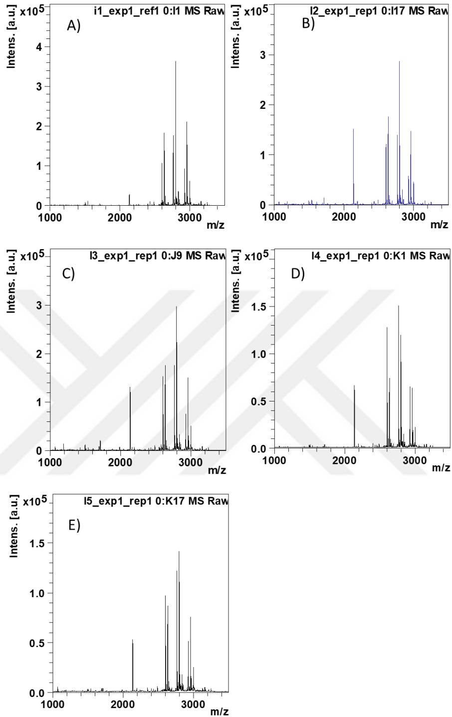
Figure Appendix A.5. MALDI-MS spectra of IgG N -glycopeptides after applied enrichment protocol with cotton stage tips in different loading conditions A) 85% ACN 1% TFA, B) 85% ACN 2% TFA, C) 85% ACN 3% TFA, D) 85% ACN 4% TFA, and E) 85% ACN 5% TFA.
