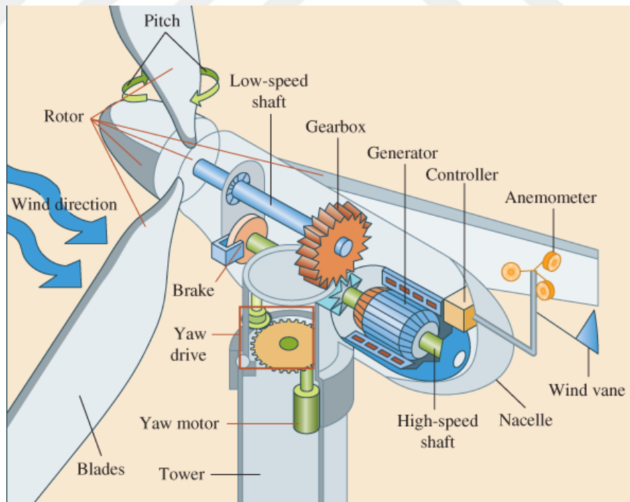
Figure 2.3 Part of Wind Turbine (Sebit, Alpman and Yilmaz 2014).
