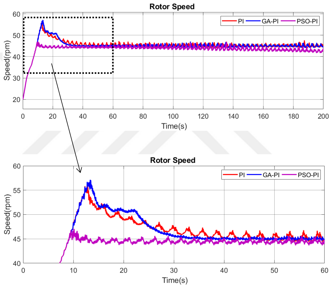
Figure 4.2 Rotor Speed.
