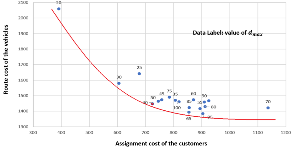
Figure 5.7 The trade-off analysis between the route and assignment costs with respect to various values of d_{max} over the instance of A-n80.cevrp
