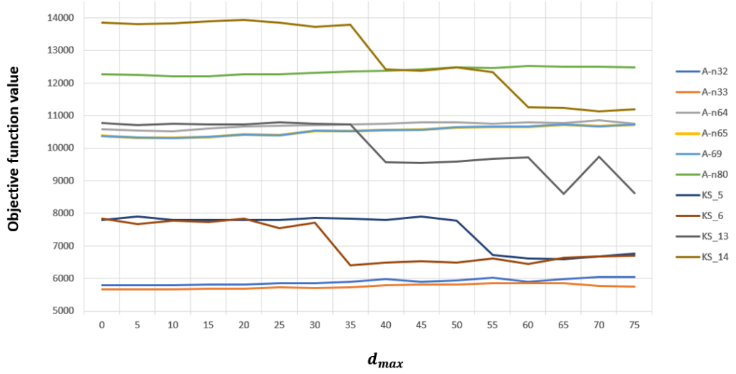
Figure 5.5 The behaviour of the objective function value in respect to the different values of d_{max} over ten CE-VRP instances
