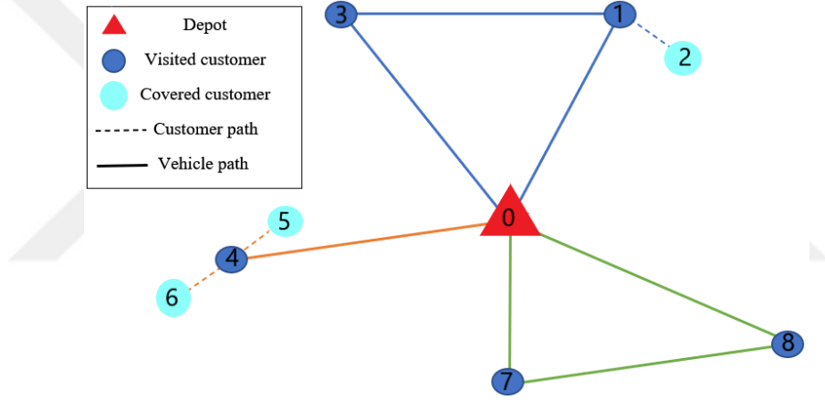
Figure 3.1 The graph of the example for CE-VRP
