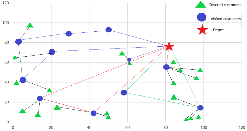
Figure 5.3 The solution found by the proposed greedy construction heuristic for the instance of A-n32-100.cevrp
