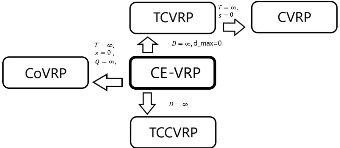
Figure 5.1 The relationship among the various addressed problems in the present thesis
