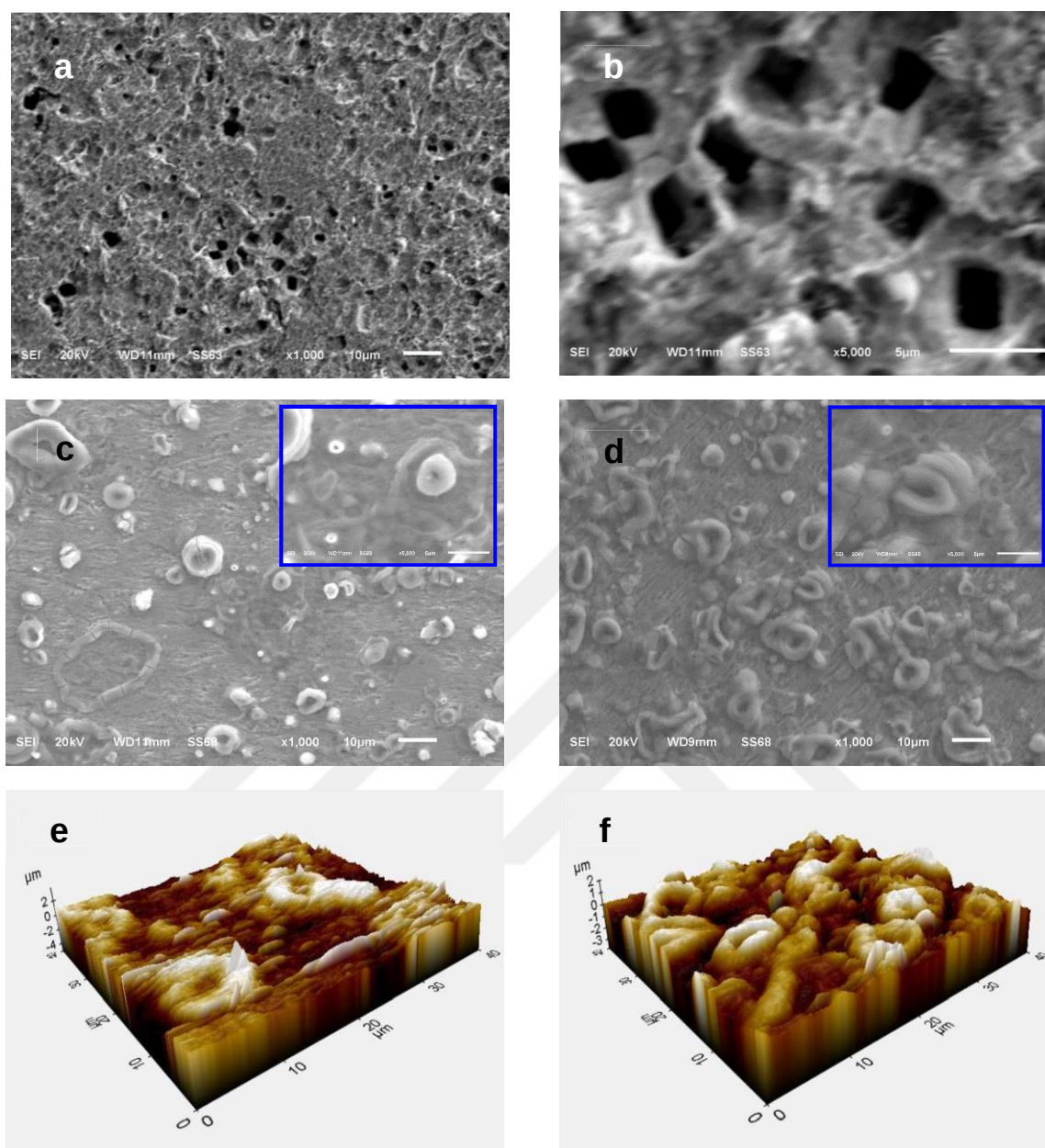
Figure 4.23. SEM images of MS taken after exposure to 1 M HCl (a and b), 1 M HCl+1000 ppm RR leaf (c) and 1 M HCl+1000 ppm RR leaf+1000 ppm KI (d) (The insets on c and d show 5 000x magnified images of the same surfaces); 3D dimensional AFM images of MS after exposure to 1 M HCl+1000 ppm RR leaf (e) and 1 M HCl+1000 ppm RR leaf+1000 ppm KI (f)
