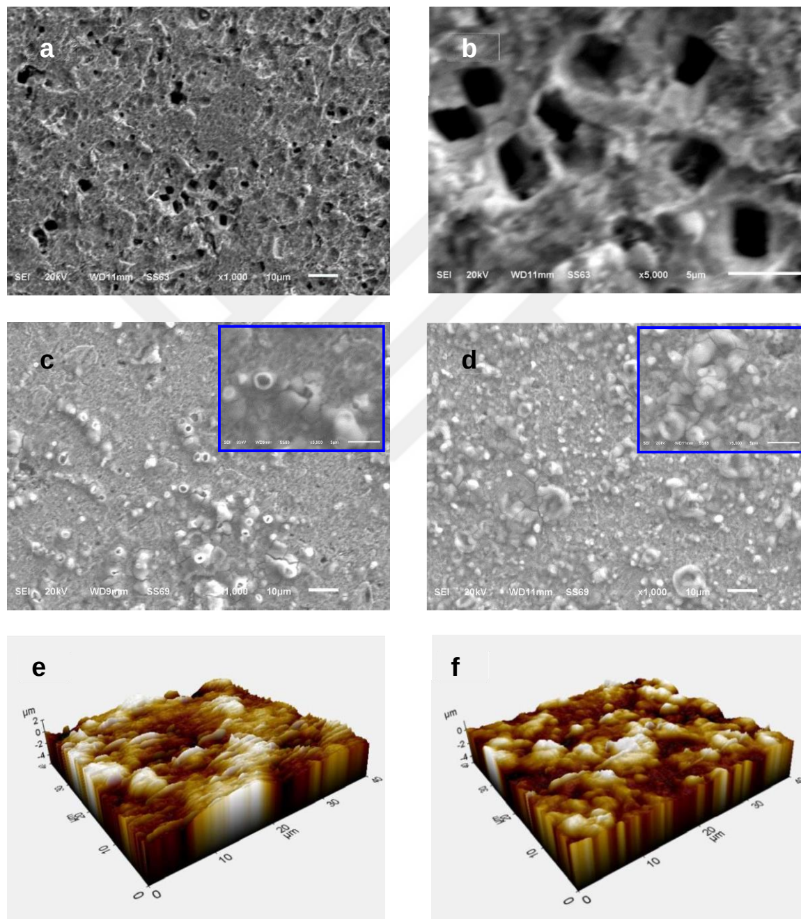
Figure 4.11. SEM images of MS taken after exposure to 1 M HCl (a and b), 1 M HCl+1000 ppm RR root (c) and 1 M HCl+1000 ppm RR root+1000 ppm KI (d) (The insets on c and d show 5 000x magnified images of the same surfaces); 3D dimensional AFM images of MS after exposure to 1 M HCl+1000 ppm RR root (e) and 1 M HCl+1000 ppm RR root+1000 ppm KI (f)
