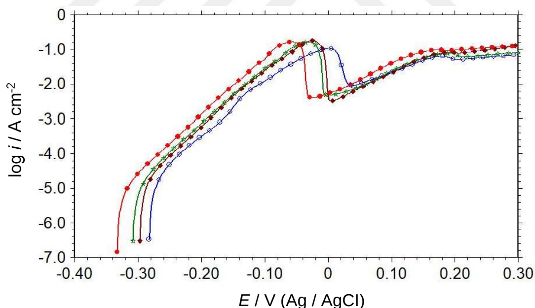
Figure 4.3. Polarization curves of Cu were obtained in 1 M HCl solution without (●) and with the addition of 1000 ppm RR flower (○), RR leaf (♦), and RR root (✱) solutions after 1-hour exposure
