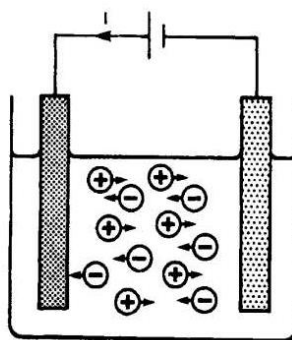
Figure 1.14. Electric current is transported through an electrolyte (Mattsson, 1996)
