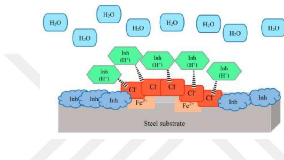
Figure 2.3. Physical adsorption scheme of protonated inhibitor in HCl medium on the metal surface (Hanini et al., 2019).
