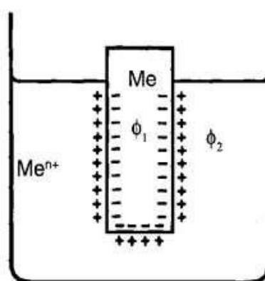
Figure 1.5. A metal (Me) has formed an electrical double layer in an aqueous solution containing metal ions, \text{Me}^{n+} (Mattsson, 1996)
