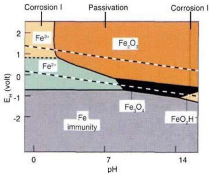
Figure 1.16. Fe-H, O potential-pH diagram at 25°C; 1 to 6 M dissolved Fe (Mattsson, 1996)
