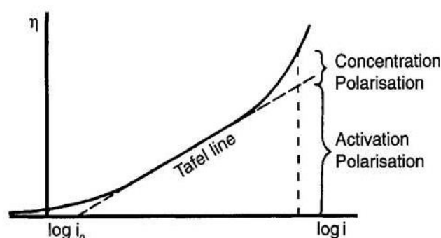
Figure 1.12. Represents polarisation( \eta ) as a function of current density( i ). The continuous line denotes total polarisation, while the logarithm denotes complete polarisation and exchange current density (Mattsson, 1996)
