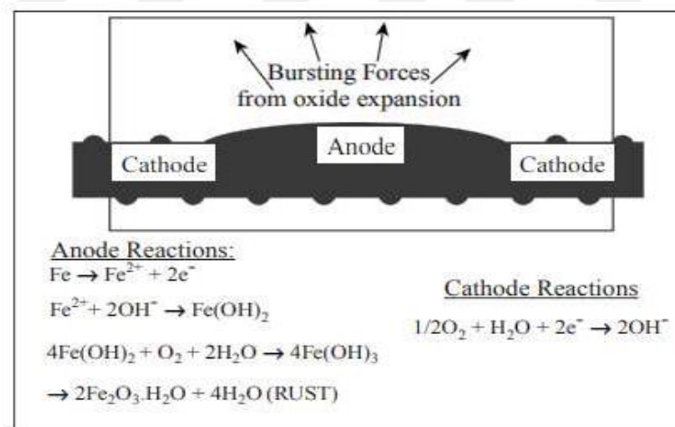
Figure 1.23. The steel corrosion process in concrete (Broomfield, 2011)
