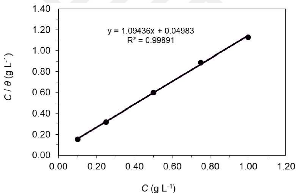
Figure 4.27. Langmuir adsorption plot of MS obtained in 1 M HCl solution with the addition of various concentrations of RR leaf extract
