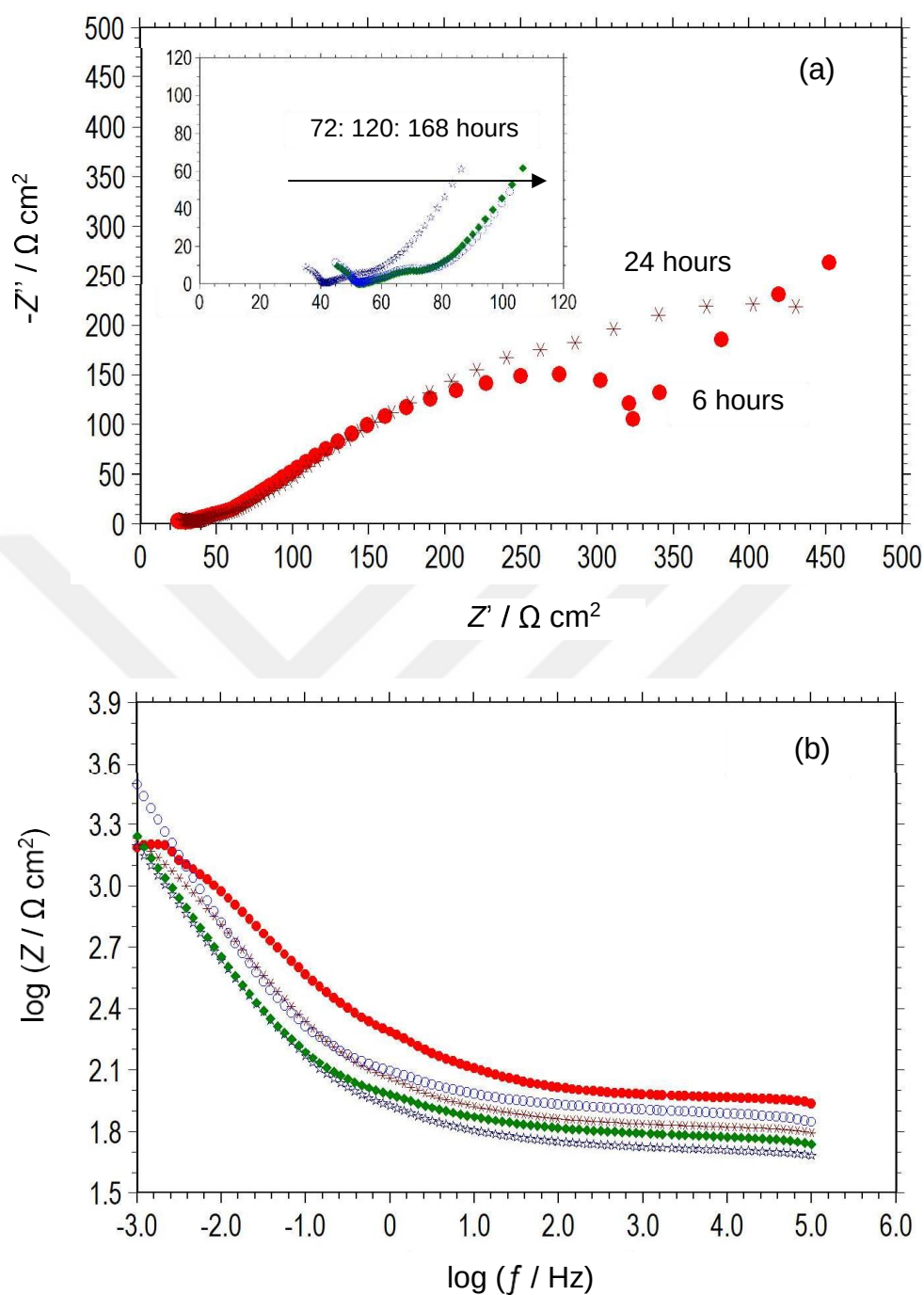
Fig. 4.43. Nyquist (a) and \log Z - \log f (Bode) (b) plots of SR, embedded in reinforced concrete without inhibitor, obtained in 3.5 % NaCl solution after various exposure times (6 hours (●), 24 hours (*), 72 hours (☆), 120 hours (◆) and 168 hours (○))
