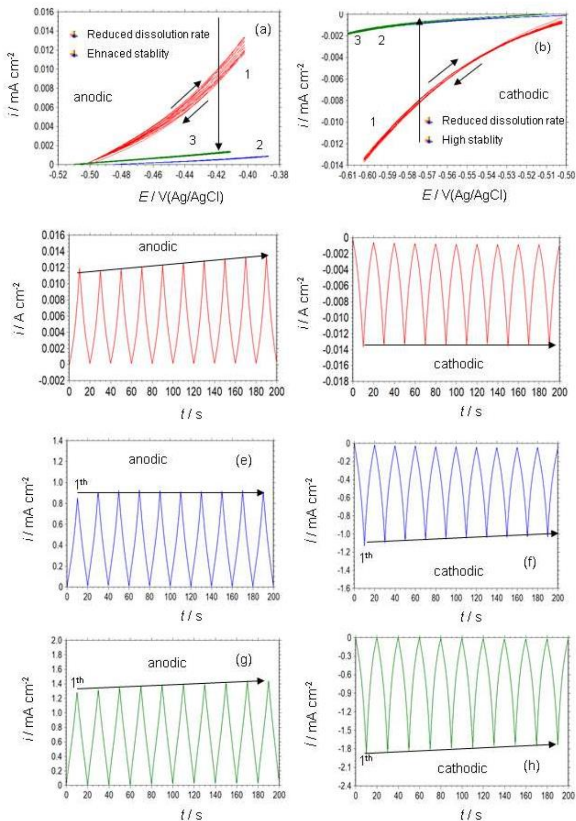
Figure 4.40. Anodic (a) and cathodic (b) CVs of MS were obtained in the test solutions (1: 1 M HCl, 2: 1 M HCl+1000 ppm RR flower, 3: 1 M HCl+1000 ppm RR flower+1000 ppm KI); Anodic CV-time plots of MS obtained in 1 M HCl (c), 1 M HCl+1000 ppm RR flower (e), 1 M HCl+1000 ppm RR flower+1000 ppm KI (g); Cathodic CV-time plots of MS obtained in 1 M HCl (d), 1 M HCl+1000 ppm RR flower (f), 1 M HCl+1000 ppm RR flower+1000 ppm KI (h)
