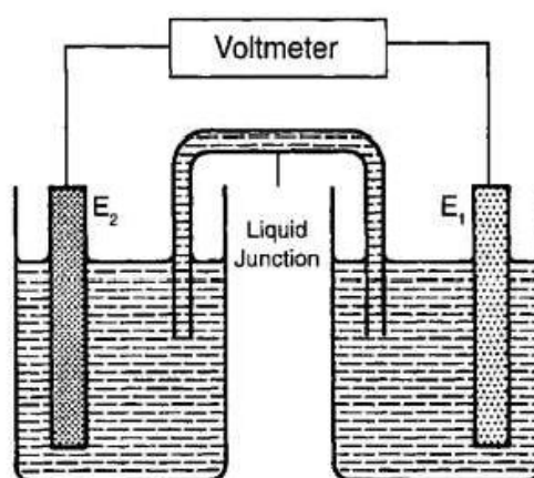
Figure 1.7. Half cells connected by a liquid junction (Mattsson, 1996)
