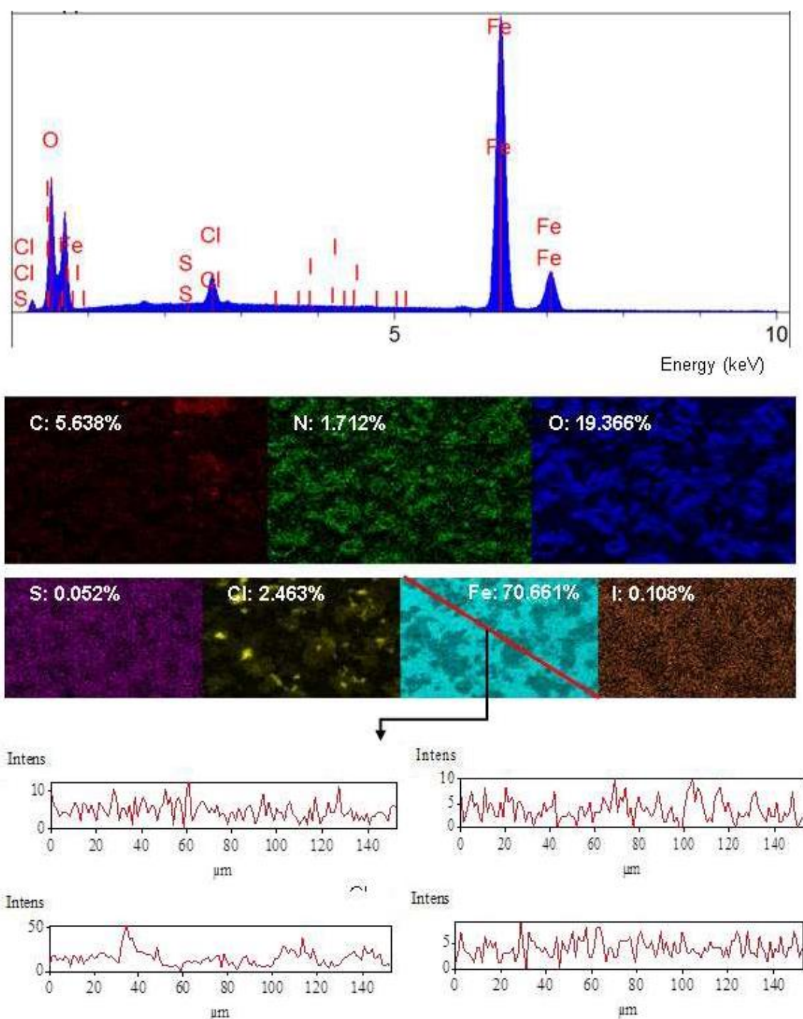
Figure 4.25. EDX spectrum of the MS surface, the distribution of some elements on the metal surface (EDX-mapping images) and cross-sectional analyses of some elements on the surface of MS after exposure to 1 M HCl solution in the presence of 1000 ppm RR leaf+1000 ppm KI
