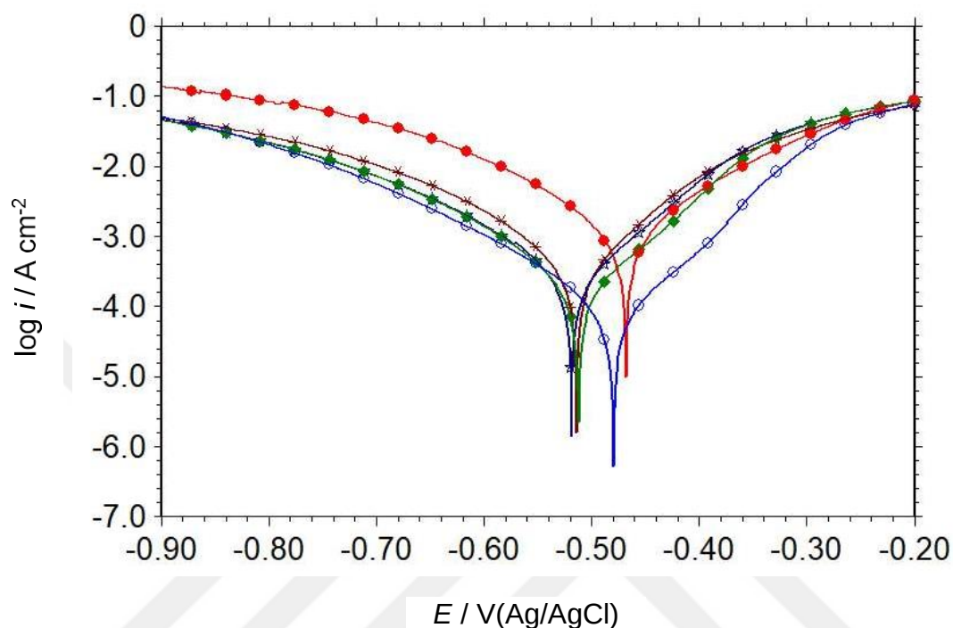
Figure 4.32. Polarization curves of MS obtained in 1 M HCl solution (●) and containing 100 (*), 250(x), 500(◆) and 1000 (○) ppm RR flower extracts
