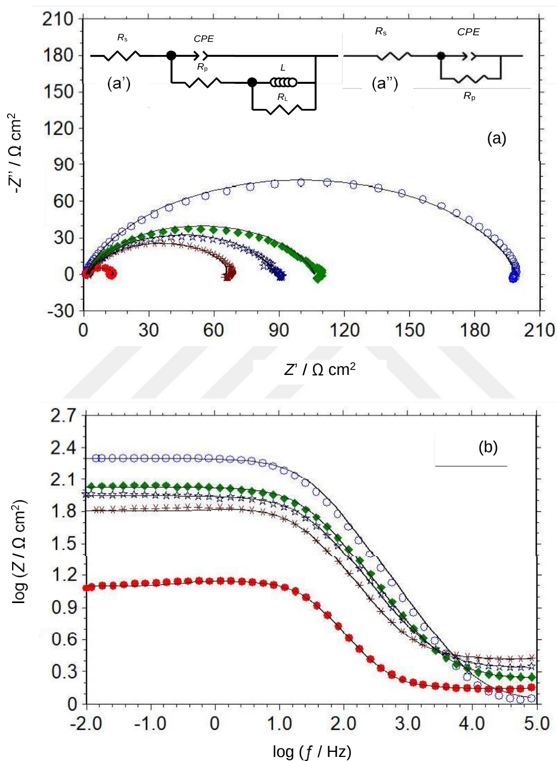
Figure 4.31. The Nyquist (a) and \log Z - \log f (Bode) (b) plots of MS obtained in 1 M HCl solution (●) and containing 100 (○), 250 (☆), 500 (◆) and 1000 (◊) ppm RR flower extracts. Solid lines show corresponding fitting curves. The insets on Fig. 3a show the related EECDS
