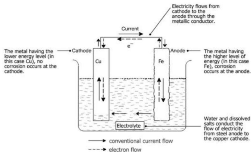
Figure 1.6. Typical galvanic cell (Ahmad, 2006)
