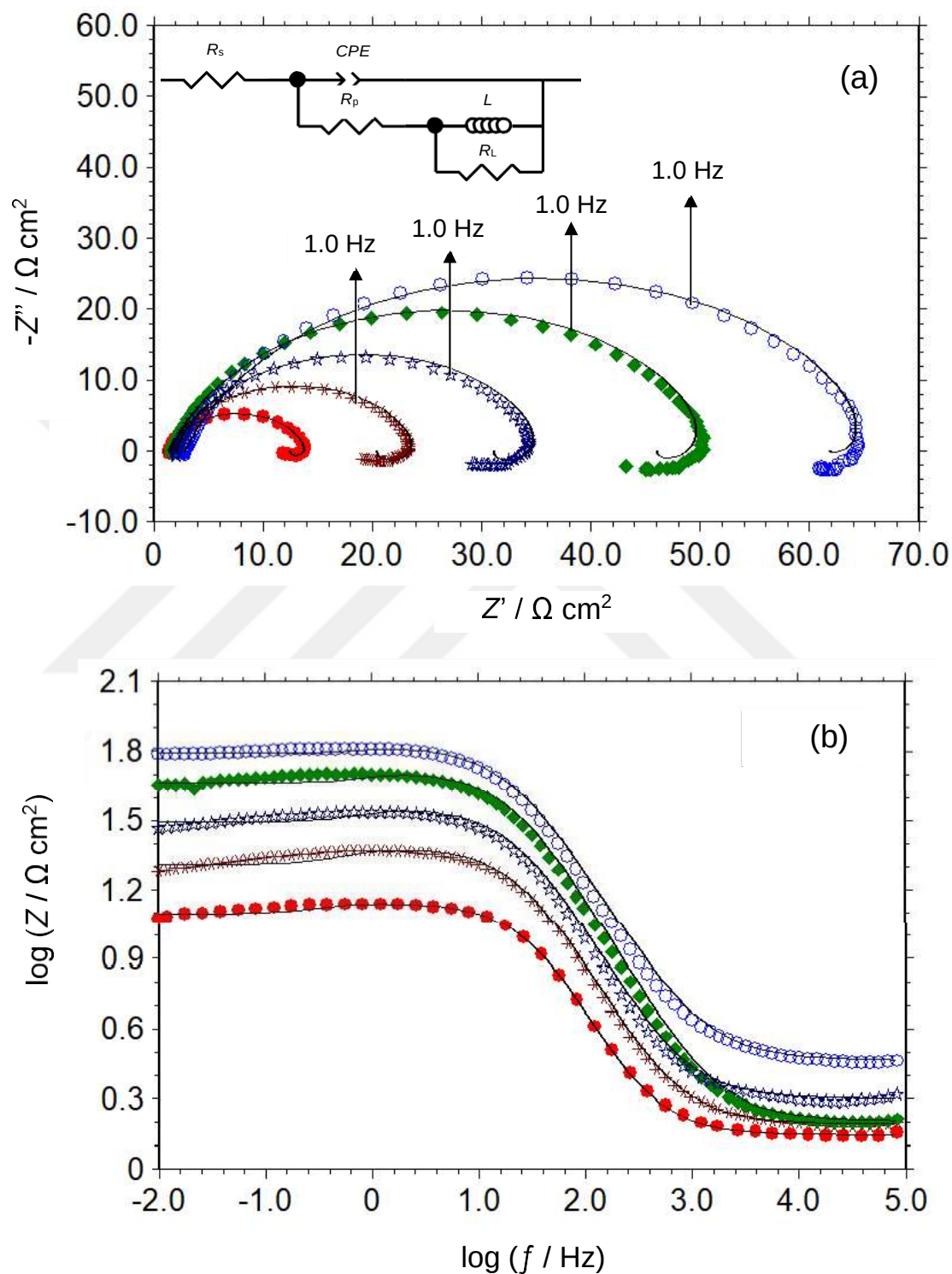
Figure 4.8. The Nyquist (a) and \log Z - \log f (Bode) (b) plots of MS obtained in 1 M HCl solution (●) and containing 100 (*), 250 (☆), 500 (◆) and 1000 (○) ppm RR root extracts. Solid lines show corresponding fitting curves. The inset on Fig. 3a shows the related electrical equivalent circuit diagram
