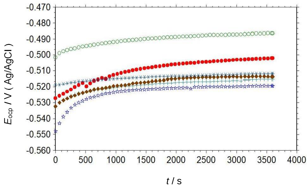
Figure 4.30. The variation of E_{ocp} of MS with immersion time in 1 M HCl solution (●) and containing 100 (☆), 250 (+), 500 (◆), 1000 (○) and 2000 (*) ppm RR flower extracts
