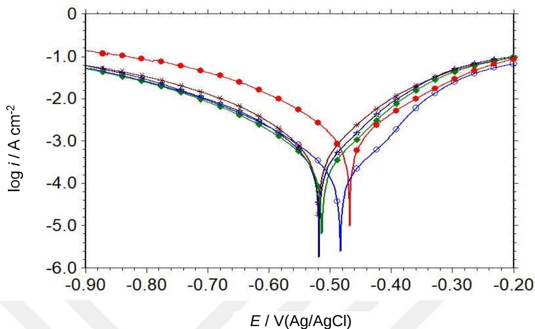
Figure 4.21. Polarization curves of MS obtained in 1 M HCl solution (●) and containing 100 (*), 250 (x), 500 (◆) and 1000 (○) ppm RR leaf extracts
