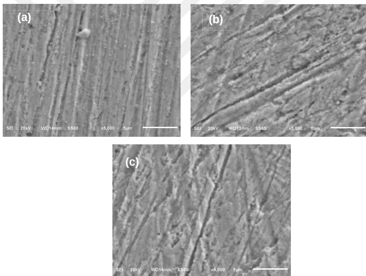
Figure 4.4. SEM images of Cu surface after exposure to 1 M HCl solution in the presence of 1000 ppm RR flower (a), RR leaf (b), and RR root (c)
