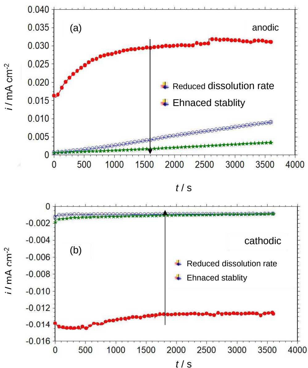
Figure 4.39. The variation of anodic and the cathodic current densities as a function of time under constant +100 mV anodic (a) and -100 mV cathodic (b) overpotentials conducted in 1 M HCl solution (●) and containing 1000 ppm RR flower (○), 1000 ppm RR flower+1000 ppm KI (★)
