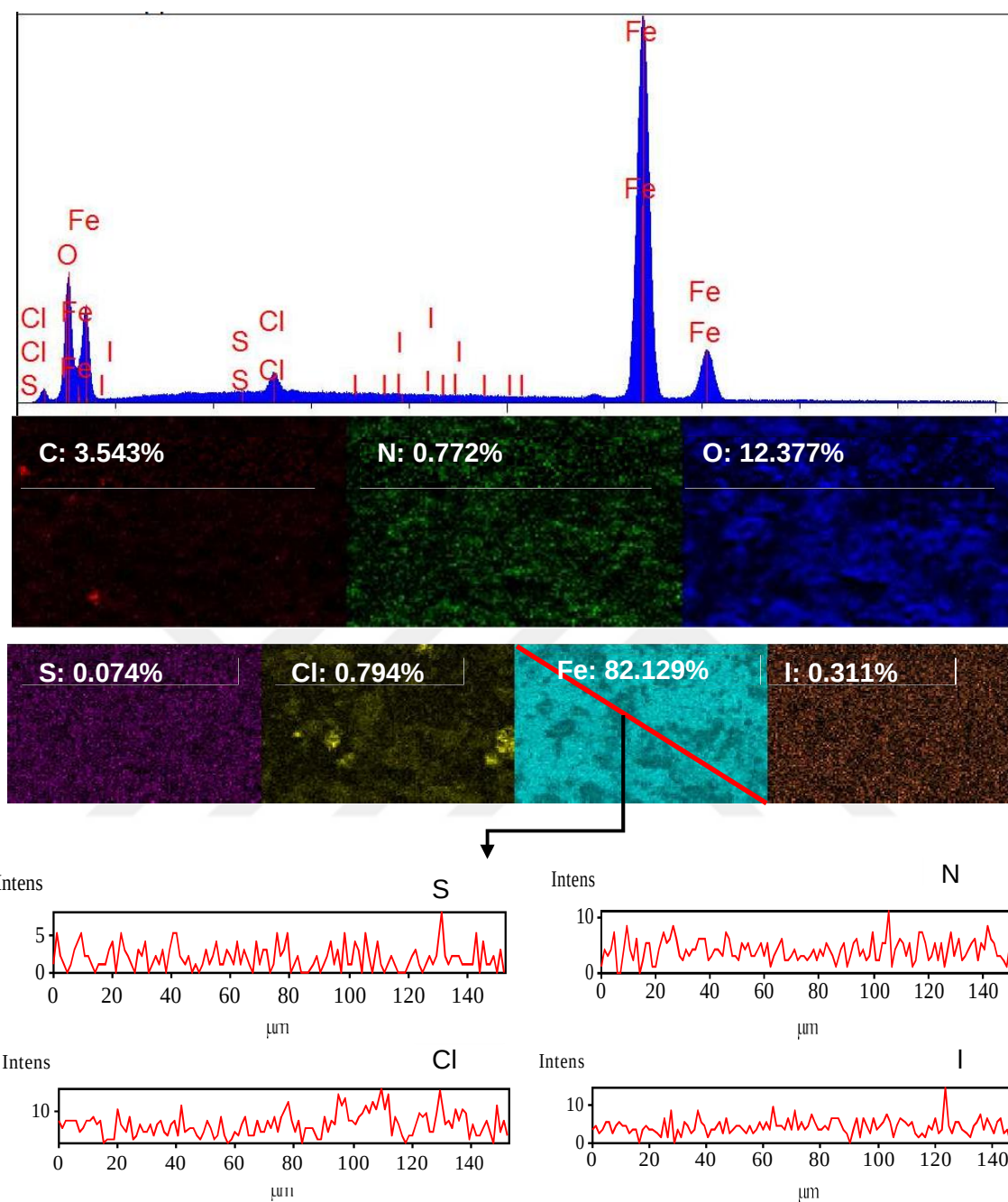
Figure 4.13. EDX spectrum of the MS surface, the distribution of some elements on the metal surface (EDX-mapping images) and cross-sectional analyses of some elements on the surface of MS after exposure to 1 M HCl solution in the presence of 1000 ppm RR root+1000 ppm KI
