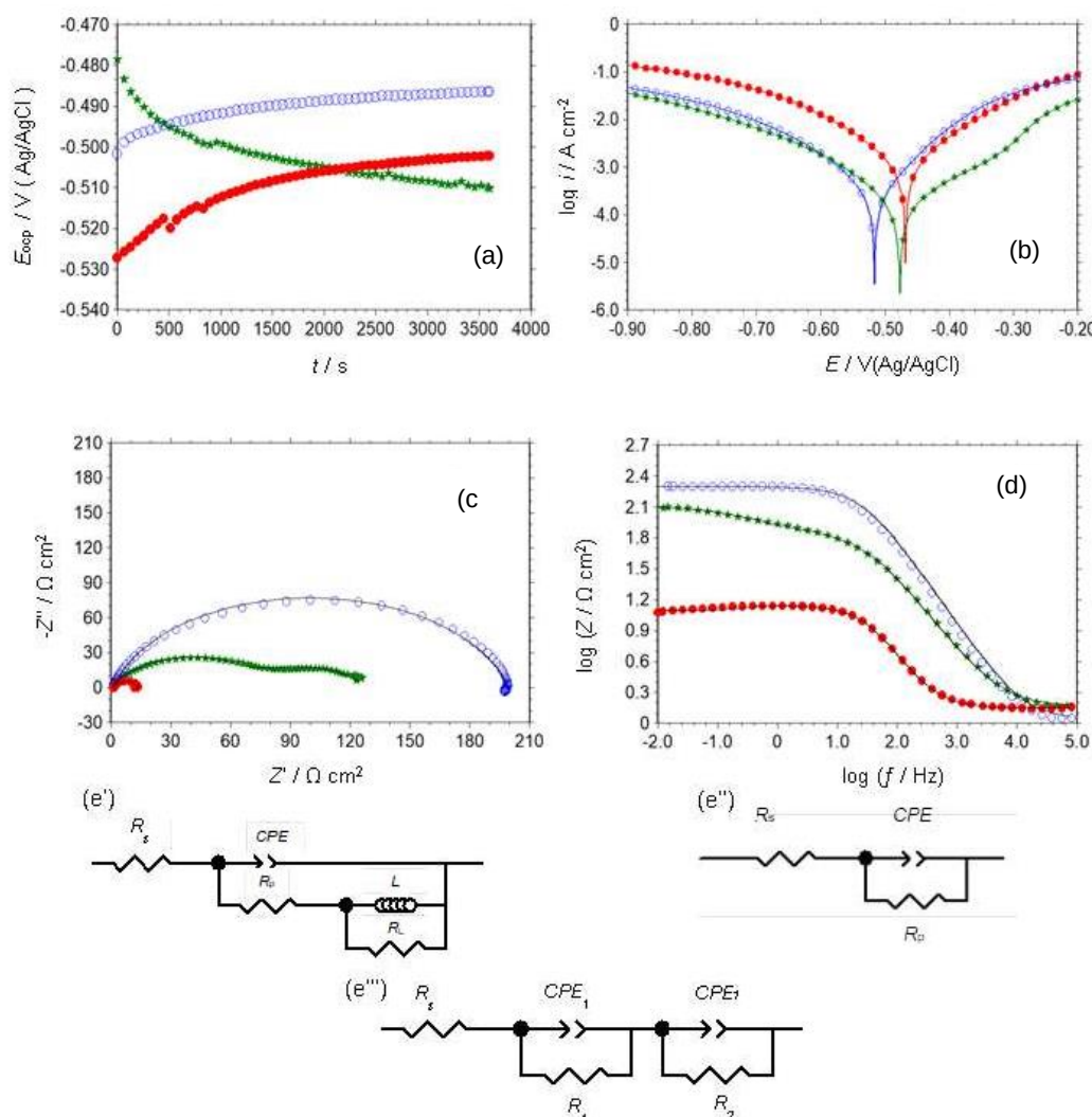
Figure 4.33. The variation of E_{ocp} of MS with immersion time (a); potentiodynamic polarization (b), Nyquist (c), and \log Z - \log f (Bode) (d) plots of MS obtained in 1 M HCl solution in the absence (●) and containing 1000 ppm RR flower (○), 1000 ppm RR flower+1000 ppm KI (★); EECs proposed for the MS/solution interface in 1 M HCl and 1 M HCl+1000 ppm RR flower (c'), 1 M HCl+1000 ppm RR flower+1000 ppm KI (c'')
