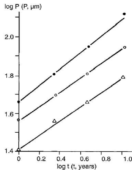
Figure 1.19. The same results are shown in Figure 1.18 as a bilogarithmic diagram of corrosion depth (P) and exposure time (r) (Mattsson, 1996)
