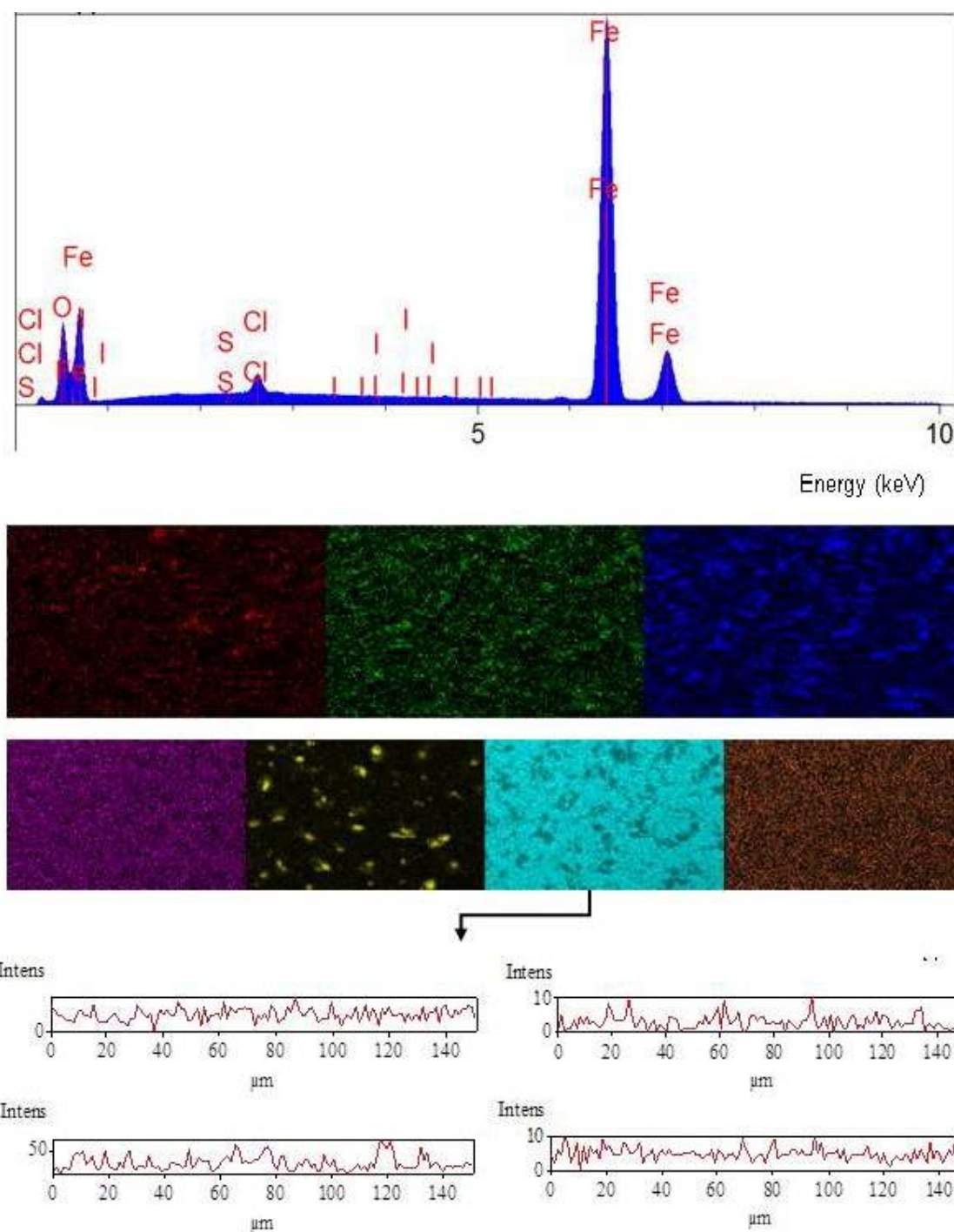
Figure 4.36. EDX spectrum of the MS surface, the distribution of some elements on the metal surface (EDX-mapping images) and cross-sectional analyses of some elements on the surface of MS after exposure to 1 M HCl solution in the presence of 1000 ppm RR flower+1000 ppm KI
