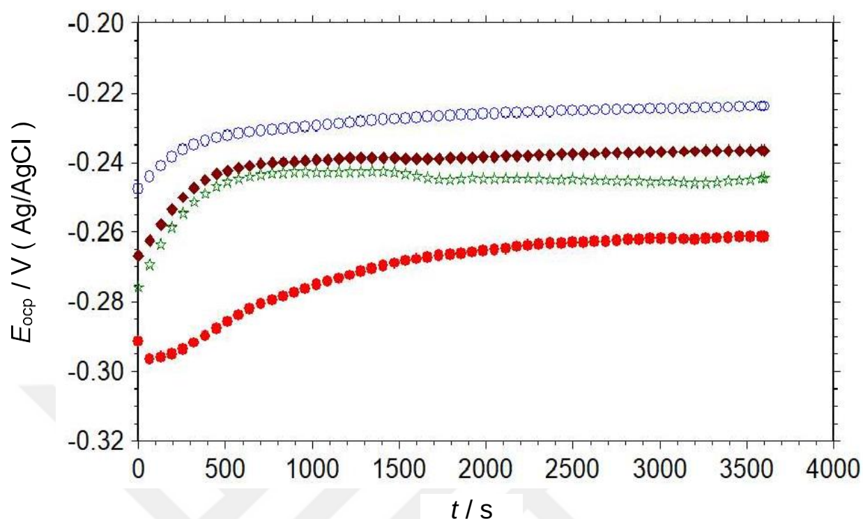
Figure 4.1. The change of open circuit potential of Cu with immersion time in 1 M HCl (●) and containing 1000 ppm RR flower (○), RR leaf (◆) and RR root (★) solutions
