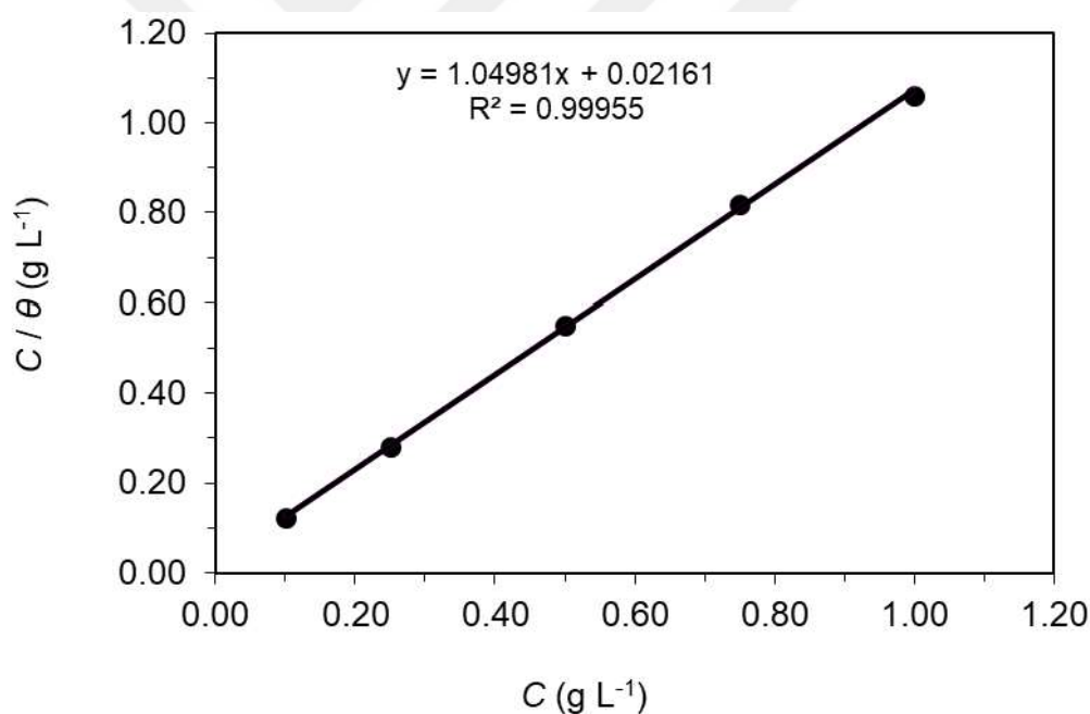
Figure 4.38. Langmuir adsorption plot of MS obtained in 1 M HCl solution with the addition of various concentrations of RR flower extract
