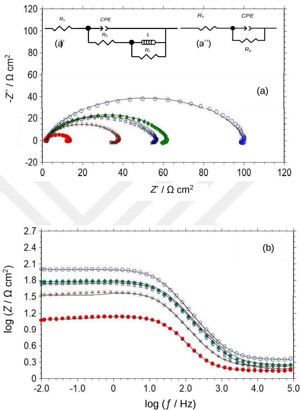
Figure 4.20. The Nyquist (a) and \log Z - \log f (Bode) (b) plots of MS obtained in 1 M HCl solution (●) and containing 100 (✱), 250 (☆), 500 (◆) and 1000 (○) ppm RR leaf extracts. Solid lines show corresponding fitting curves. The insets on Fig. 3a show the related EECDs
