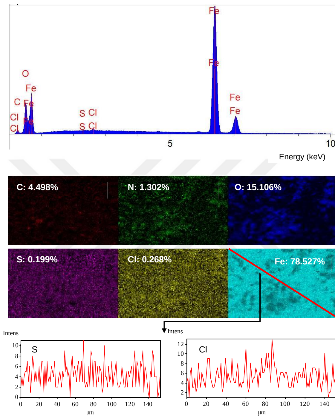
Figure. 4.12. EDX spectrum of the MS surface, the distribution of some elements on the metal surface (EDX-mapping images) and cross-sectional analyses of some elements on the surface of MS after exposure to 1 M HCl solution in the presence of 1000 ppm RR root for 1 hour
