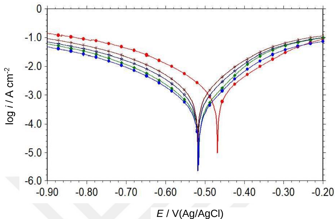
Figure 4.9. Polarization curves of MS obtained in 1 M HCl solution (●) and containing 100 (*), 250 (☆) 500 (◆) and 1000 (○) ppm RR root extracts
