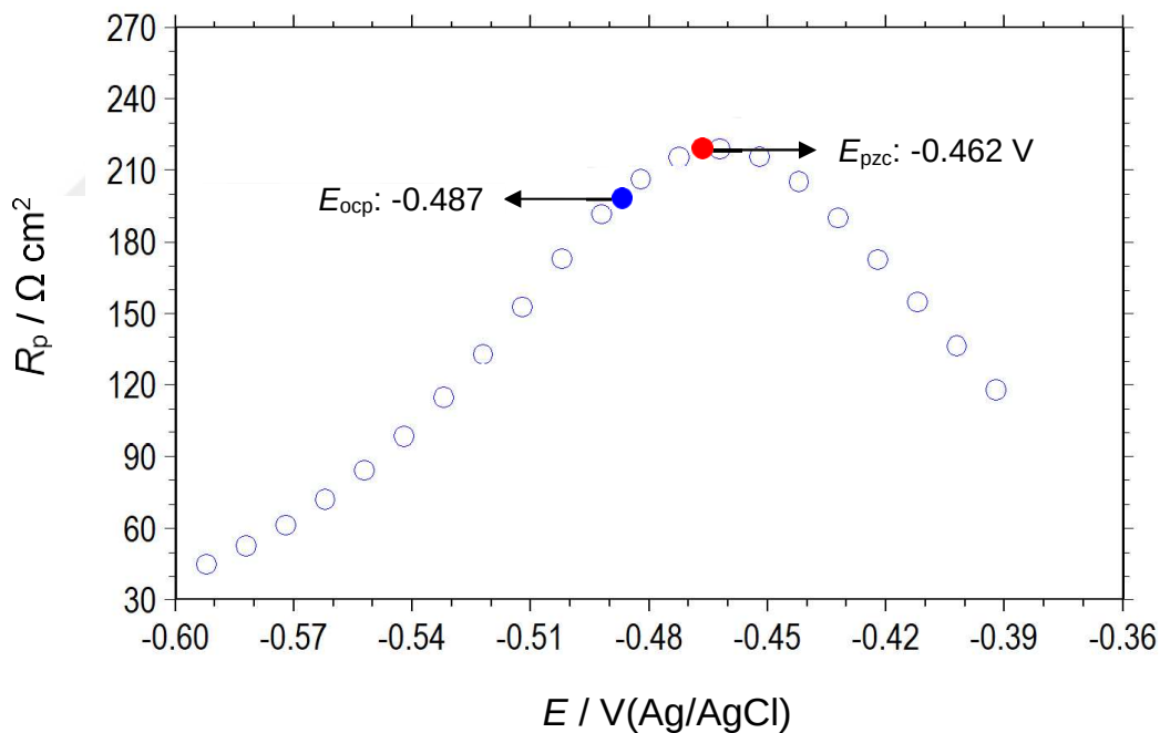
Figure 4.42. R_p vs applied potential plot in 1 M HCl solution containing 1000 ppm RR flower extract
