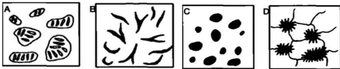
Figure 1.15. Cast iron structures: A, white cast iron; cementite ( \text{Fe}_3\text{C} ) matrix with pearlite precipitates; B, grey cast iron; pearlite or ferrite matrix graphite flakes; C, spheroidal cast iron; pearlite or ferrite matrix graphite nodules; D, malleable iron; irregular graphite grains in a pearlite or ferrite matrix (Mattsson, 1996)
