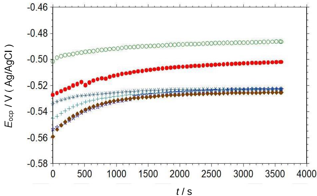
Figure 4.19. The variation of open circuit potential of MS with immersion time in 1 M HCl solution (●) and containing 100 (☆), 250 (+) 500 (◆) 1000 (○) and 2000 (*) ppm RR leaf extracts
