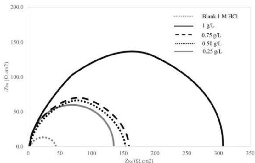
Figure 2.2. Nyquist plots for different concentrations of pomegranate bark extract in 1 M HCl (Marsoul et al., 2020)
