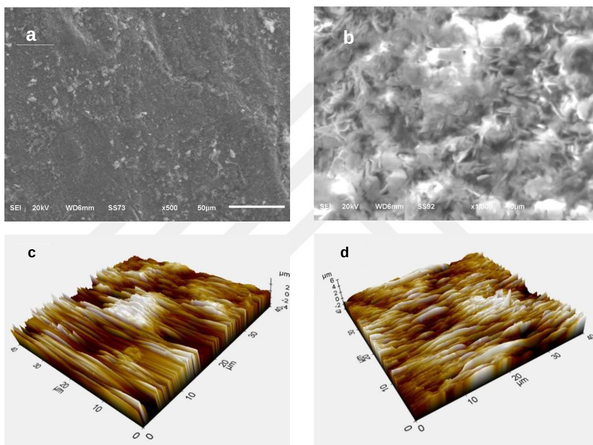
Figure 4. 44. SEM and 3D AFM images of the surface of SR embedded in reinforced concrete without (a and c) and with 1000 ppm RR flower (b and d) were obtained in 3.5 % NaCl solution after 168 hours of exposure
