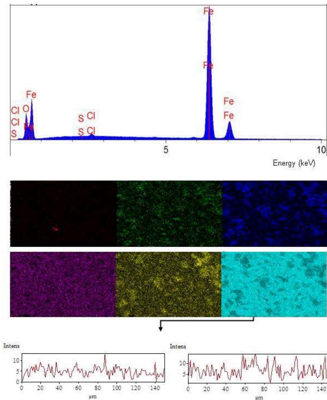
Fig. 4.35. EDX spectrum of the MS surface, the distribution of some elements on the metal surface (EDX-mapping images) and cross-sectional analyses of some elements on the surface of MS after exposure to 1 M HCl solution in the presence of 1000 ppm RR flower for 1 hour
