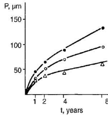
Figure 1.18. Corrosion depth (P) as a function of exposure time (t) on atmospheric corrosion of steel: e, Millheim, Ruhr; o, Cuxhaven; A, Olpe (Mattsson, 1996)
