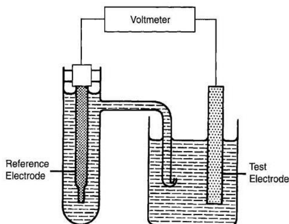
Figure 1.9. Determination of electrode potential using a reference electrode(Mattsson, 1996)
