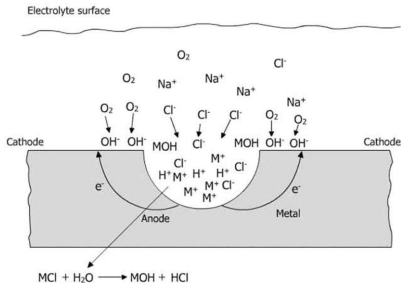
Figure 1.3. Schematic of an active corrosion pit on metal in a chloride solution (Ahmad, 2006)
