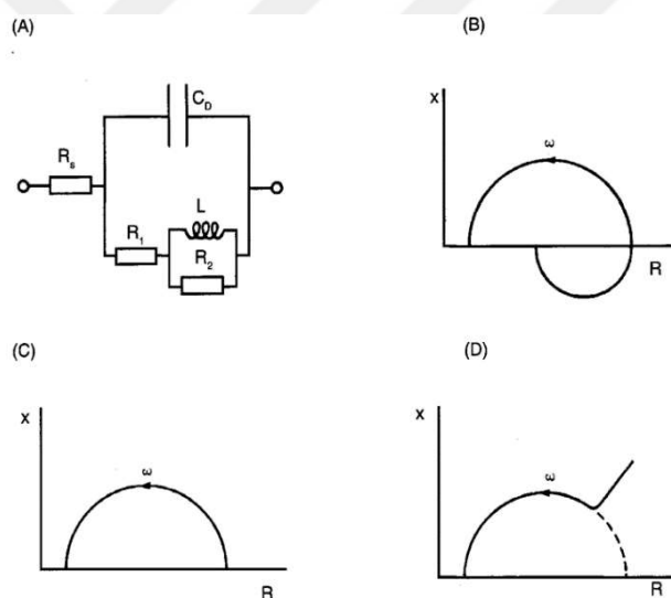
Figure 1.13. A. An electrical analogue of an electrode; R = electrolyte resistance, CD = double layer capacitance, L = inductance, R_1 and R_2 = resistances. Impedance spectra for various electrode types (B-D); R = resistive part, X = reactive part; arrows indicate increased frequency ( \omega ) (Mattsson, 1996)
