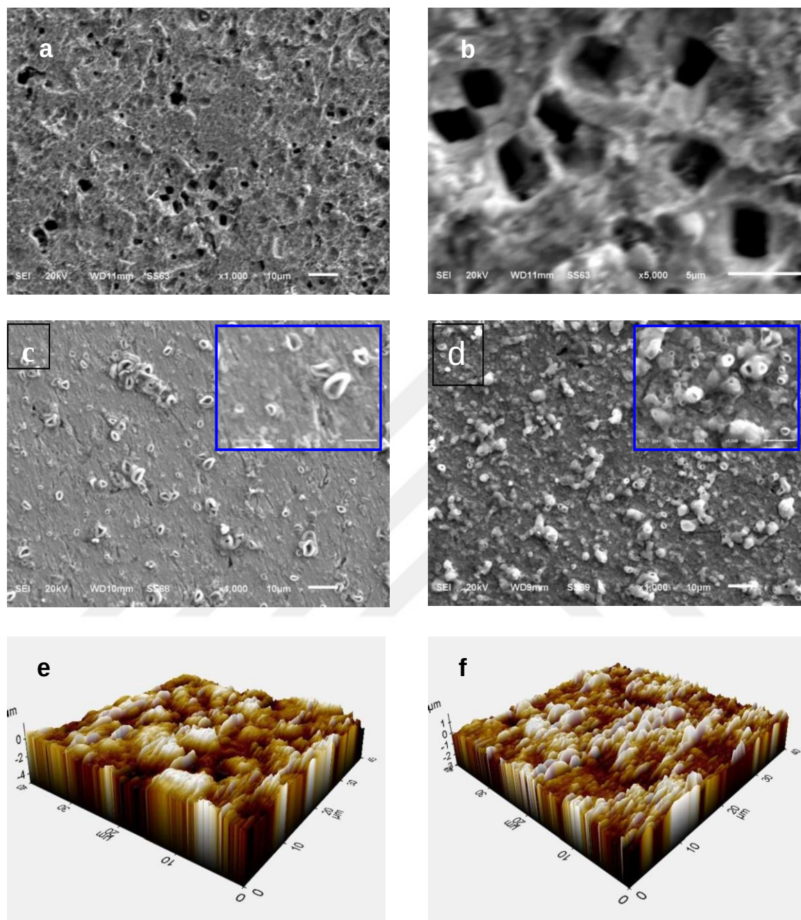
Figure 4.34. SEM images of MS taken after exposure to 1 M HCl (a and b), 1 M HCl+1000 ppm RR flower (c) and 1 M HCl+1000 ppm RR flower+1000 ppm KI (d) (The insets on c and d show 5 000x magnified images of the same surfaces); 3D dimensional AFM images of MS after exposure to 1 M HCl+1000 ppm RR flower (e) and 1 M HCl+1000 ppm RR flower+1000 ppm KI (f)
