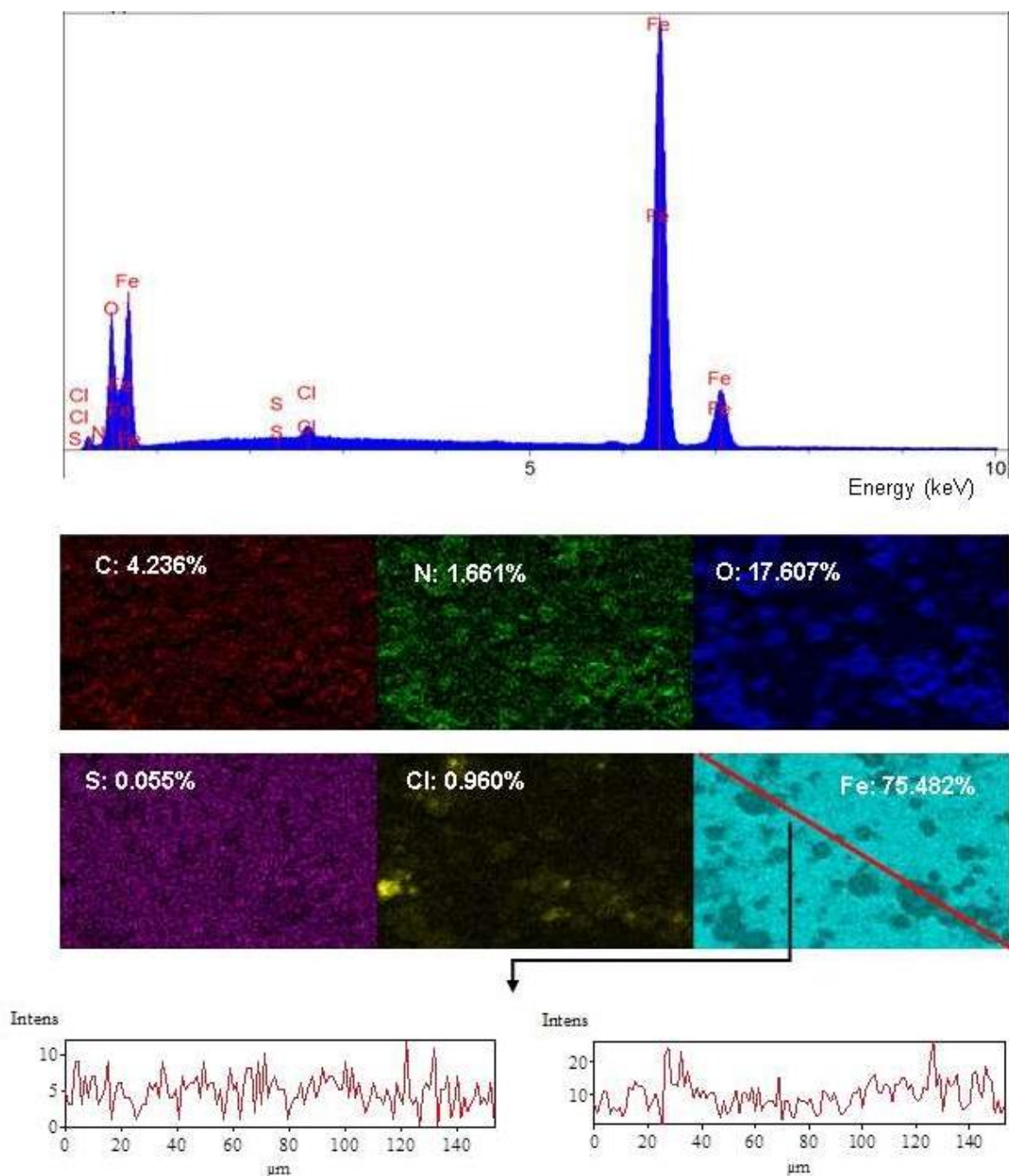
Fig. 4.24. EDX spectrum of the MS surface, the distribution of some elements on the metal surface (EDX-mapping images) and cross-sectional analyses of some elements on the surface of MS after exposure to 1 M HCl solution in the presence of 1000 ppm RR leaf for 1 hour
