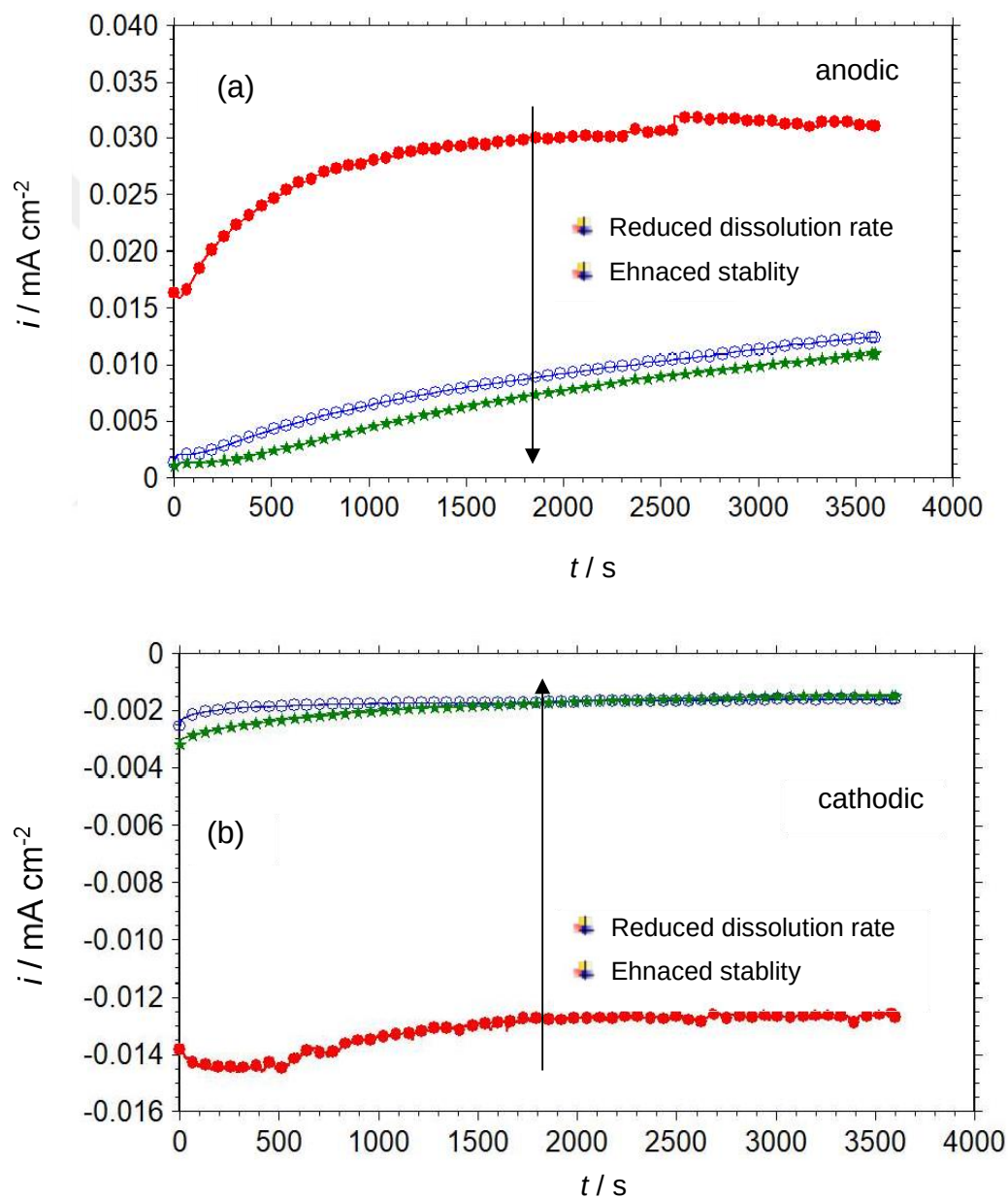
Figure 4.28. The variation of anodic and the cathodic current densities as a function of time under constant +100 mV anodic (a) and -100 mV cathodic (b) overpotentials conducted in 1 M HCl solution (●) and containing 1000 ppm RR leaf (○), 1000 ppm RR leaf+1000 ppm KI (★)
