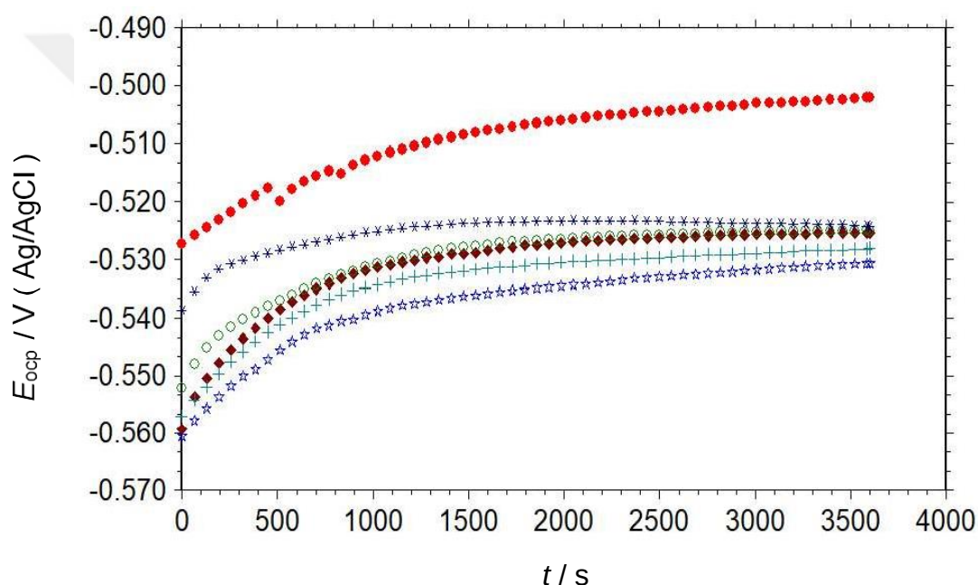
Figure 4.7. The variation of open circuit potential of MS with immersion time in 1 M HCl solution (●) and containing 100 (☆), 250 (+) 500 (◆) 1000 (○), and 2000 (⌘) ppm RR root extracts
