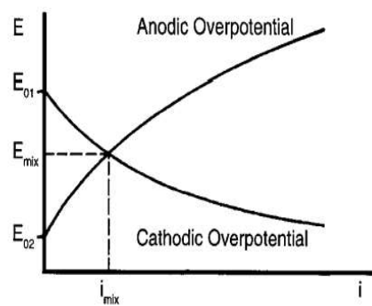
Figure 1. 11. Overpotential curves for two simultaneous electrode reactions at an electrode surface; E = electrode potential, i = current density (Mattsson, 1996)
