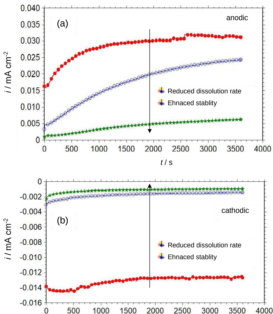
Figure 4.17. The variation of anodic and the cathodic current densities as a function of time under constant +100 mV anodic (a) and -100 mV cathodic (b) overpotentials conducted in 1 M HCl solution (●) and containing 1000 ppm RR root (○), 1000 ppm RR root+1000 ppm KI (★)
