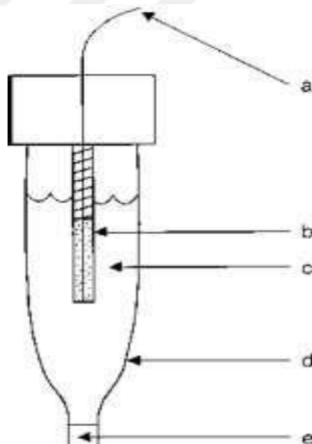
Figure 1.8. Components of typical commercial reference electrode: (a) electrical connection, (b) metal-metal salt electrode, (c) filling solution that maintains electrode interface equilibrium, (d) glass or polymeric electrode body, (e) porous frit (Kelly, 2002)
