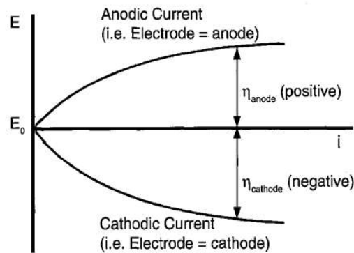
Figure 1.10. The anodic and cathodic polarisation curves; E = electrode potential, i = current density and \eta = polarisation (Mattsson, 1996)
