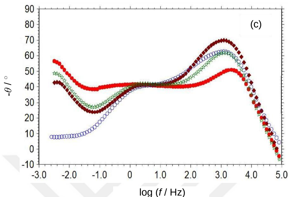
Figure 4.2. The Nyquist (a), \log Z - \log f (b), and phase angle- \log f (c) (Bode) plots of Cu obtained in 1 M HCl solution without (●) and with the addition of 1000 ppm RR flower (○), RR leaf (◆) and RR root (☆) solutions after 1-hour exposure.
