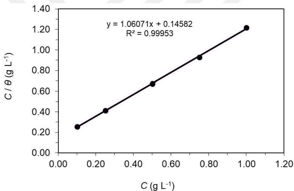
Figure 4.15 Langmuir adsorption plot of MS obtained in 1 M HCl solution with the addition of various concentrations of RR root extract
