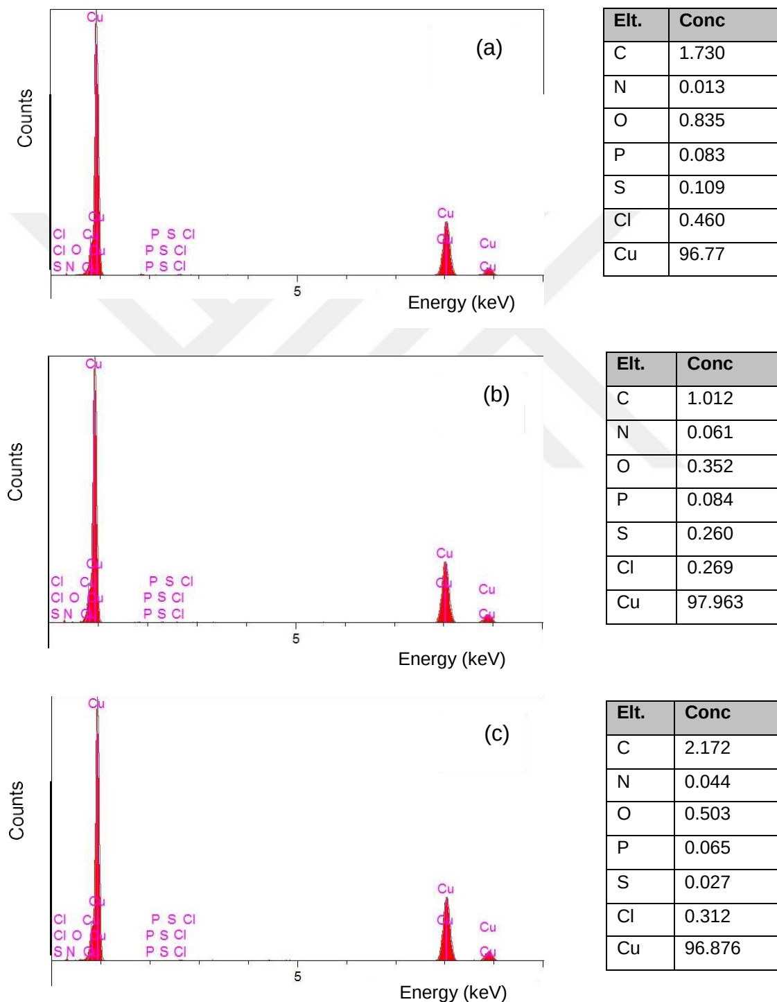
Figure 4.5. EDX spectrums and elemental composition of Cu surface after exposure to 1 M HCl solution in the presence of 1000 ppm RR flower (a), RR leaf (b), and RRroot (c)
