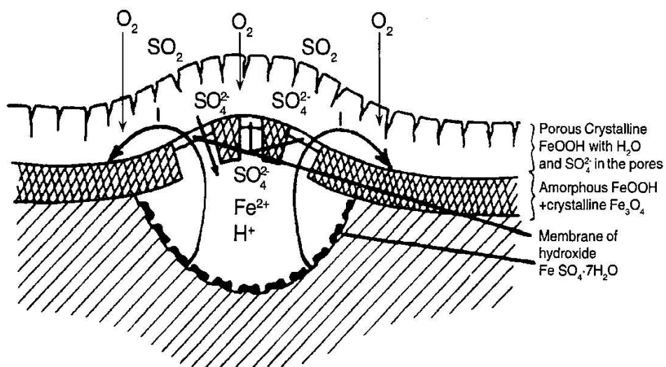
Figure 1.17. Corrosion cells, sulfate nest, active in the atmospheric corrosion of steel (Mattsson, 1996)
