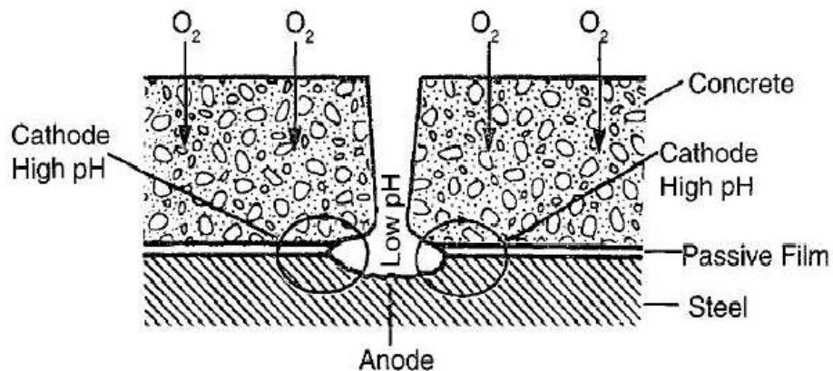
Figure 1.22. Active/passive cell concrete structures on steel (Mattsson, 1996)
