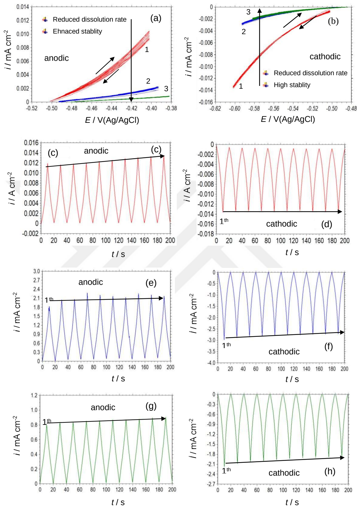
Figure 4.29. Anodic (a) and cathodic (b) CVs of MS obtained in the test solutions (1: 1 M HCl, 2: 1 M HCl+1000 ppm RR leaf, 3: 1 M HCl+1000 ppm RR leaf+1000 ppm KI); Anodic CV-time plots of MS obtained in 1 M HCl (c), 1 M HCl+1000 ppm RR leaf (e), 1 M HCl+1000 ppm RR leaf+1000 ppm KI (g); Cathodic CV-time plots of MS obtained in 1 M HCl (d), 1 M HCl+1000 ppm RR leaf (f), 1 M HCl+1000 ppm RR leaf+1000 ppm KI (h)
