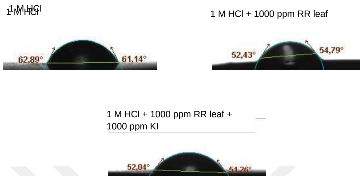
Figure 4.26. Contact angle images of the MS surface after exposure to 1 M HCl, 1 M HCl + 1000 ppm RR leaf and 1 M HCl + 1000 ppm RR leaf + 1000 ppm KI solutions for 1 hours
