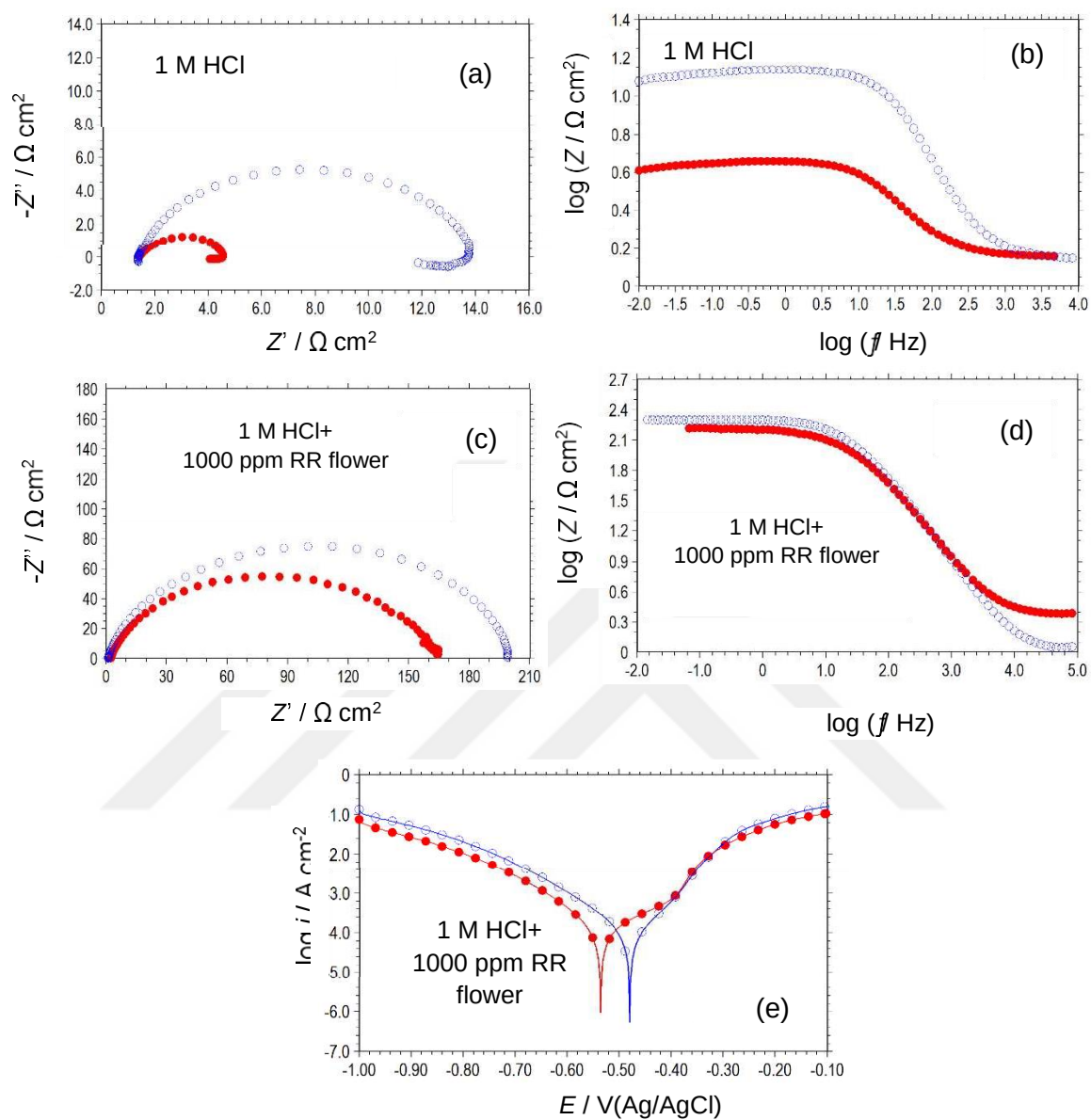
Figure 4.41. Nyquist (a, c) and Bode (b, d) plots of MS obtained in 1 M HCl solution without and with the inhibitor after 1 hour (●) and 6 hours (○) immersion; Polarization curves (e) of MS obtained in 1000 ppm RR flower extract containing 1 M HCl solution after 1 hour (●) and 6 hours (○) immersion
