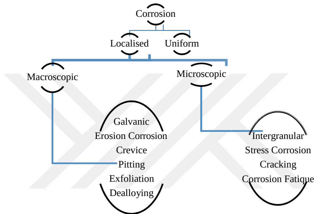
Figure 1.1. Macroscopic and microscopic forms of localized corrosion (Url-3, 2022)
