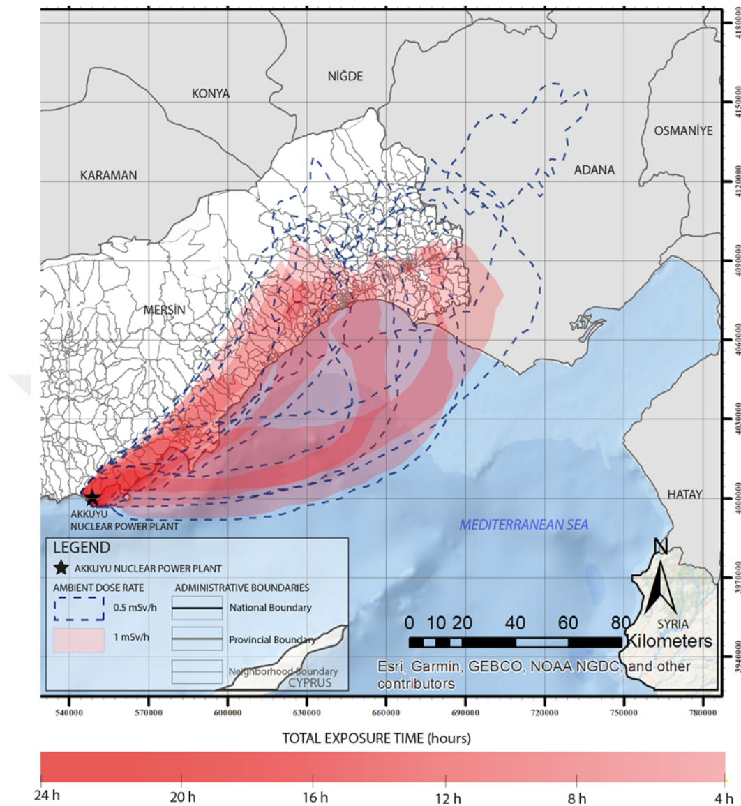
Figure 5.21. Superposed nuclear hazard map displaying total exposure time for Akkuyu Nuclear Power Plant: Scenario 2 day 2 (From 12.00 pm 16 May 2021 to 17 May 2021) (Grid size: 30x30 km)
