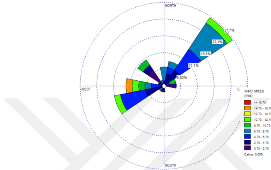
Figure 4.2. The wind rose diagram indicating wind directions (blowing from) and speeds in Mersin Province in 2021
