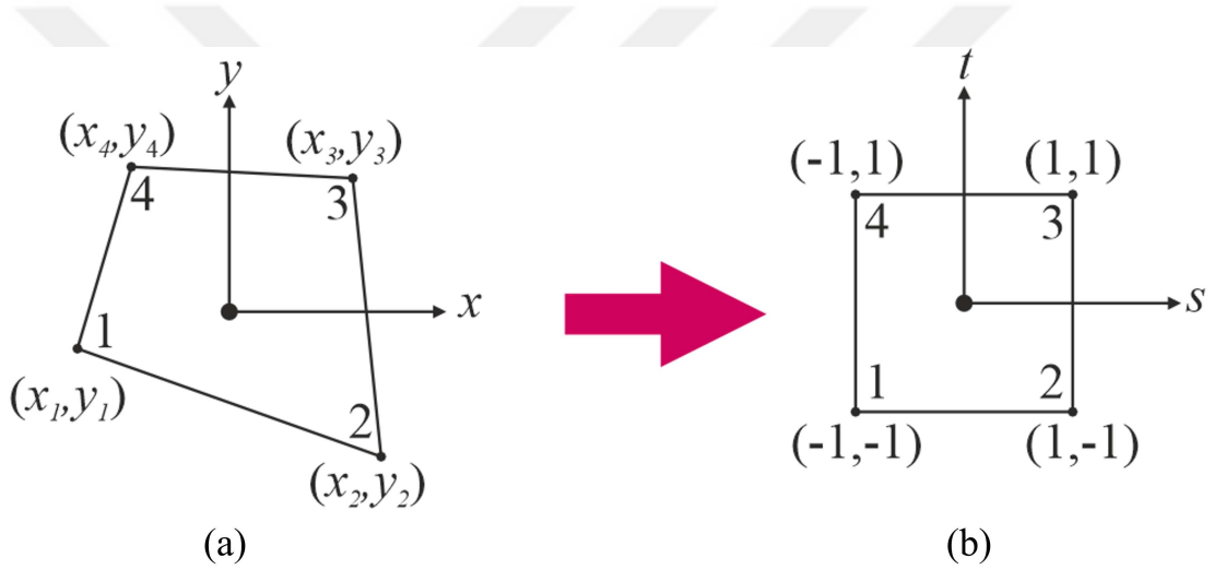
Figure 2.5 (a) Local coordinate system for the inverse-shell element, iQS4; (b) Isoparametric coordinate system.
