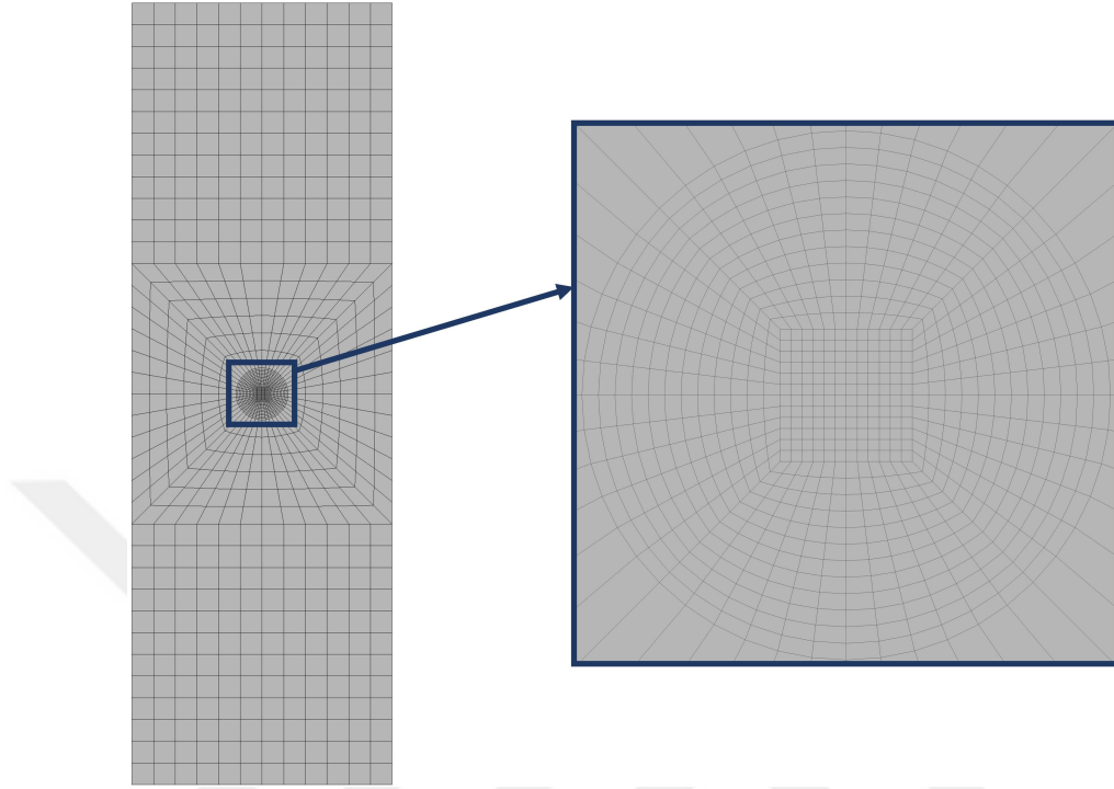
Figure 4.2 Discretization of the problem domain with 1296 elements for conducting the forward analysis.
