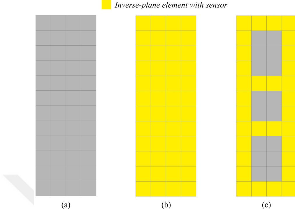
Figure 4.4 (a) Discretization of the problem domain with 48 inverse-plane elements in order to conduct inverse analysis; (b) Dense, D, sensor placement model; (c) Sparse, S, sensor placement model.
