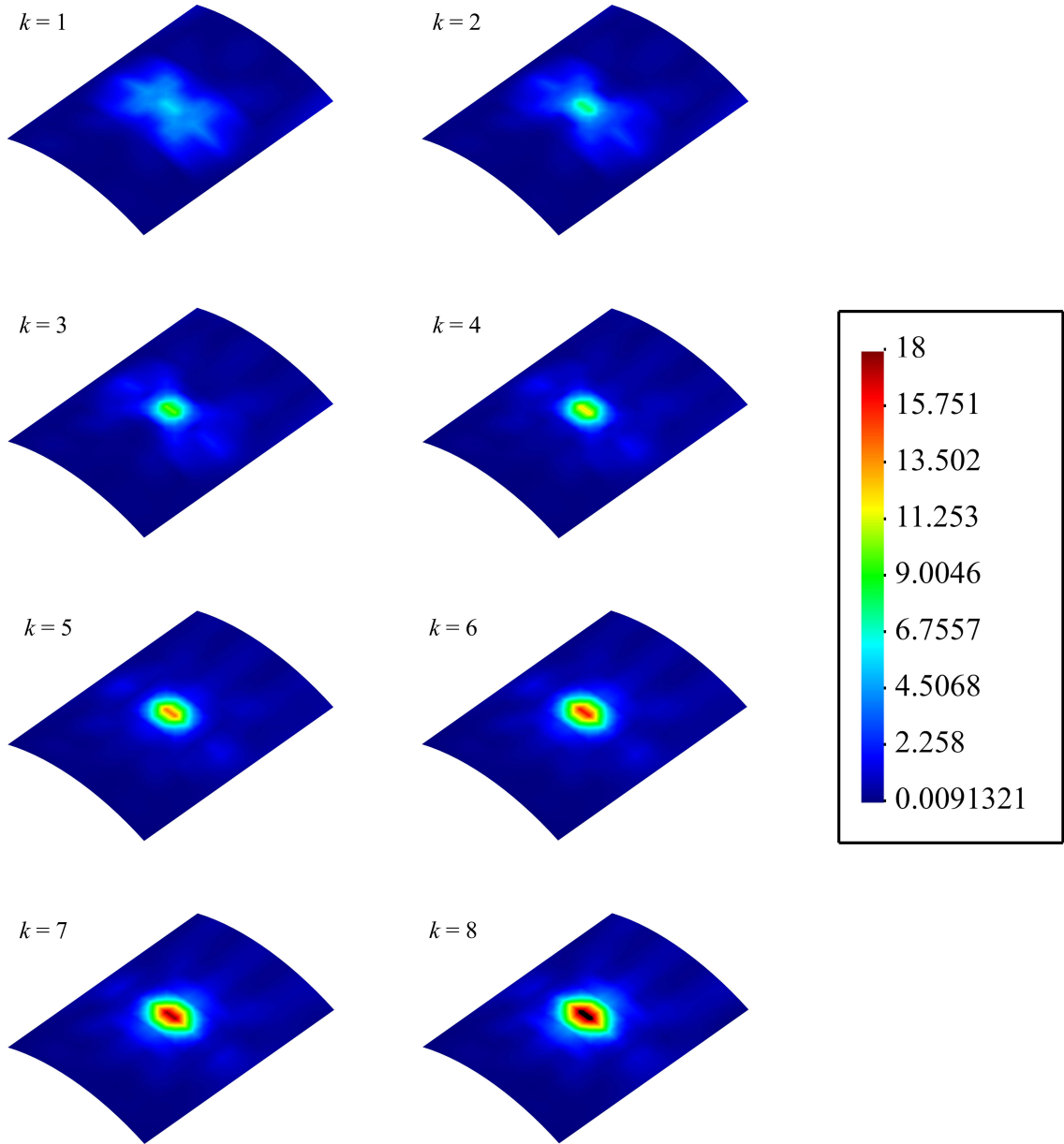
Figure 4.38 Damage indices calculated for each layer of the curved composite panel, for detection of the through-the-thickness location of the defected region.
