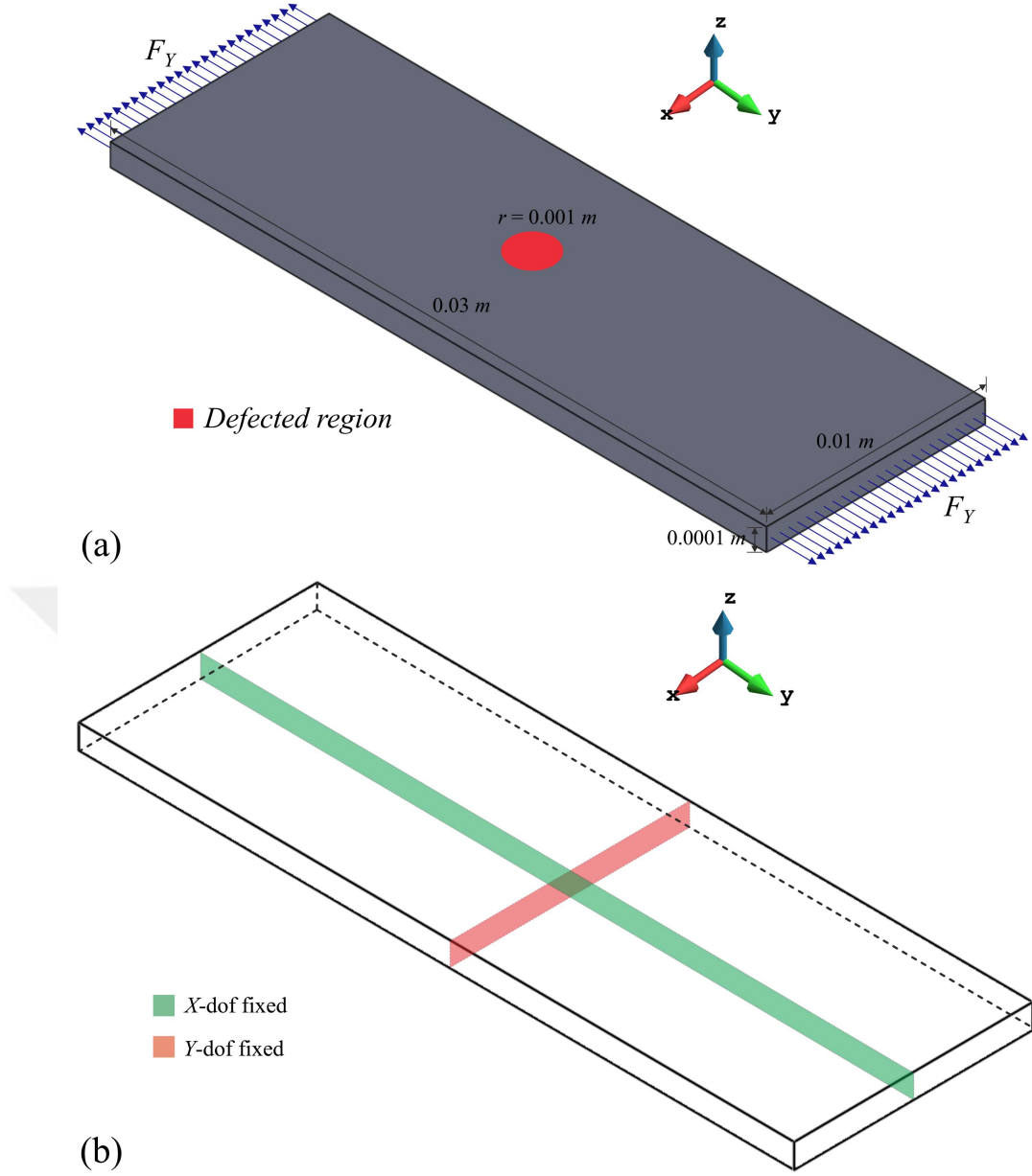
Figure 4.1 (a) Geometry and loading conditions for the plate; (b) Boundary conditions.
