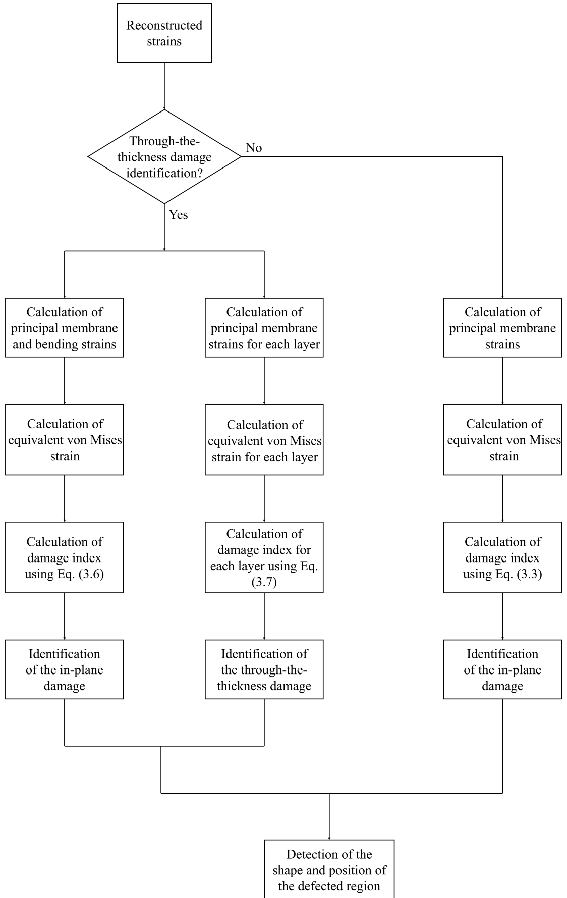
Figure 3.1 The flowchart illustrating the damage detection process.
