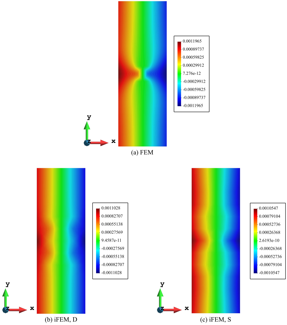
Figure 4.5 Displacement U contours: (a) Forward FEM analysis; (b) iFEM analysis using dense sensor distribution; (c) iFEM analysis using sparse sensor distribution.
