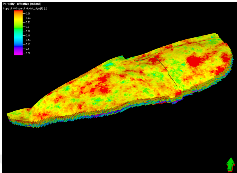
Figure 19 - Porosity distribution map (Bender and Yilmaz, 2014)
