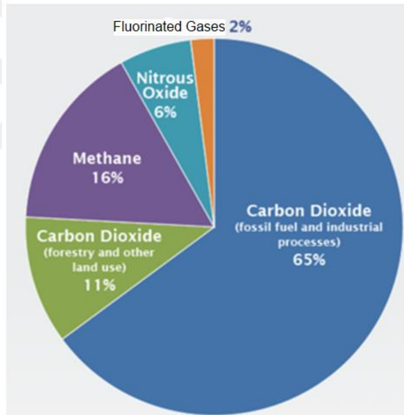
Figure 10- Global greenhouse emissions by gas (Pachauri and Meyer, 2014)
