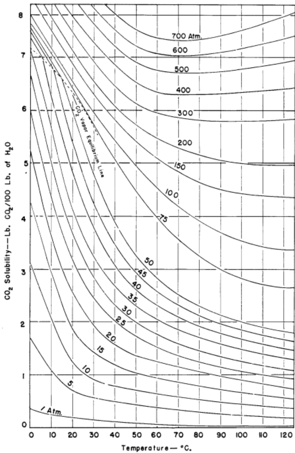
Figure 2 - CO 2 Solubility in water vs pressure and temperature (Dodds et al., 1956)
