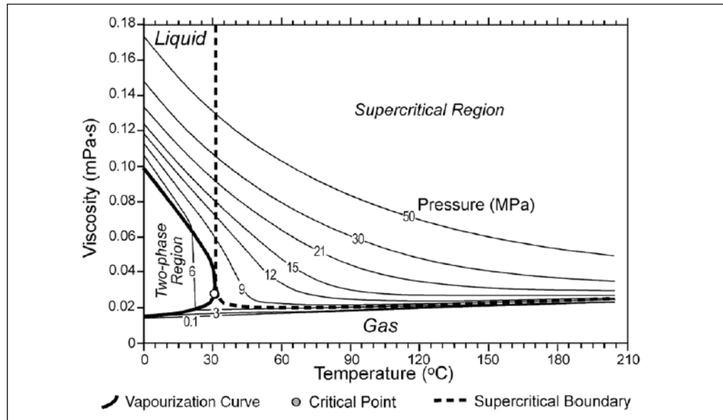
Figure 8 - CO 2 Viscosity vs temperature and pressure (Bachu, 2003)
