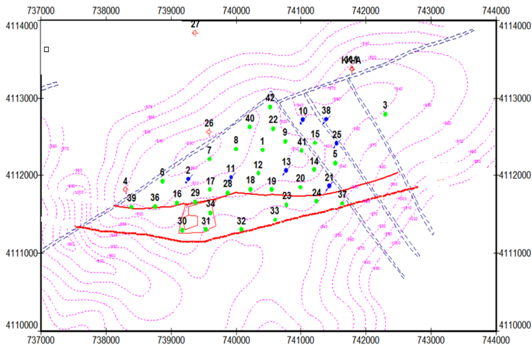
Figure 15- Field structure map (Bender and Yilmaz, 2014)
