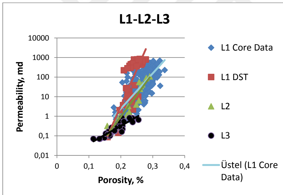
Figure 20 - Permeability and porosity relationship for Layers 1, 2, 3
