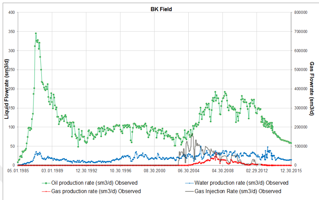
Figure 16 - Field production and injection history
