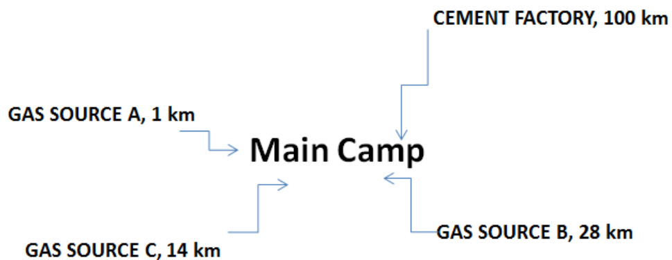
Figure 12 - Distance of the sources to the main camp
