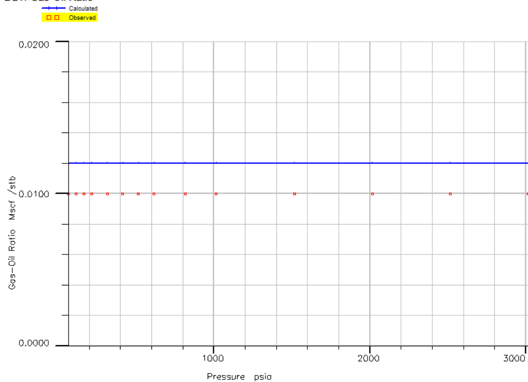
Figure 25 - GOR from DLE experiment vs calculated
