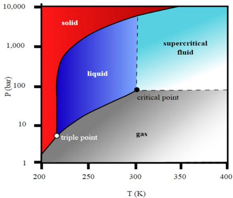
Figure 6 - CO 2 Phase diagram (Lower, 2016)
