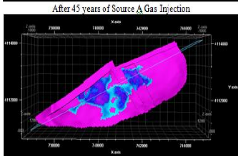
Figure 43 - 3D view of gas saturation distributions for CO 2 injection case, flue gas injection case and Source A gas injection case, 01.01.2116
