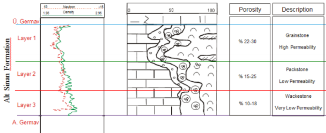
Figure 17 - Petrographic and log characteristics of the reservoir (Bender and Yilmaz, 2014)
