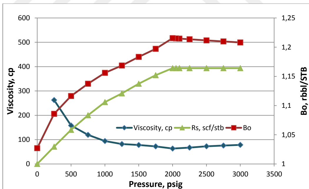
Figure 14 - Oil & Gas mixture properties vs pressure (Bender and Yilmaz, 2014)
