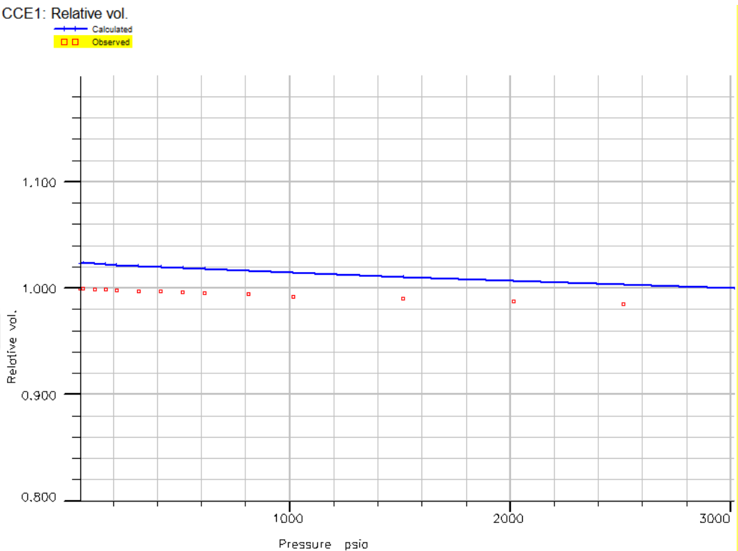
Figure 23 - Relative volumes from CCE experiment vs calculated
