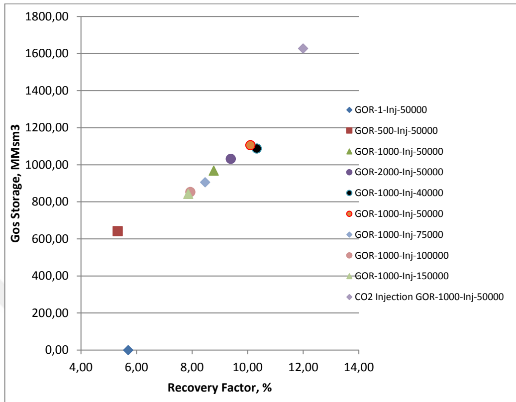
Figure 35 - Amount of flue gas storage vs recovery factor
