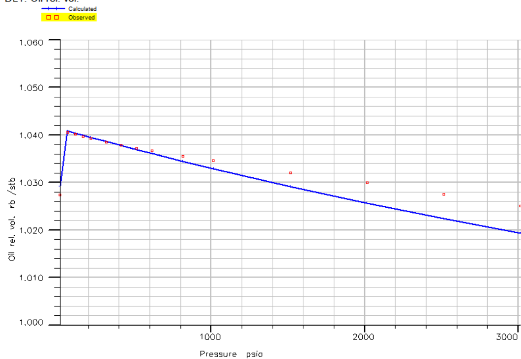
Figure 26 - B_0 from DLE experiment vs calculated
