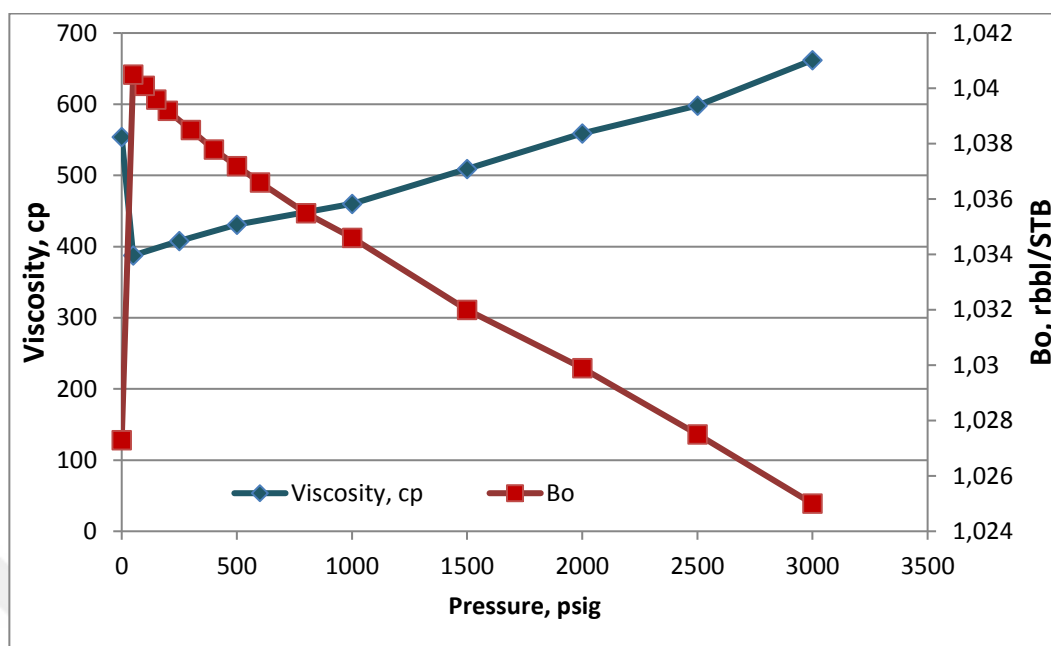
Figure 13 - Oil properties vs pressure (Bender and Yilmaz, 2014)
