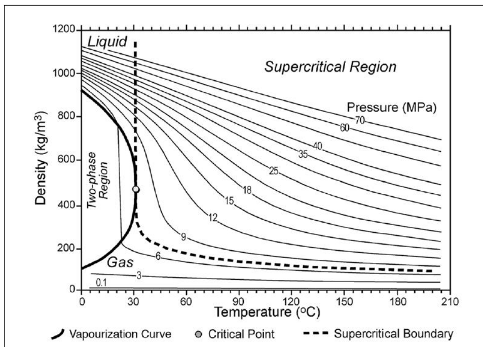
Figure 7 - CO 2 Density vs temperature and pressure (Bachu, 2003)
