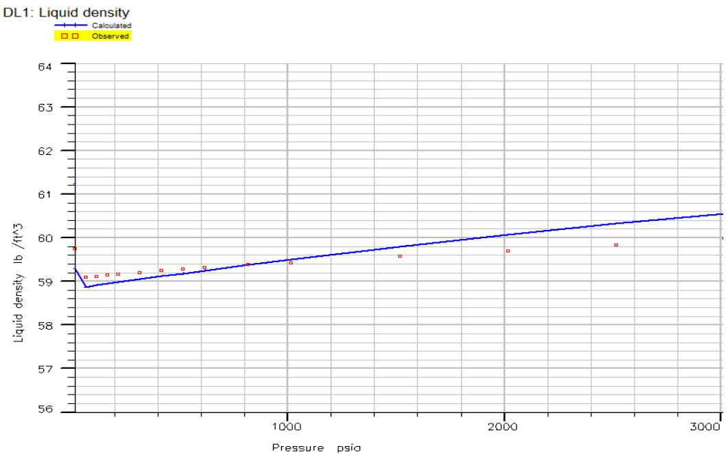
Figure 24 - Liquid density from DLE experiment vs calculated
