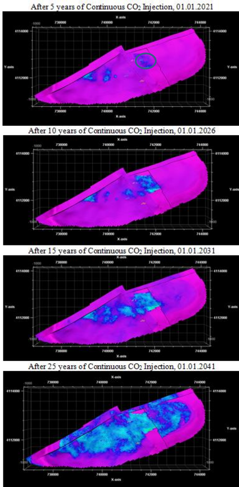
Figure 40 - 3D view of CO 2 saturation distribution from 2021 to 2041 (Continuous CO 2 injection case)
