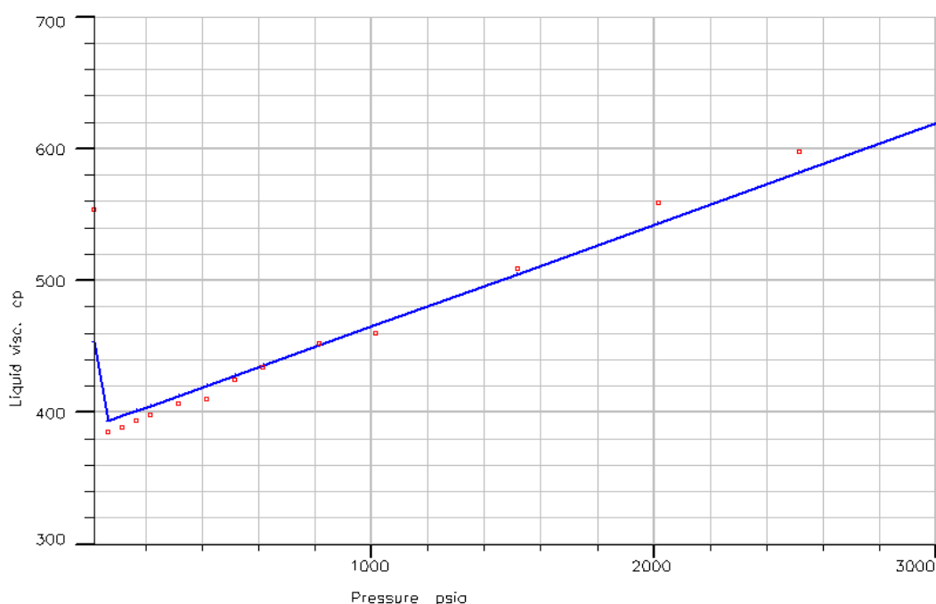
Figure 27 - Viscosity from viscosity experiment vs calculated
