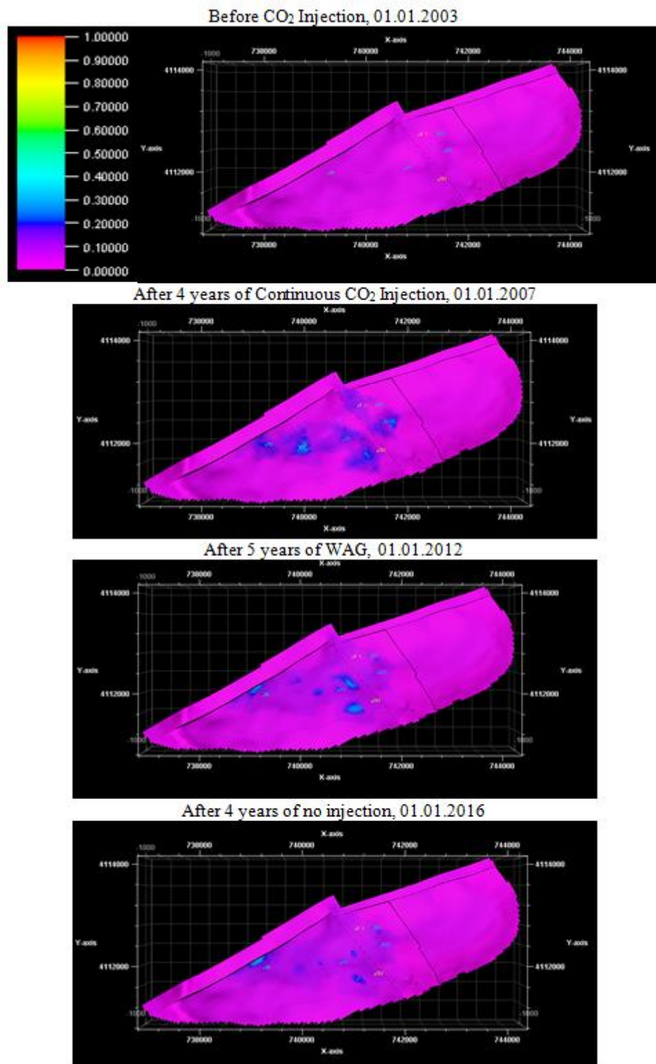
Figure 39 - 3D view of CO 2 saturation distribution from 2003 to 2016 (Real case)
