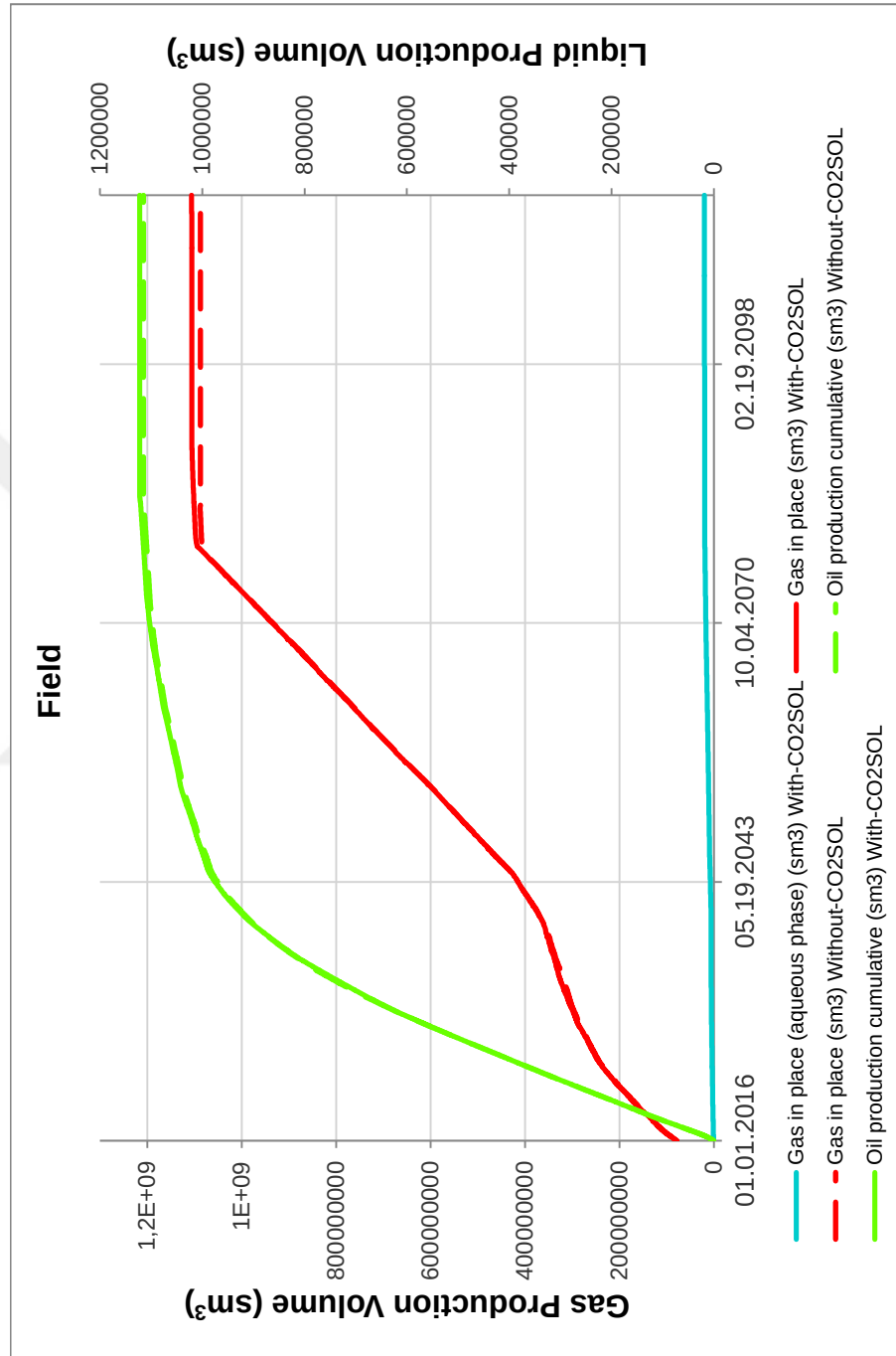
Figure 32 - Cumulative oil production, gas in place and CO 2 dissolved in aqueous phase with and without CO 2 SOL
