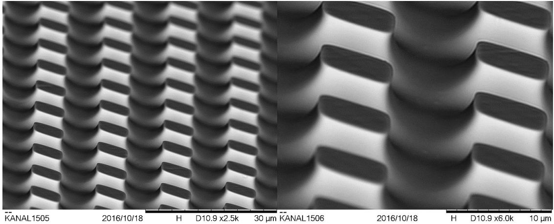
Figure 3.4: SEM images of mesa etch profile.
