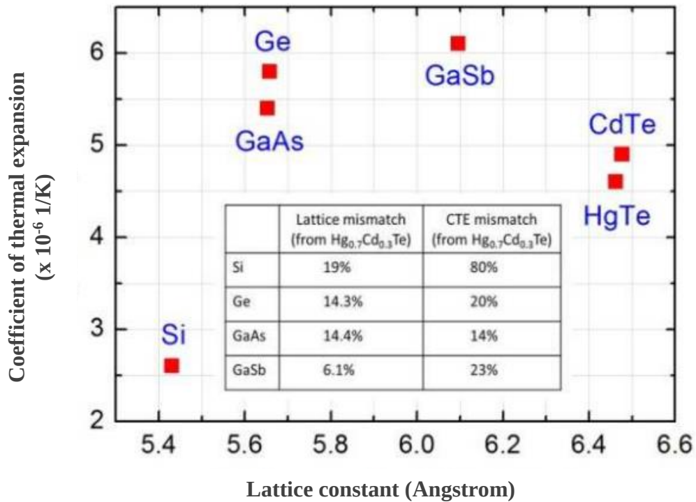
Figure 2.14: Lattice constant and CTEs for various semiconductors used as a substrate for HgCdTe growth [34].
