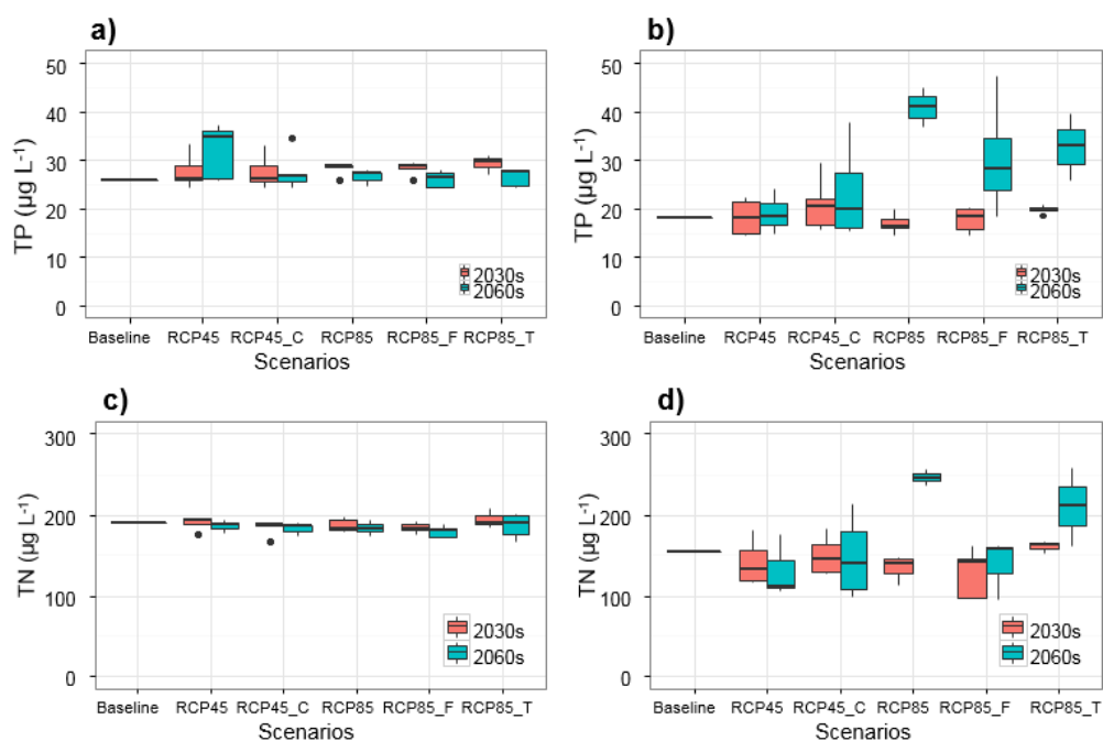
Figure 4.8 Future outputs of lake models for lake a-b) TP and c-d) TN. Left panels indicate the results of GLM-AED model; right panels indicate the results of PCLake model. RCP 4.5 and RCP 8.5: All GCMs without land use change for RCP 4.5 and RCP 8.5 scenarios, respectively. RCP45_C: RCP 4.5 with Consensus World Scenario; RCP 85_F: RCP 8.5 with Fragmented World Scenario; RCP85_T: RCP 8.5 with Techno World Scenario. Each boxplot was generated using averages of each GCM results.
