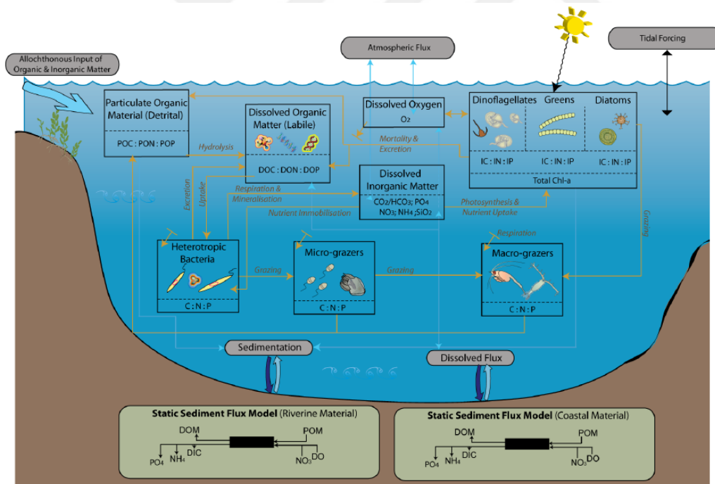
Figure 1.5 Overview of the Aquatic EcoDynamics Library (AED) conceptual model (Hipsey et al., 2013) for nutrient pathways and organisms. Text in black box indicates the simulated variables and gray text indicates the simulated processes.
