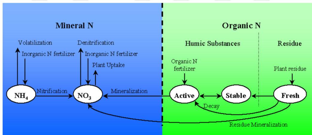
Figure 1.2 Nitrogen cycle in SWAT model (taken from Neitsch et al., 2011)
