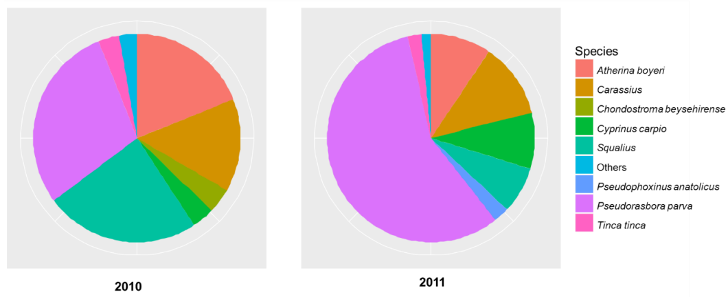
Figure 2.9 Relative abundances of the fish in Lake Beyşehir in September 2010 and 2011. Carassius includes both Carassius carassius and Carassius sp. , Squalius includes Squalis anatolicus , Squalis lepidus , and Squalis cephalus .
