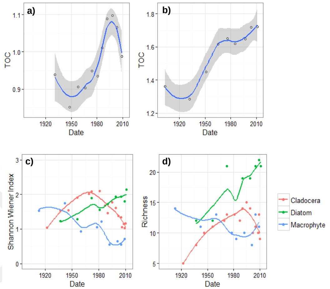
Figure 5.5 Supporting services indicators of Lake Beyşehir a-b) Total organic carbon for pelagic (left) and littoral (right), c) Shannon-Wiener index, d) Richness for Cladocera, Diatoms, and Macrophytes. Solid lines indicate curve-fitted with Loess function. Gray band indicates the confidence interval of the curve fitting.
