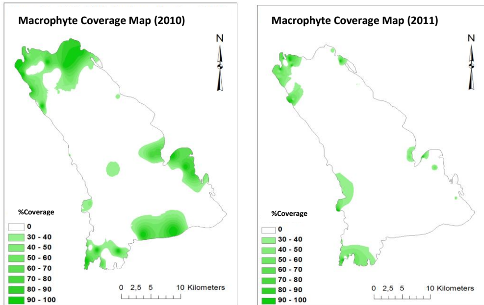
Figure 2.7 Macrophyte coverage of the Lake Beyşehir for a) 2010 and, b) 2011
