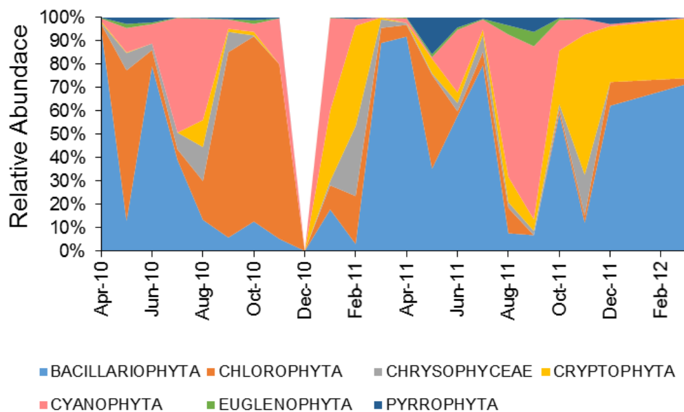
Figure 2.5 Relative abundances of phytoplankton groups during the 2010-2012 sampling period. Phytoplankton sample was not available for December 2010.
