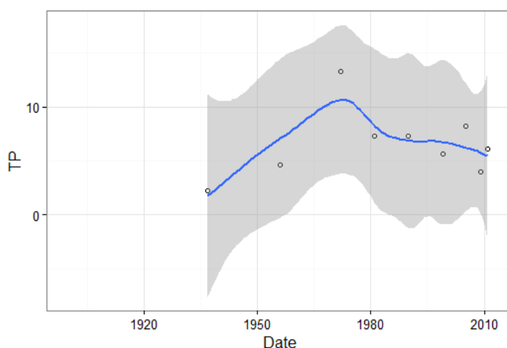
Figure 5.10 Reconstructed TP concentrations inferred from Diatom. The solid blue line shows curve fitted with Loess function. Gray band indicates the confidence interval of the curve fitting.
