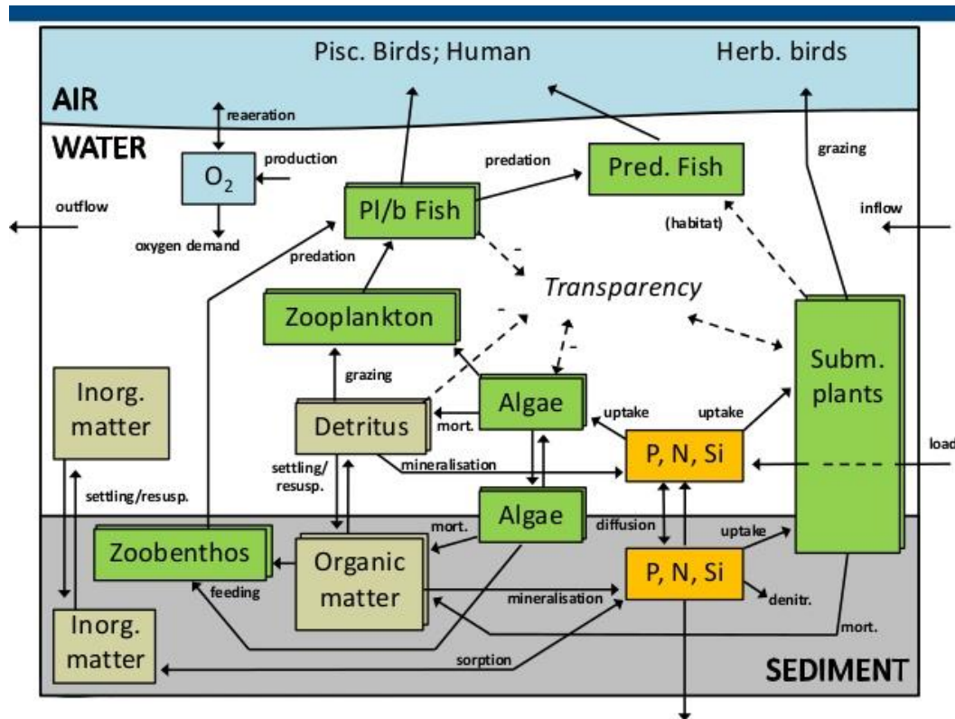
Figure 1.3 Model structure of PCLake. Solid lines represent mass fluxes; dashed lines represents interactions (taken from Jeuken & Janssen, 2014).
