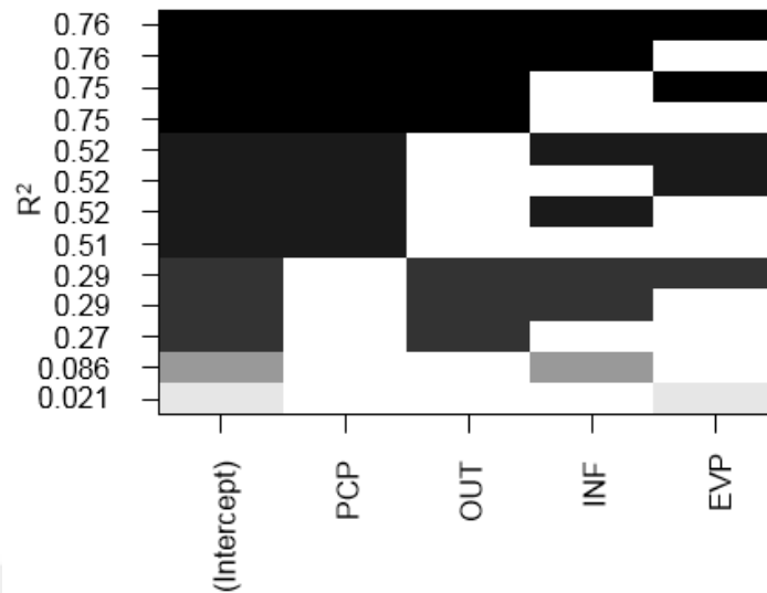
Figure 5.3 R^2 values of different linear model subsets, determining water level change. The black boxes indicate a strong relationship, while gray boxes indicate a weak relationship. PCP: Precipitation, INF: Inflow, OUT: Water abstraction from the lake, EVP: Evaporation. Each row in the graph indicates different subsets of models. For example, the first row at the bottom shows that including only evaporation in the model explains 2% of the variation in water level, while the first row at the top shows full model, which including all variables, explained the 76% of the variation in water level together.
