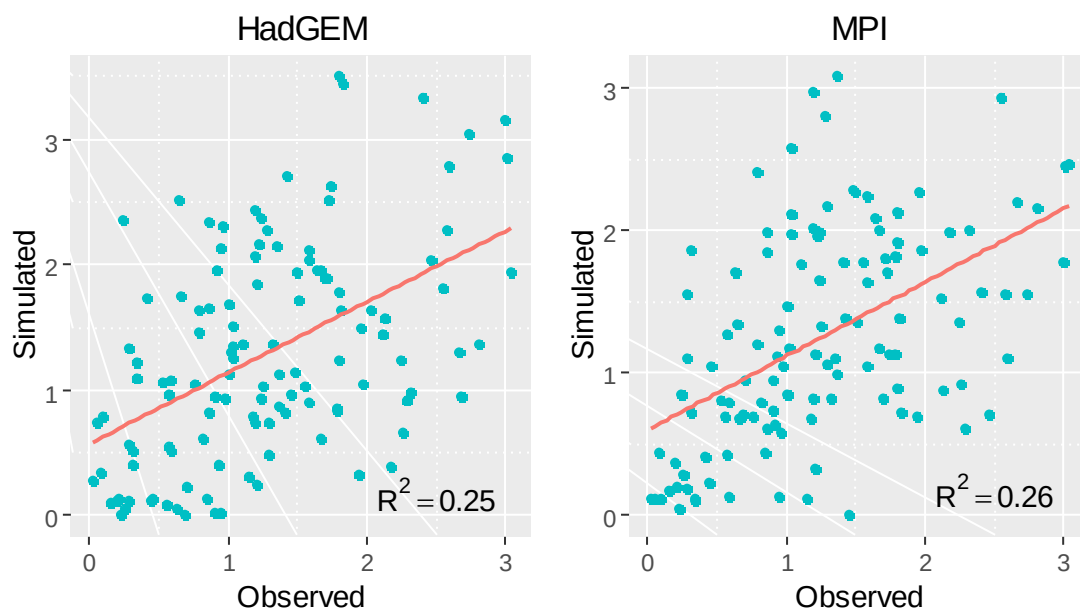
Figure D.3. Comparisons of the observed and bias-corrected simulated values for precipitation (mm) for the period 1971-2000: (a) HadGEM model, (b) MPI model.
