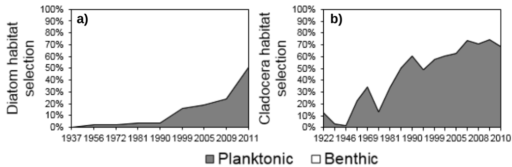
Figure 5.6 Relative distribution of benthic and planktonic species in the sediment a) Diatoms, b) Cladocera.
