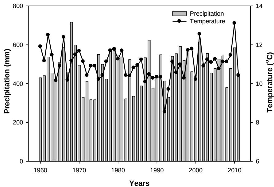
Figure 2.2 Changes in total annual precipitation and the annual average temperature during 1960-2011 recorded in Beyşehir meteorological station. (Data source: Turkish State Meteorological Service, www.mgm.gov.tr ).
