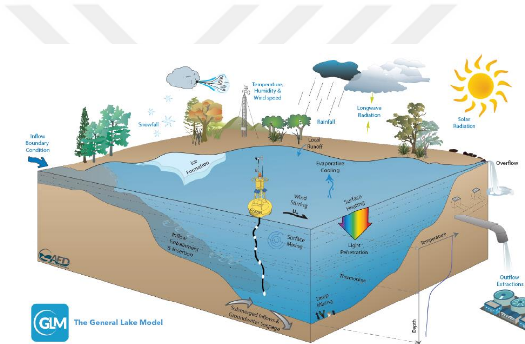
Figure 1.4 Overview of the GLM model (Hipsey et al., 2014). Blue text indicates input information required for setting up the model, while black text indicates key processes simulated.
