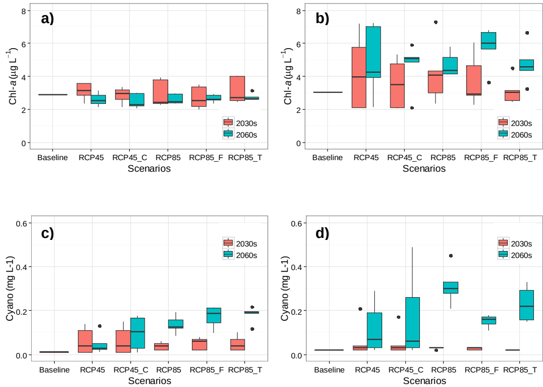
Figure 4.10 Predicted a-b) Chl- a concentrations and, c-d) Cyanobacteria biomass for future scenarios. Left panel represents the outputs of GLM-AED model, right panel represent the outputs of PCLake model. RCP 4.5 and RCP 8.5: All GCMs without land use change for RCP 4.5 and RCP 8.5 scenarios, respectively. RCP45_C: RCP 4.5 with Consensus World Scenario; RCP 85_F: RCP 8.5 with Fragmented World Scenario; RCP85_T: RCP 8.5 with Techno World Scenario. Each boxplot was generated using averages of each GCM results.
