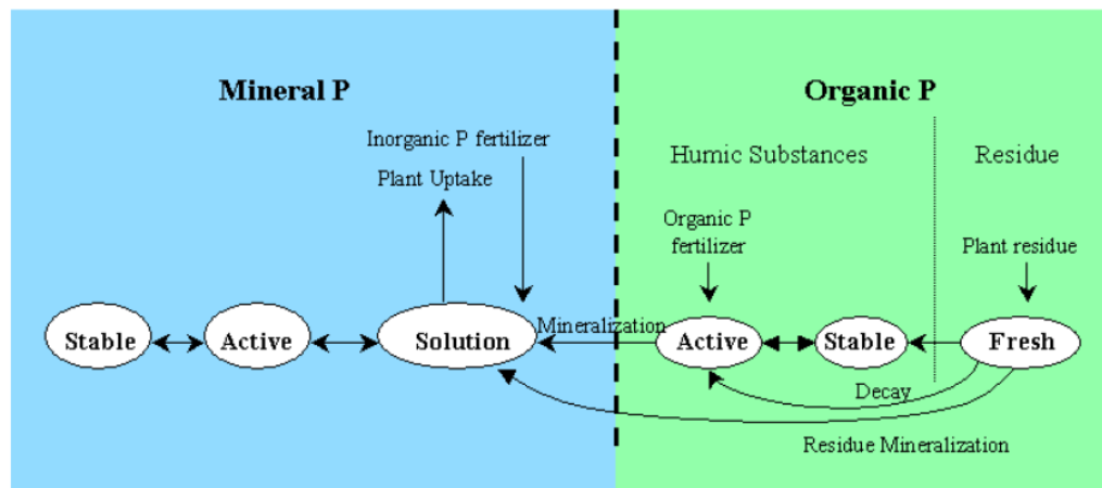
Figure 1.1 Phosphorus cycle in SWAT model (taken from Neitsch et al., 2011)
