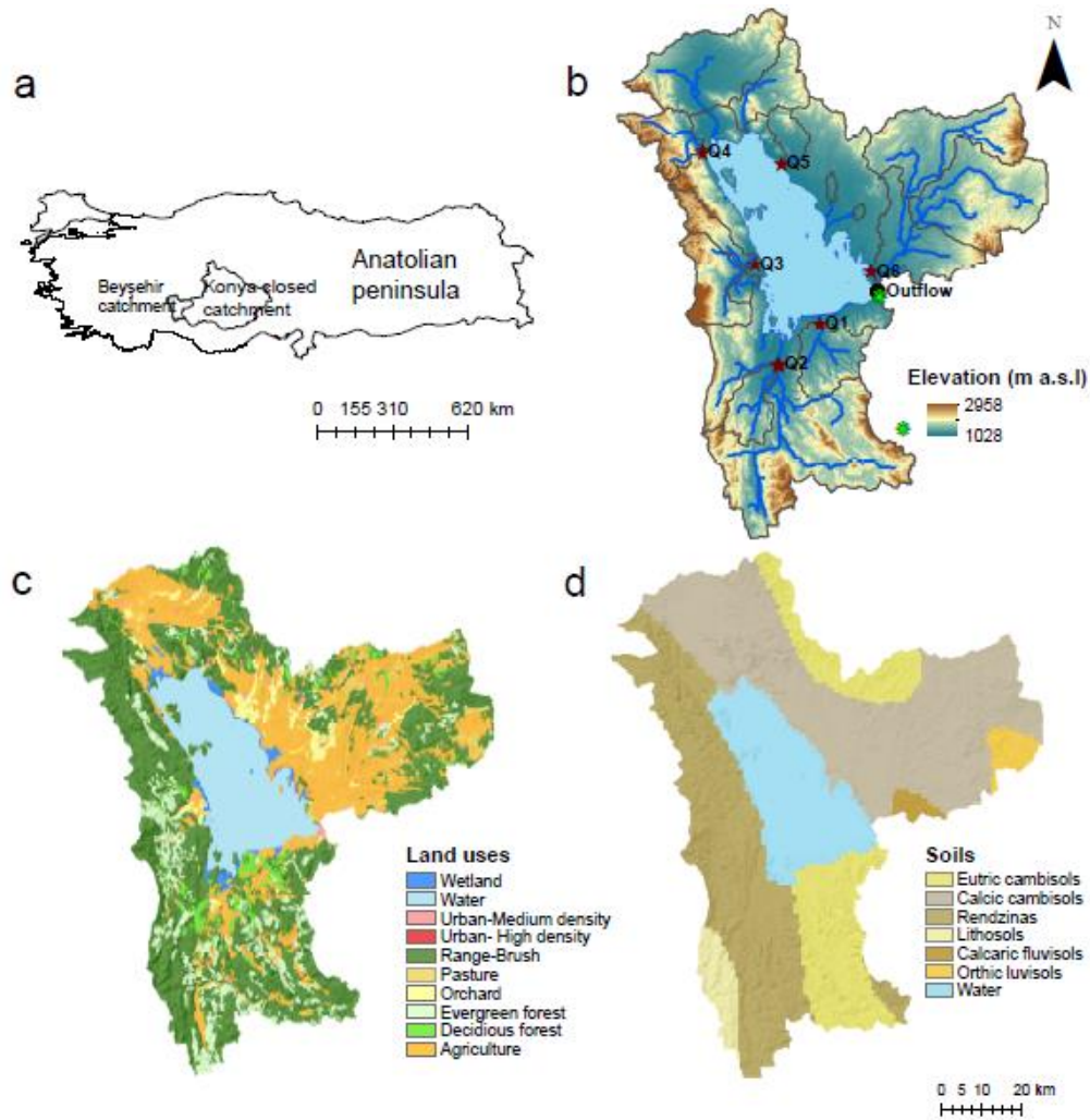
Figure 3.1 Location of the study site and GIS layers used in the SWAT model. (a) Location of the study site; (b) digital elevation map of the Beyşehir catchment. Brown borders show the sub-catchment boundaries. Numbers indicate the inflows (local names of inflows are: Q1: Üstünler, Q2: Soğuksu, Q3: Hizar, Q4: Çelteç, Q5: Tolca-Ozan, Q6: Sarısu) used in the calibration, the black circle shows the outflow, green symbol indicates the meteorology station; (c) distribution of land use categories; (d) soil map.
