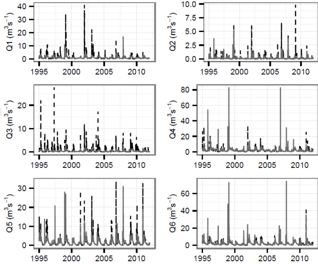
Figure 3.2 Calibration and validation results. Daily simulated (gray, solid lines) and observed (black, dashed lines) flows after calibration of the SWAT model. Q1: Üstünler, Q2: Soğuksu, Q3: Hizar, Q4: Çelteç, Q5: Tolca-Ozan, Q6: Sarısu. X axis indicates dates.
