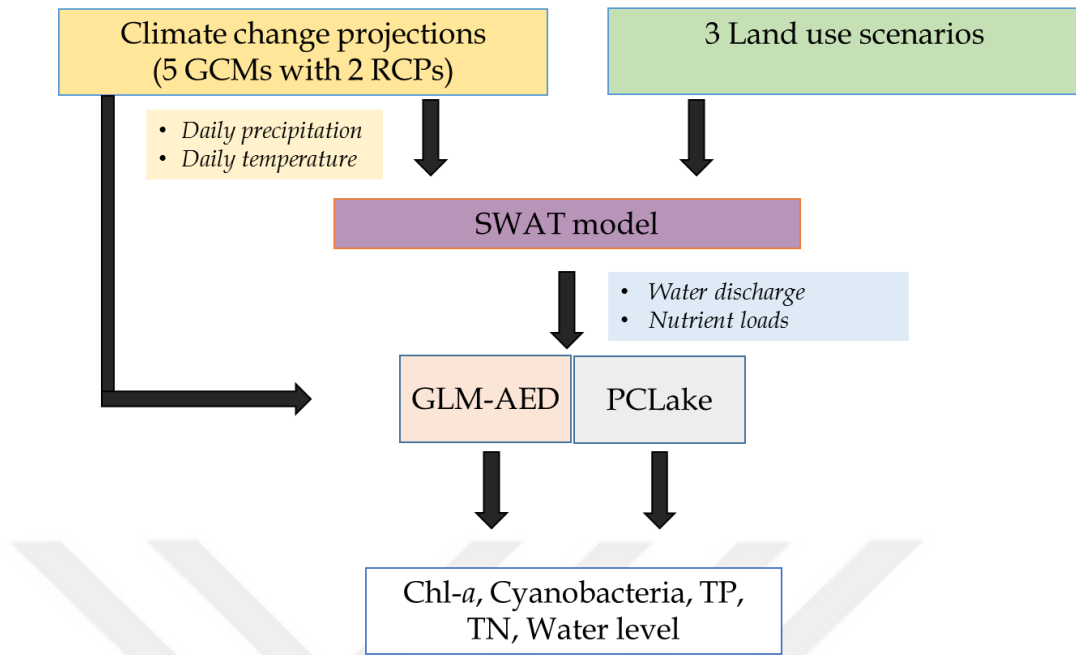
Figure 4.1 Modeling framework used in this study. GCM: General Circulation Model, RCP: Representative Concentrations Pathways, TP: Total Phosphorus, TN: Total Nitrogen, GLM-AED: General Lake Model coupled to Aquatic EcoDynamics Library.
