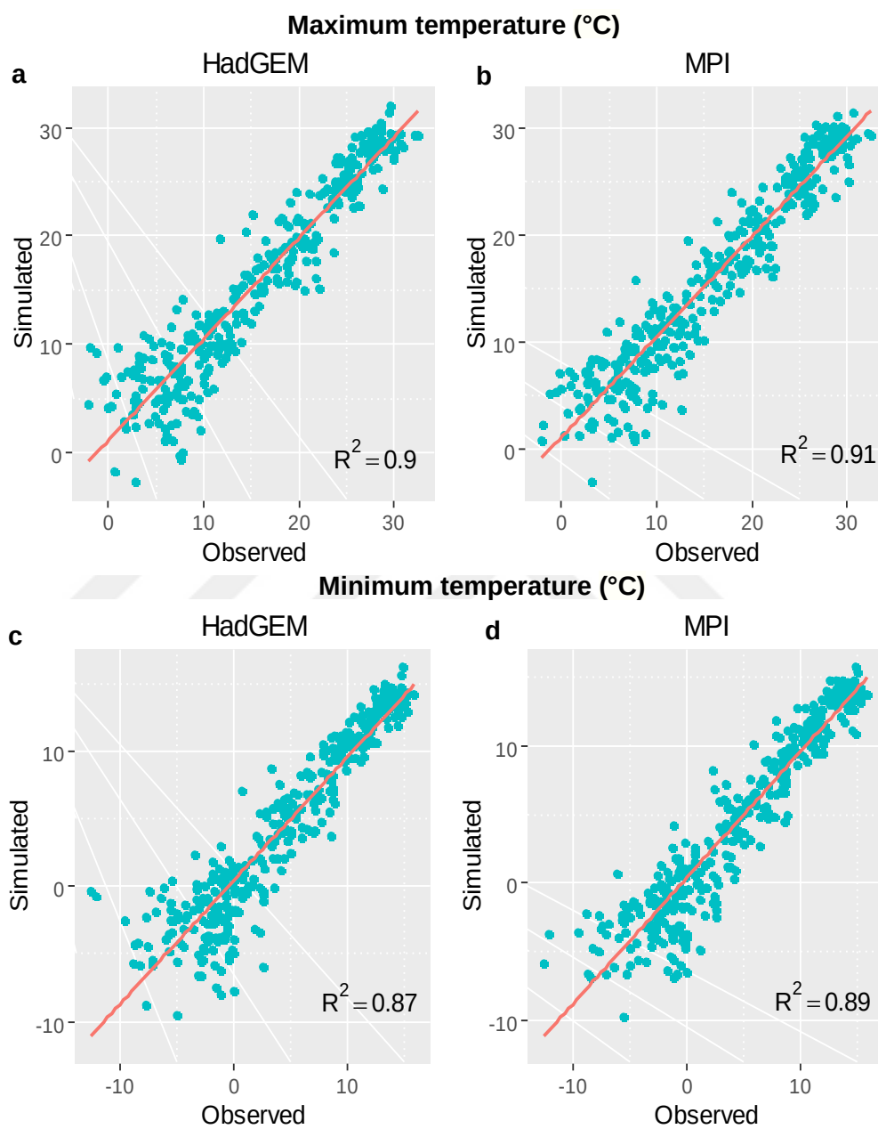
Figure D.1. Comparisons of the observed and bias-corrected simulated values for maximum temperature: (a) HadGEM model, (b) MPI model; and minimum temperature: (c) HadGEM model; (d) MPI model, for the period 1971-2000.
