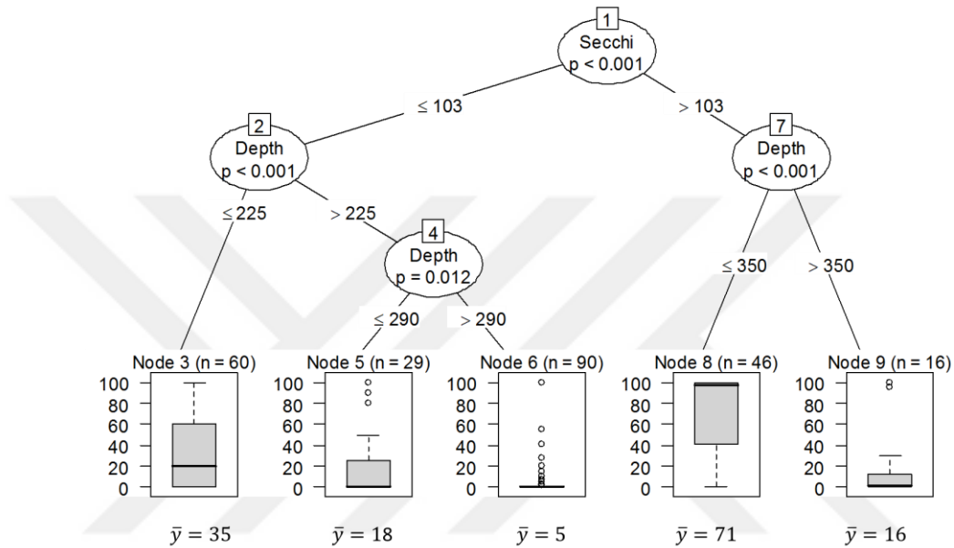
Figure 2.8 Conditional inference trees for macrophyte coverage. \bar{y} indicates mean coverage.
