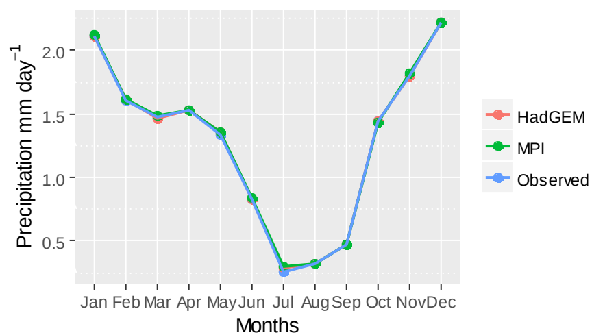
Figure D.4. Comparisons of long term monthly averages of observed and bias-corrected simulated values for the period 1971-2000 for precipitation: (a) HadGEM model and (b) MPI model
