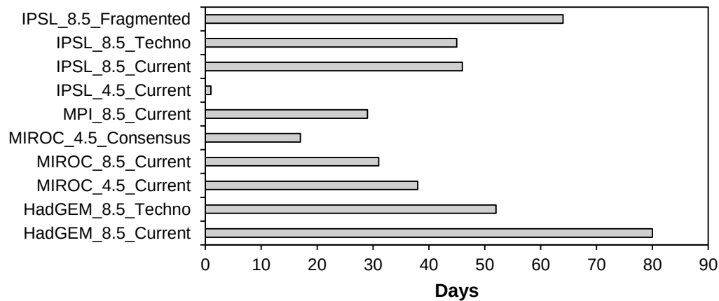
Figure 5.12 Number of days exceeding the low risk WHO limits ( 10 \text{ mg m}^{-3} cyanobacterial Chl- a ) according to future land use and climate scenarios of 2060s period. These outputs were extracted from PCLake results given in Chapter 4. The scenario outputs that did not exceed WHO limits are not shown in the figure.
