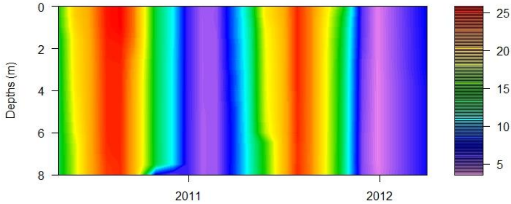
Figure 2.4 Temperature (°C) profile of Lake Beyşehir during the monitoring period of 2010-2012.
