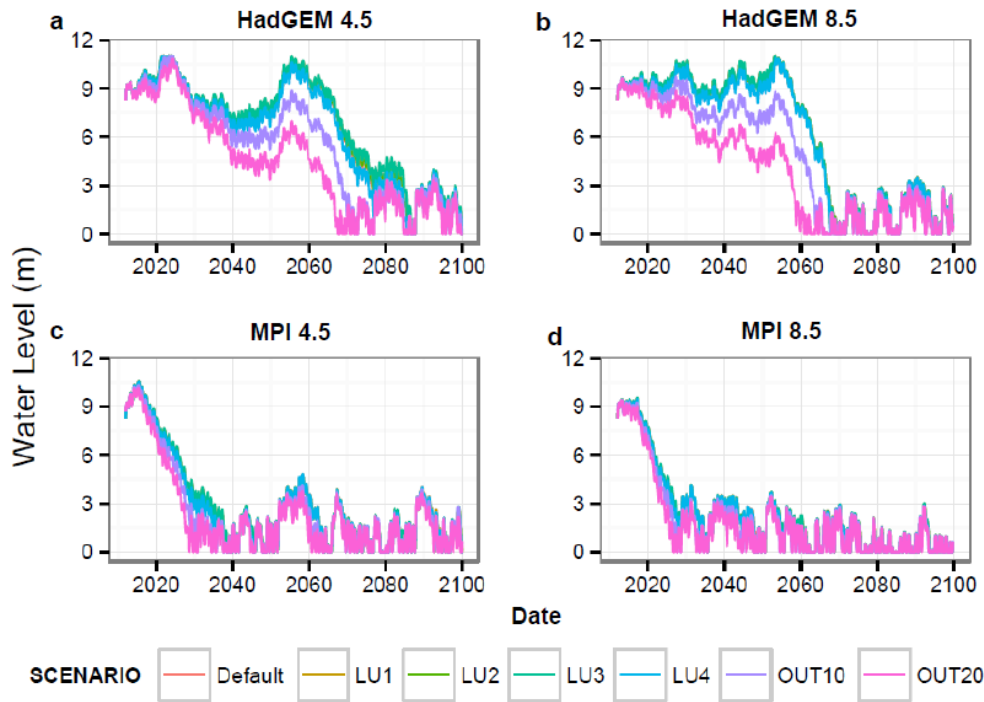
Figure 3.5 The changes in water level in Lake Beyşehir under different climate and land use scenarios during the simulation period for a) HadGEM model, RCP 4.5 scenario, b) HadGEM model, RCP 8.5 scenario, c) MPI model, RCP 4.5 scenario, d) MPI model, RCP 8.5 scena
