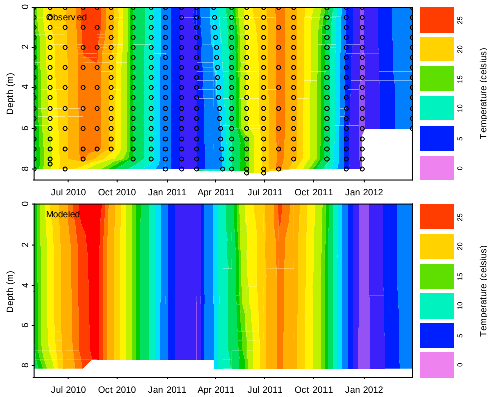
Figure 4.2 Comparison of observed and modeled (GLM-AED) water temperatures for the whole water column during the period of April 2010-March 2012.
