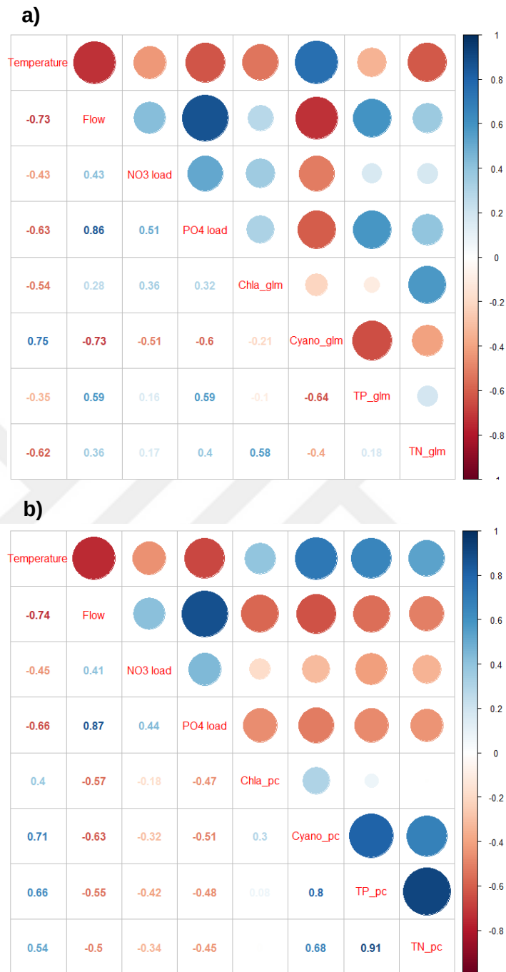
Figure 4.9 Correlation matrix for temperature, flow, NO 3 load, SRP load, Chl- a , Cyanobacteria, lake TP and lake TN for a) GLM-AED model, b) PCLake model. Cyano: Cyanobacteria biomass. Size and color of the circles and the numbers indicate the strength and direction of the correlation.
