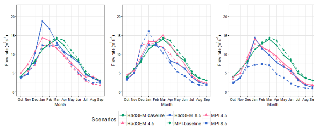
Figure B.1. Changes in average monthly discharges for the different climate scenarios. Baseline period covers 1971-2000, while future scenarios cover the period 2012-2099.
