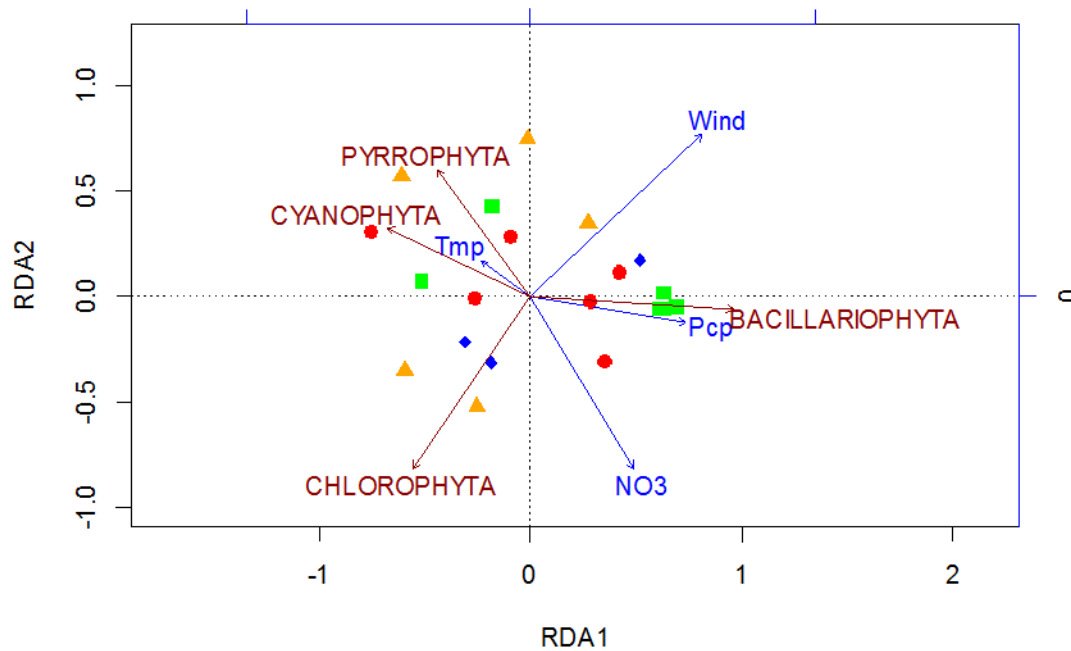
Figure 2.6 RDA results for phytoplankton composition. Orange triangles: autumn, blue diamonds: winter, green squares: spring, red circles: summer. Pcp: Precipitation, Tmp: Temperature.
