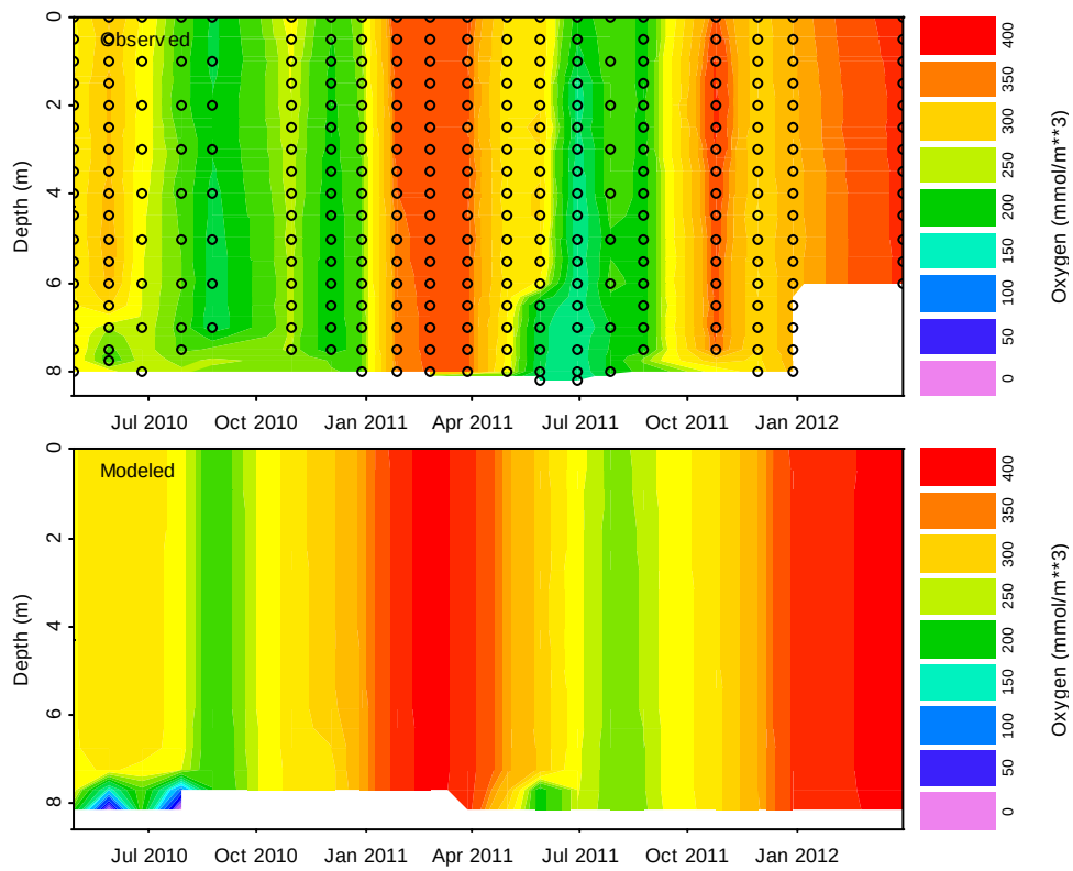
Figure 4.3 Comparison of observed and modeled (GLM-AED) dissolved oxygen concentration profiles for the whole water column during the period of April 2010-March 2012.
