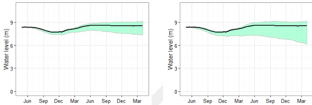
Figure 4.7 Future water levels for all climate change and land use scenarios for a) the 2030s, b) the 2060s. Black lines indicate baseline water level; light green areas indicate the band of all scenario results.
