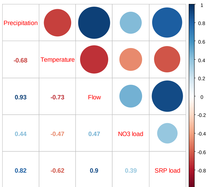
Figure 4.6 Correlation matrix for meteorological variables (precipitation and temperature) with SWAT outputs of flow, NO 3 load, and SRP load. Size and color of the circles and the numbers indicate the strength and direction of the correlation.
