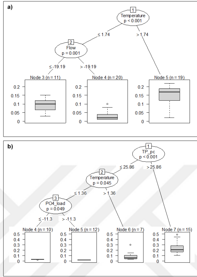
Figure 4.11 Conditional inference trees for Cyanobacteria biomass for a) GLM-AED model, b) PCLake model. Temperature: Relative change to baseline, PO 4 load and flow: % changes compared to baseline, TP_pc: Lake TP concentrations according to PCLake model
