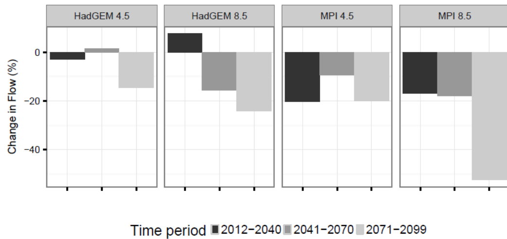
Figure 3.4 Changes in total flow compared with the baseline simulation for 2012-2040, 2041-2070 and 2071-2099 for the MPI and HadGEM climate change models and the RCP 4.5 and RCP 8.5 scenarios.
