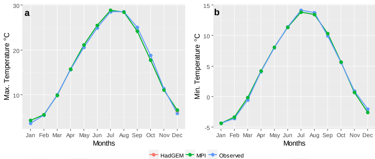
Figure D.2. Comparisons of long term monthly averages of observed and bias-corrected simulated values for the period 1971-2000 for (a) maximum temperature; (b) minimum temperature.
