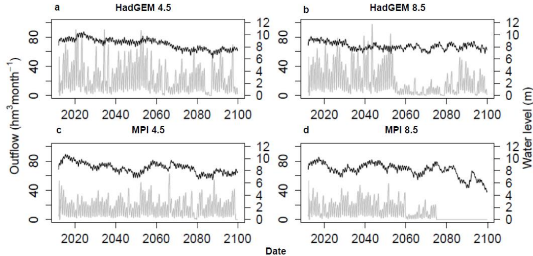
Figure 3.6 Monthly calculated outflow volumes and water level changes for a) HadGEM model, RCP 4.5 scenario, b) HadGEM model, RCP 8.5 scenario, c) MPI model, RCP 4.5 scenario, d) MPI model, RCP 8.5 scenario. Gray lines indicate the outflow and black lines indicate
