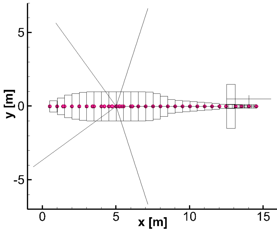
Figure 33. Schematic Representation of Monitor Stations, Top View
