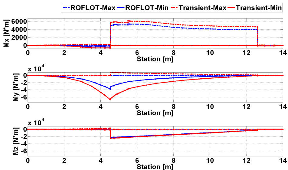
Figure 89. Comparison of Trim and Transient Solution Torsional and Bending Moments for Sea Level, Hover, Gust From Down Condition
