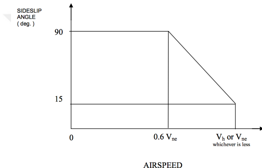
Figure 2. Resulting Sideslip Angle vs. Flight Speed for Yaw Maneuver [7]
