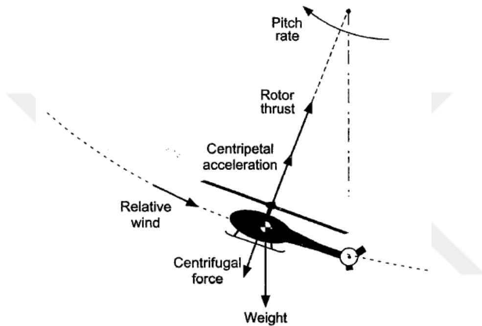
Figure 1. Schematic Representation of the Pull-up Maneuver [5]
