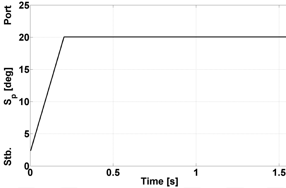
Figure 44. Time History of the Pedal Input Used for the Transient Analysis of the Yaw Maneuver in 80 [knot]
