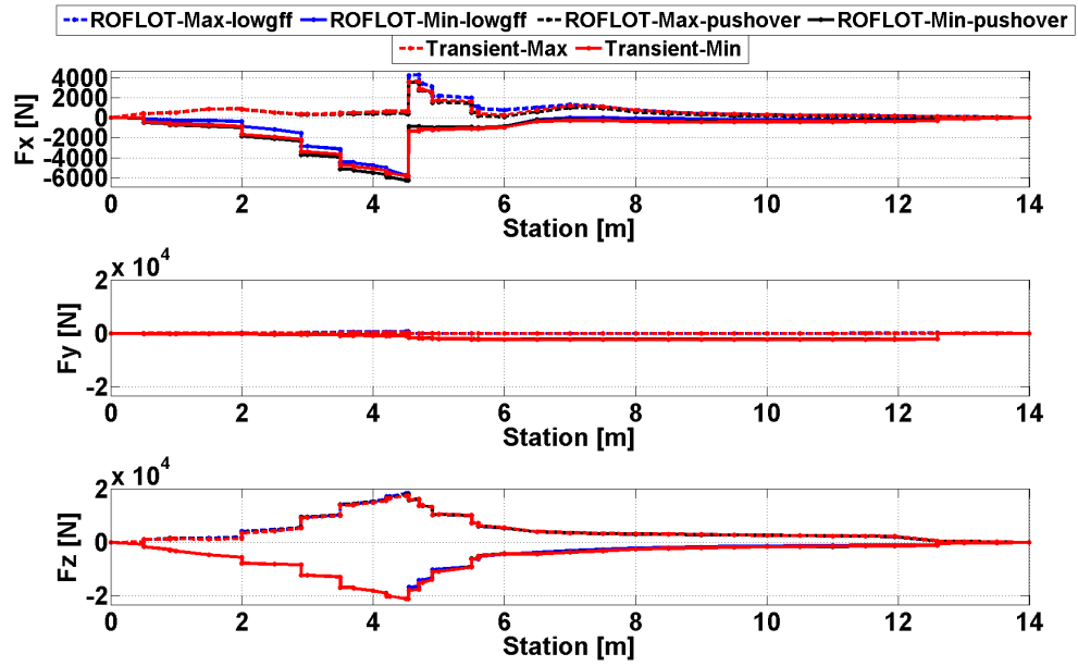
Figure 60. Comparison of Trim and Transient Solution Overall Maximum and Minimum Axial and Shear Forces of the Push-over Maneuvers
