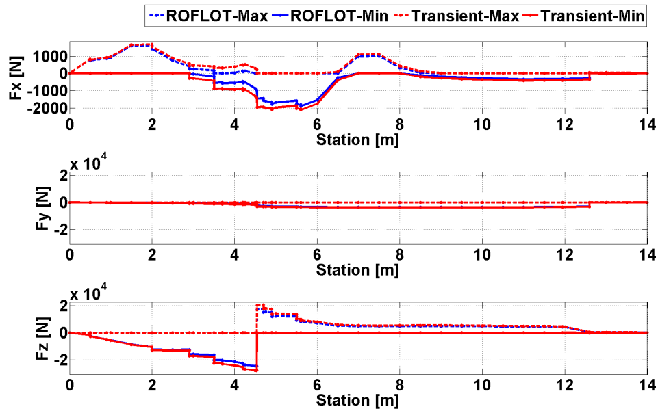
Figure 74. Comparison of Trim and Transient Solution Axial and Shear Forces for Sea Level, 160 [knot] Forward Flight, Gust From Forward Condition
