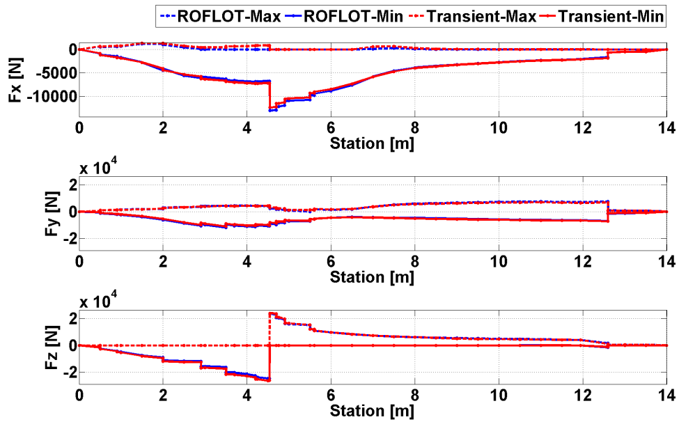
Figure 68. Comparison of Trim and Transient Solution Overall Maximum and Minimum Axial and Shear Forces of the Yaw Maneuvers
