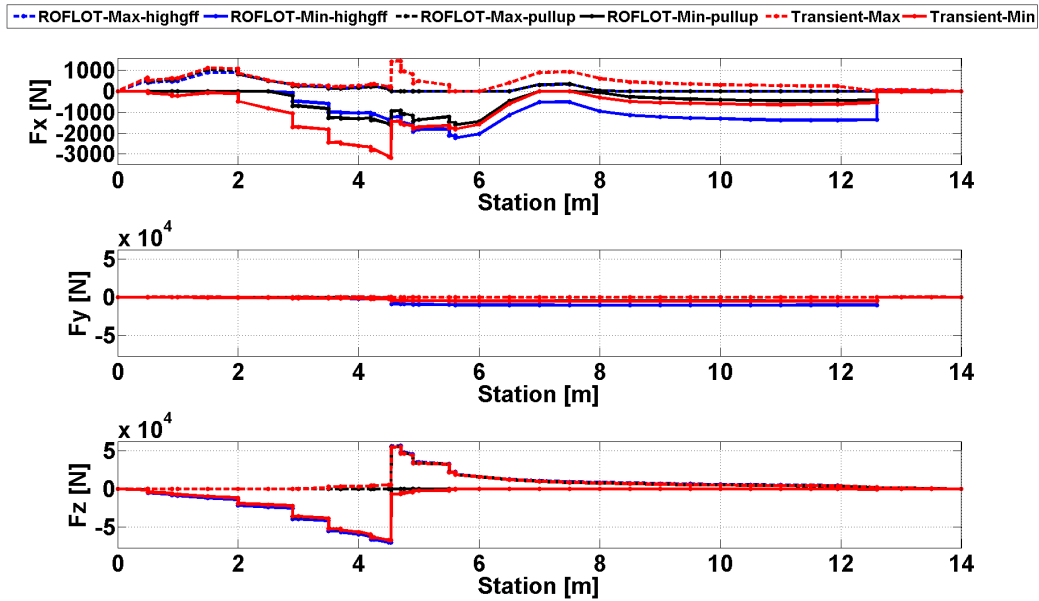
Figure 52. Comparison of Trim and Transient Solution Axial and Shear Forces for Sea Level, ISA -55 C 0 , 120 [knot], 3.5 [g] Pull-up Maneuver
