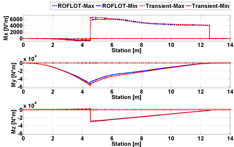
Figure 75. Comparison of Trim and Transient Solution Torsional and Bending Moments for Sea Level, 160 [knot] Forward Flight, Gust From Forward Condition
