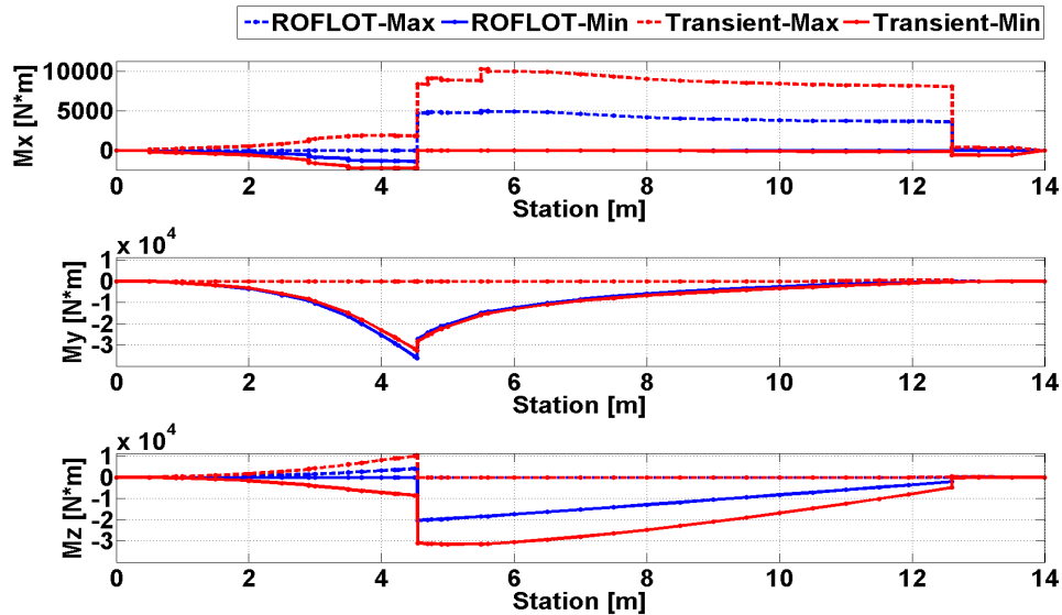
Figure 95. Comparison of Trim and Transient Solution Torsional and Bending Moments for Sea Level, Hover, Gust From Left Condition
