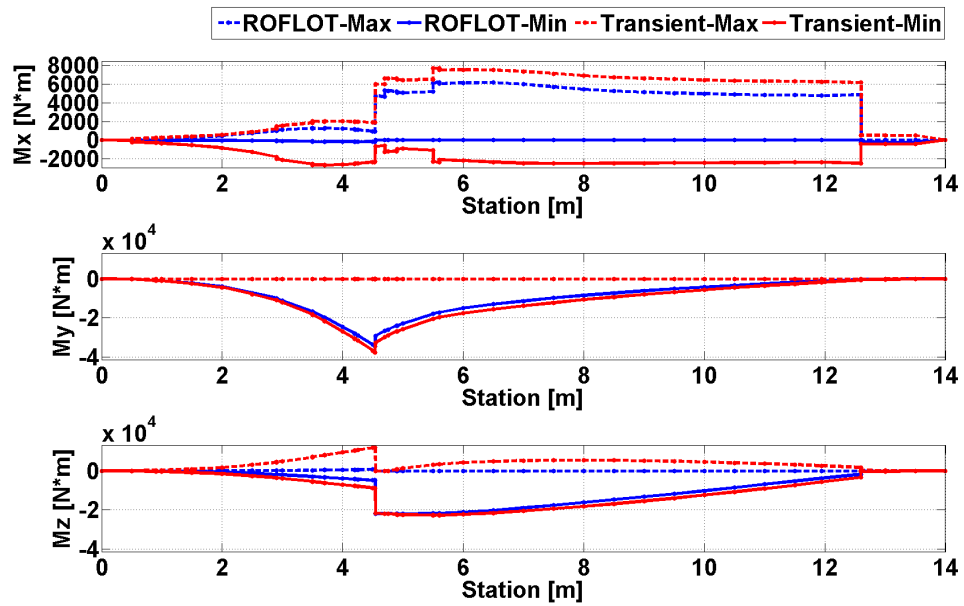
Figure 103. Comparison of Trim and Transient Solution Torsional and Bending Moments for Sea Level, 80 [knot] Forward Flight, Gust From Right Condition
