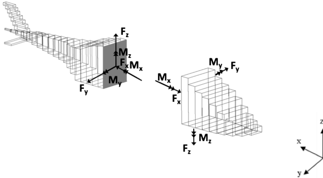
Figure 21. Fuselage Loads Axis System
