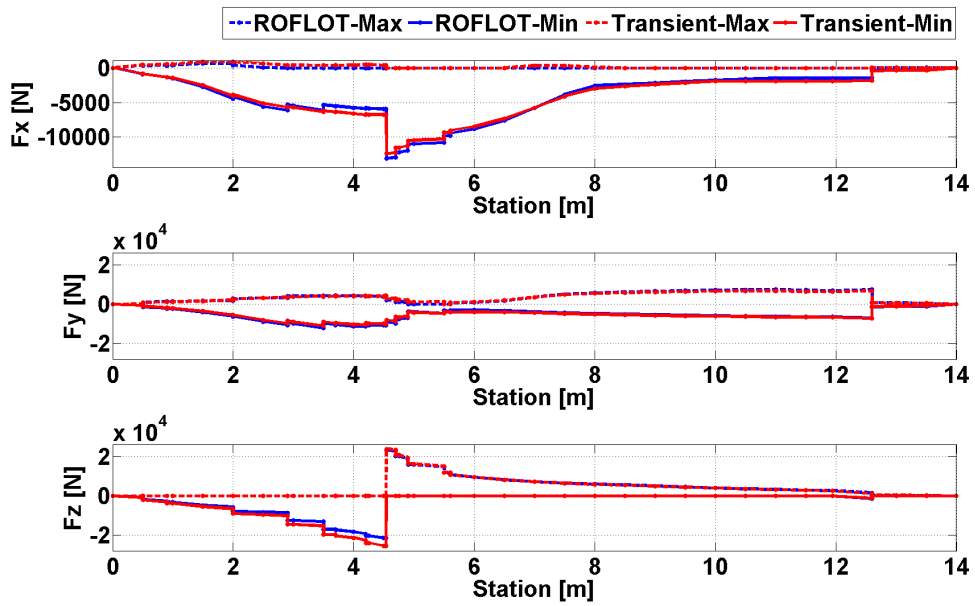
Figure 64. Comparison of Trim and Transient Solution Axial and Shear Forces for Sea Level, 120 [knot], Yaw to Port Maneuver
