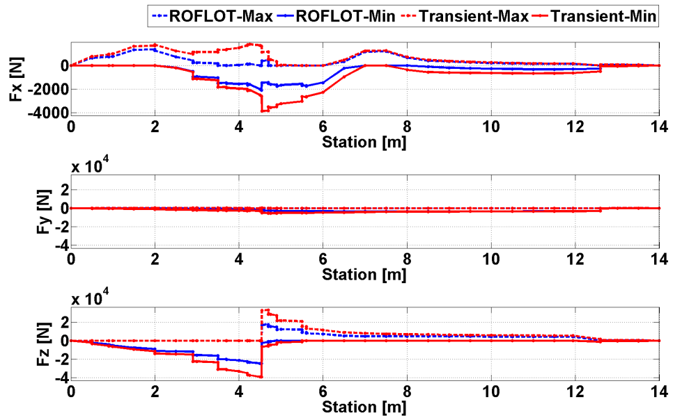
Figure 86. Comparison of Trim and Transient Solution Axial and Shear Forces for Sea Level, 160 [knot] Forward Flight, Gust From Up Condition
