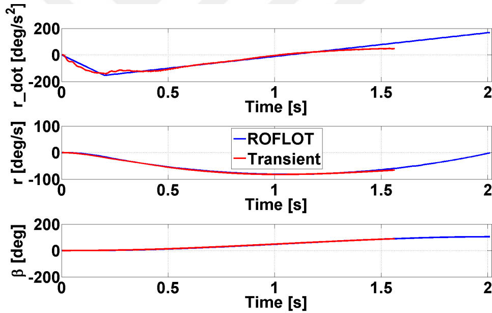
Figure 46. Comparison of the Yaw Acceleration, Yaw Velocity and Sideslip Angle Estimated and Obtained from the Transient Analysis of Yaw to Port Maneuver in 80 [knot]
