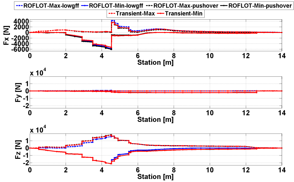
Figure 58. Comparison of Trim and Transient Solution Axial and Shear Forces for Sea Level, ISA -55 C 0 , 120 [knot], -1 [g] Push-over Maneuver
