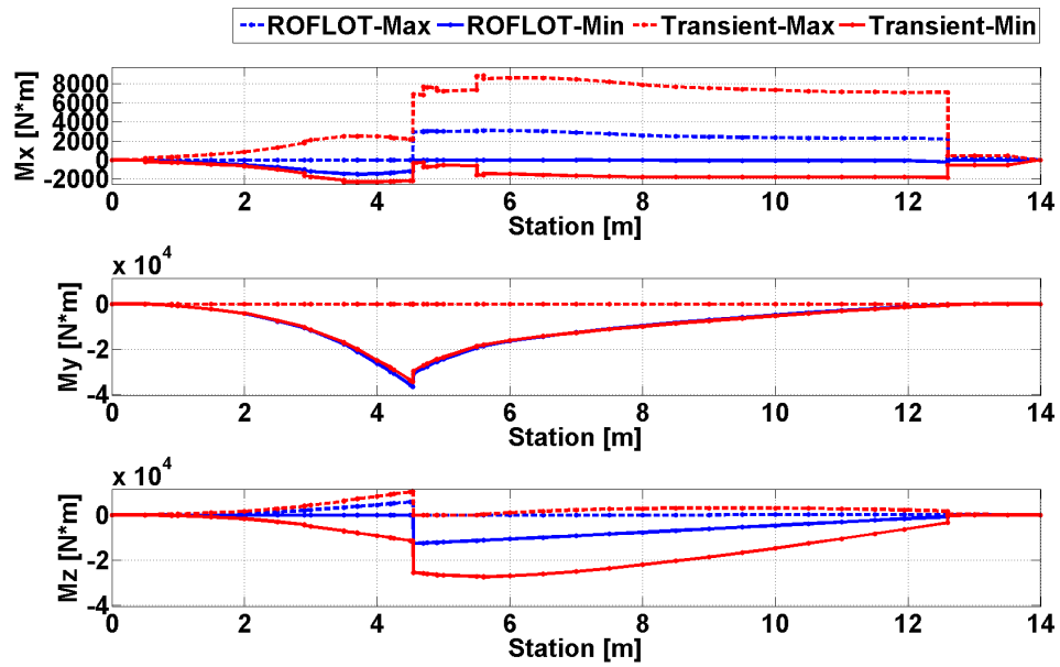
Figure 97. Comparison of Trim and Transient Solution Torsional and Bending Moments for Sea Level, 80 [knot] Forward Flight, Gust From Left Condition
