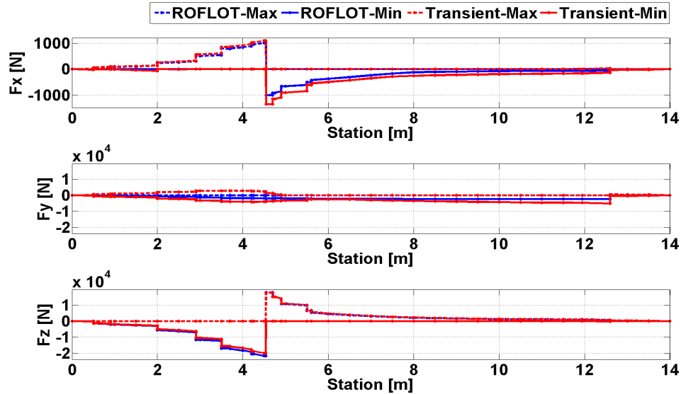
Figure 94. Comparison of Trim and Transient Solution Axial and Shear Forces for Sea Level, Hover, Gust From Left Condition
