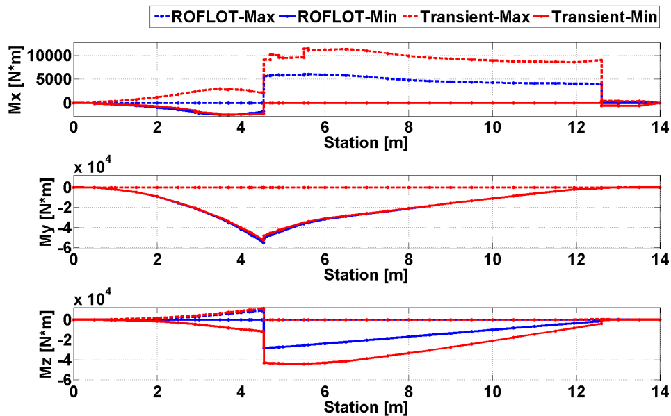
Figure 99. Comparison of Trim and Transient Solution Torsional and Bending Moments for Sea Level, 160 [knot] Forward Flight, Gust From Left Condition
