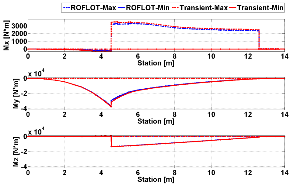
Figure 73. Comparison of Trim and Transient Solution Torsional and Bending Moments for Sea Level, 80 [knot] Forward Flight, Gust From Forward Condition
