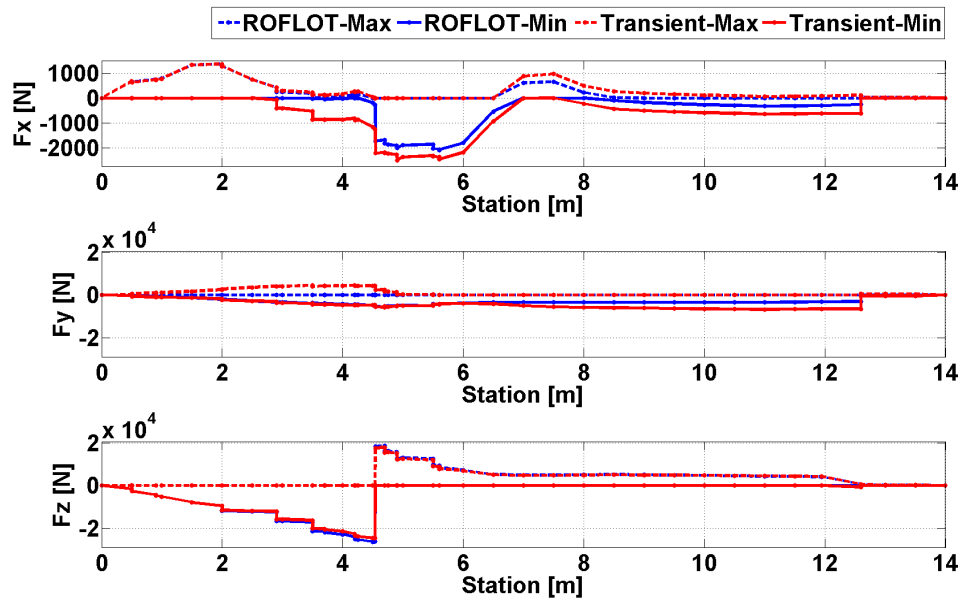
Figure 98. Comparison of Trim and Transient Solution Axial and Shear Forces for Sea Level, 160 [knot] Forward Flight, Gust From Left Condition
