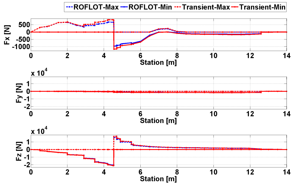
Figure 72. Comparison of Trim and Transient Solution Axial and Shear Forces for Sea Level, 80 [knot] Forward Flight, Gust From Forward Condition
