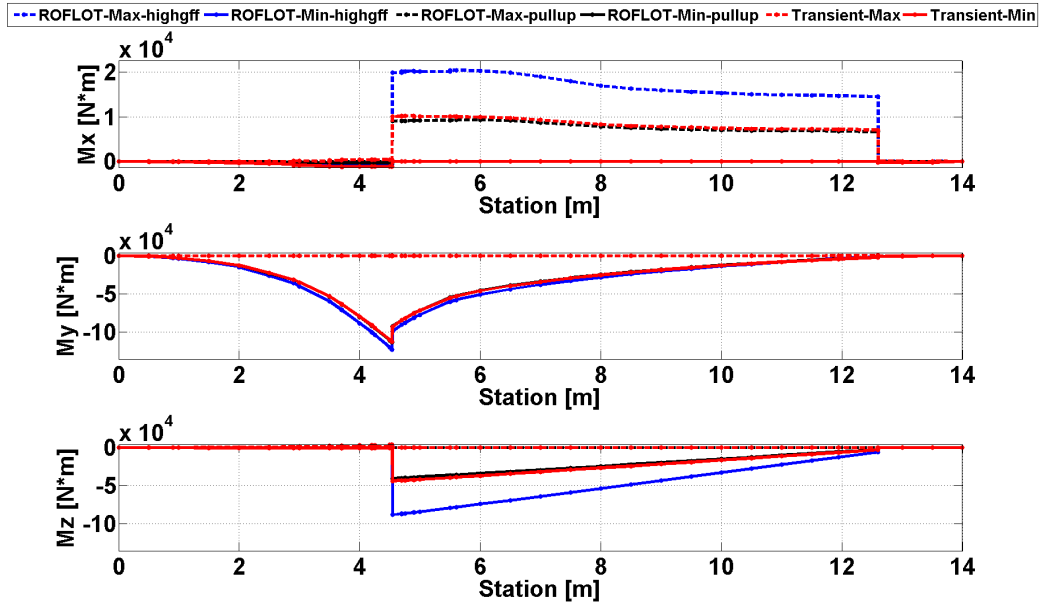
Figure 53. Comparison of Trim and Transient Solution Torsional and Bending Moments for Sea Level, ISA -55 C 0 , 120 [knot], 3.5 [g] Pull-up Maneuver
