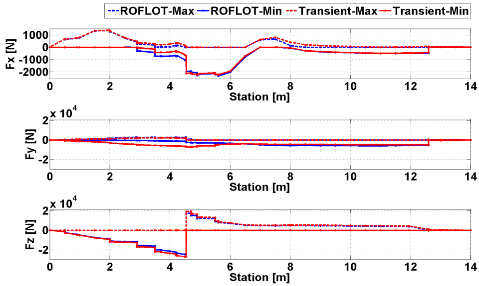
Figure 104. Comparison of Trim and Transient Solution Axial and Shear Forces for Sea Level, 160 [knot] Forward Flight, Gust From Right Condition
