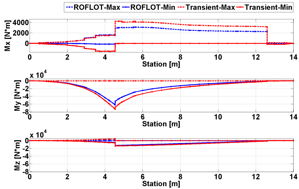
Figure 91. Comparison of Trim and Transient Solution Torsional and Bending Moments for Sea Level, 80 [knot] Forward Flight, Gust From Down Condition
