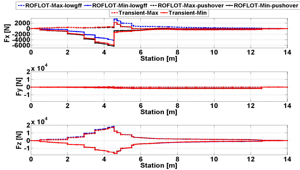
Figure 56. Comparison of Trim and Transient Solution Axial and Shear Forces for Sea Level, ISA -55 C^0 , 80 [knot], -1 [g] Push-over Maneuver
