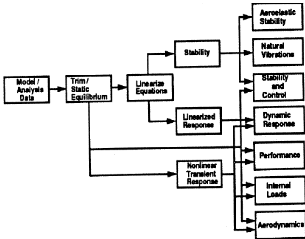
Figure 13. 2GCHAS Analysis Options [15]
