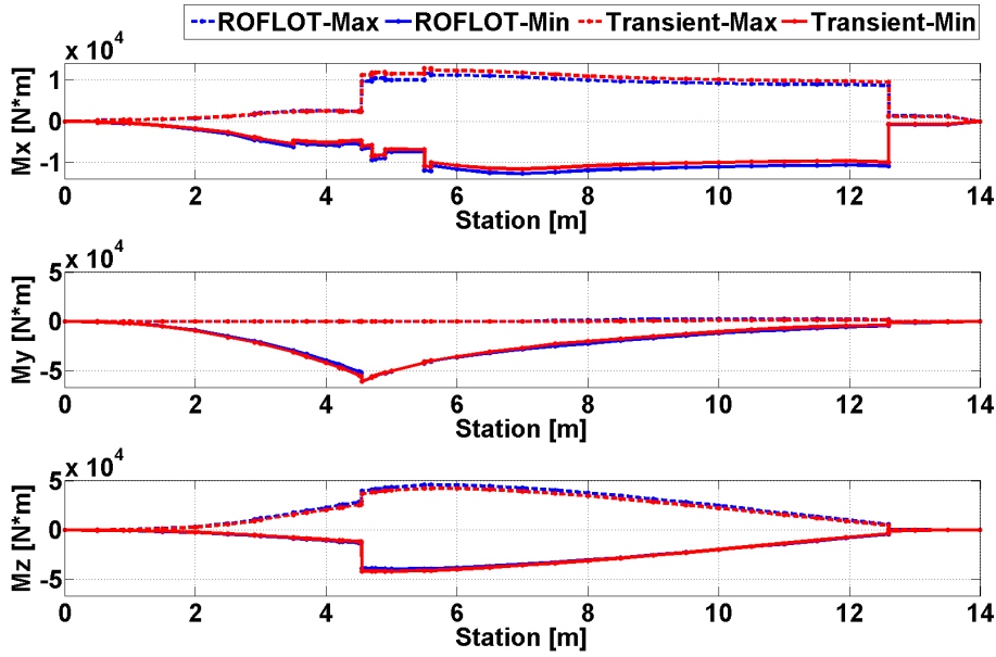
Figure 69. Comparison of Trim and Transient Solution Overall Maximum and Minimum Torsional and Bending Moments of the Yaw Maneuvers
