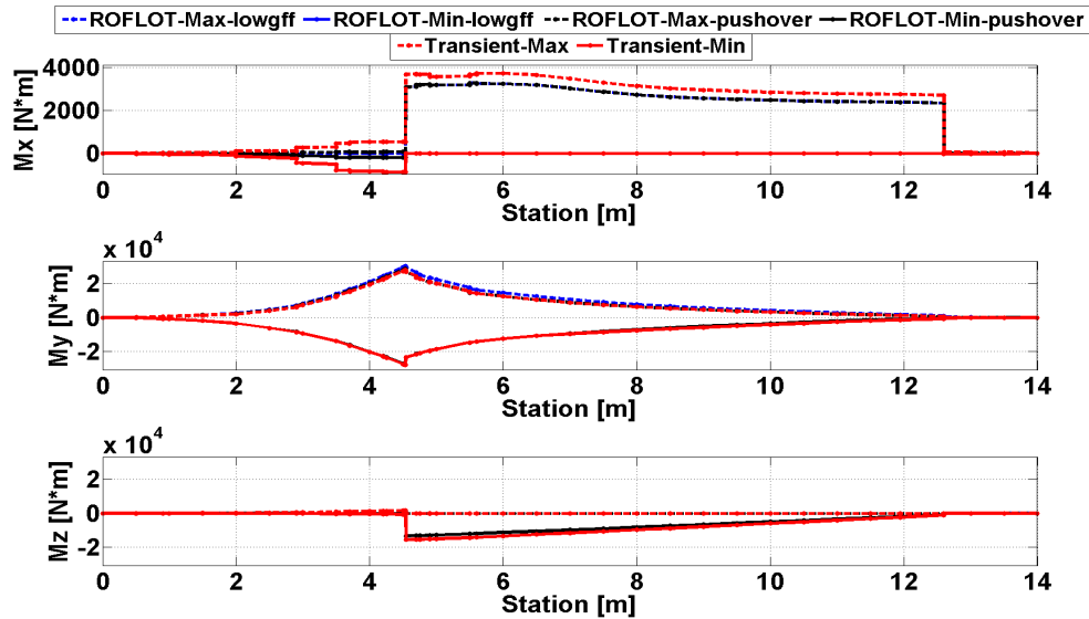
Figure 57. Comparison of Trim and Transient Solution Torsional and Bending Moments for Sea Level, ISA -55 C^0 , 80 [knot], -1 [g] Push-over Maneuver
