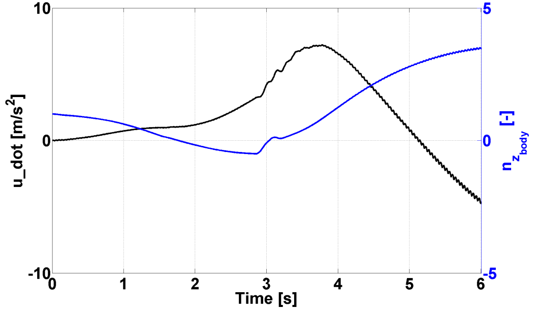
Figure 41. Time History of the Time Derivative of the Velocity in x_{\text{body}} Direction for the Pull-up Maneuver Transient Analysis in 80 [knot]
