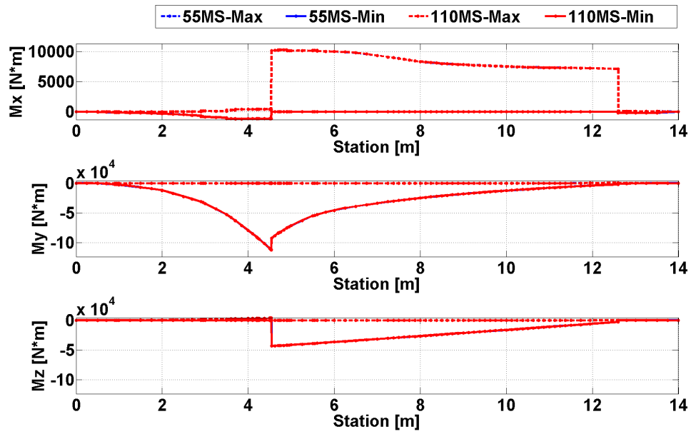
Figure 113. Comparison of Torsional and Bending Moments for Two Different Number of Monitor Stations for Sea Level, ISA -55 C 0 , 120 [knot], 3.5 [g] Pull-up Maneuver
