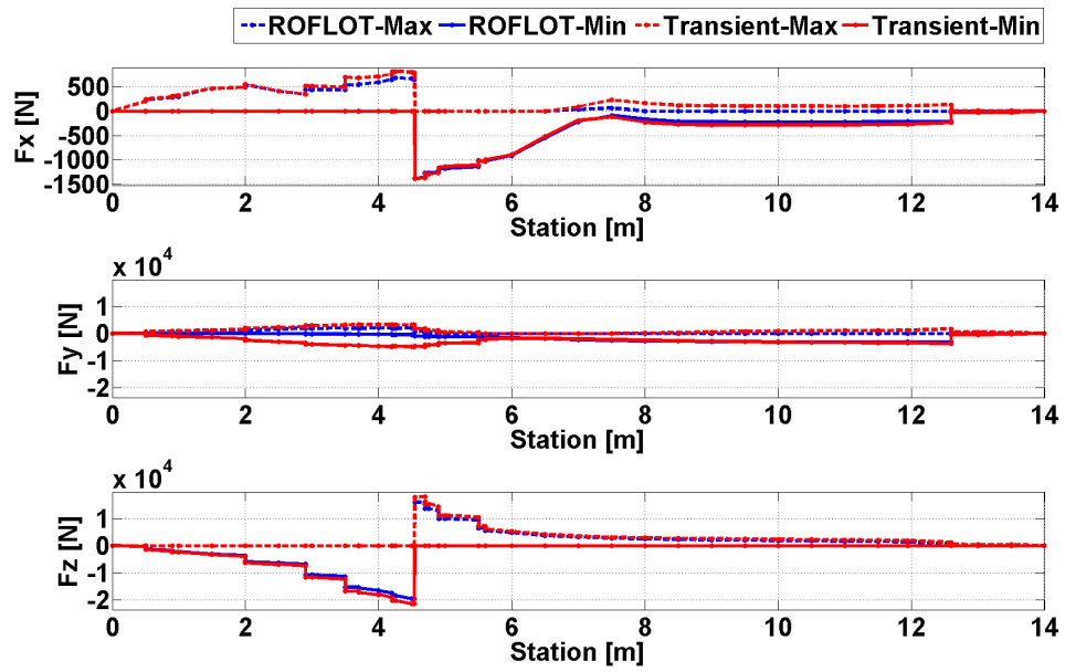
Figure 102. Comparison of Trim and Transient Solution Axial and Shear Forces for Sea Level, 80 [knot] Forward Flight, Gust From Right Condition
