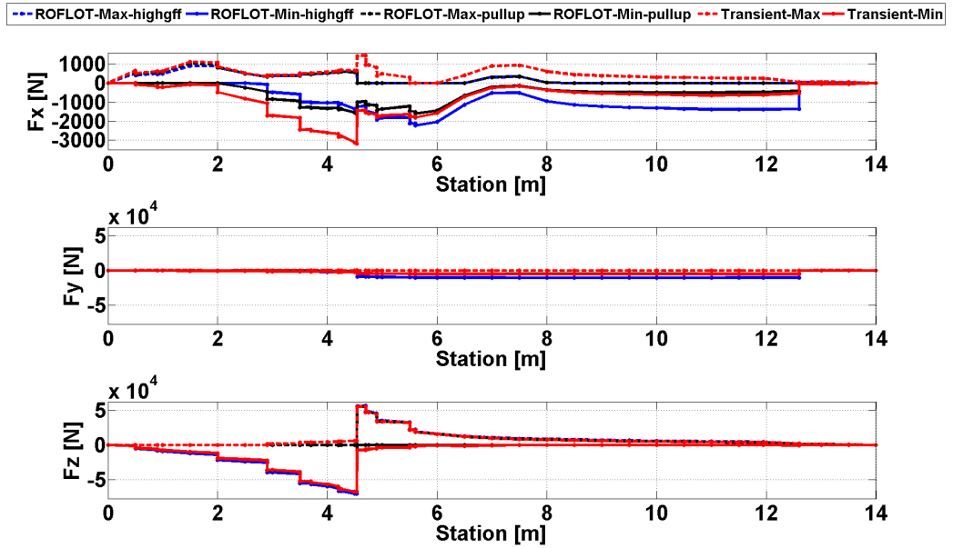
Figure 54. Comparison of Trim and Transient Solution Overall Maximum and Minimum Axial and Shear Forces of the Pull-up Maneuvers
