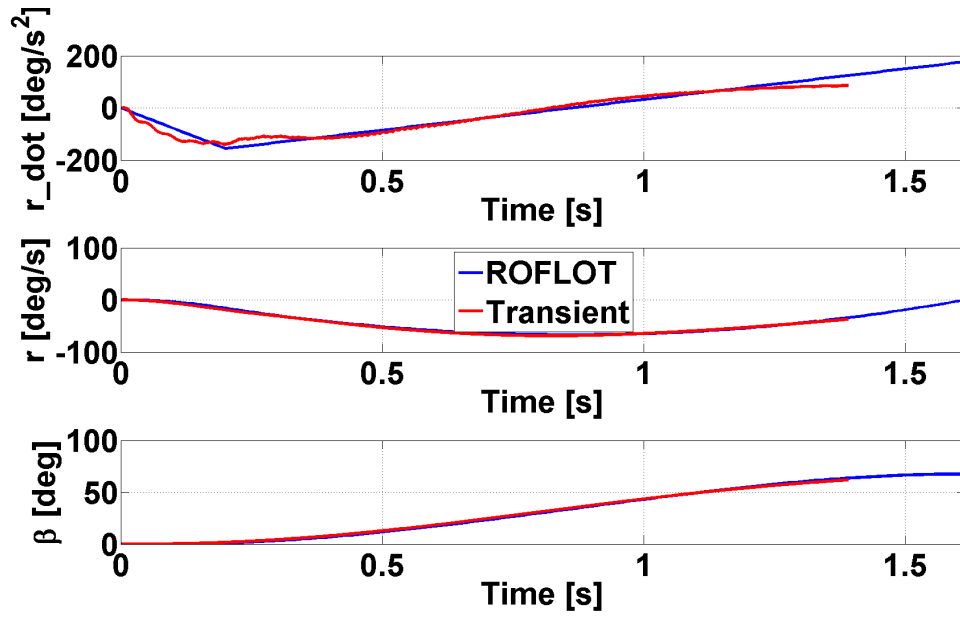
Figure 47. Comparison of the Yaw Acceleration, Yaw Velocity and Sideslip Angle Estimated and Obtained from the Transient Analysis of Yaw to Port Maneuver in 120 [knot]
