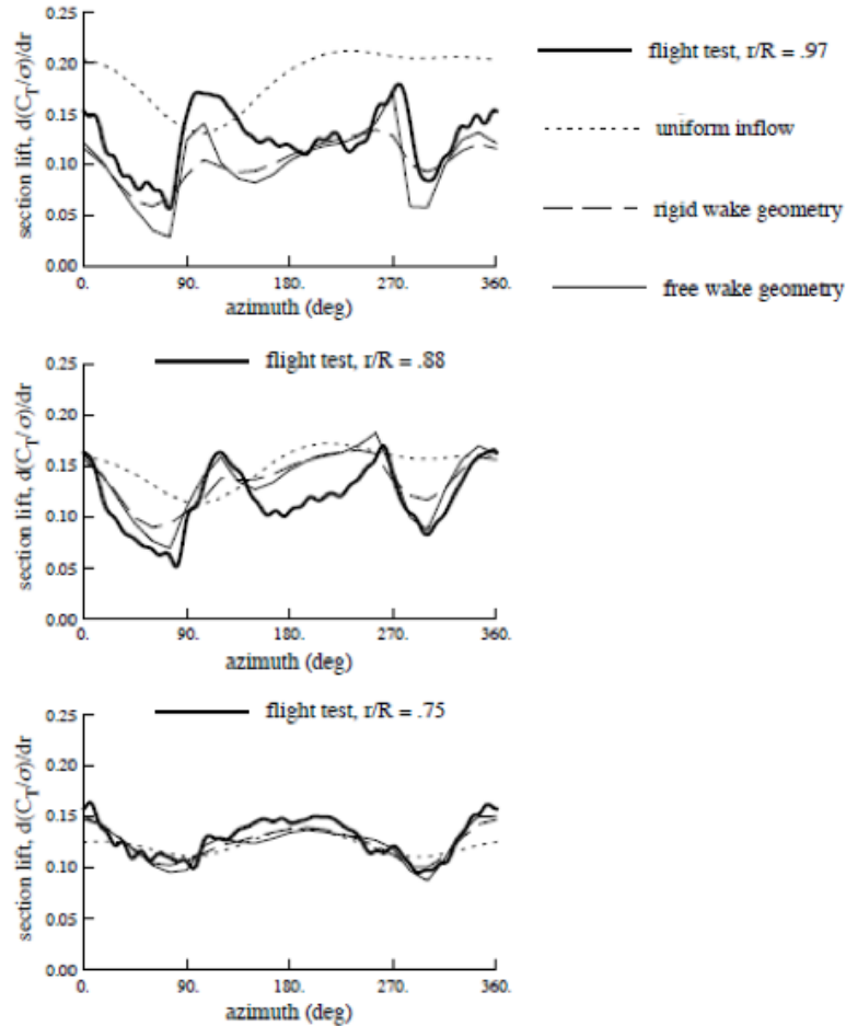
Figure 15. CAMRAD II Section Lift Correlation with SA349/2 Helicopter Flight Test Data at CT/\sigma = 0.065 and \mu = 0.14 [23]
