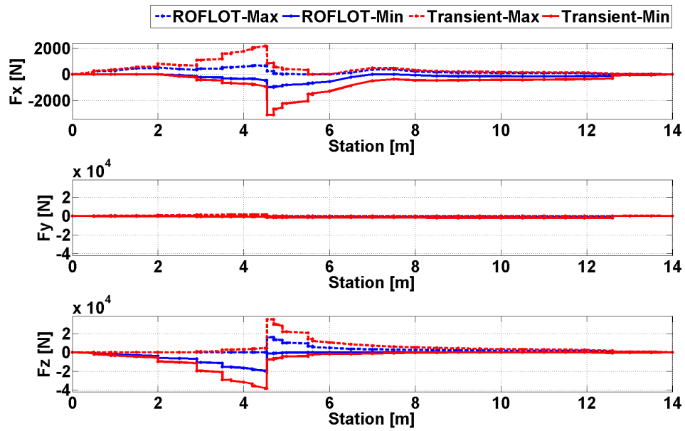
Figure 84. Comparison of Trim and Transient Solution Axial and Shear Forces for Sea Level, 80 [knot] Forward Flight, Gust From Up Condition
