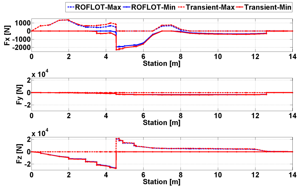
Figure 80. Comparison of Trim and Transient Solution Axial and Shear Forces for Sea Level, 160 [knot] Forward Flight, Gust From Rear Condition
