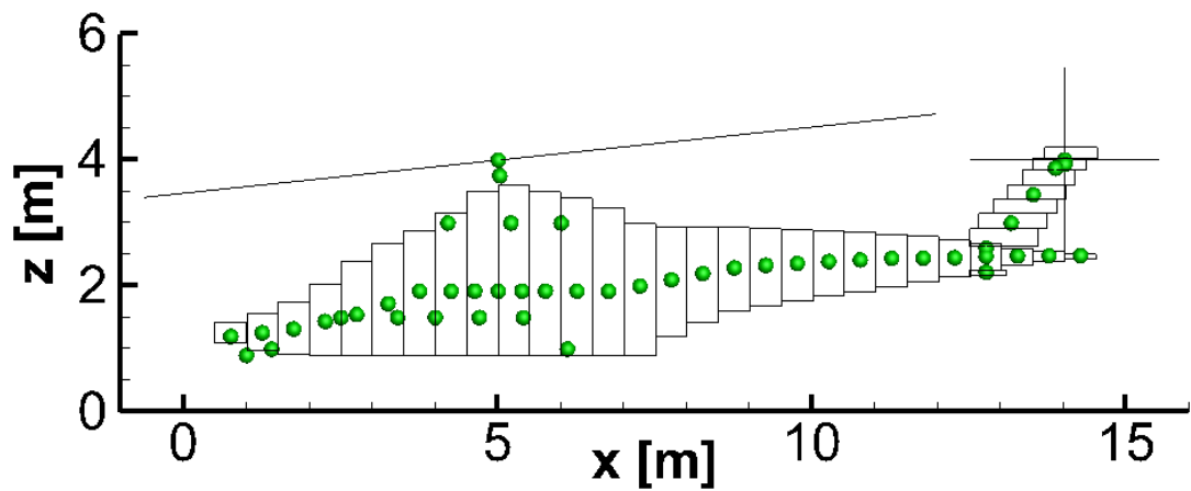
Figure 29. Schematic Representation of Mass State M01, Side View
