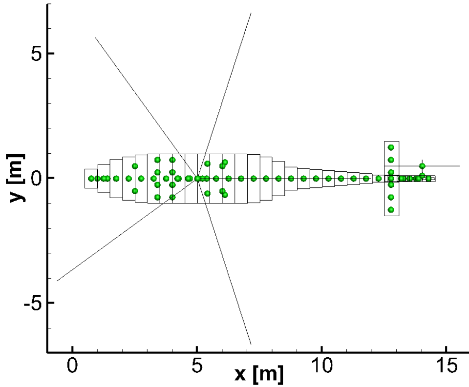
Figure 30. Schematic Representation of Mass State M01, Top View
