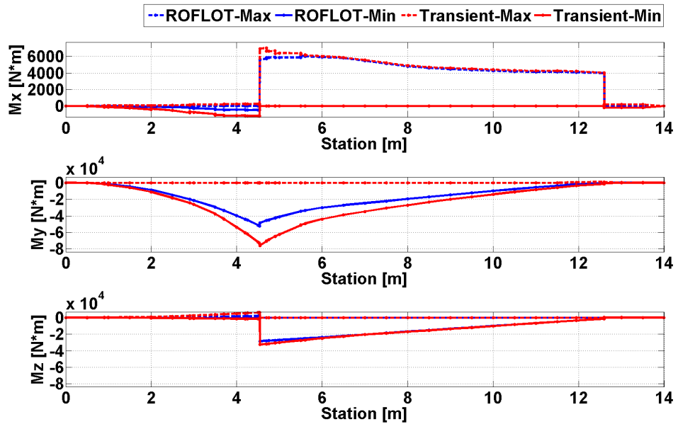
Figure 87. Comparison of Trim and Transient Solution Torsional and Bending Moments for Sea Level, 160 [knot] Forward Flight, Gust From Up Condition
