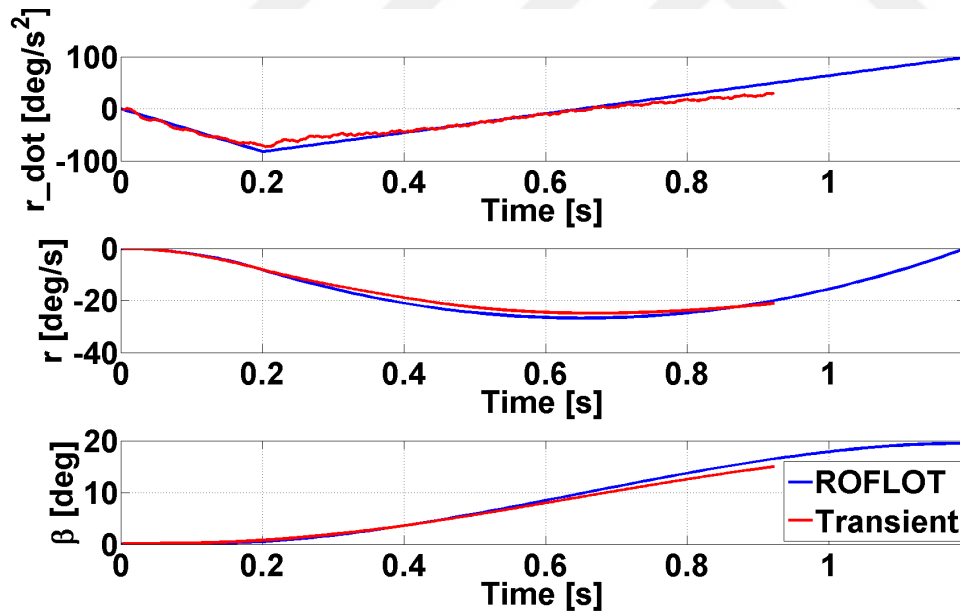
Figure 48. Comparison of the Yaw Acceleration, Yaw Velocity and Sideslip Angle Estimated and Obtained from the Transient Analysis of Yaw to Port Maneuver in 160 [knot]
