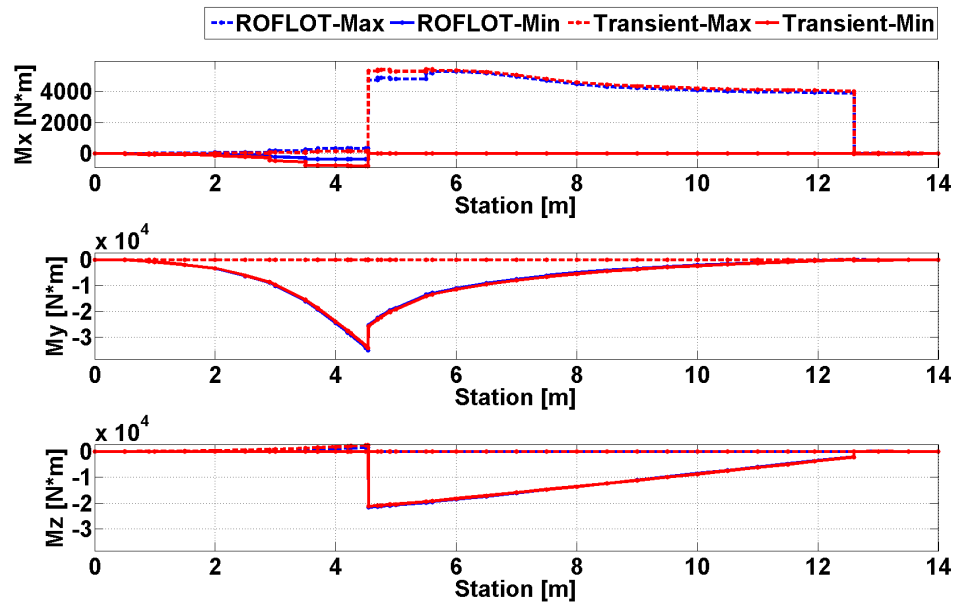
Figure 71. Comparison of Trim and Transient Solution Torsional and Bending Moments for Sea Level, Hover, Gust From Forward Condition
