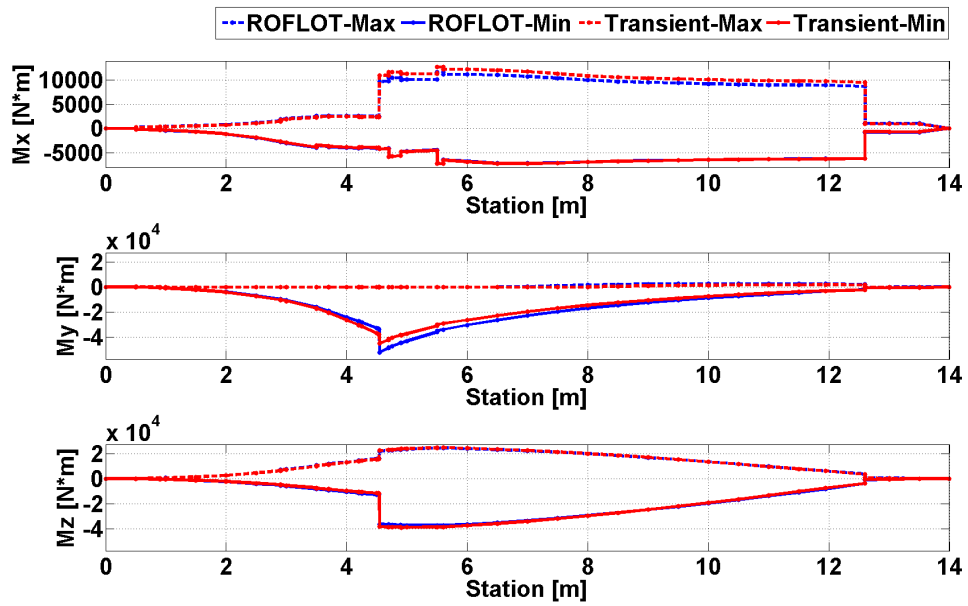
Figure 63. Comparison of Trim and Transient Solution Torsional and Bending Moments for Sea Level, 80 [knot], Yaw to Port Maneuver
