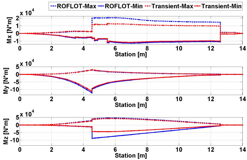
Figure 111. Comparison of Trim and Transient Solution Overall Maximum and Minimum Torsional and Bending Moments of All the Maneuvers and Gust Conditions when High-g and Low-g Forward Flight Trim Methods are Employed
