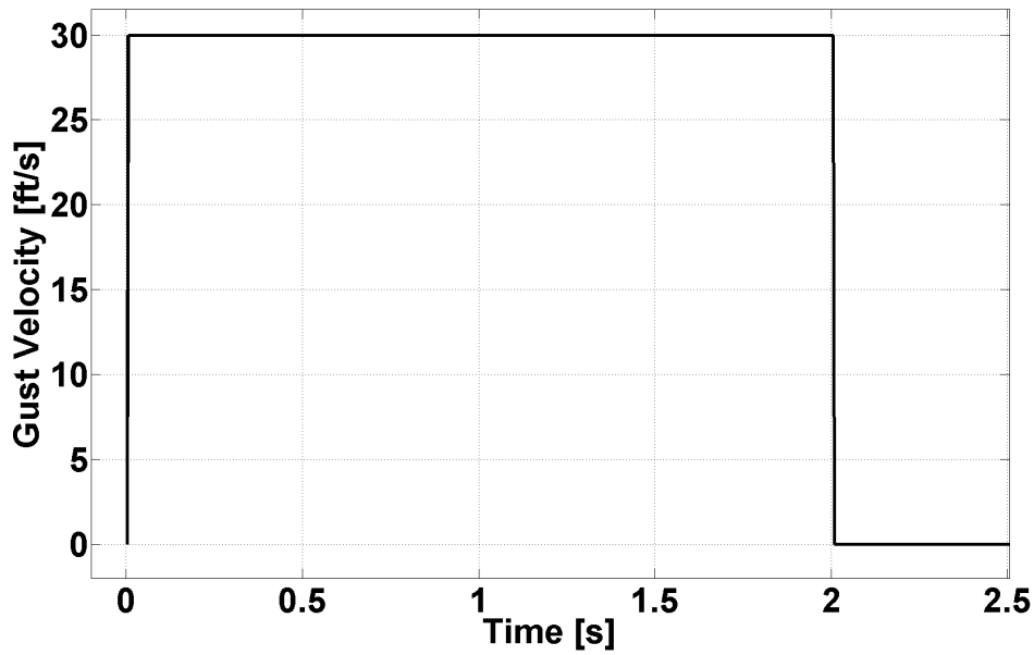
Figure 49. Gust Profile Used for the Transient Analysis of the Gust Conditions in Hover
