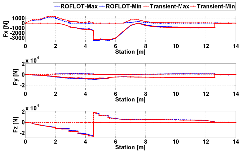
Figure 66. Comparison of Trim and Transient Solution Axial and Shear Forces for Sea Level, 160 [knot], Yaw to Port Maneuver
