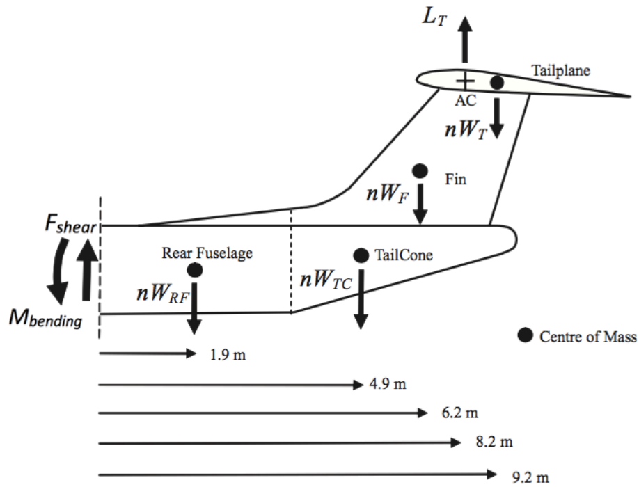
Figure 7. Cut on the Rear Fuselage and Distributed Inertial Loads together with a Discrete Aerodynamic Load in Maneuvering [6]
