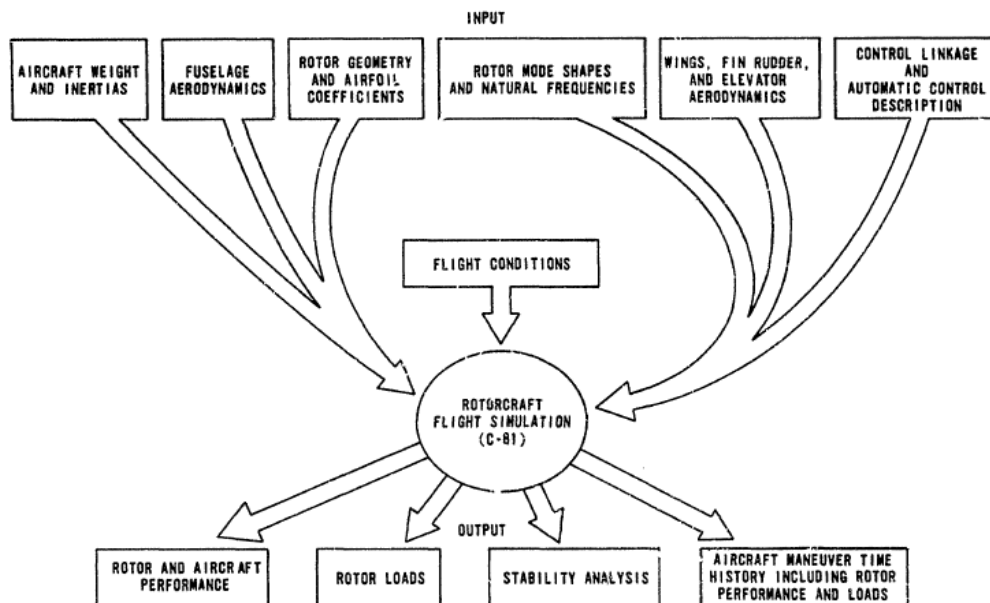
Figure 10. Inputs and Outputs of C81 [14]
