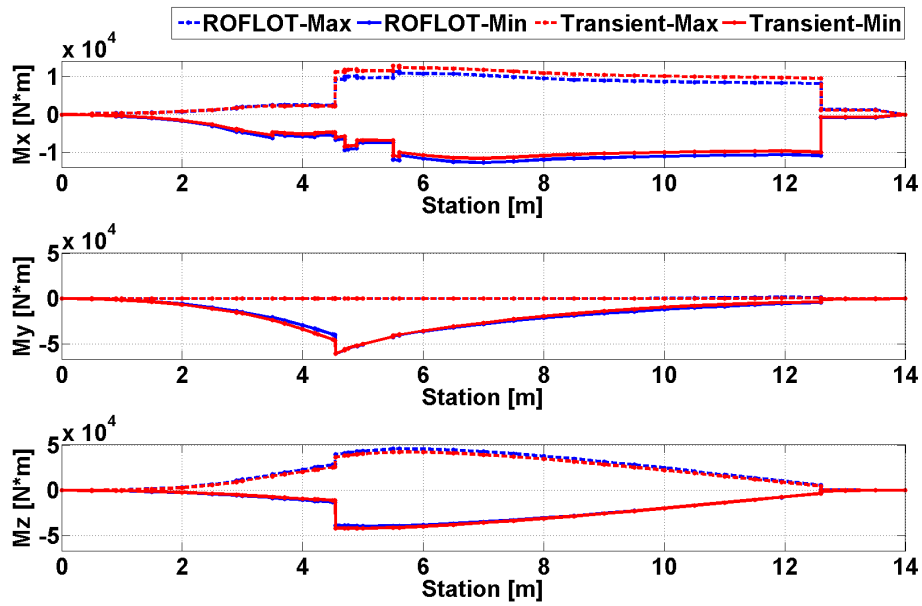
Figure 65. Comparison of Trim and Transient Solution Torsional and Bending Moments for Sea Level, 120 [knot], Yaw to Port Maneuver
