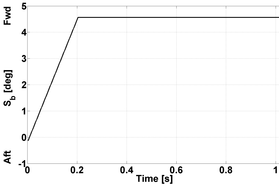
Figure 42. Time History of the Longitudinal Cyclic Position for the Transient Analysis of Push-over Maneuver in 120 [knot]
