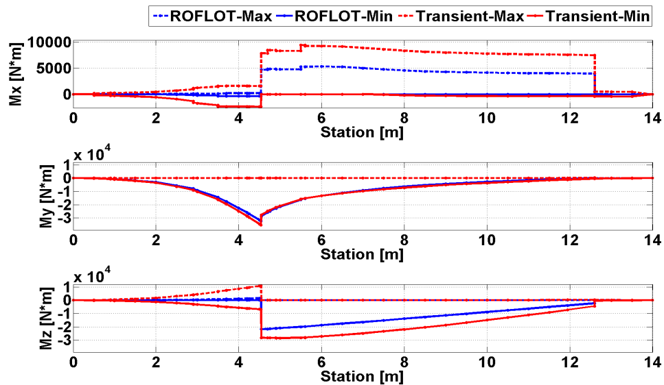
Figure 101. Comparison of Trim and Transient Solution Torsional and Bending Moments for Sea Level, Hover, Gust From Right Condition
