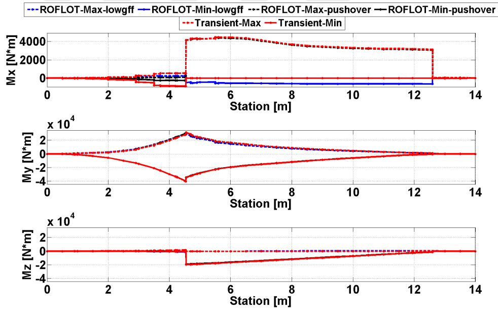
Figure 61. Comparison of Trim and Transient Solution Overall Maximum and Minimum Torsional and Bending Moments of the Push-over Maneuvers
