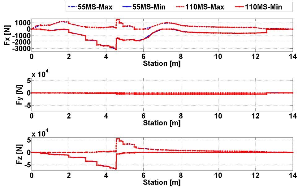
Figure 112. Comparison of Axial and Shear Forces for Two Different Number of Monitor Stations for Sea Level, ISA -55 C 0 , 120 [knot], 3.5 [g] Pull-up Maneuver
