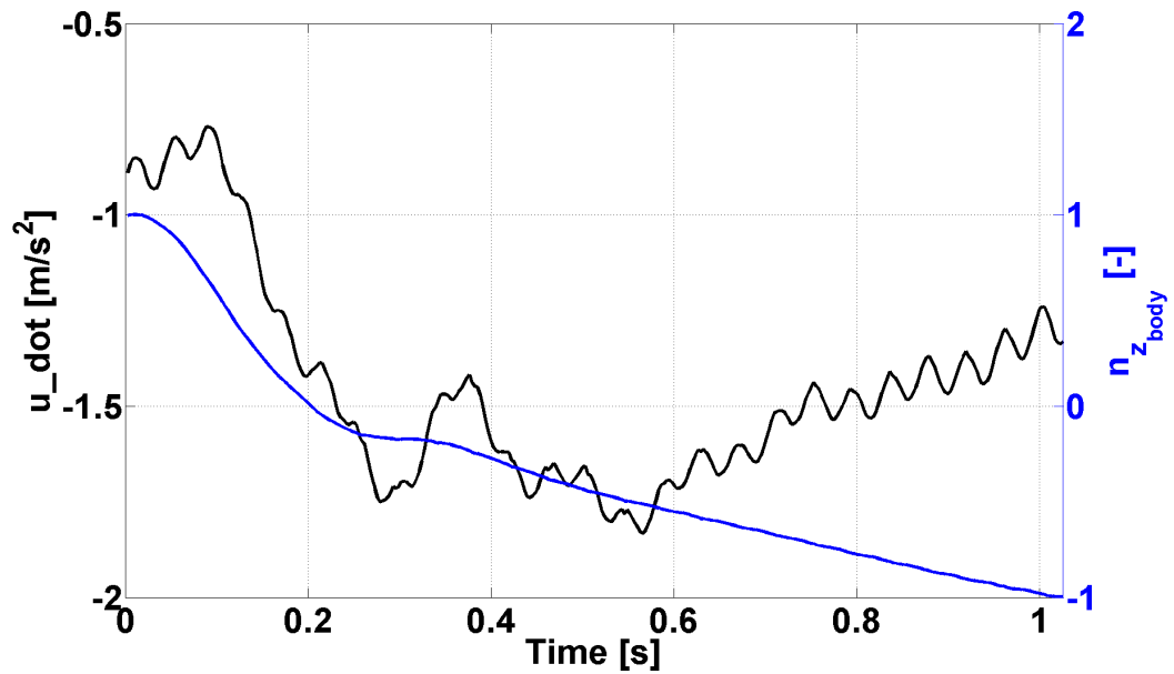
Figure 43. Time History of the Time Derivative of the Velocity in x_{\text{body}} Direction for the Push-over Maneuver Transient Analysis in 120 [knot]
