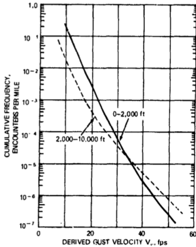
Figure 4. Gust Velocity Probability Curve [4]
