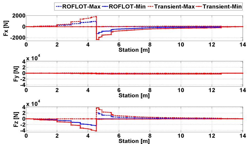
Figure 88. Comparison of Trim and Transient Solution Axial and Shear Forces for Sea Level, Hover, Gust From Down Condition
