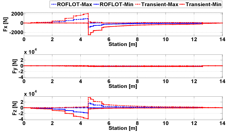
Figure 82. Comparison of Trim and Transient Solution Axial and Shear Forces for Sea Level, Hover, Gust From Up Condition
