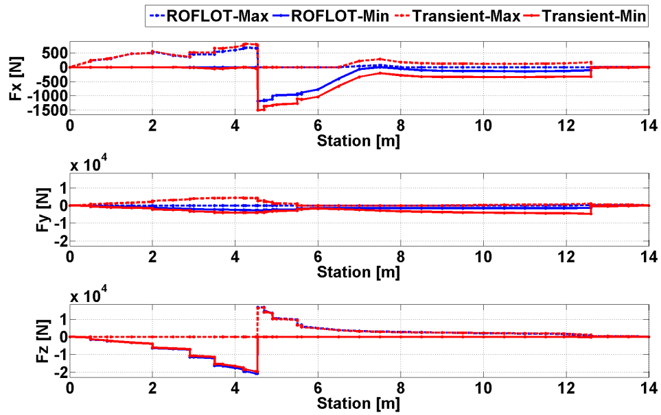
Figure 96. Comparison of Trim and Transient Solution Axial and Shear Forces for Sea Level, 80 [knot] Forward Flight, Gust From Left Condition
