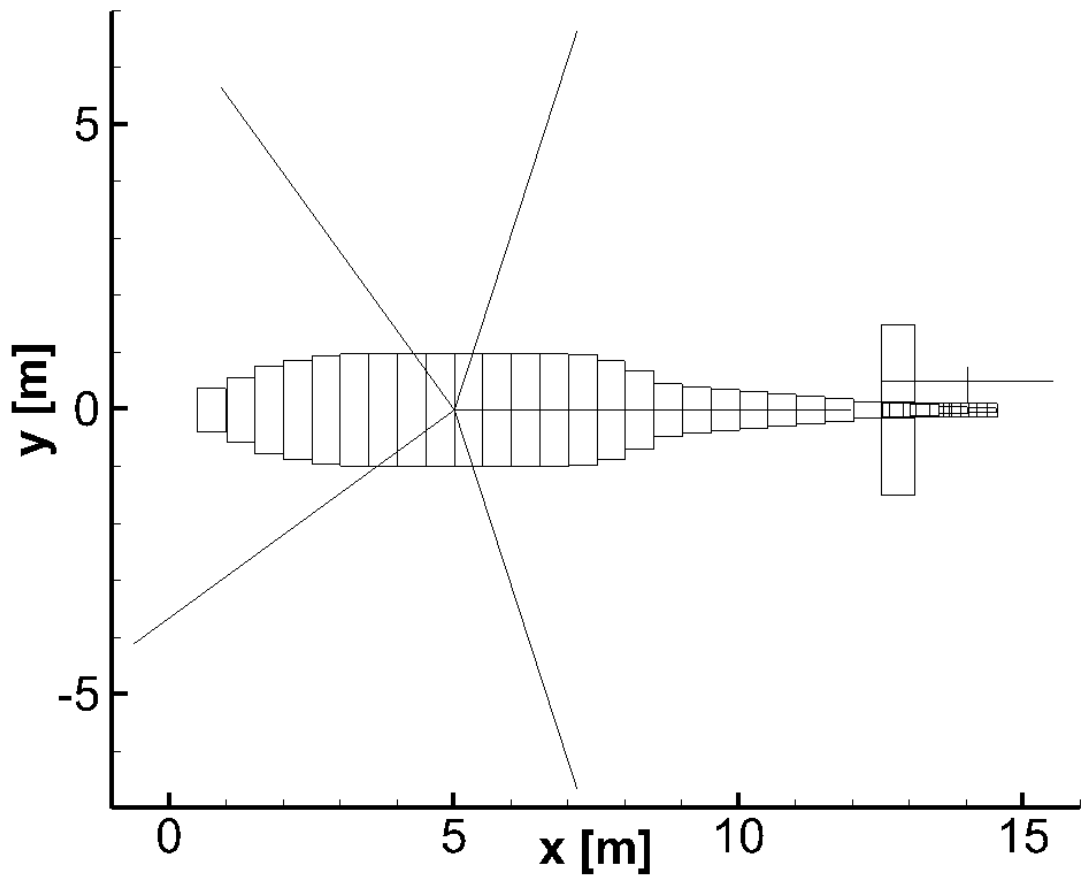
Figure 23. Schematic Representation of the Rotorcraft, Top View
