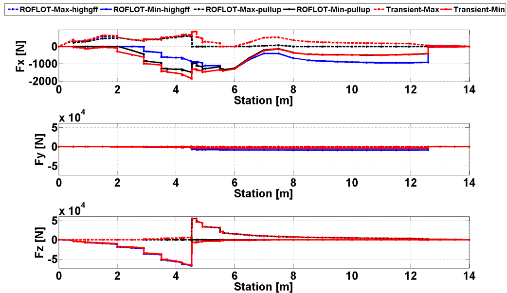
Figure 50. Comparison of Trim and Transient Solution Axial and Shear Forces for Sea Level, ISA -55 C°, 80 [knot], 3.5 [g] Pull-up Maneuver
