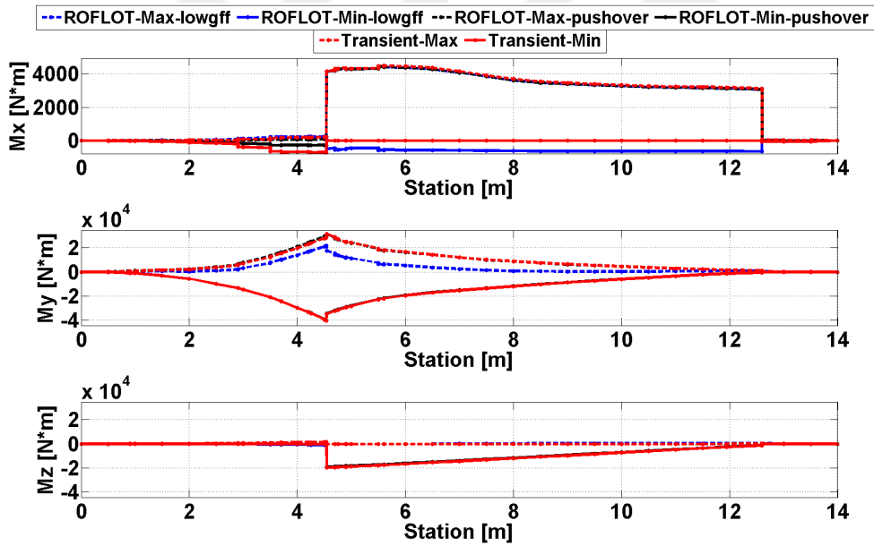
Figure 59. Comparison of Trim and Transient Solution Torsional and Bending Moments for Sea Level, ISA -55 C 0 , 120 [knot], -1 [g] Push-over Maneuver
