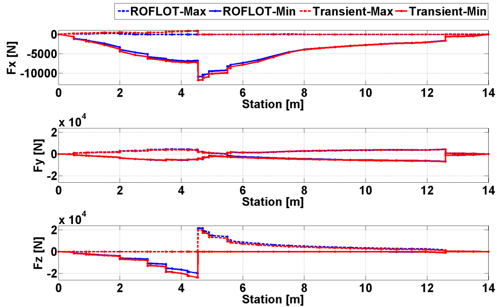
Figure 62. Comparison of Trim and Transient Solution Axial and Shear Forces for Sea Level, 80 [knot], Yaw to Port Maneuver
