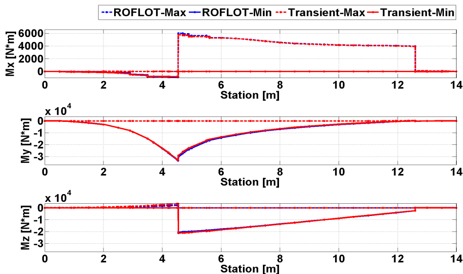
Figure 77. Comparison of Trim and Transient Solution Torsional and Bending Moments for Sea Level, Hover, Gust From Rear Condition
