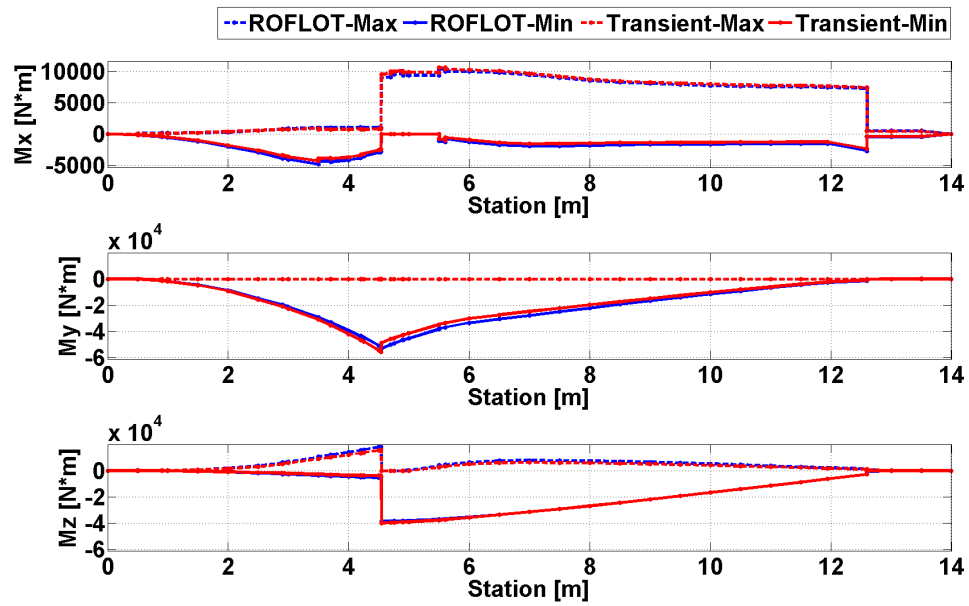
Figure 67. Comparison of Trim and Transient Solution Torsional and Bending Moments for Sea Level, 160 [knot], Yaw to Port Maneuver
