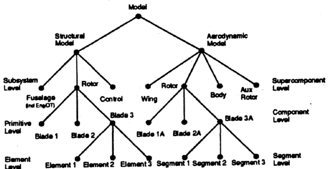
Figure 11. 2GCHAS Hierarchical System Model [15]
