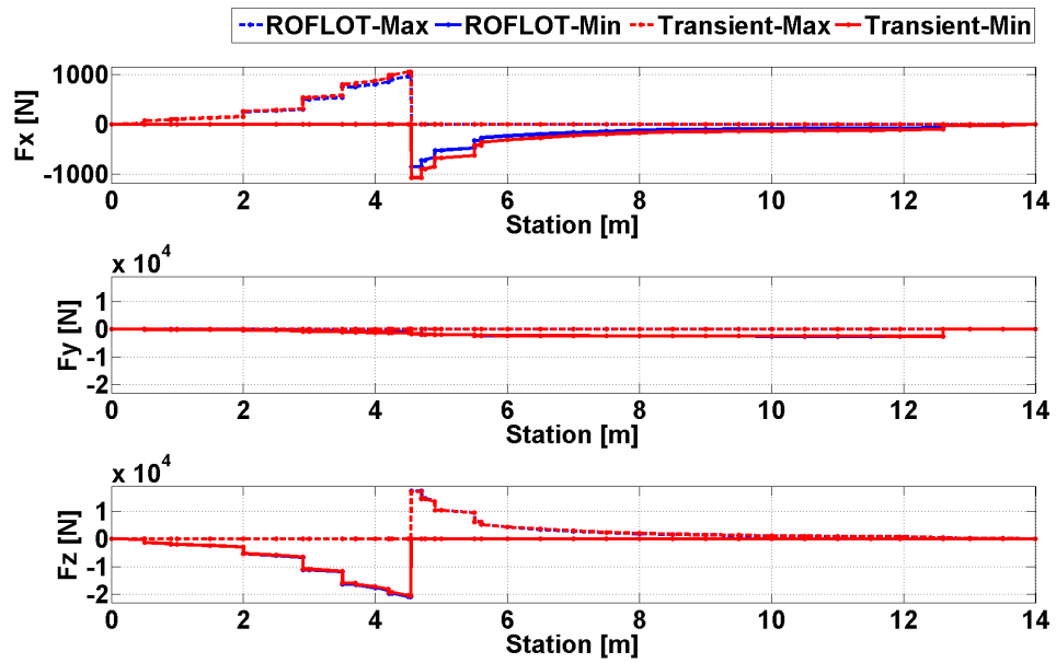
Figure 70. Comparison of Trim and Transient Solution Axial and Shear Forces for Sea Level, Hover, Gust From Forward Condition
