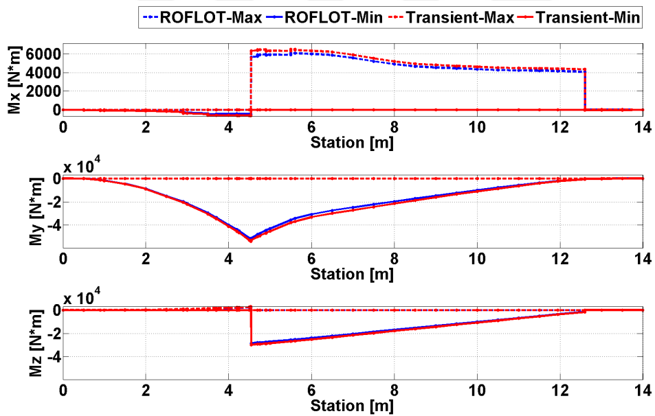
Figure 81. Comparison of Trim and Transient Solution Torsional and Bending Moments for Sea Level, 160 [knot] Forward Flight, Gust From Rear Condition
