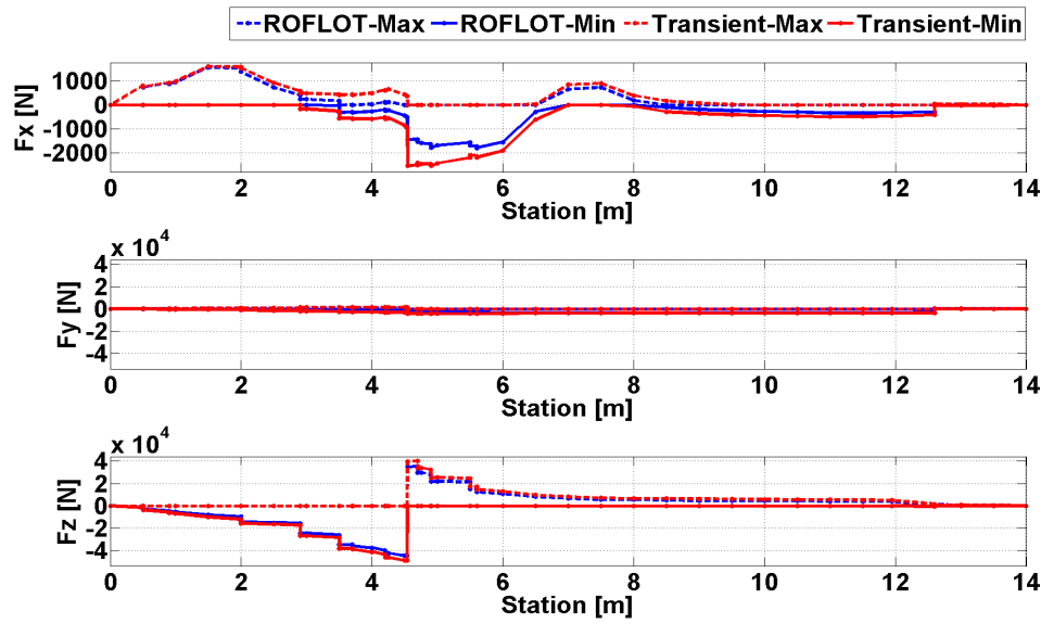
Figure 92. Comparison of Trim and Transient Solution Axial and Shear Forces for Sea Level, 160 [knot] Forward Flight, Gust From Down Condition
