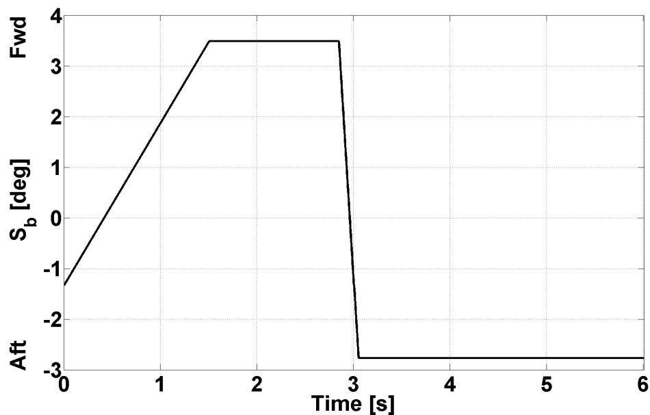
Figure 40. Time History of the Longitudinal Cyclic Position for the Transient Analysis of Pull-up Maneuver in 80 [knot]
