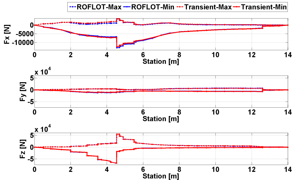
Figure 108. Comparison of Trim and Transient Solution Overall Maximum and Minimum Axial and Shear Forces of All the Maneuvers and Gust Conditions when Pull-up and Push-over Trim Methods are Employed
