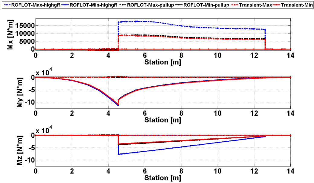
Figure 51. Comparison of Trim and Transient Solution Torsional and Bending Moments for Sea Level, ISA -55 C 0 , 80 [knot], 3.5 [g] Pull-up Maneuver
