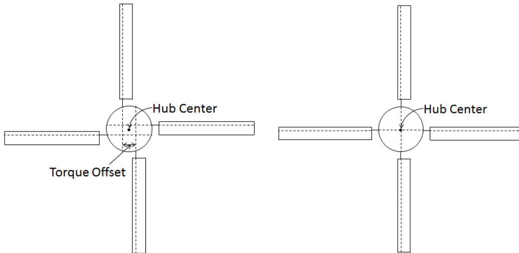
Figure 19. Hub Center Location with and without Torque Offset
