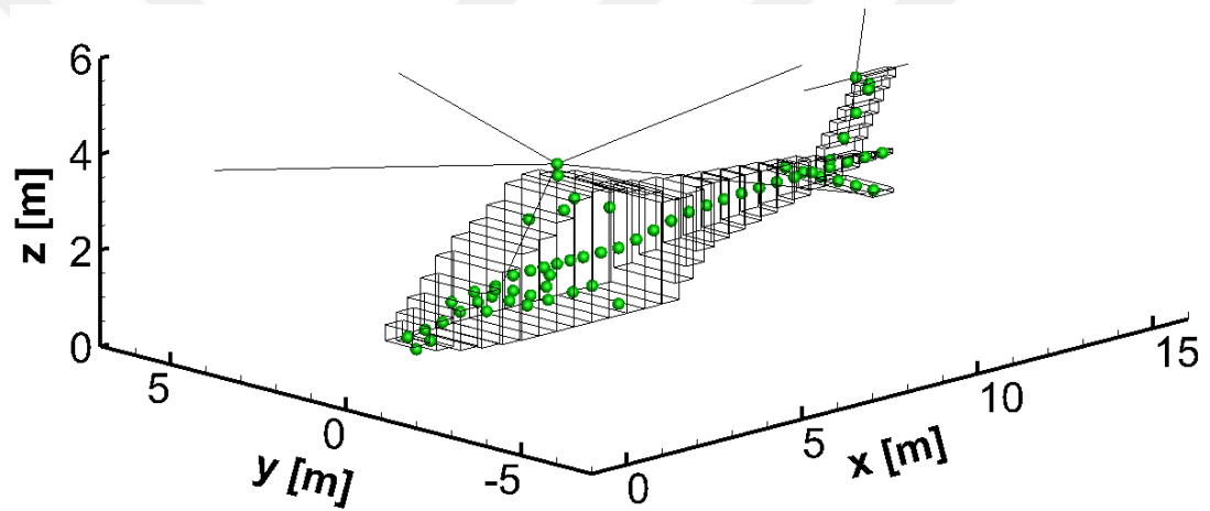
Figure 28. Schematic Representation of Mass State M01, Isometric View
