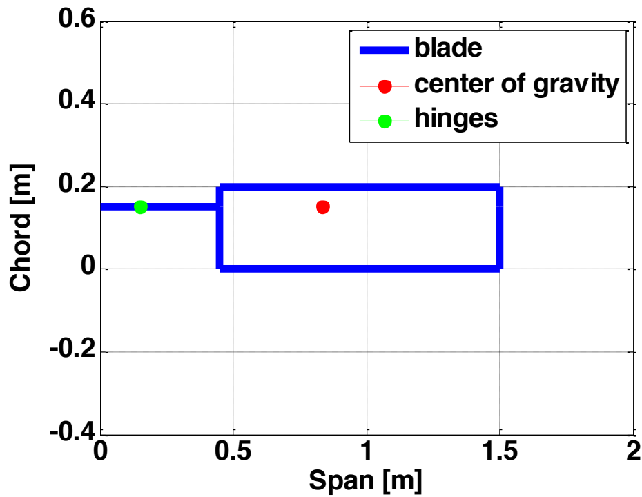
Figure 27. Schematic Representation of Tail Rotor Blade Geometry
