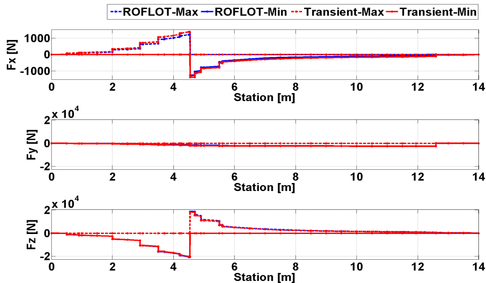
Figure 76. Comparison of Trim and Transient Solution Axial and Shear Forces for Sea Level, Hover, Gust From Rear Condition
