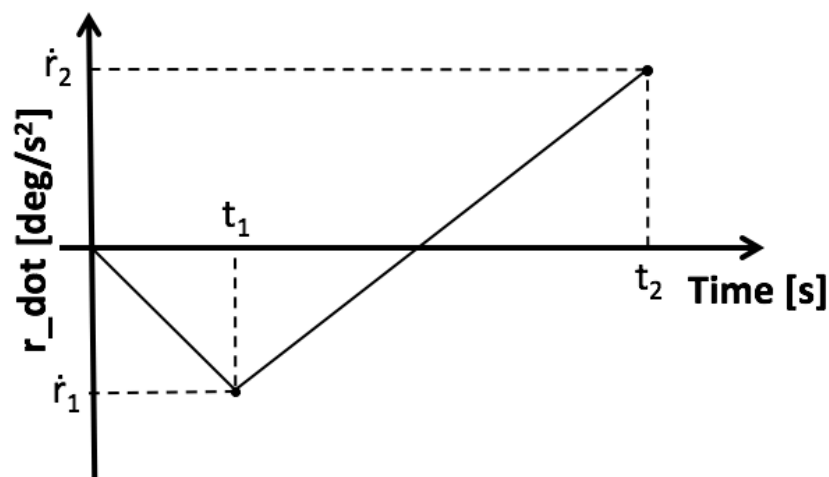
Figure 45. Assumed Yaw Acceleration
