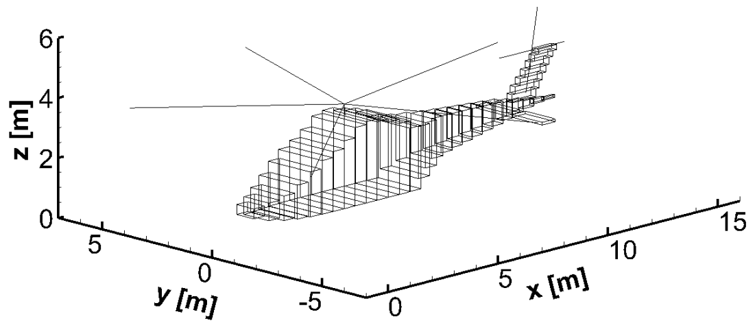
Figure 22. Schematic Representation of the Rotorcraft, Isometric View
