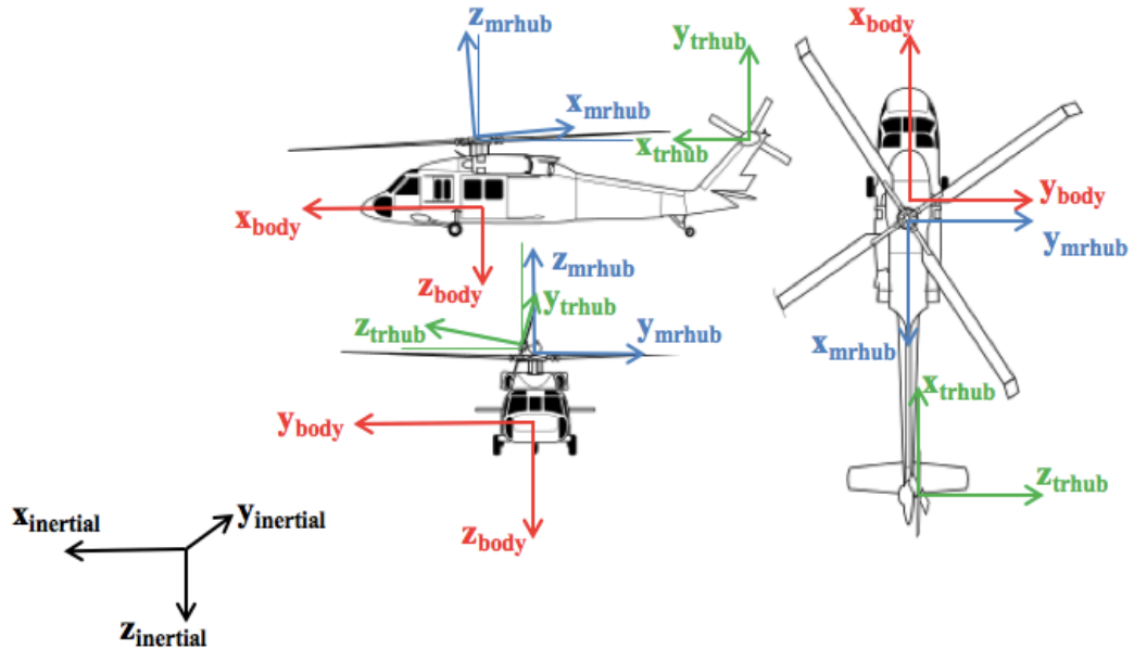
Figure 18. Body Axis System, Inertial Axis System, and Main Rotor and Tail Rotor Hub Axis Systems
