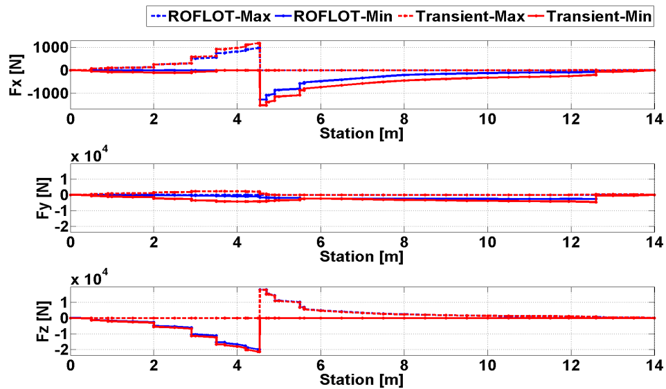
Figure 100. Comparison of Trim and Transient Solution Axial and Shear Forces for Sea Level, Hover, Gust From Right Condition
