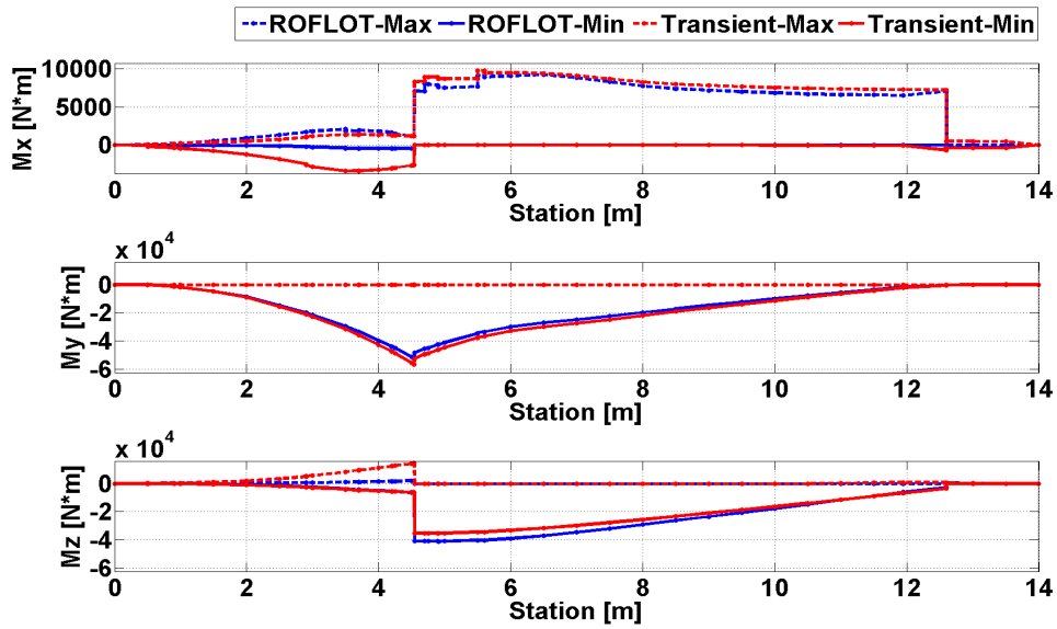
Figure 105. Comparison of Trim and Transient Solution Torsional and Bending Moments for Sea Level, 160 [knot] Forward Flight, Gust From Right Condition
