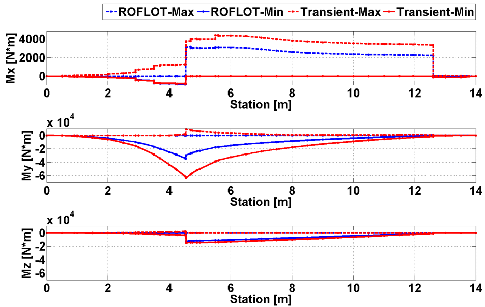
Figure 85. Comparison of Trim and Transient Solution Torsional and Bending Moments for Sea Level, 80 [knot] Forward Flight, Gust From Up Condition
