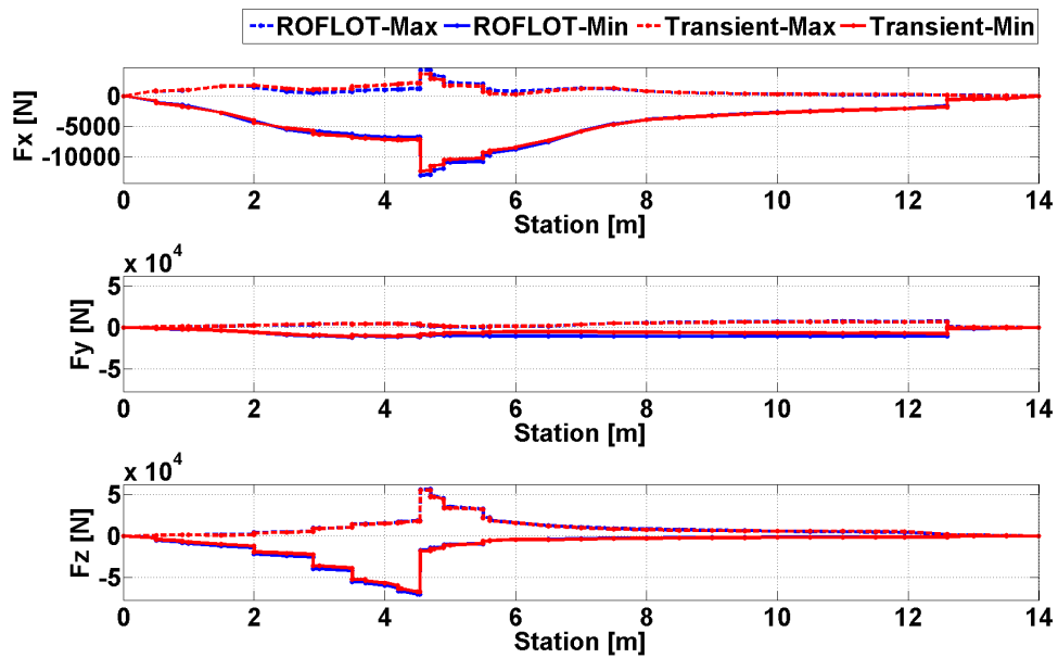
Figure 110. Comparison of Trim and Transient Solution Overall Maximum and Minimum Axial and Shear Forces of All the Maneuvers and Gust Conditions when High-g and Low-g Forward Flight Trim Methods are Employed
