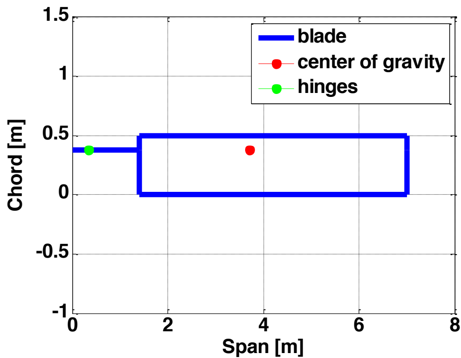
Figure 26. Schematic Representation of Main Rotor Blade Geometry
