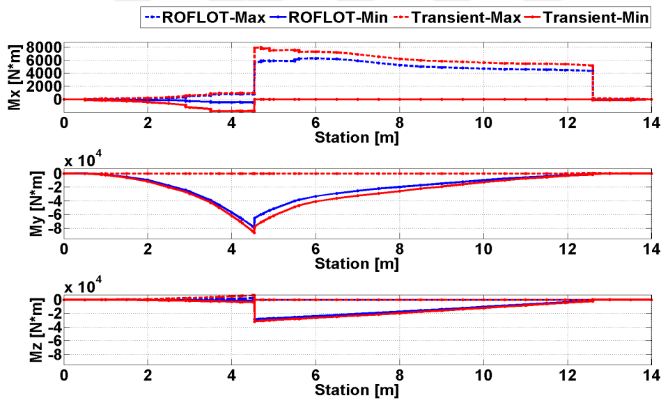
Figure 93. Comparison of Trim and Transient Solution Torsional and Bending Moments for Sea Level, 160 [knot] Forward Flight, Gust From Down Condition
