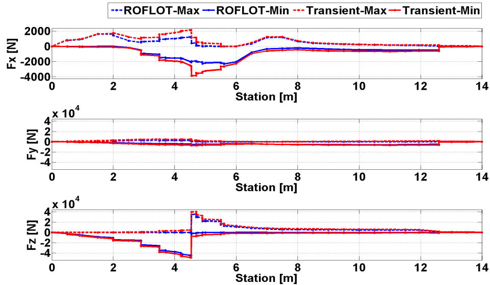
Figure 106. Comparison of Trim and Transient Solution Overall Maximum and Minimum Axial and Shear Forces of the Gust Conditions
