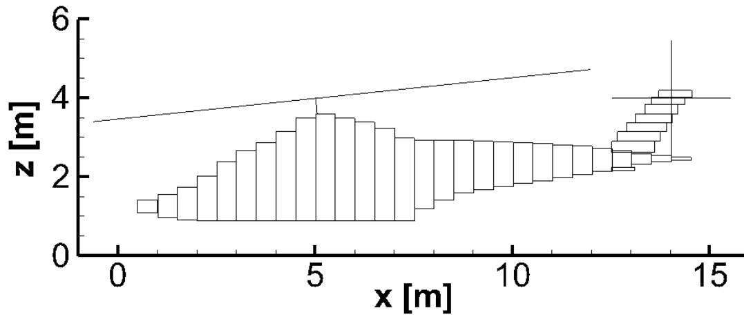
Figure 24. Schematic Representation of the Rotorcraft, Side View
