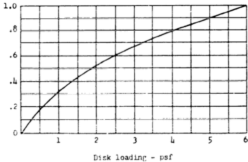
Figure 3. Change of Gust Alleviation Factor with Disk Loading [3]
