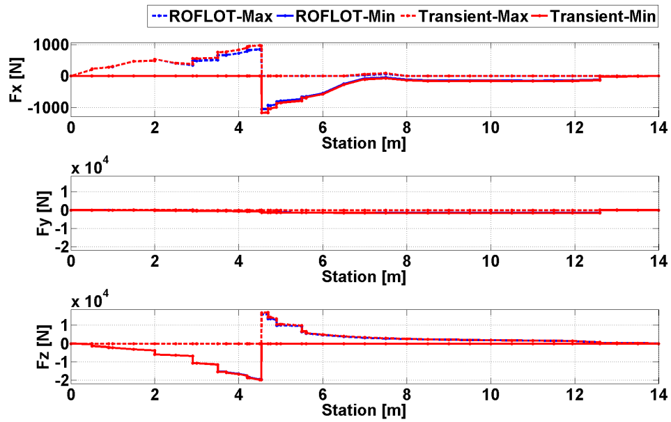
Figure 78. Comparison of Trim and Transient Solution Axial and Shear Forces for Sea Level, 80 [knot] Forward Flight, Gust From Rear Condition
