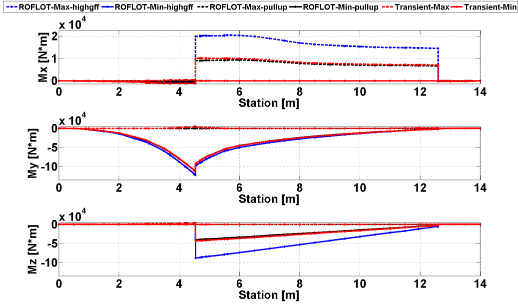
Figure 55. Comparison of Trim and Transient Solution Overall Maximum and Minimum Torsional and Bending Moments of the Pull-up Maneuvers
