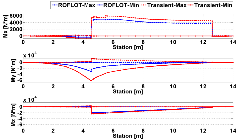
Figure 83. Comparison of Trim and Transient Solution Torsional and Bending Moments for Sea Level, Hover, Gust From Up Condition
