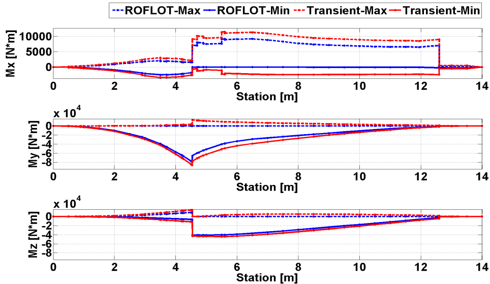
Figure 107. Comparison of Trim and Transient Solution Overall Maximum and Minimum Torsional and Bending Moments of the Gust Conditions
