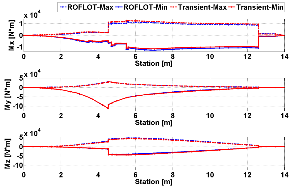
Figure 109. Comparison of Trim and Transient Solution Overall Maximum and Minimum Torsional and Bending Moments of All the Maneuvers and Gust Conditions when Pull-up and Push-over Trim Methods are Employed
