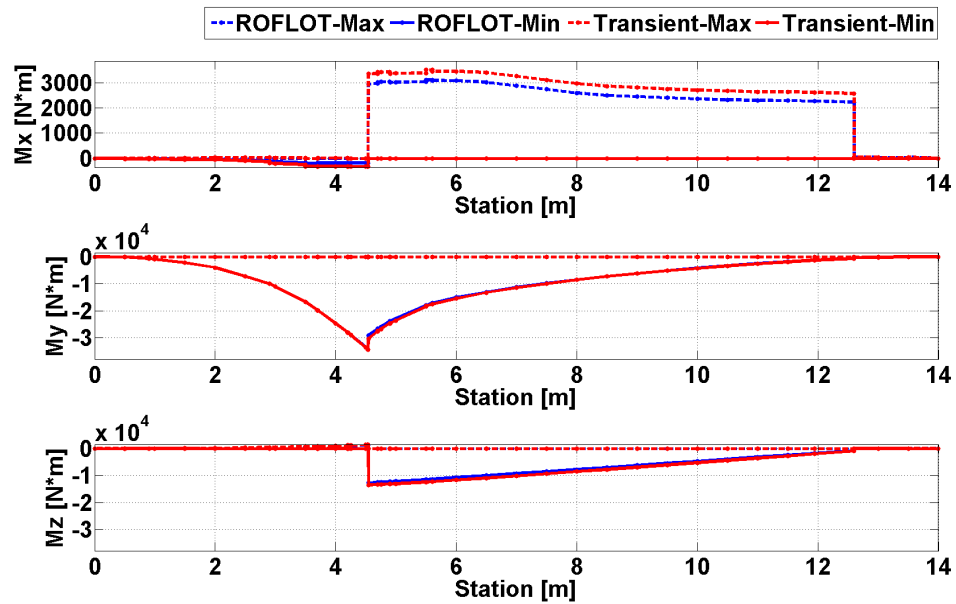
Figure 79. Comparison of Trim and Transient Solution Torsional and Bending Moments for Sea Level, 80 [knot] Forward Flight, Gust From Rear Condition
