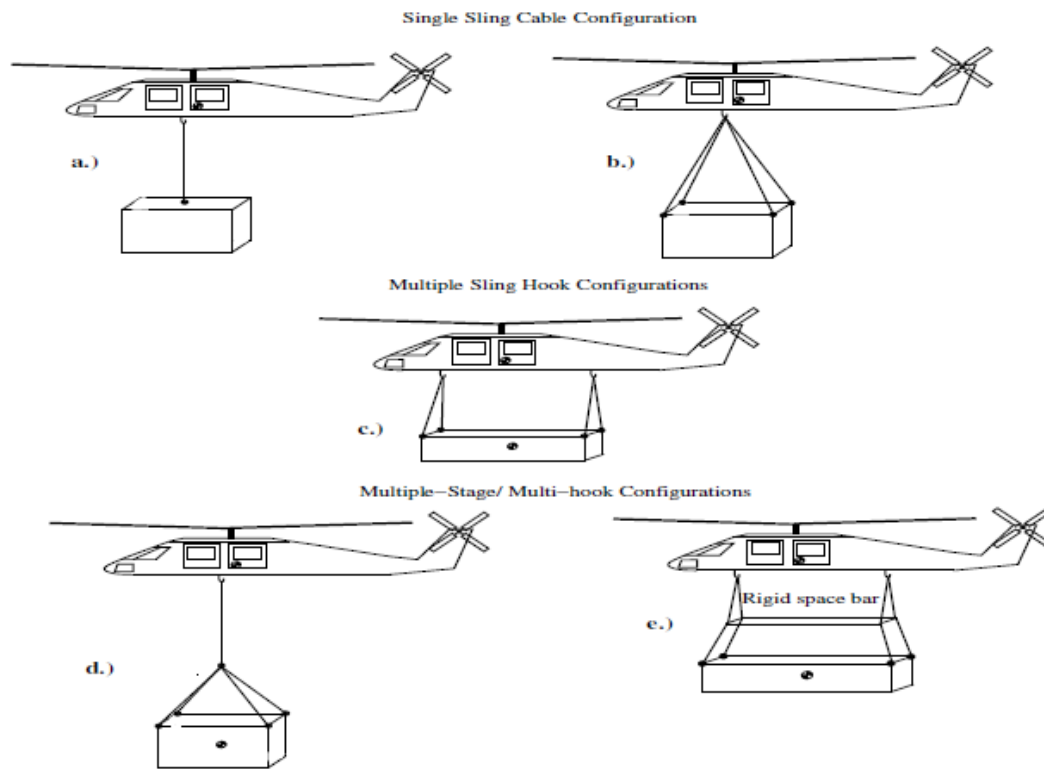
Figure 17. Various Sling Configurations Supported by FLIGHTLAB [28]
