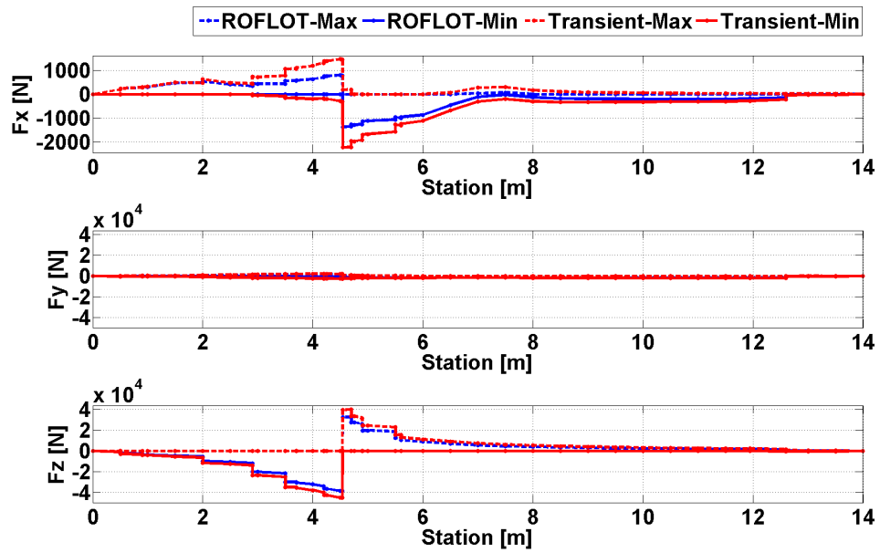
Figure 90. Comparison of Trim and Transient Solution Axial and Shear Forces for Sea Level, 80 [knot] Forward Flight, Gust From Down Condition
