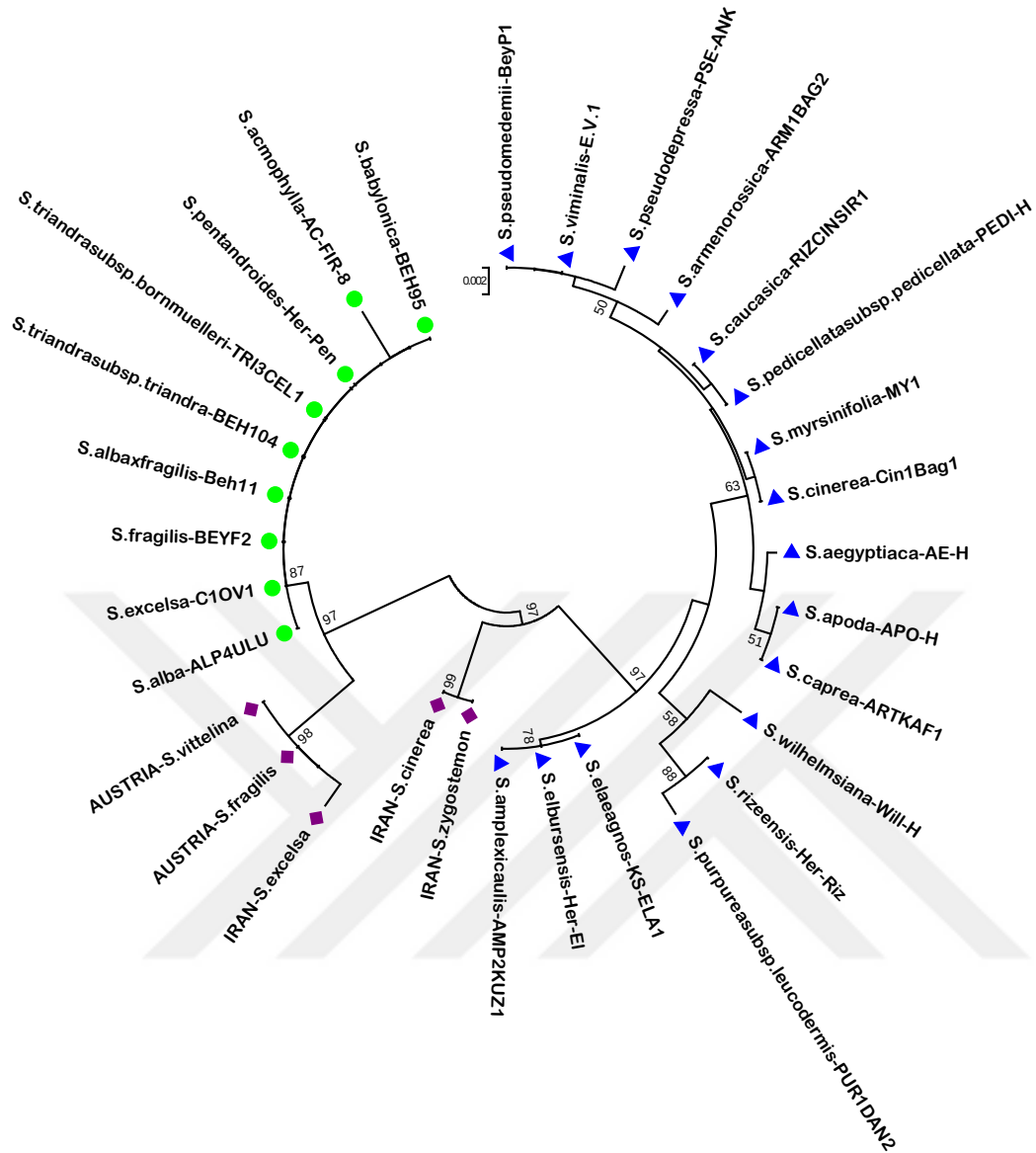
Figure 3.20. Phylogenetic tree ( trnL ) showing relations of Turkish Salix species with ones from the world (◆; OWS; Old World Salix , ▲; Subg. Vetrix , ●; Subg. Salix )
