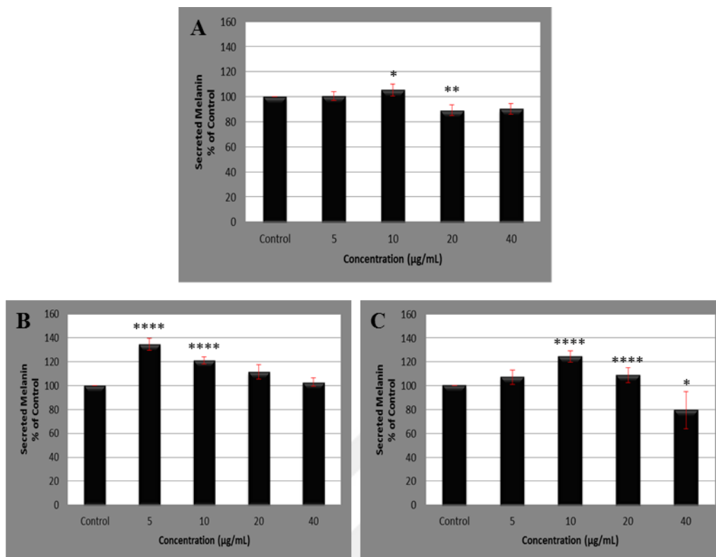
Figure 3.11: After 72 hours treatment, effect of A) crude extract and B) ethyl acetate fraction C) chloroform fraction on the secreted melanin amount for WM-115 melanoma cells. The absorbance of medium was measured at 405 nm with ELISA reader. Each percentage value in the treated cells was calculated with respect to that in the control cells. The results were expressed as \pm SD of two different experiments each carried out triplicate. *Significantly different from the control (* p \leq 0.05 , ** p \leq 0.01 , *** p \leq 0.001 , **** p \leq 0.0001 ).
