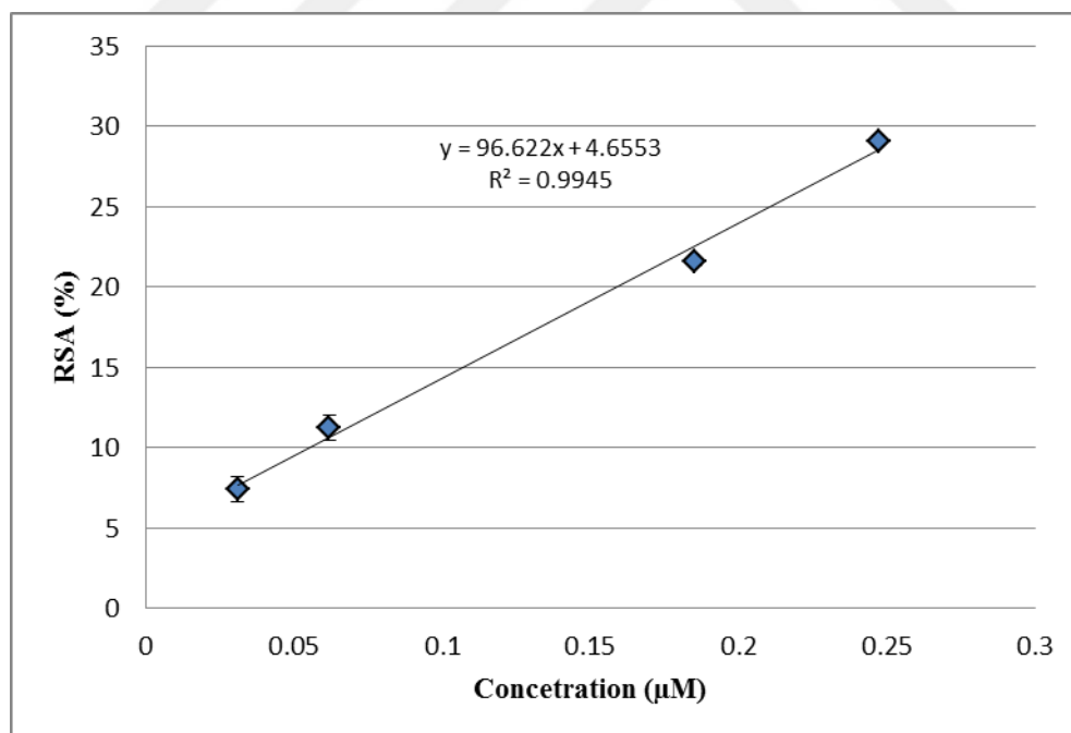
Figure 3.3: Radical scavenging activity in percent versus Trolox concentration.
