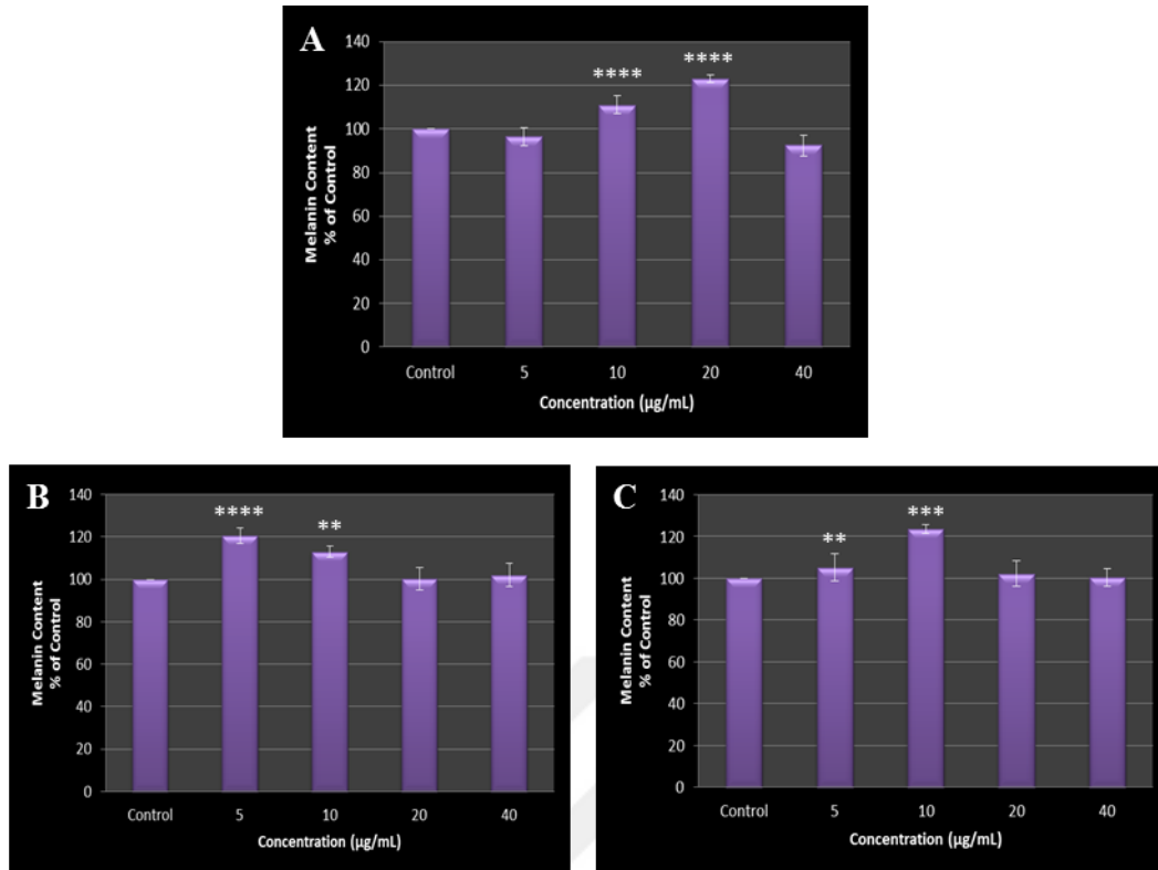
Figure 3.12: Effect of 72 hours treatment with A) crude extract and B) ethyl acetate fraction and C) chloroform fraction on the intracellular melanin content of the primary epidermal melanocytes. The absorbances were measured at 405 nm. The results were expressed as \pm SD of three different experiments each carried out duplicate. *Significantly different from the control cells (* p \leq 0.05 , ** p \leq 0.01 , *** p \leq 0.001 , **** p \leq 0.0001 ).
