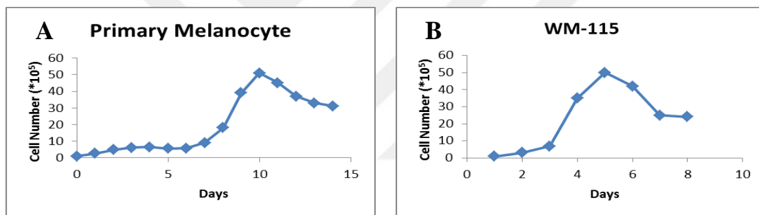
Figure 3.7: The growth curve of A)Primary epidermal melanocytes and B)WM-115 human melanoma cells in 14 days and 7 days, respectively.
