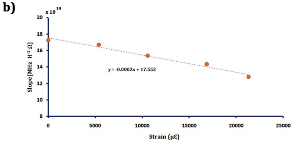
Figure 3.4: (a): Resonance frequency variation under different strain levels at different interrogation distances. Linear fits at various strain values intersect at a common interpolated reference point. Due to close proximity of the sensor and reader antenna (dominant coupling effect), measured signals tend to intersect at this point at different strain levels. (b): The calculated slope of any measured point with the reference point corresponds to an individual strain value (measured by strain gauge).
