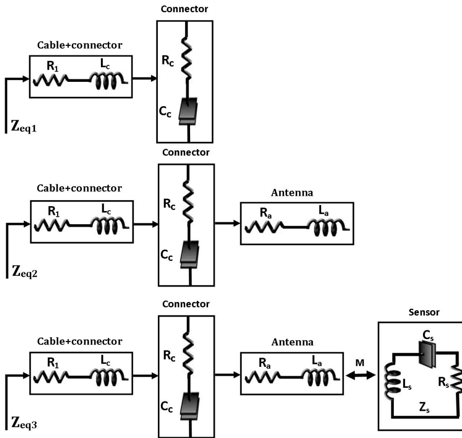
Figure 2.1: Schematic of the proposed system. The sensor is inductively coupled to the pick-up reader antenna. To obtain the exact value of the resonance frequency ( f_0 ) of the sensor, all the resistance, capacitance and inductance values induced by the cable, the connector, and the antenna are included.
