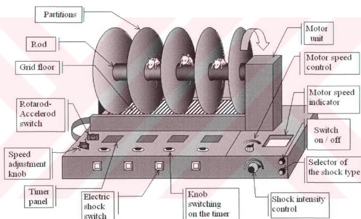
Figure 2.6. Rotarod / Accelerod Apparatus (Adopted from Uzbay, 2004).
