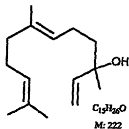
Nerolidol ( 48 )
