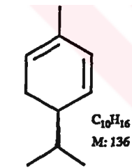
(-)- \alpha - Fellandren ( 3 )
