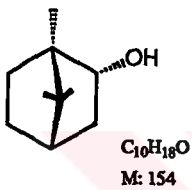
(-)- Borneol ( 18 )
