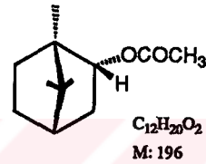
(-)- Bornilasetat ( 20 )
