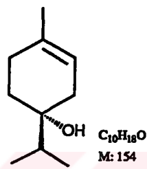
(-)- Terpinen-4-ol ( 36 )
