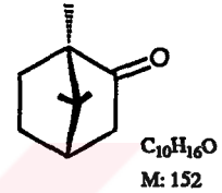
(+)- Kafur ( 21 )
