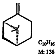
(-)- \beta - Pinen ( 11 )
