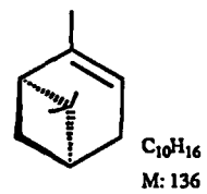
(-)- \alpha - Pinen ( 10 )
