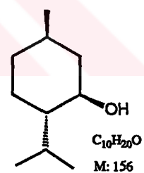
(-)- Mentol ( 25 )
