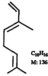
trans- Osimen ( 9 )
