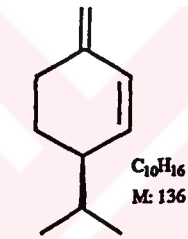
(-)- \beta - Fellandren ( 4 )
