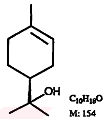
(-)-α- Terpineol ( 37 )
