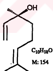
(-)- Linalol ( 24 )
