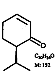
(-)- Piperiton ( 30 )
