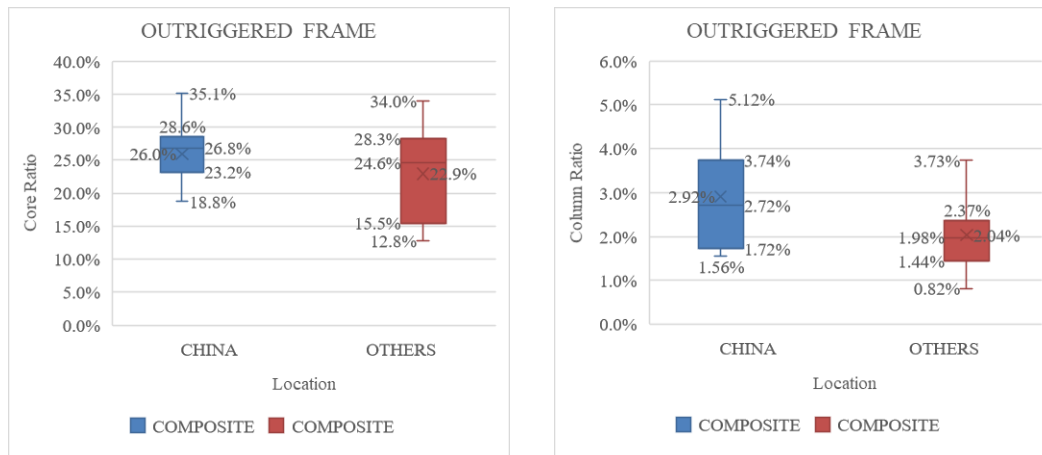
Figure 4.28. Interrelation between core and column ratio and location in composite outriggered frame systems
