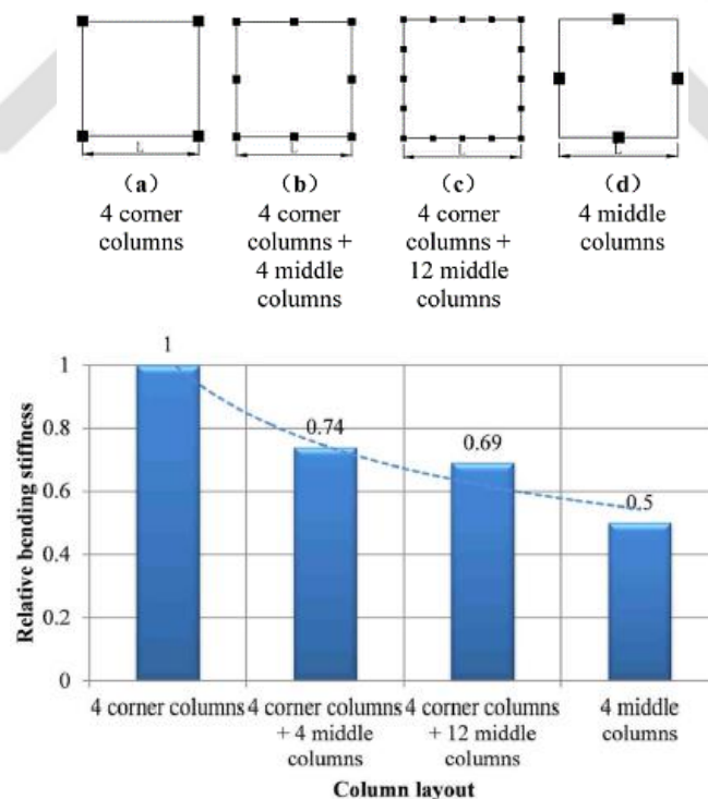
Figure 2.11. Relative bending stiffness of different vertical members (Source: Zhou et al. , 2014)
