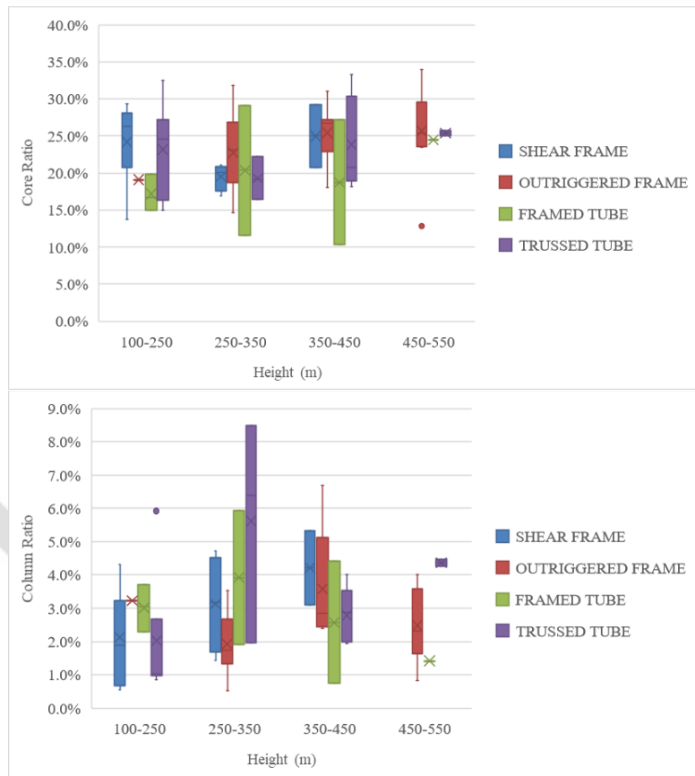
Figure 4.12. Core and column ratio distribution based on different height range in different structural systems in SG3
