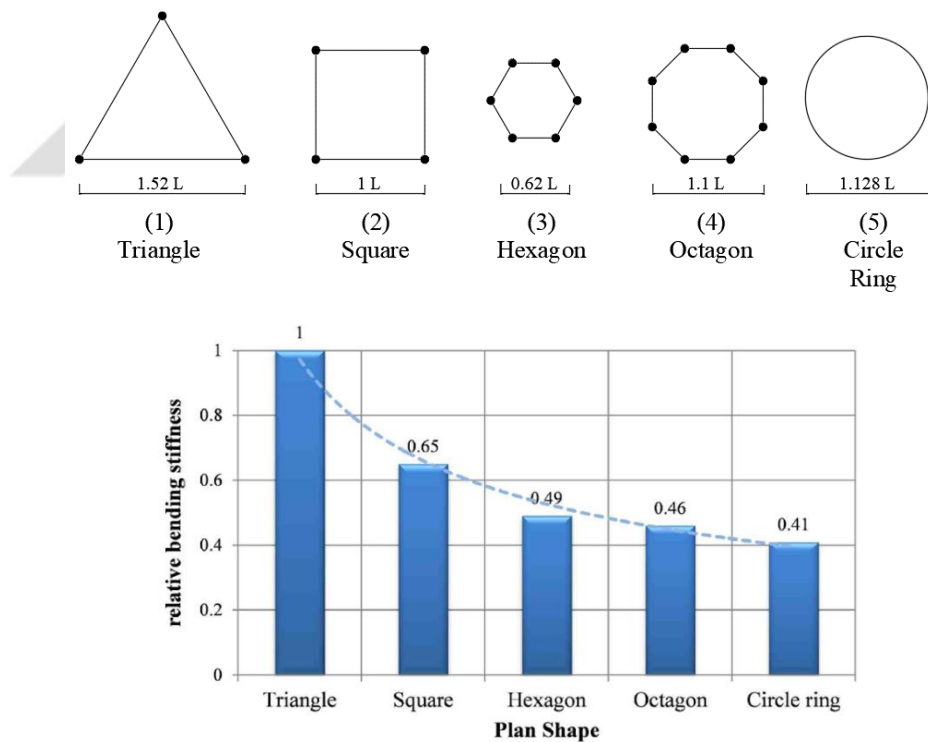
Figure 2.10. Relative bending stiffness of different floor plan shapes (Source: Zhou et al. , 2014)
