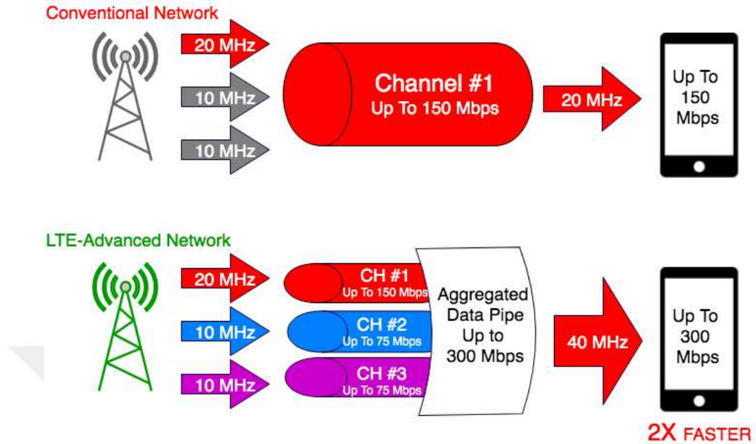
Figure 1.5. Comparison of conventional network with LTE-Advanced network, which aggregates one 20 MHz CC and two 10 MHz CCs.
