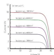
Current-Voltage Curve (LR6-60HPH-310M)
