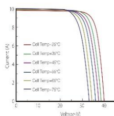
Current-Voltage Curve (LR6-60HPH-310M)
