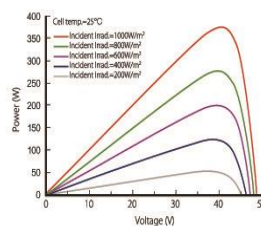
Power-Voltage Curve (LR6-72HPH-375M)
