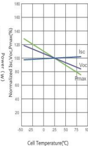
Temperature Dependence of Isc, Voc, Pmax
