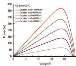
Power-Voltage Curve (LR6-72PH-370M)
