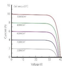
Current-Voltage Curve (LR6-60PE-310M)
