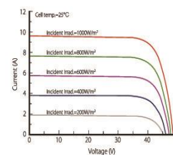
Current-Voltage Curve (LR6-72HPH-375M)
