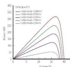
Power-Voltage Curve (LR6-60HPH-310M)
