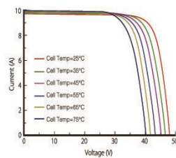
Current-Voltage Curve (LR6-72PH-370M)
