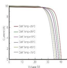
Current-Voltage Curve (LR6-60PE-310M)
