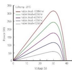
Power-Voltage Curve (LR6-60PE-310M)
