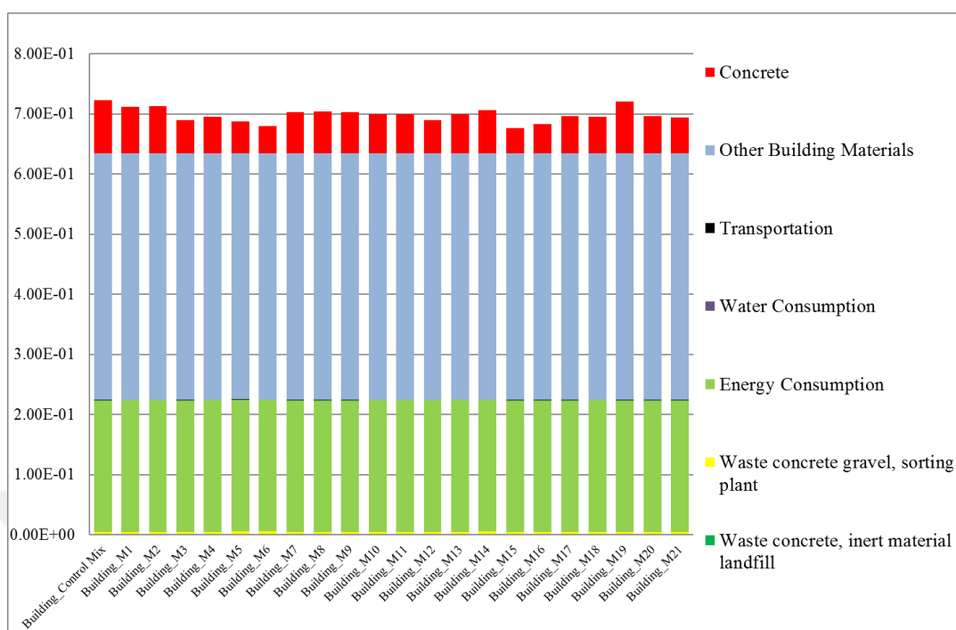
Figure 5.38. Characterization results of different building scenario for EP [kg PO 4 eq]
