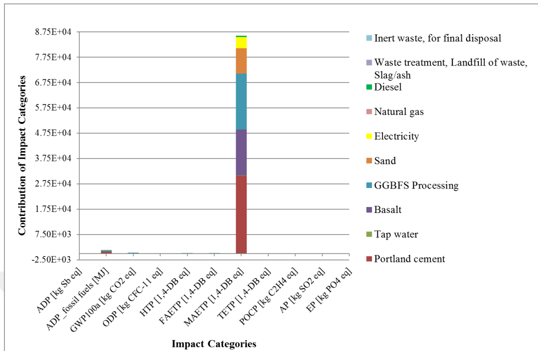
Figure 5.12. Characterization results of the Mixture-12 (Please see Table 4.12 for the definition of the impact categories)
