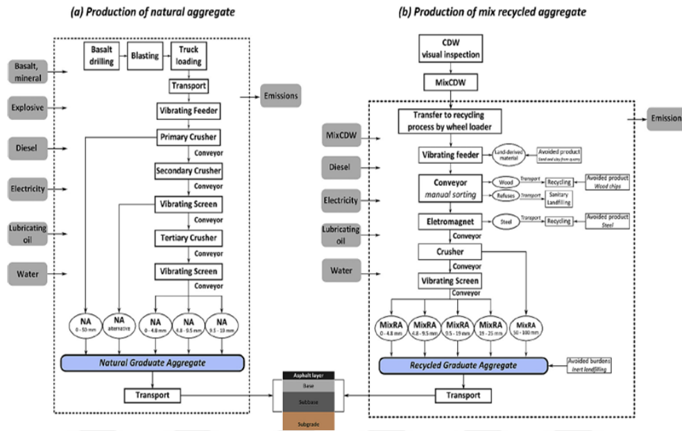
Figure 2.9. Conceptual diagram for natural and recycled aggregates [69]
