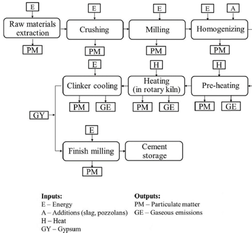
Figure 2.7. Representative process flow diagram for cement production [61]
