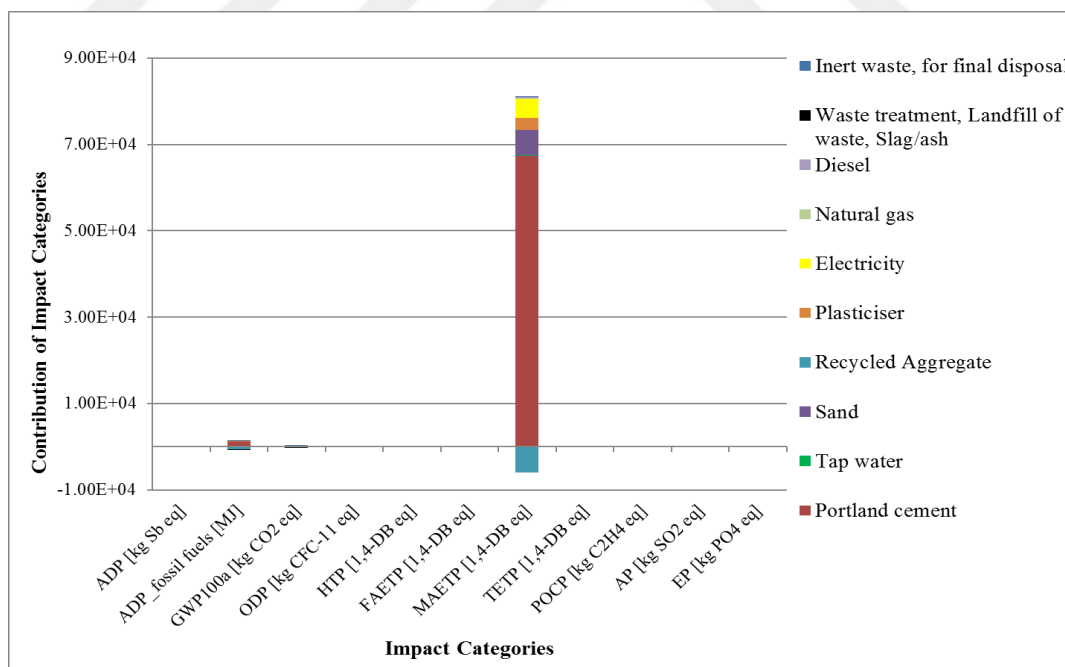
Figure 5.21. Characterization results of the Mixture-21 (Please see Table 4.12 for the definition of the impact categories)
