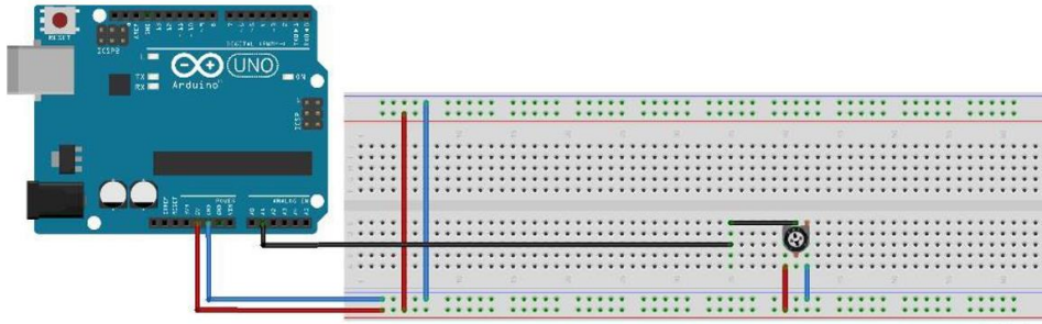
Figure 3.17. Potentiometer Circuit
