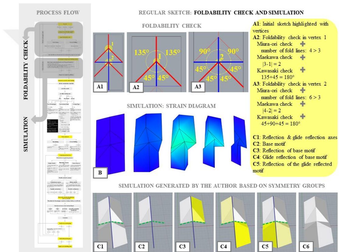
Figure 4.7. Foldability Check and Simulation of Regular Sketch (developed by the author)
