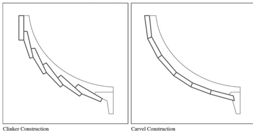
Figure 2: Clinker and Carvel Planking 74
