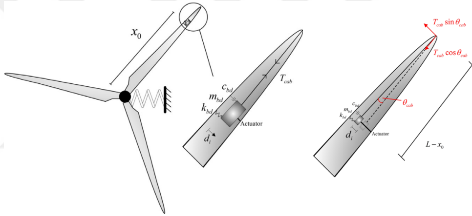
Figure 2.16: Cable connected ATMD inside the blade and cable arrangement[15]
