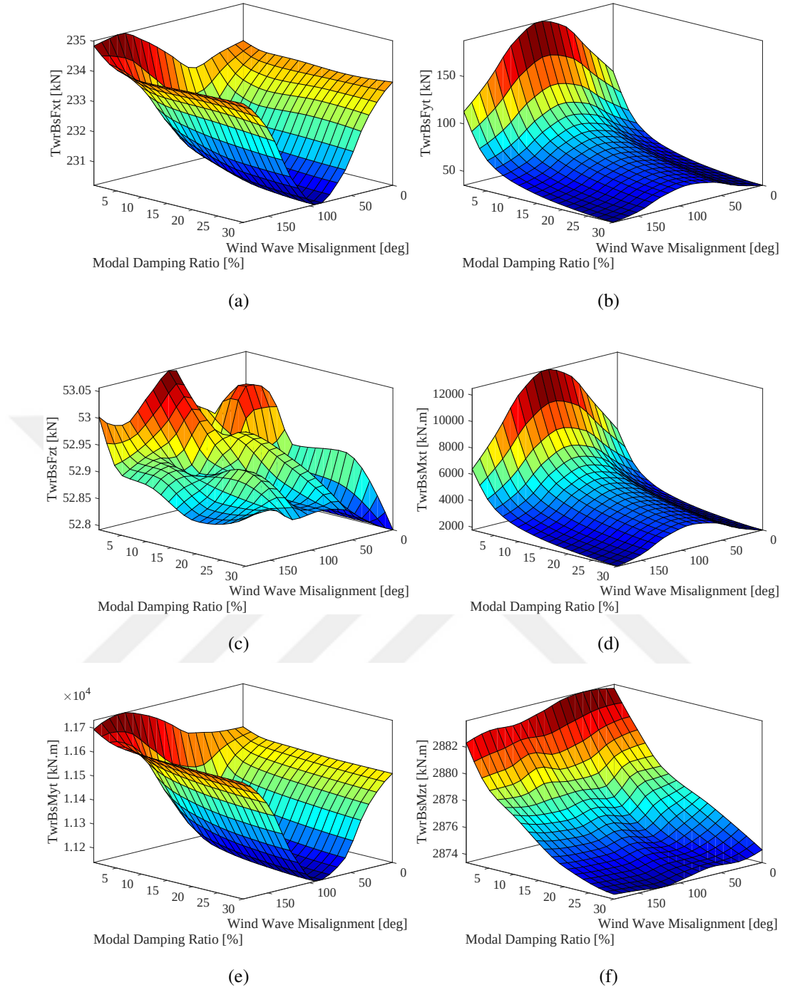
Figure 5.24: Damage Equivalent Loads for offshore wind turbine system with additional tower side-side modal damping
