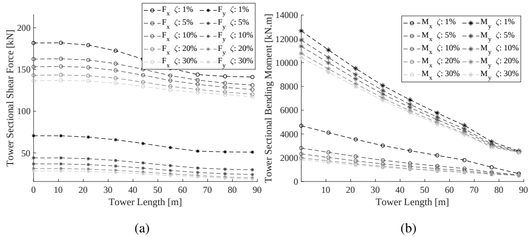
Figure 5.9: Sectional Lifetime Damage Equivalent Loads along the tower length( -\circ- : X / -* : Y )
