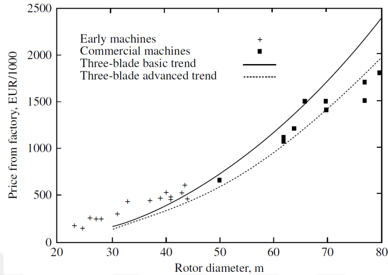
Figure 2.3: Relation between rotor diameter and cost[1]
