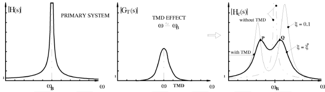
Figure 2.14: TMD effect on a system [13]
