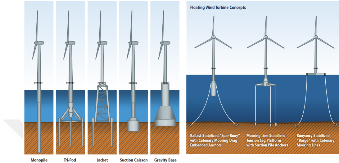
Figure 2.5: Shallow water structure[7]
