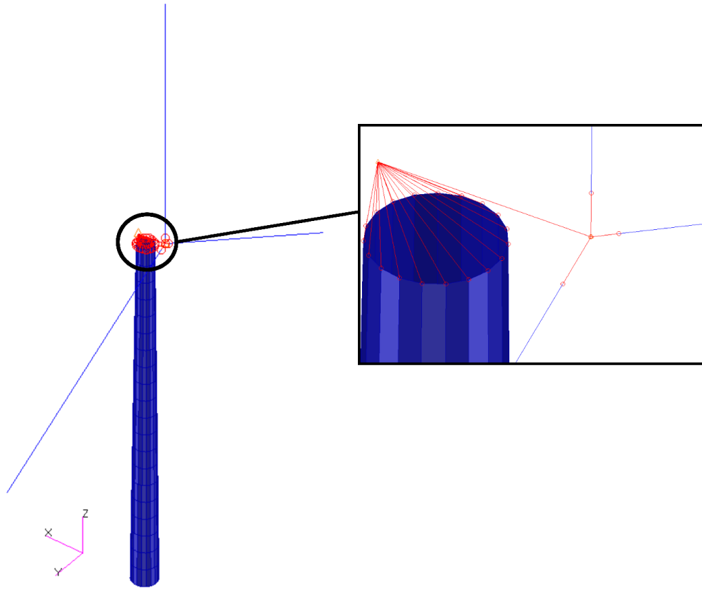
Figure 6.1: Finite Element Model of NREL 5 MW Wind Turbine
