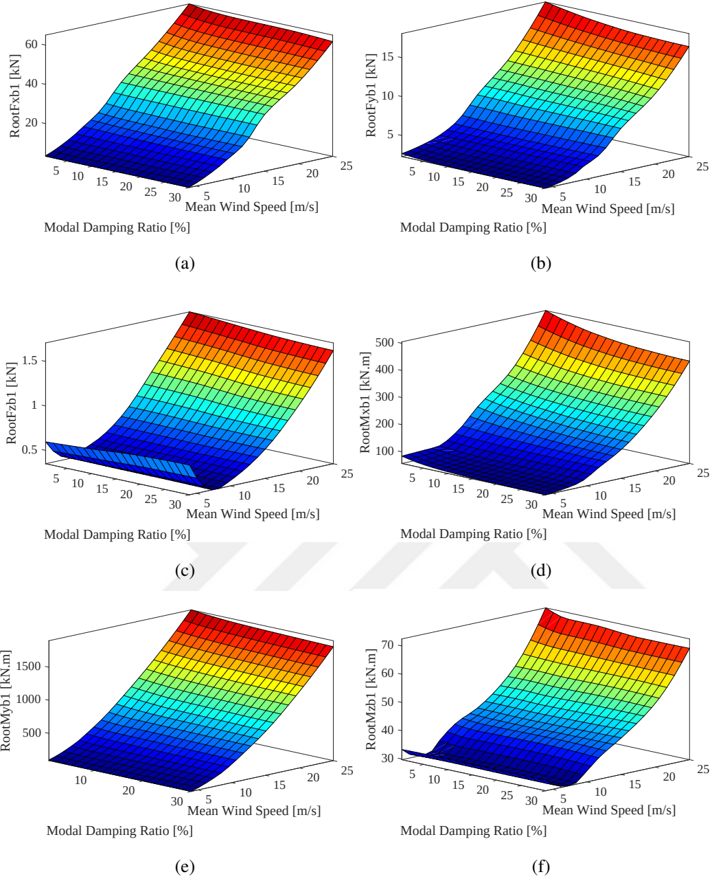
Figure 5.16: Damage Equivalent Loads for parked cases with additional blade flap-wise modal damping
