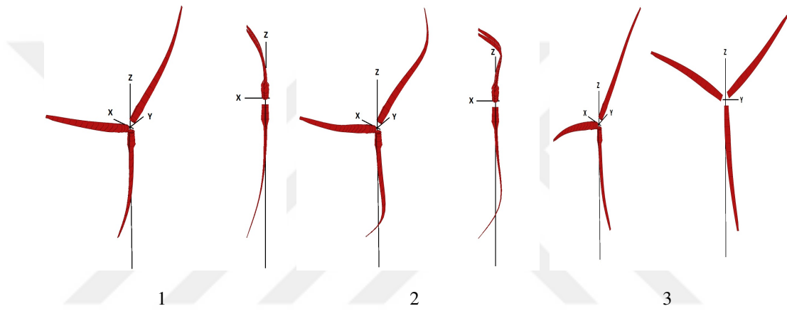
Figure 4.6: Mode shapes of the blade (1: first flapwise, 2: second flapwise, 3: first edgewise)
