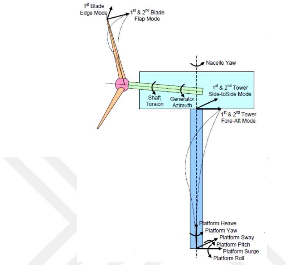
Figure 3.2: DOFs of a wind turbine in FAST model [17]
