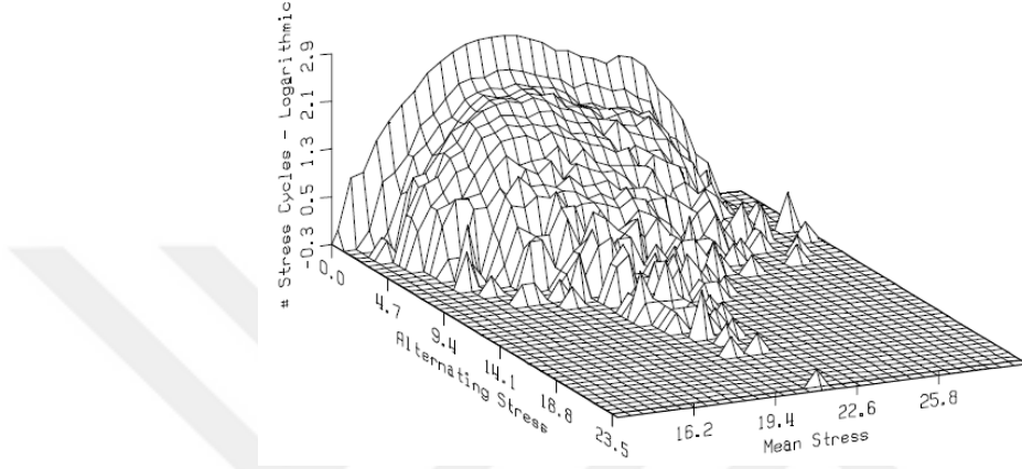
Figure 3.5: Rainflow counted stress data [20]
