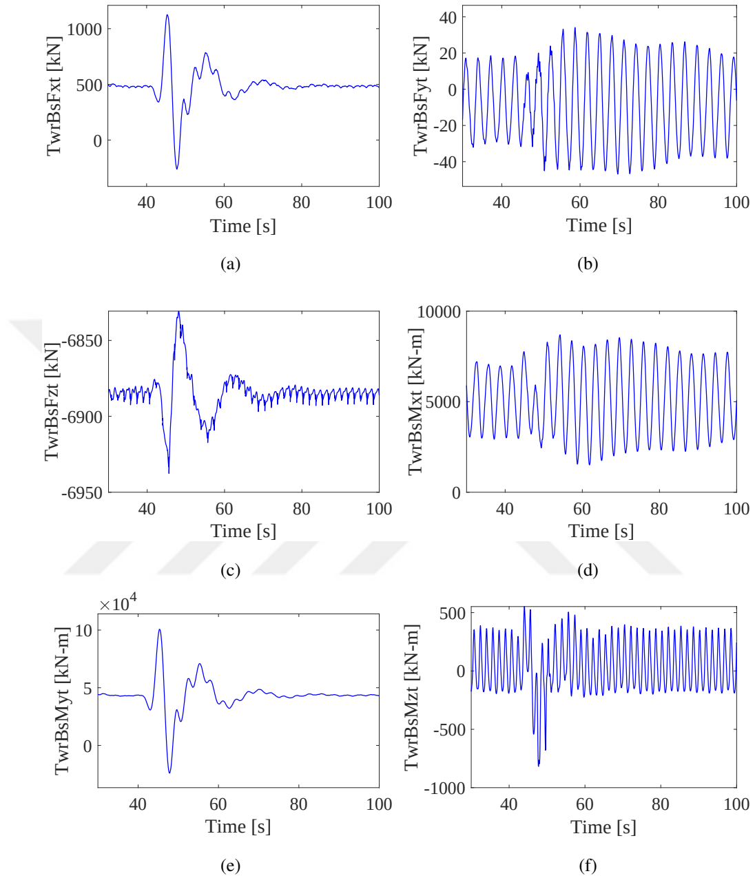
Figure 5.28: Tower base response to the Gust
