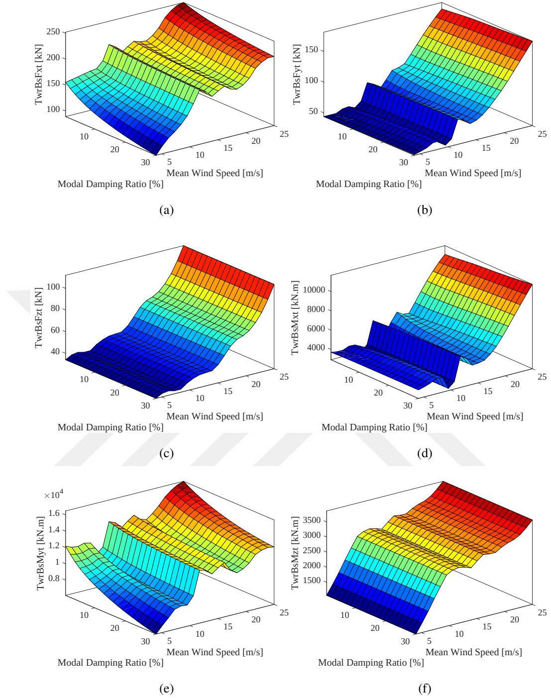
Figure 5.18: Damage Equivalent Loads for operating cases with additional tower fore-aft modal damping
