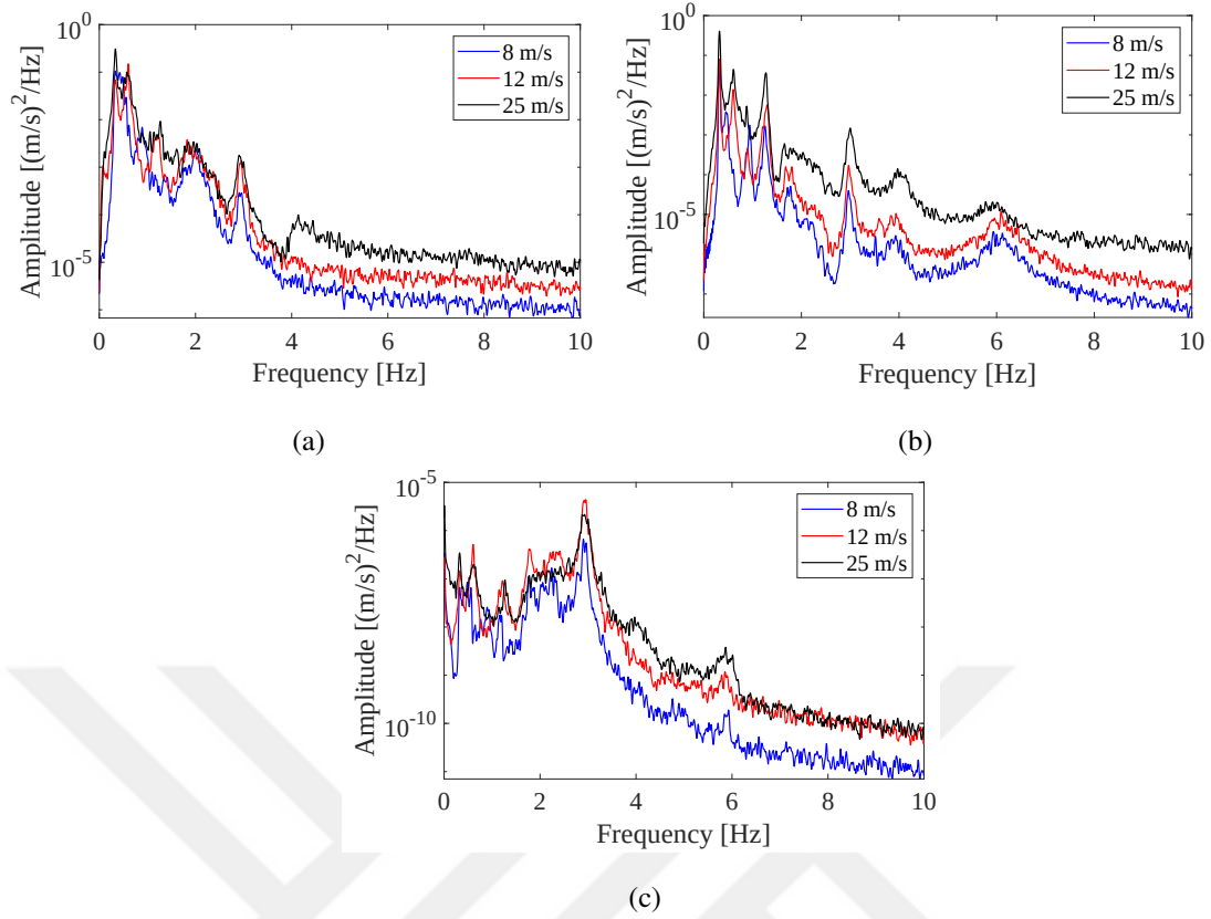
Figure 5.3: Tower top acceleration PSDs ((a): X, (b): Y, (c): Z)
