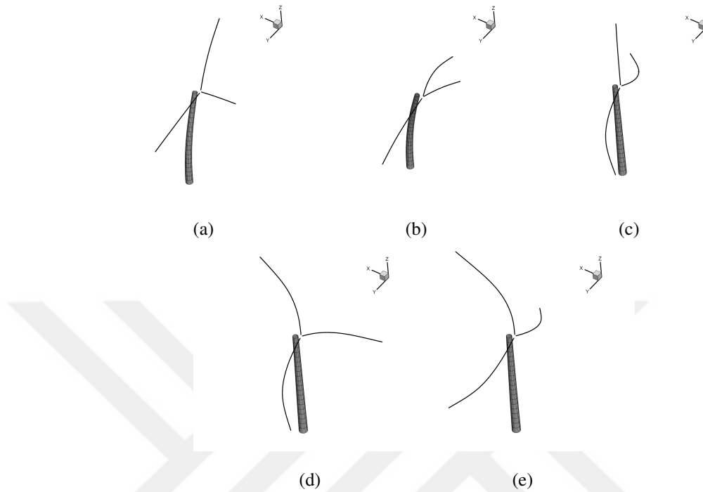
Figure 6.2: The first five mode shapes of the finite element model
