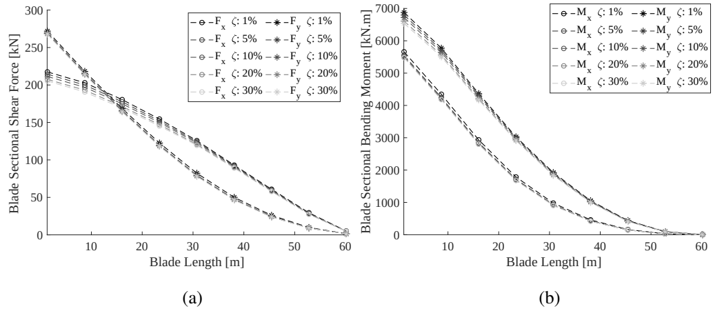
Figure 5.8: Sectional Lifetime Damage Equivalent Loads along the blade length ( -\circ- : X / -* : Y )
