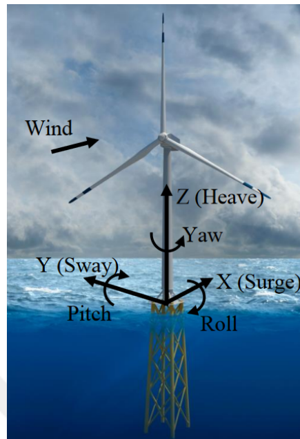
Figure 3.1: Global coordinate axes of FAST [16]
