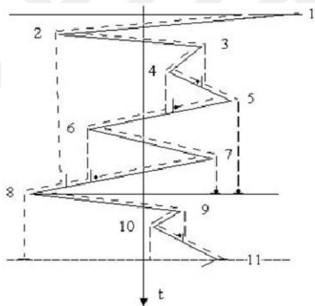
Figure 3.4: Rainflow counting [19]
