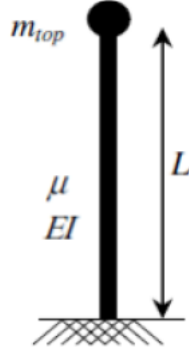
Figure 2.13: Cantilever beam model of a wind turbine [12]
