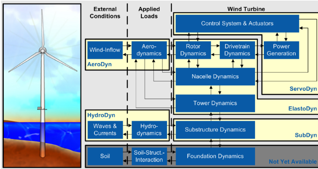
Figure 3.3: Main FAST scheme [18]
