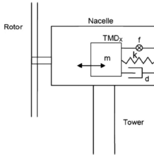
Figure 2.15: Construction of TMD in wind turbine[14]
