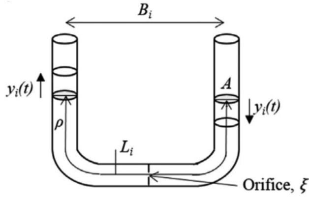
Figure 2.17: Tuned liquid column damper[14]
