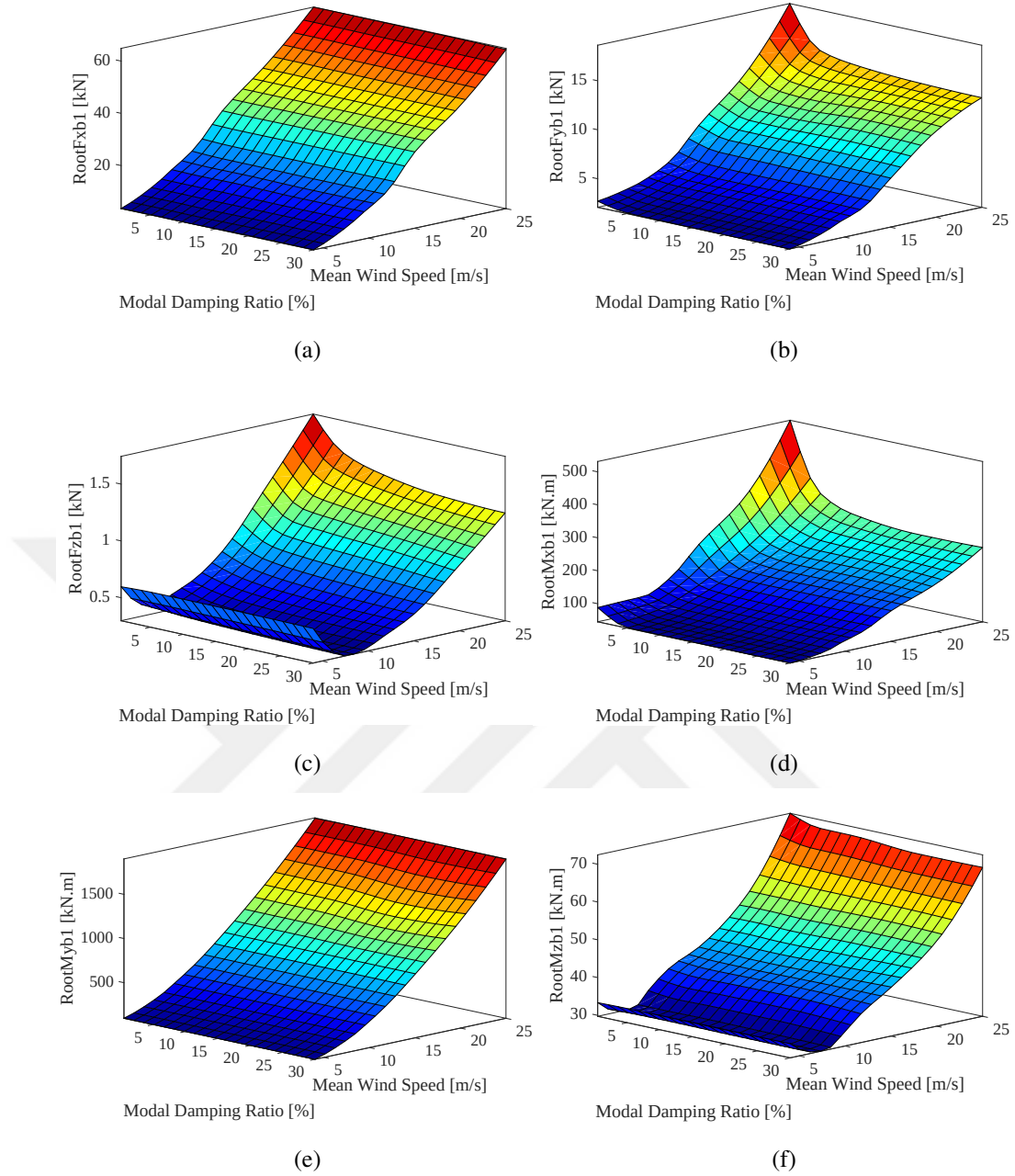
Figure 5.17: Damage Equivalent Loads for parked cases with additional blade edge-wise modal damping
