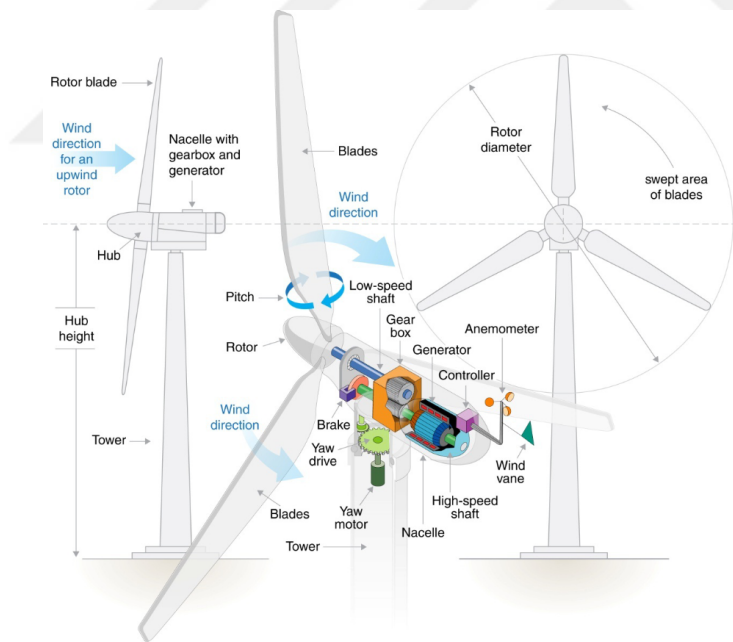
Figure 2.7: Wind turbine layout[9]
