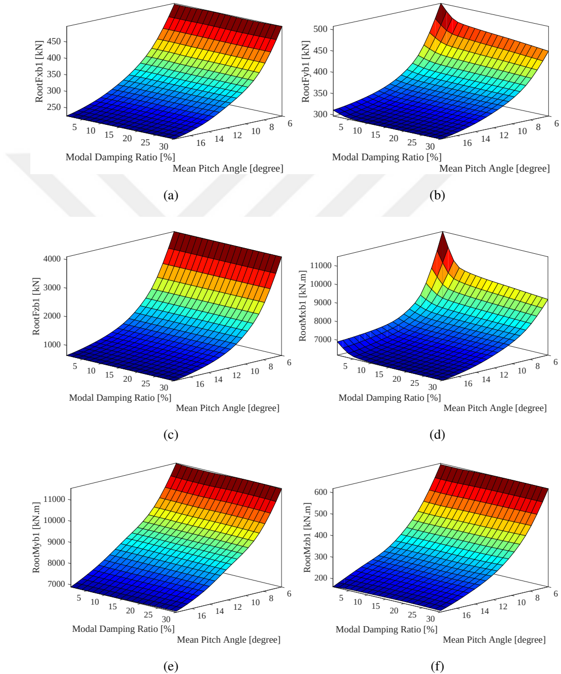
Figure 5.13: Damage Equivalent Loads for pitch cases with additional blade edgewise modal damping
