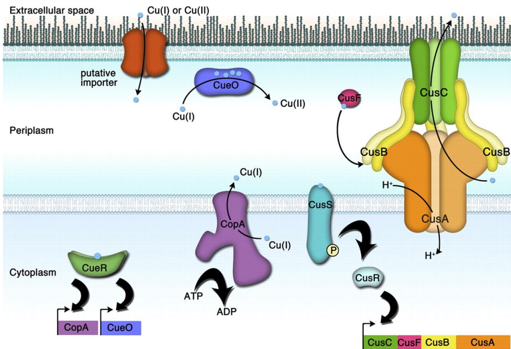
Figure 1.1. Copper homeostasis mechanisms in Escherichia coli (Kim et al., 2011).
