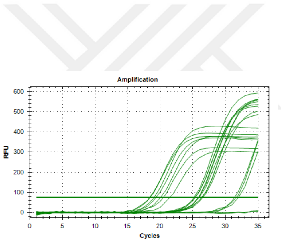
Figure 3.19. Amplification of all samples for cusF .
