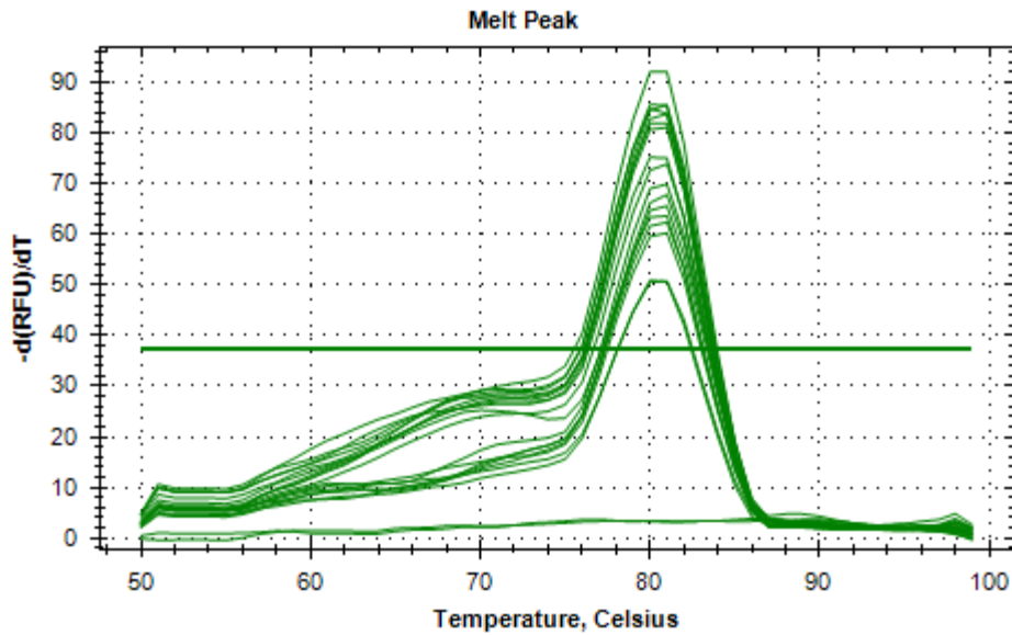
Figure 3.22. Melt peak of all samples for cusF .
