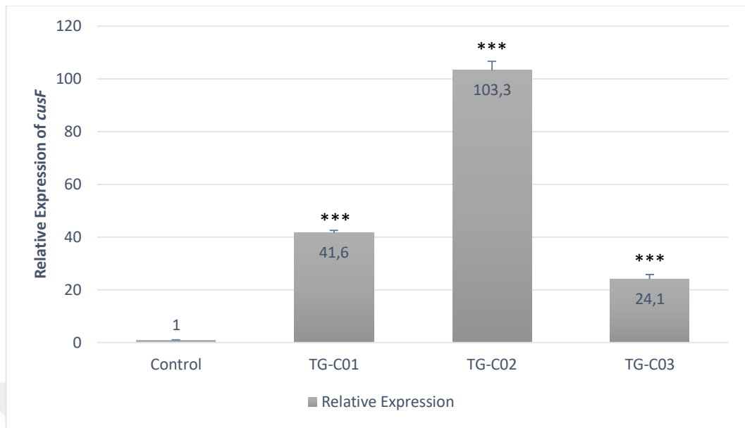
Figure 3.32. Relative expression of cusF in spontaneous (TG-C01 and TG-C02) and UV-induced (TG-C03) mutants. The relative expression of cusF was normalized in reference to tus gene. Fold changes are given within the bars for each mutant and calculated relative to the control strain; E.coli ATCC 8739. Standard Error of Mean (SEM) was used to represent the error bars. The confidence interval was 95%. P values; *( p \leq 0.05 ), ** ( p \leq 0.01 ), *** ( p \leq 0.001 ) by using one-way ANOVA test with Tukey's multiple comparison test.
