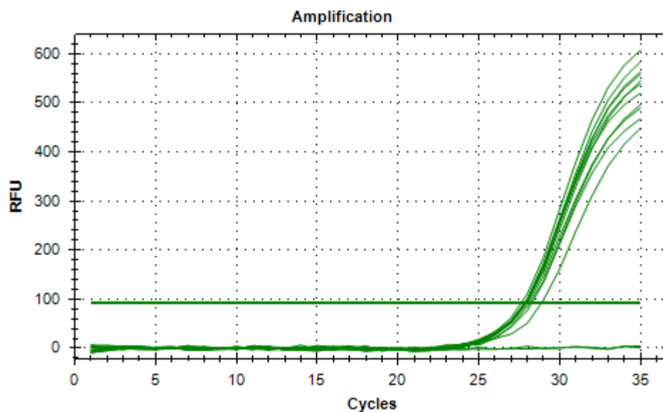
Figure 3.27. Amplification of all samples for tus .
