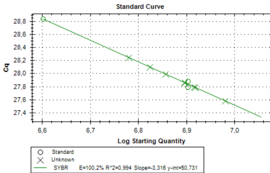
Figure 3.28. Standard curve analysis of all samples for tus .
