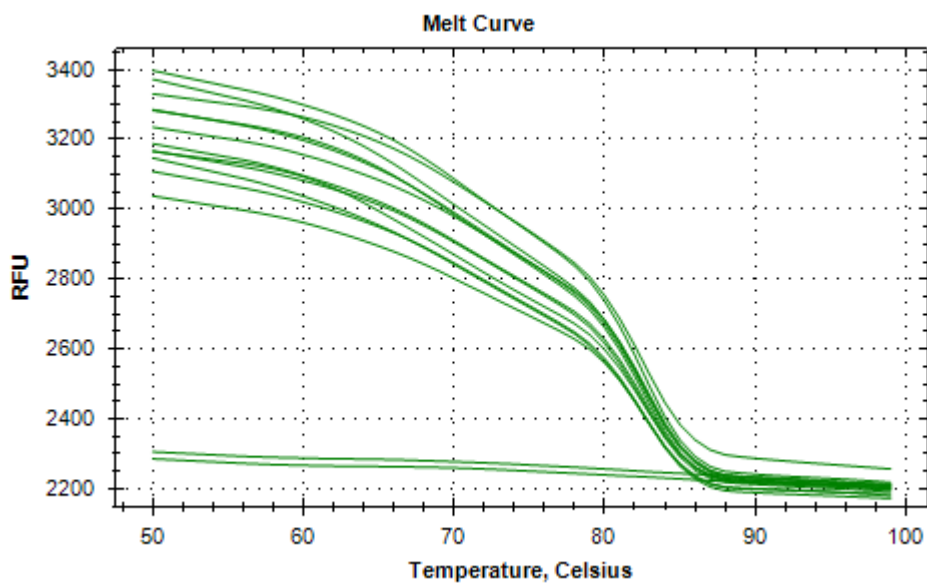
Figure 3.29. Melt curve of all samples for tus .
