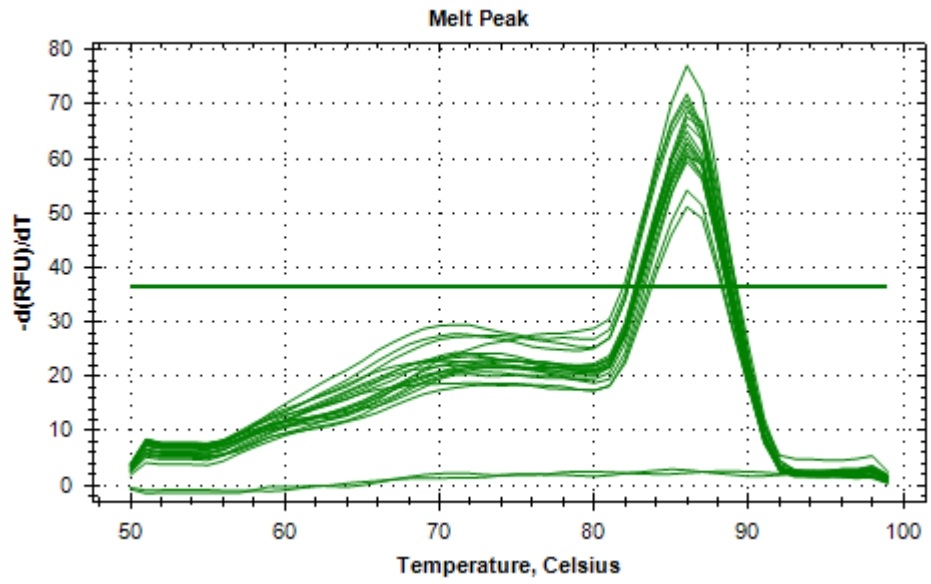
Figure 3.18. Melt peaks of all samples for copA .
