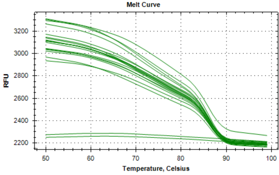
Figure 3.17. Melt curves of all samples for copA .
