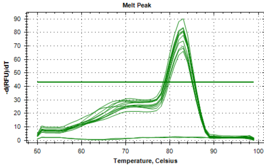
Figure 3.30. Melt peak of all samples for tus .
