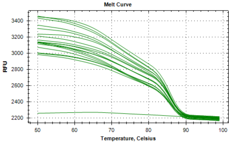
Figure 3.25. Melt curve of all samples for cusS .
