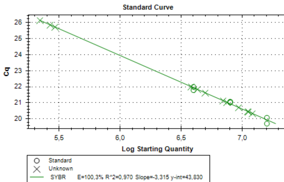
Figure 3.16. Standard curve analysis of all samples for copA .
