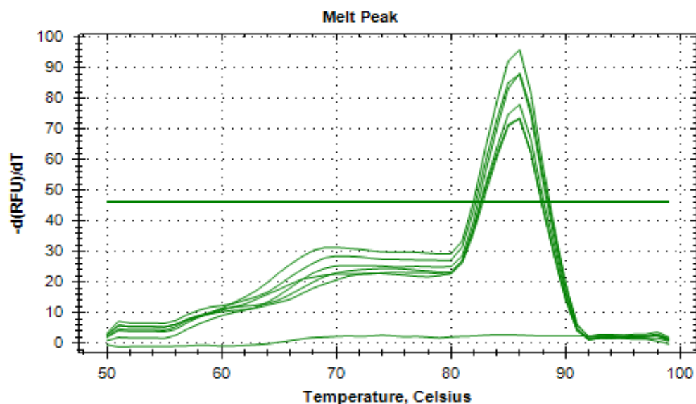
Figure 3.12. cusS melt curve analysis for standard curve determination.
