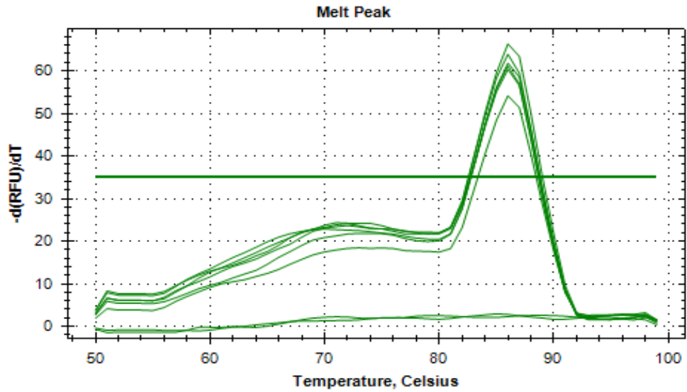
Figure 3.8. copA melt curve analysis for standard curve determination.
