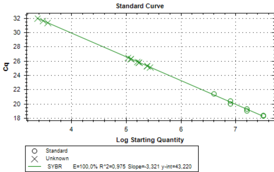
Figure 3.20. Standard curve analysis of all samples for cusF .
