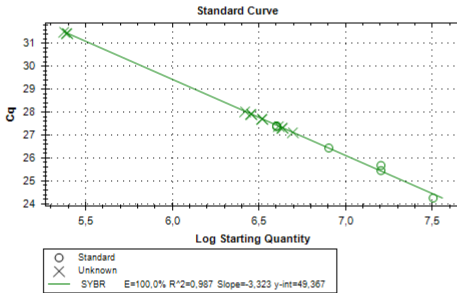
Figure 3.24. Standard curve analysis of all samples for cusS .
