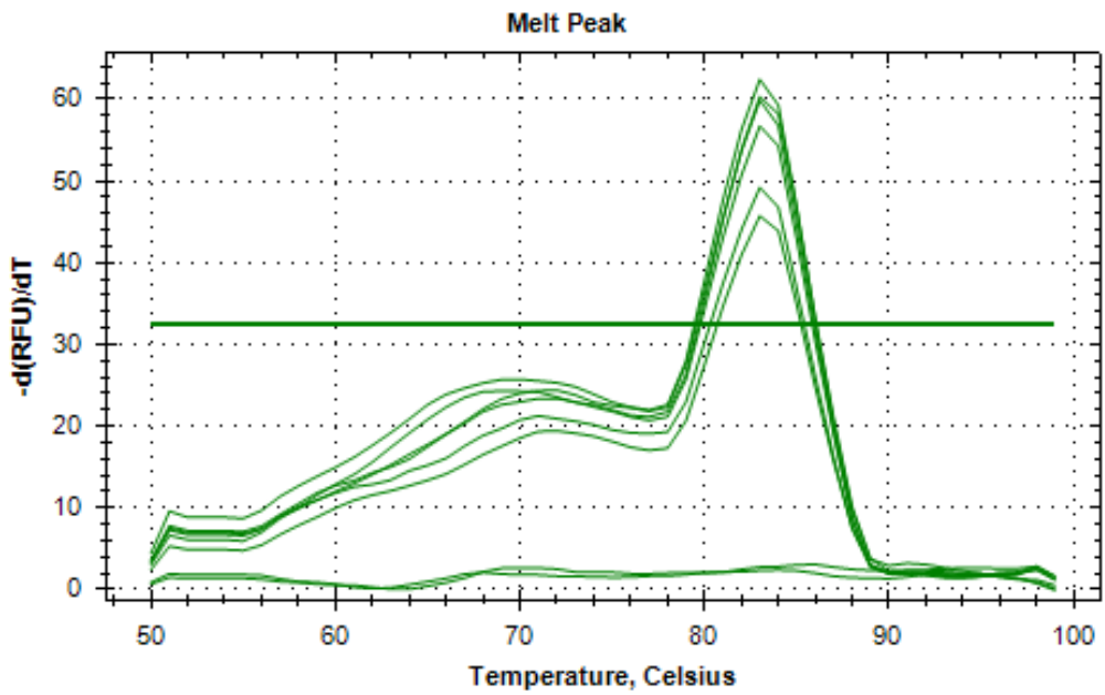
Figure 3.14. tus melt curve analysis for standard curve determination.
