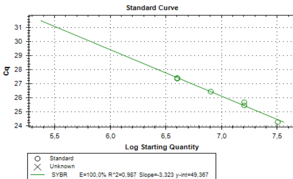
Figure 3.11. Standard curve analysis for cusS gene.
