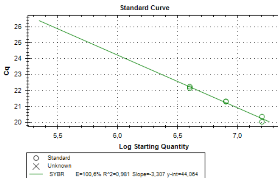
Figure 3.7. Standard curve analysis of copA gene.
