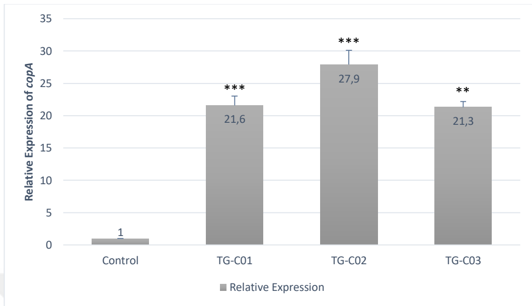
Figure 3.31. Relative expression of copA in spontaneous (TG-C01 and TG-C02) and UV-induced (TG-C03) mutants. The relative expression of copA was normalized in reference to tus gene. Fold changes are given within the bars for each mutant and calculated relative to the control strain; E.coli ATCC 8739. The error bars represent Standard Error of Mean (SEM). The confidence interval was taken as 95%. P values; * ( p \leq 0.05 ), ** ( p \leq 0.01 ), *** ( p \leq 0.001 ) by using one-way ANOVA test with Tukey's multiple comparison test.
