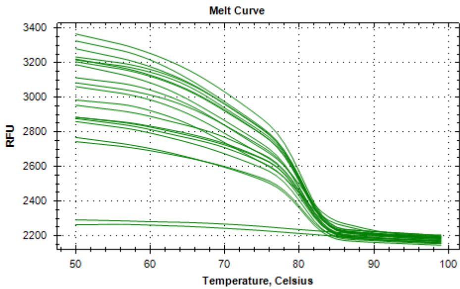
Figure 3.21. Melt curve of all samples for cusF .
