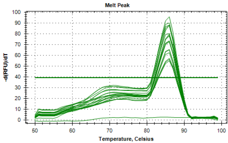
Figure 3.26. Melt peak of all samples for cusS .
