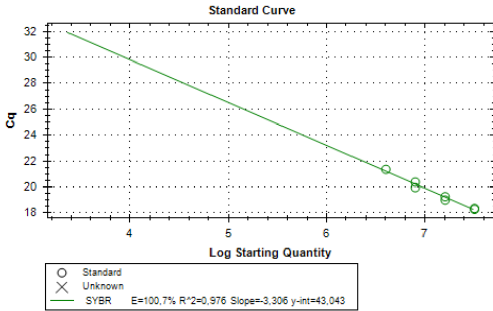
Figure 3.9. Standard curve analysis for cusF gene.
