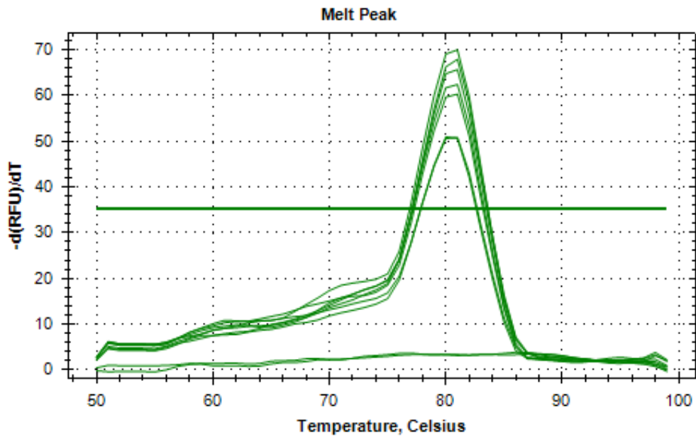
Figure 3.10. cusF melt curve analysis for standard curve determination.
