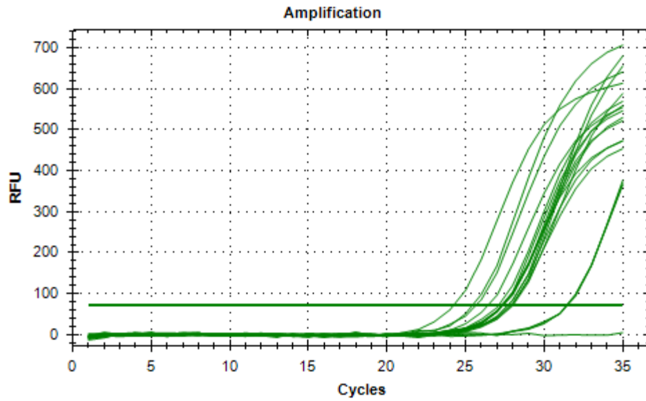
Figure 3.23. Amplification of all samples for cusS .
