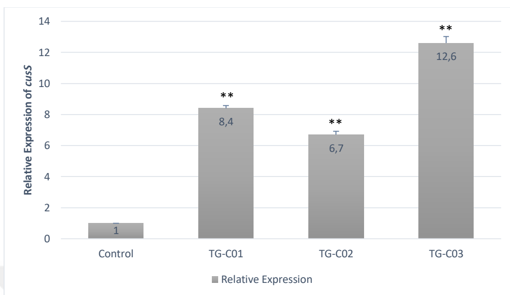
Figure 3.33. Relative expression of cusS in spontaneous (TG-C01 and TG-C02) and UV-induced (TG-C03) mutants. The relative expression of cusS was normalized in reference to tus gene. Fold changes are given within the bars for each mutant and calculated relative to the control strain; E.coli ATCC 8739. Standard Error of Mean (SEM) was used to represent the error bars. The confidence interval was 95%. P values; *( p \leq 0.05 ), ** ( p \leq 0.01 ), *** ( p \leq 0.001 ) by using one-way ANOVA test with Tukey's multiple comparison test.
