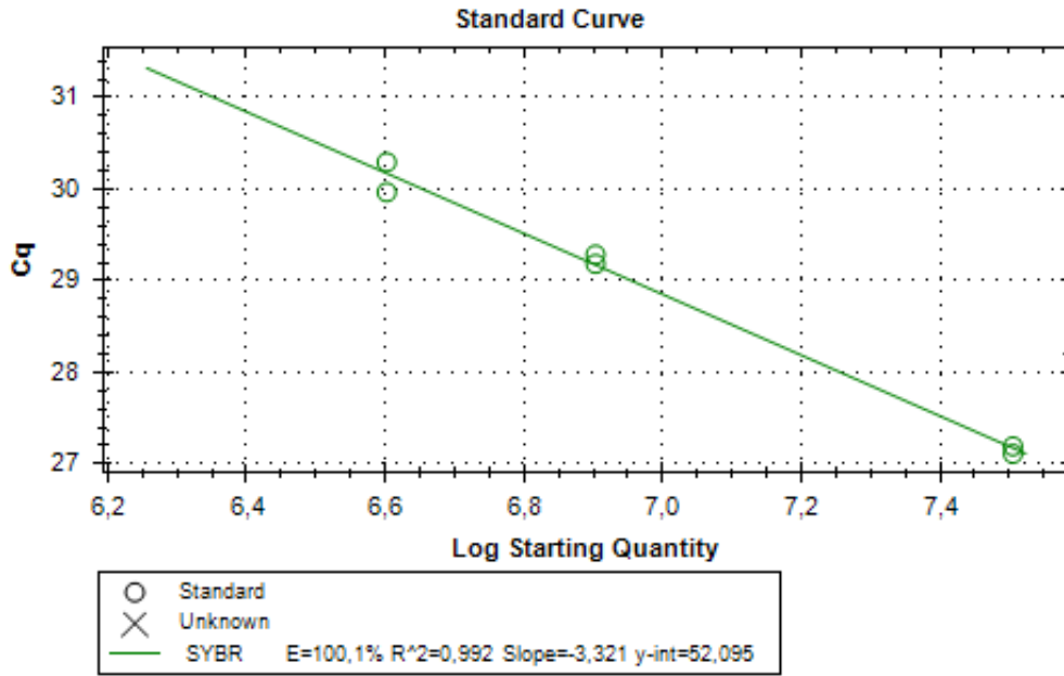
Figure 3.13. Standard curve analysis for tus gene.
