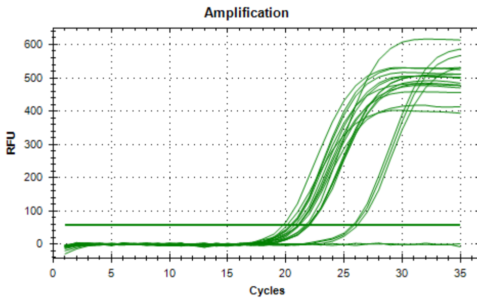
Figure 3.15. Amplification curves of all samples for copA .
