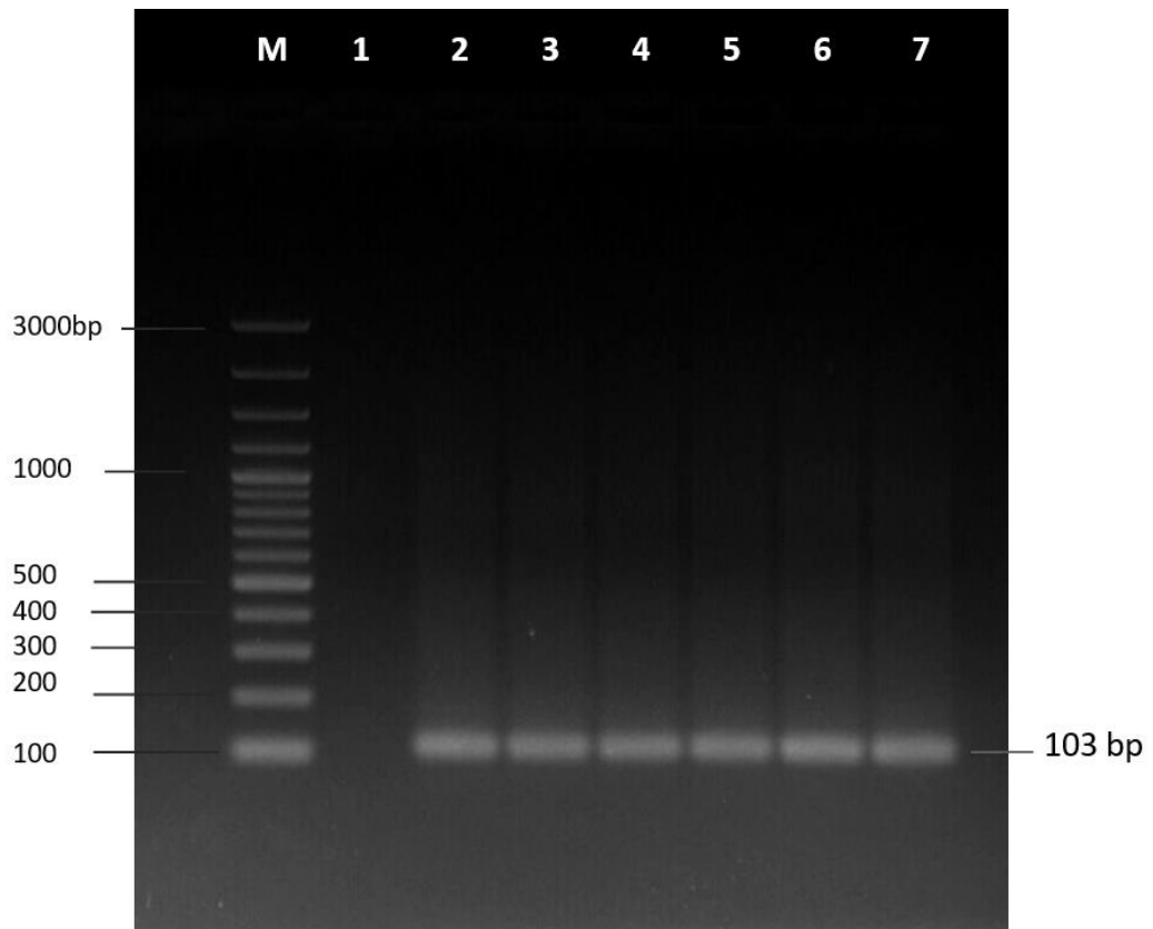
Figure 3.1. Annealing temperature optimization with temperature gradient PCR for tus : M, GeneRuler 100 bp Plus DNA Ladder; No template control (1); 54°C (2); 55,5°C (3); 58°C (4); 59,6°C (5); 62,3°C (6); 64°C (7).
