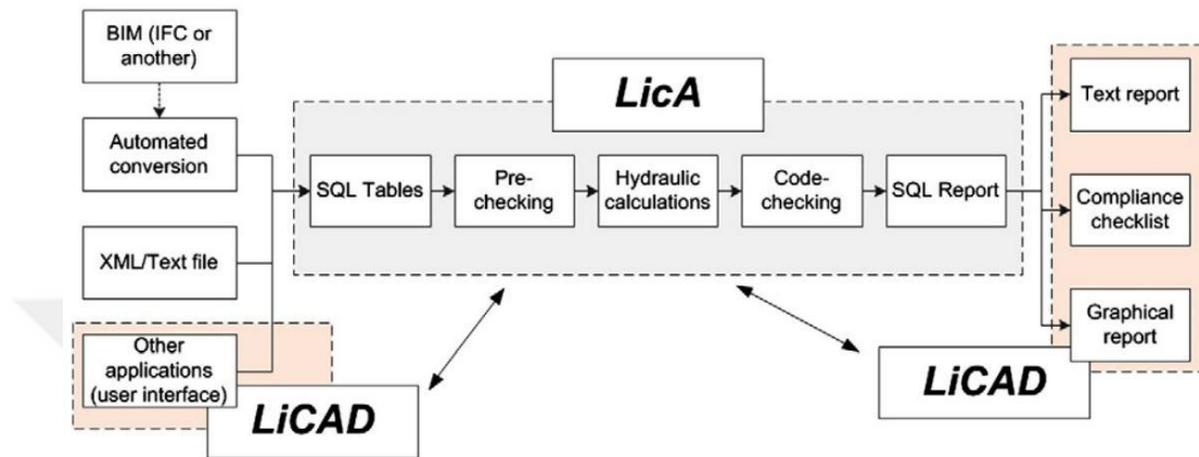
Figure 2.20. Conceptual Relations Between LicA and LICAD (Martins and Montiero, 2013)
