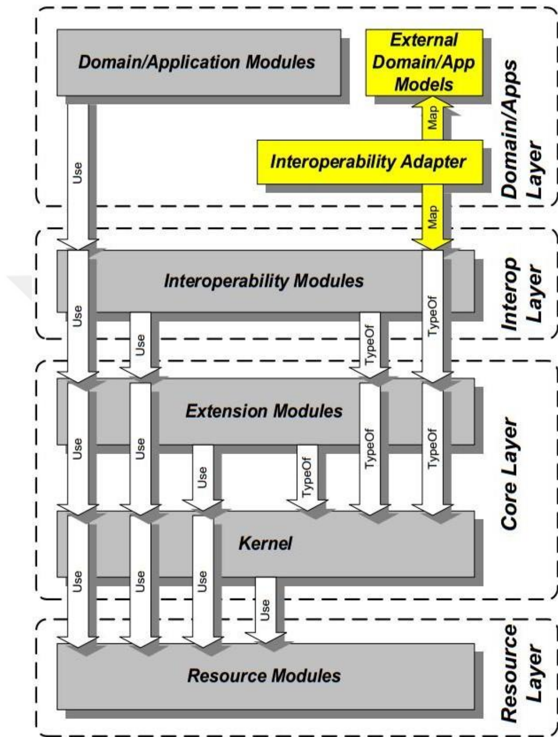
Figure 2.7. IFC Data Model Structure (International Alliance for Interoperability, 1999)
