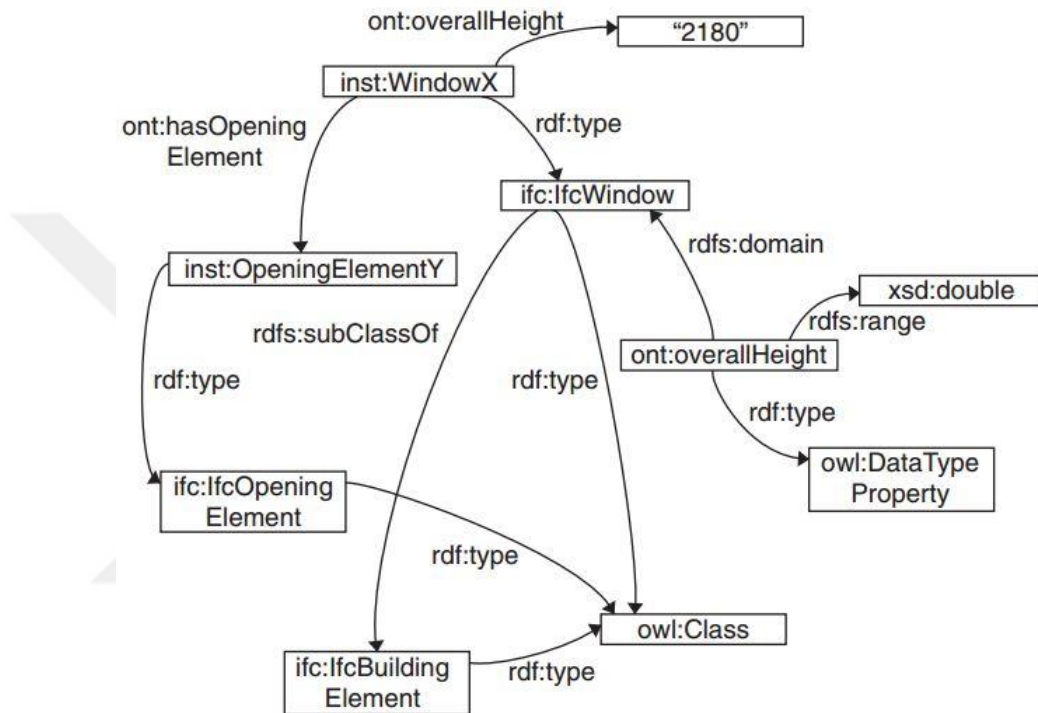
Figure 2.5. Graph Description of Window (Pauwels et al., 2011)
