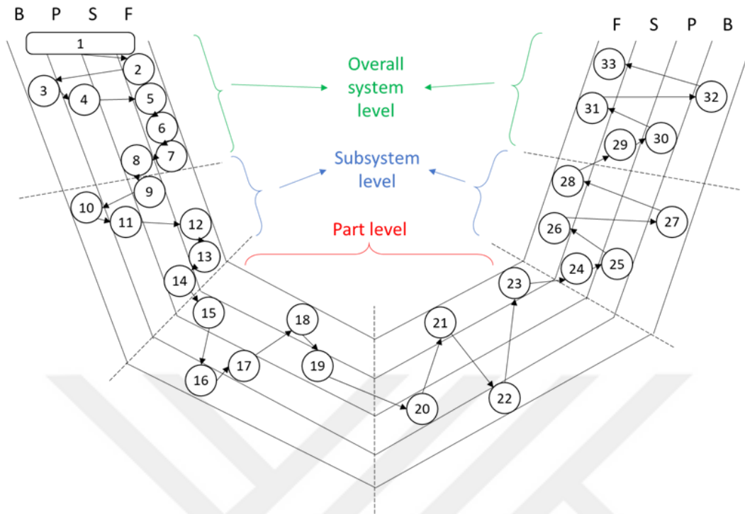
Figure A.5. Advanced procedure model of PPD on modified V-model [8]
