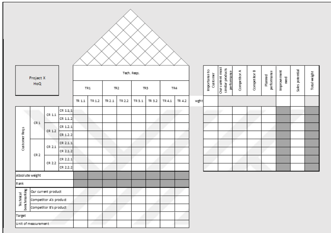
Figure 2.4. Representative HoQ chart
