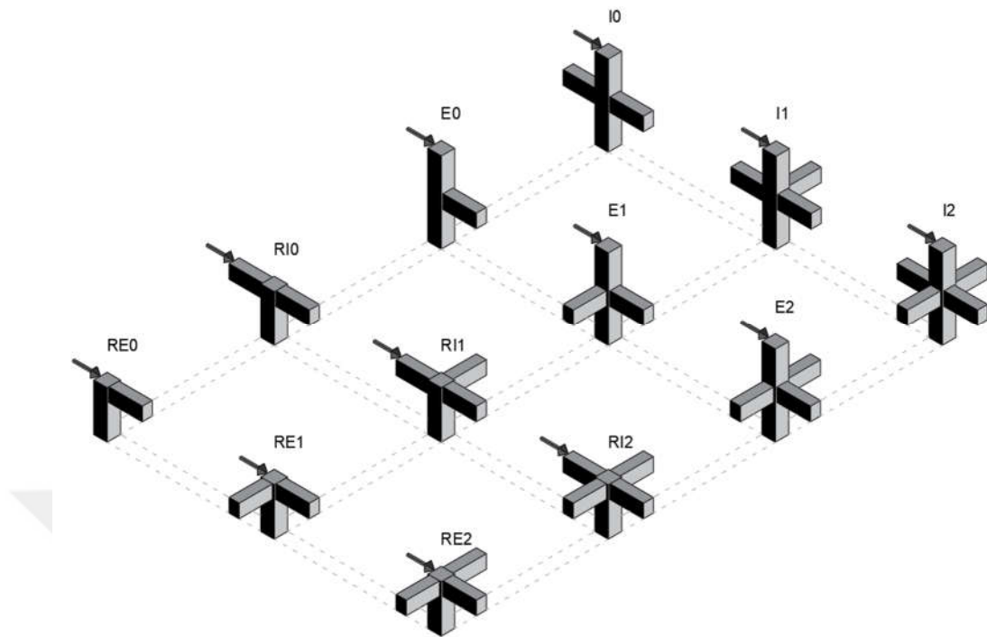
Figure 2.2. Beam-to-Column Joint Types proposed in this Study.
