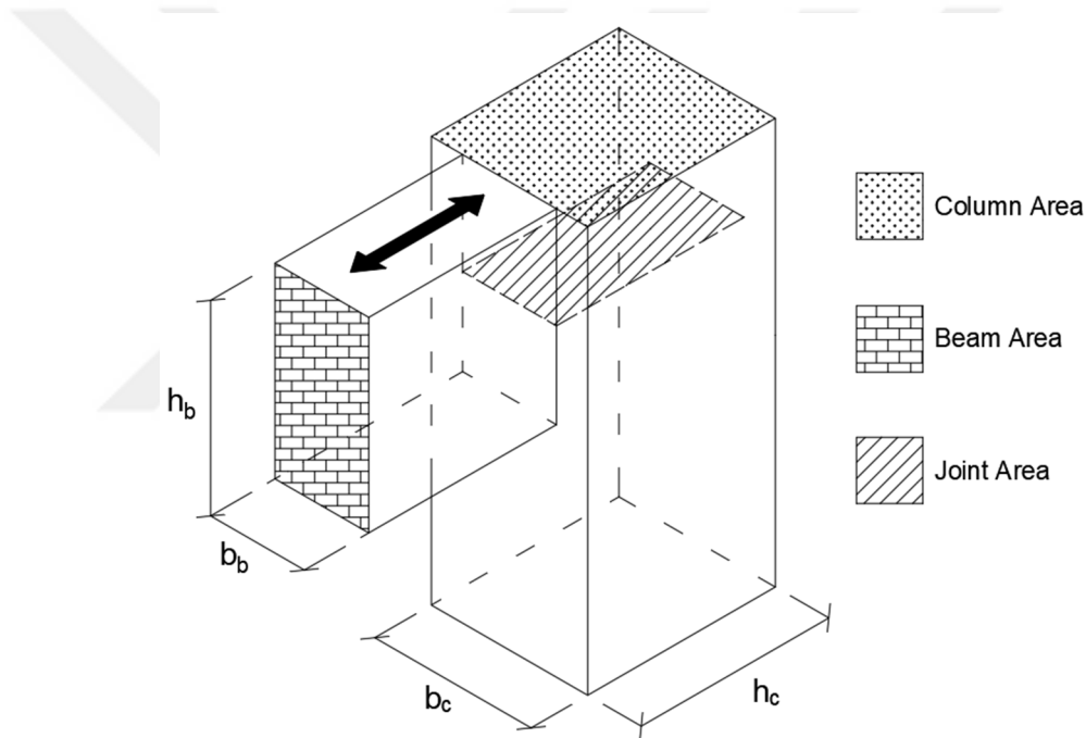
Figure 4.9. Column, beam and joint areas.
