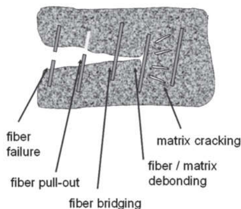
Figure 2.12. The mechanism by which fibers function. (ACI 544.4-18, 2018).
