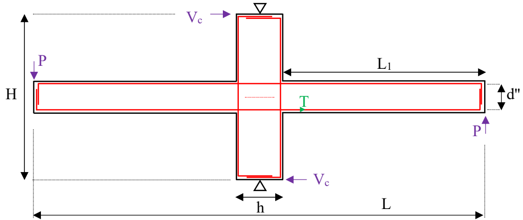
Figure 4.4. Interior beam-to-column connection loaded at beam ends.
