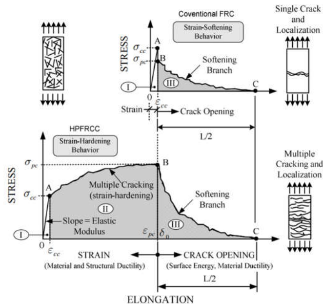
Figure 2.1. Comparison Tensile Behavior of FRCC & HPFRCC (Naaman, 2008).
