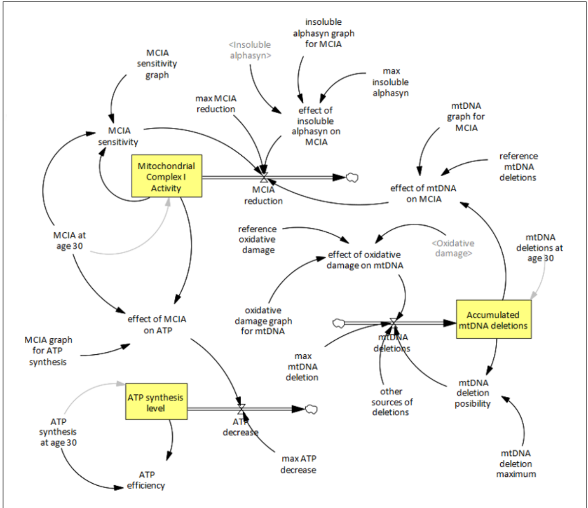
Figure 5.17. Stock-flow diagram of the mitochondria sector.
