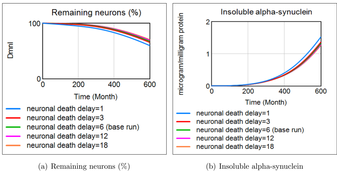
Figure 7.12. Model sensitivity to different neuronal death delay values.
