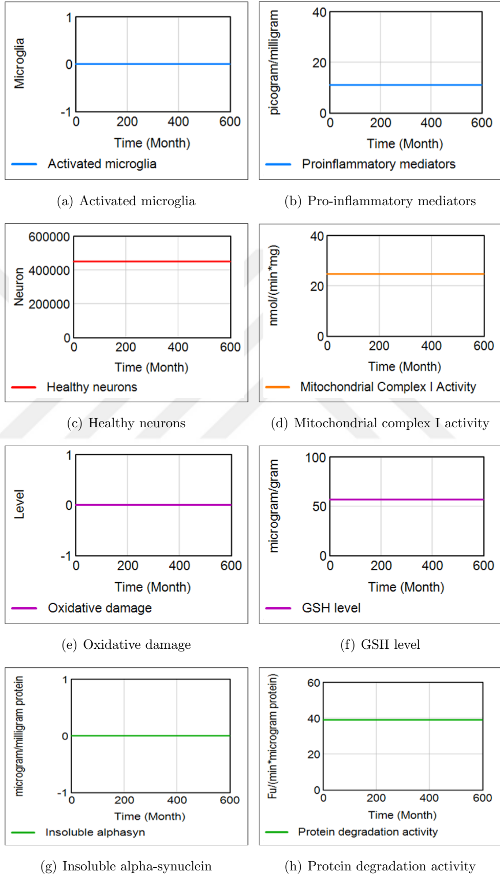
Figure 6.2. Hypothetical equilibrium run.
