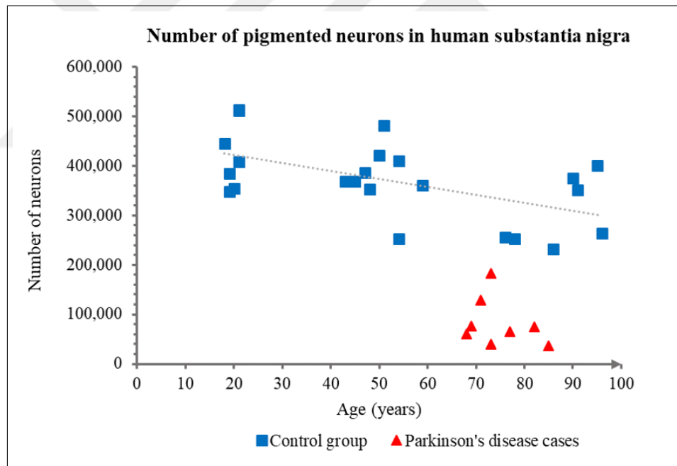
Figure 6.3. Real reference behavior of dopaminergic neurons (data from [116]).
