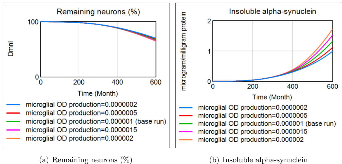
Figure 7.10. Model sensitivity to different microglial OD production values.
