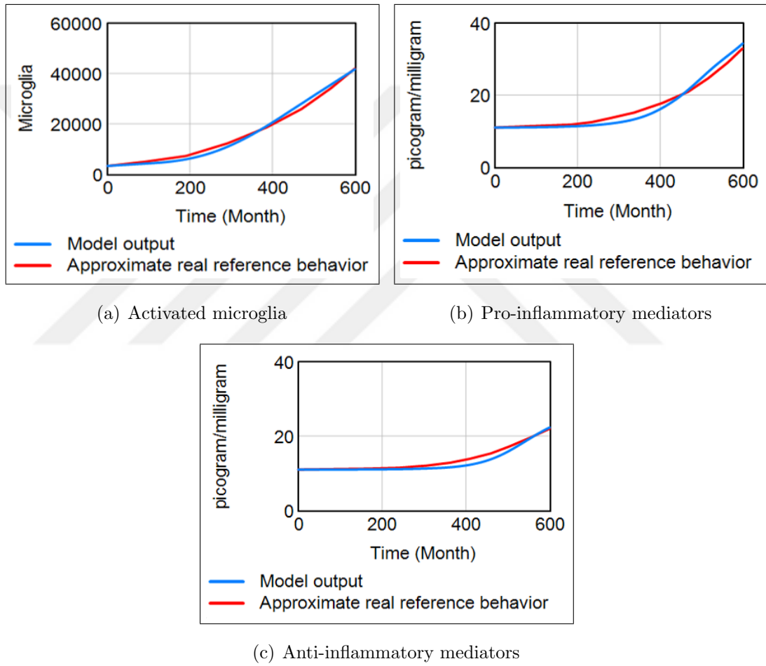
Figure 6.12. Comparison of model behavior and approximate real reference behavior for neuroinflammation sector.
