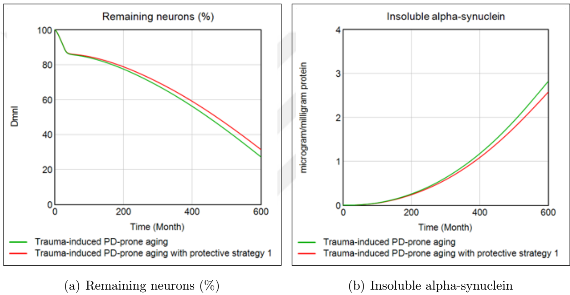
Figure 8.13. Comparative plots of Protective Strategy 1.
