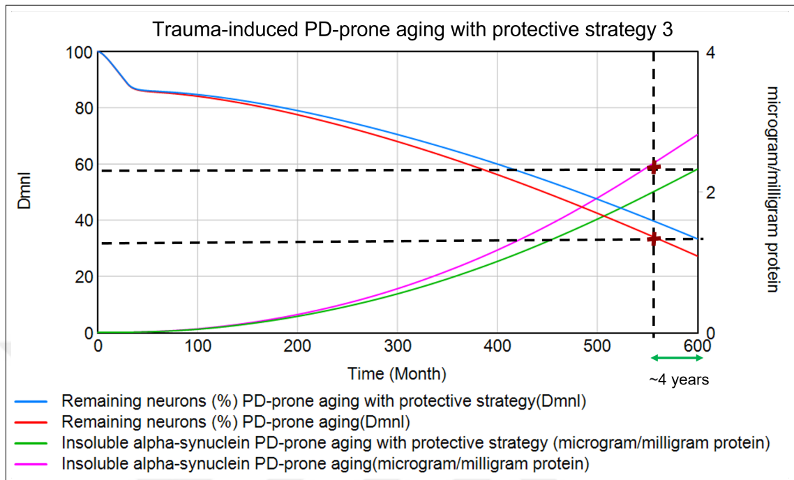
Figure 8.17. Potential disease symptom delay by protective strategy 3.
