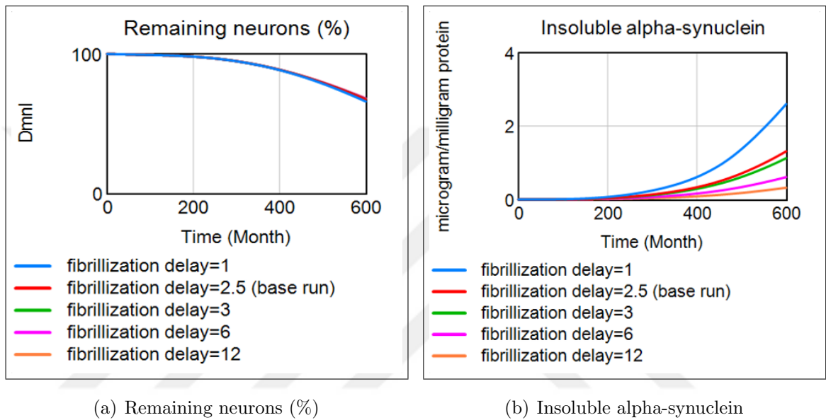
Figure 7.11. Model sensitivity to different fibrillization delay values.
