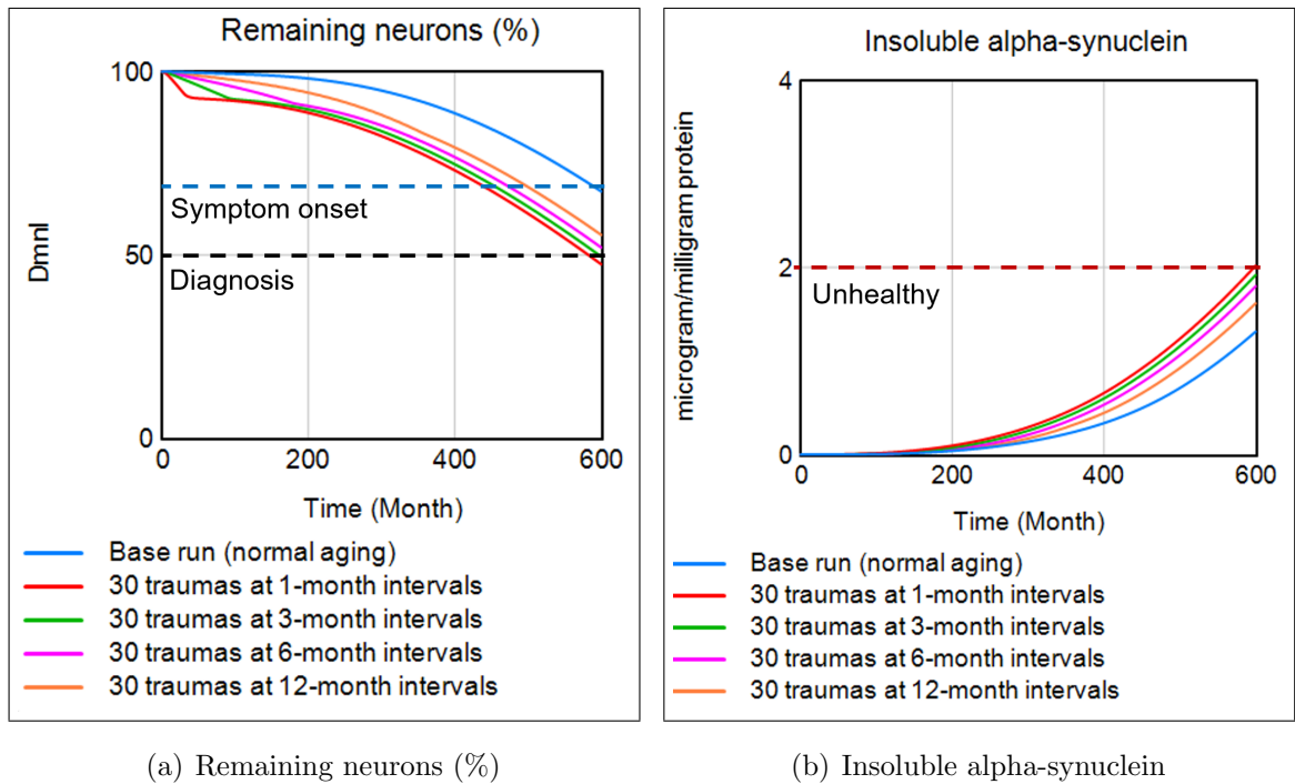
Figure 8.10. Comparative plots of Scenario 3.
