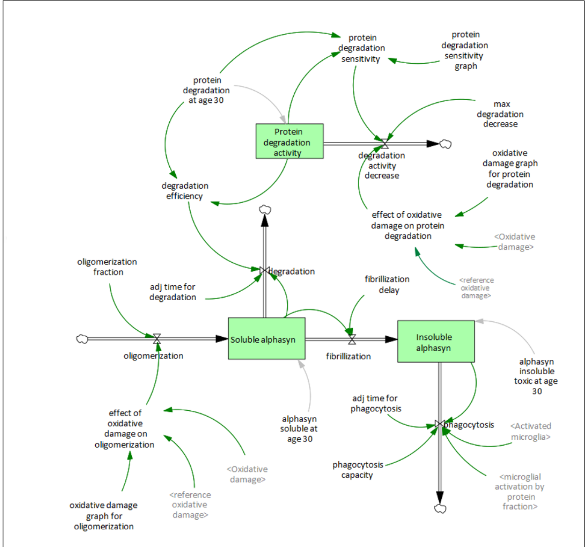
Figure 5.9. Stock-flow diagram of the protein aggregation sector.
