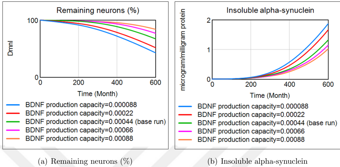
Figure 7.9. Model sensitivity to different BDNF production capacity values.
