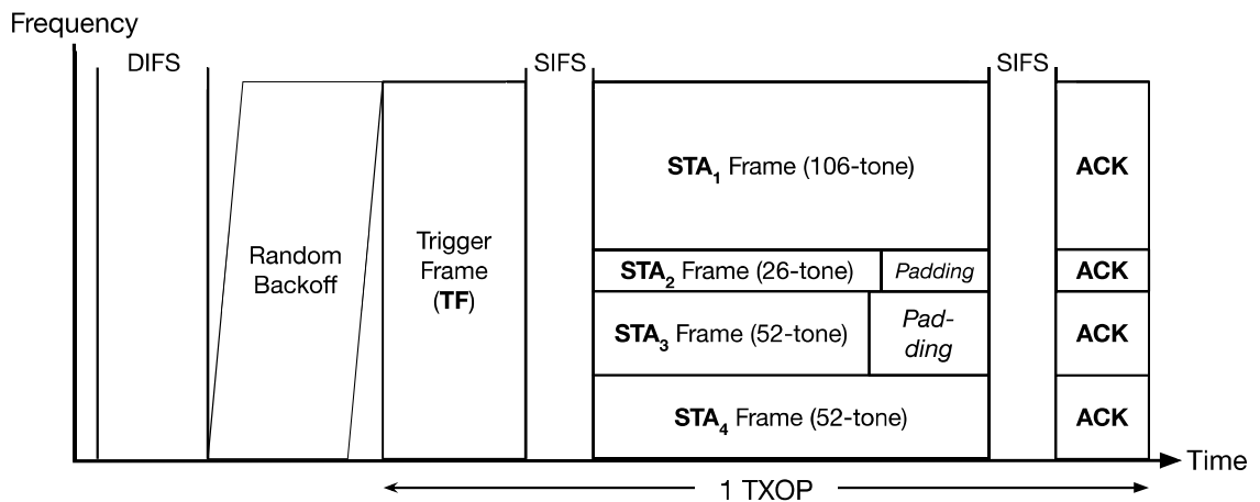
Figure 3.4. An example of IEEE 802.11ax UL-MU access for 20 MHz channel bandwidth with (106, 26, 52, 52) subcarrier allocations.
