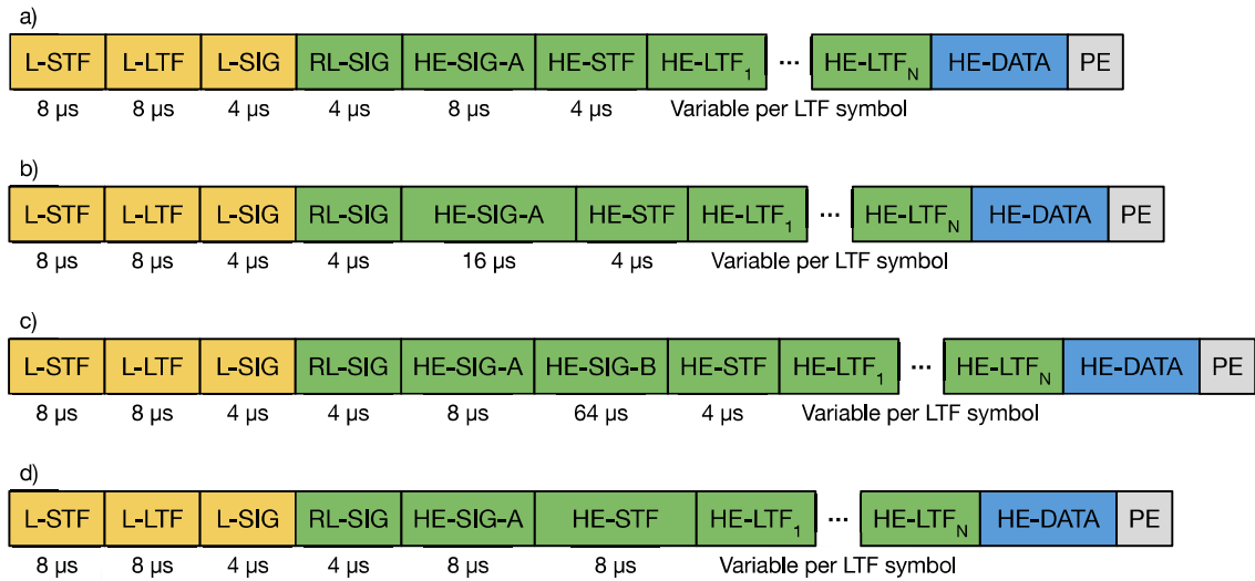
Figure 3.6. IEEE 802.11ax High Efficiency (HE) PPDU formats. a) HE Single User (SU) PPDU, b) HE Extended Range (ER) Single User (SU) PPDU, c) HE Multi-User (MU) PPDU, d) HE Trigger-based PPDU. Yellow ones (left) are legacy preamble, green ones are high-efficiency preamble, blue is data, and gray is packet extension.
