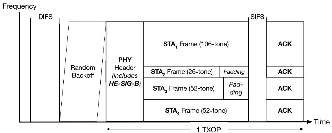
Figure 3.3. An example of IEEE 802.11ax DL-MU access for 20 MHz channel bandwidth with (106, 26, 52, 52) subcarrier allocations.
