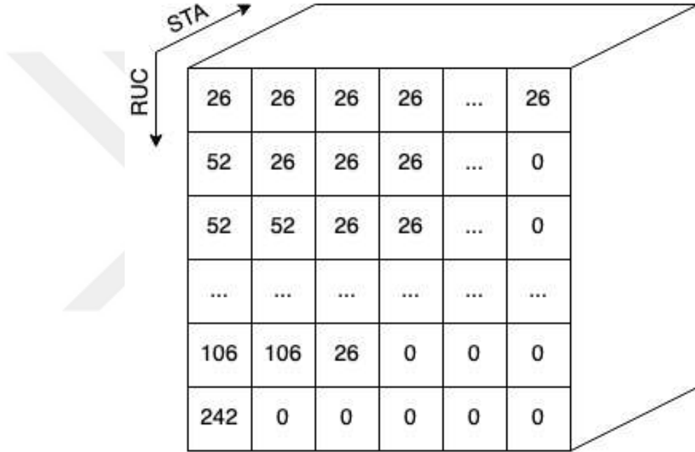
Figure 4.1. 3-dimensional depiction of the scheduling problem: Stations (STAs), RU configurations (RUCs), and Resource Units (RUs).
