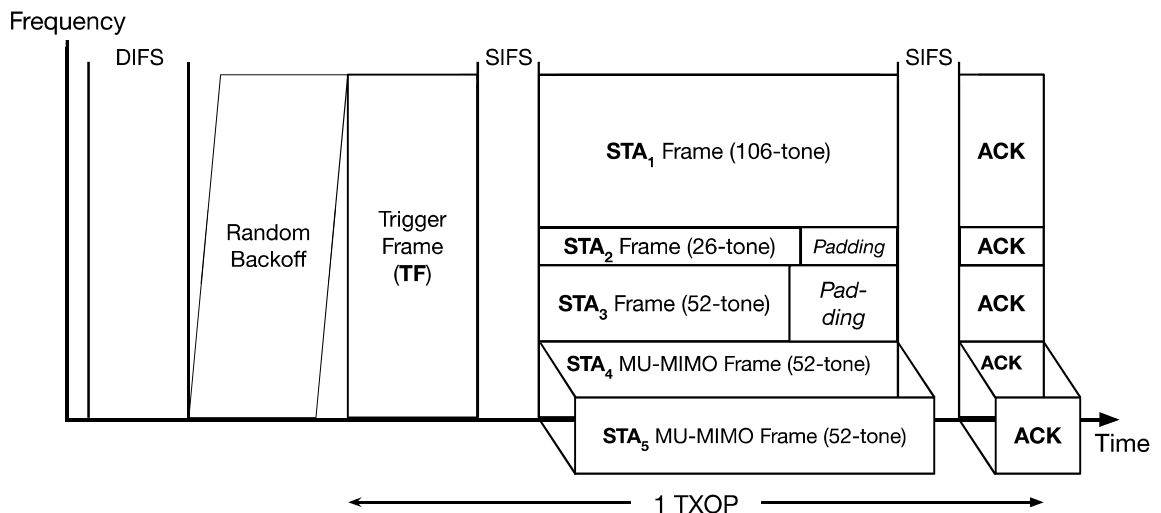
Figure 3.5. An example of IEEE 802.11ax UL-MU MIMO access for 20 MHz channel bandwidth. Here STA 5 is served on a different spatial stream.
