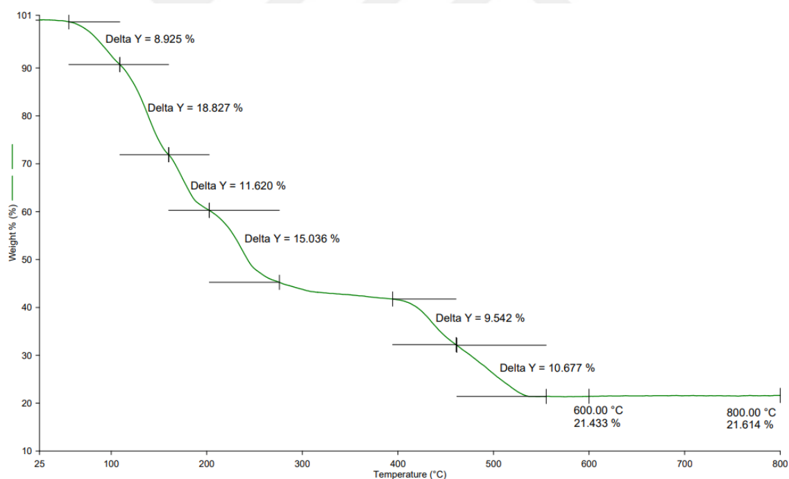
Figure 3. 7. TGA Analysis for \text{MgCl}_2 \cdot 6\text{H}_2\text{O}
