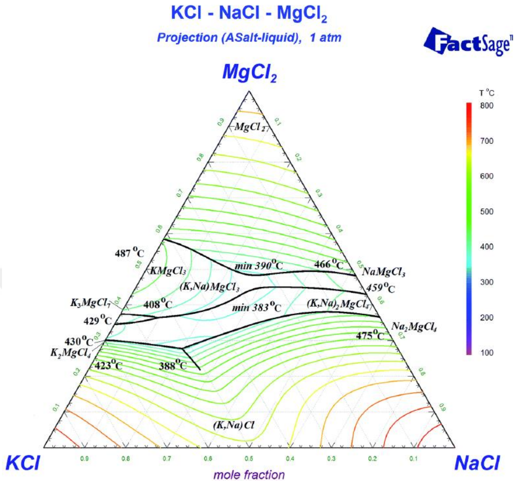
Figure 2. 17. Ternary phase diagram of NaCl MgCl 2 KCl by using FactSage Software 74 .
