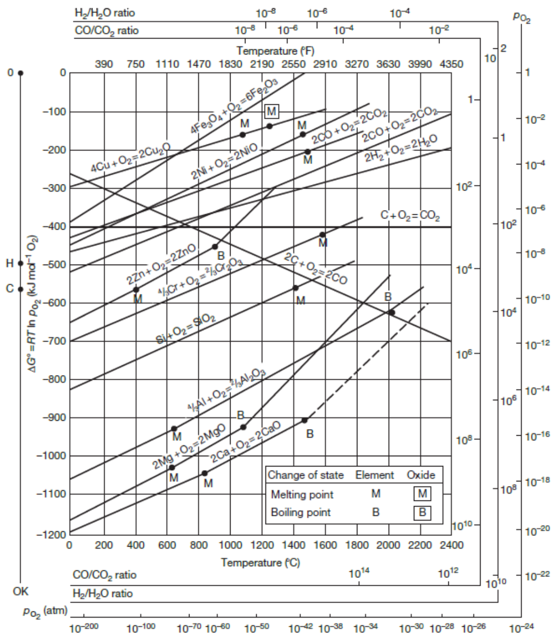
Figure 2. 11. Ellingham Diagram 52 .
