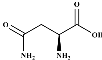
Şekil 2.20. L-Asparagin ( \text{C}_4\text{H}_8\text{N}_2\text{O}_3 ).
