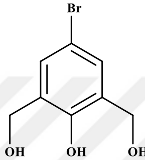
Şekil 2.19. BBHMP ( \text{BrC}_8\text{H}_5\text{O}_3 ).
