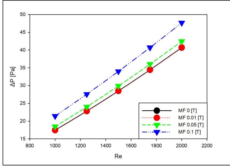
Figure 4. 33 Variation of Pressure drop with Re number for different MF intensities.
