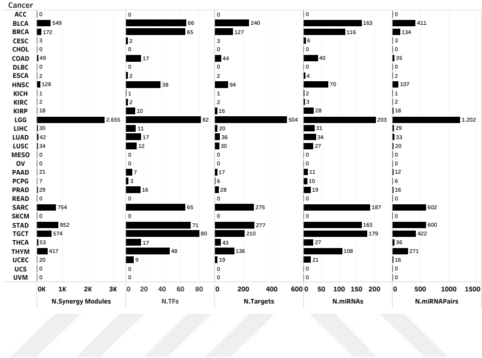
Figure 4.16 Each bar represents statistics for one cancer in Synergy Modules Type 3. From left to right: number of synergy modules, unique TFs, unique target mRNAs, unique miRNAs and unique miRNA pairs
