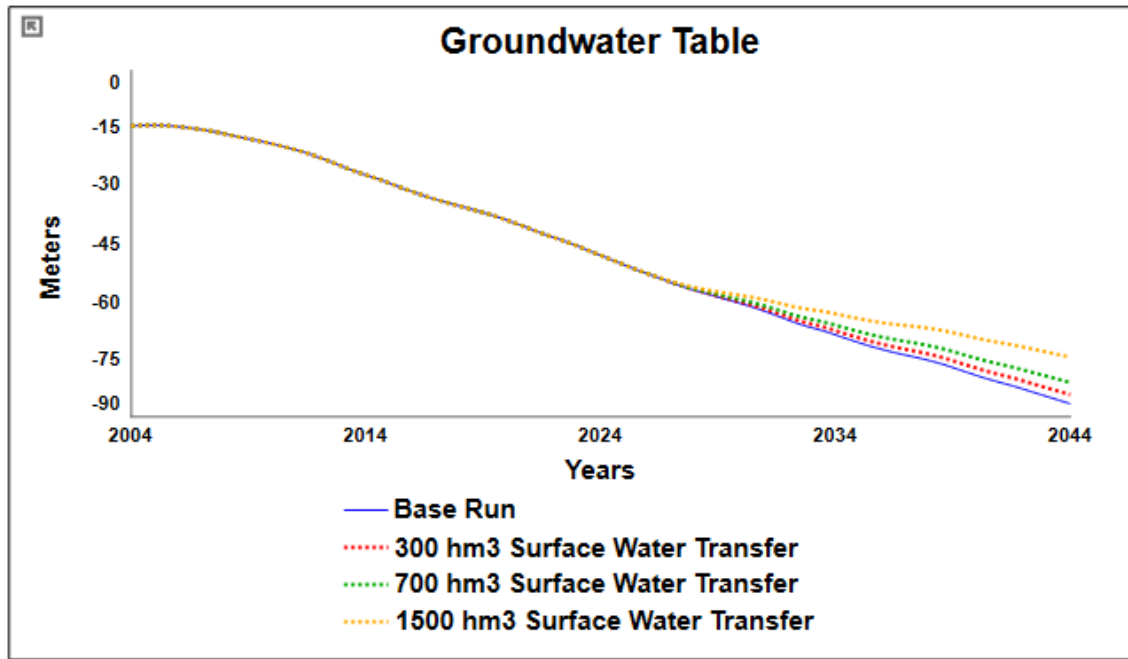
Figure 7.2. Scenario analysis 1: Groundwater table.
