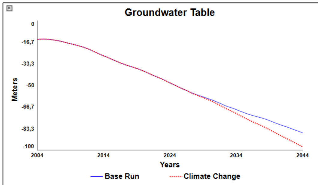
Figure 7.9. Scenario analysis 2: Groundwater table.
