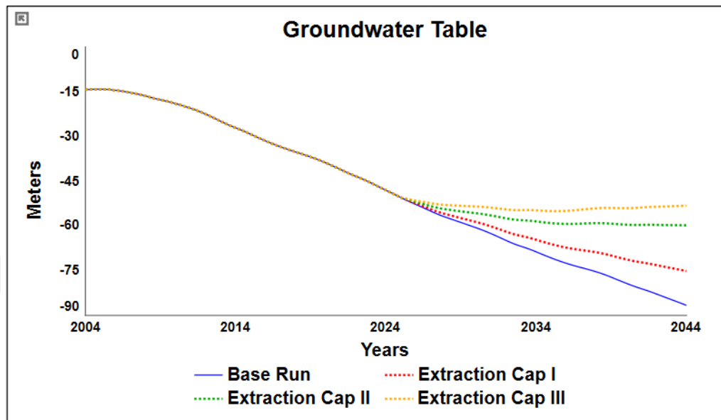
Figure 8.14. Policy analysis 3: Groundwater table.
