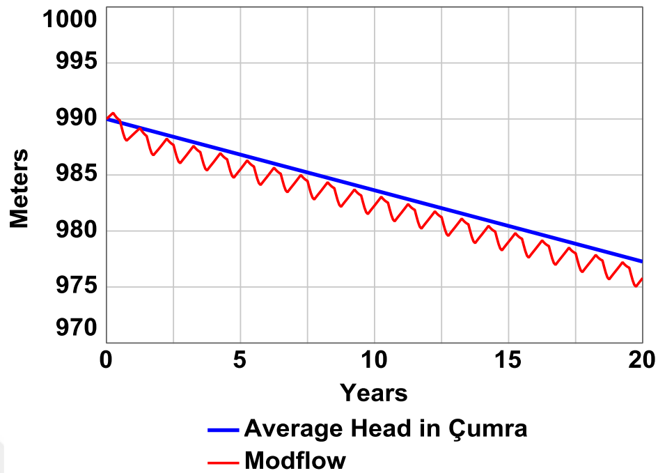
Figure 6.20. Precipitation-irrigation run.
