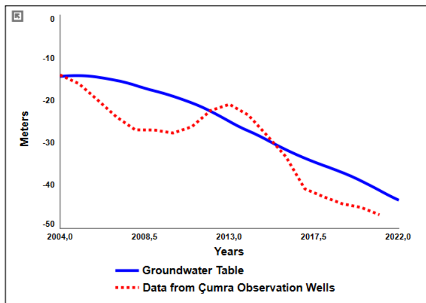
Figure 6.35. Groundwater table: data and simulation.
