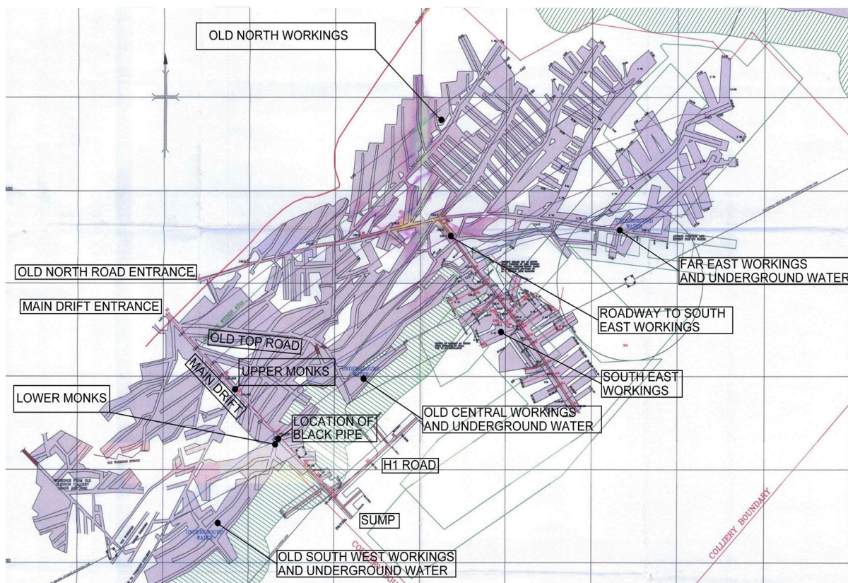
Figure 7-2 Mine Map 7 (Health and Safety Executive, 2015a)
