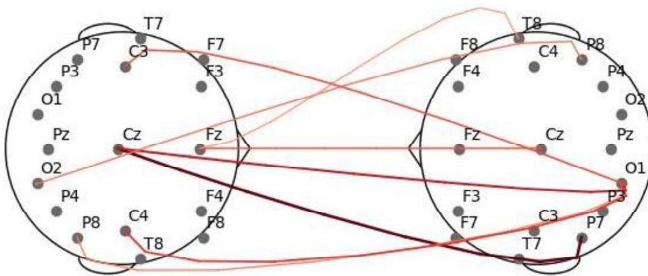
Figure 95: Topography figure showing significant interbrain connectivity comparisons in the beta band between 3-back and 0-back, the thickness of the line correlates with the \eta_p^2 value.
