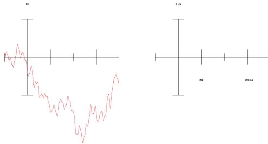
Figure 84: ERP for missed trial on T8 on extraverts' 1-back over task setting, the figure on right shows axis values.
