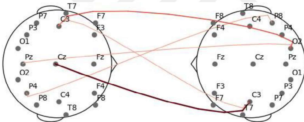
Figure 91: Topography figure showing significant interbrain connectivity comparisons in the alpha band between 2-back and 0-back, the thickness of the line correlates with the \eta_p^2 value.
