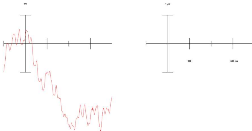
Figure 81: ERP for correct response to letter on P8 on social session between 0- and 2-back, the figure on right shows axis values.
