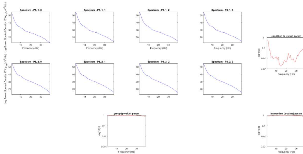
Figure 59: Results of EEG Power Spectrum Analysis on electrode P8 for n-back levels across all participants over extraversion in social setting. Spectrum-1 means introverts' data and Spectrum-2 means extraverts' data, whereas the numbers next to them show n-back level and electrode.
