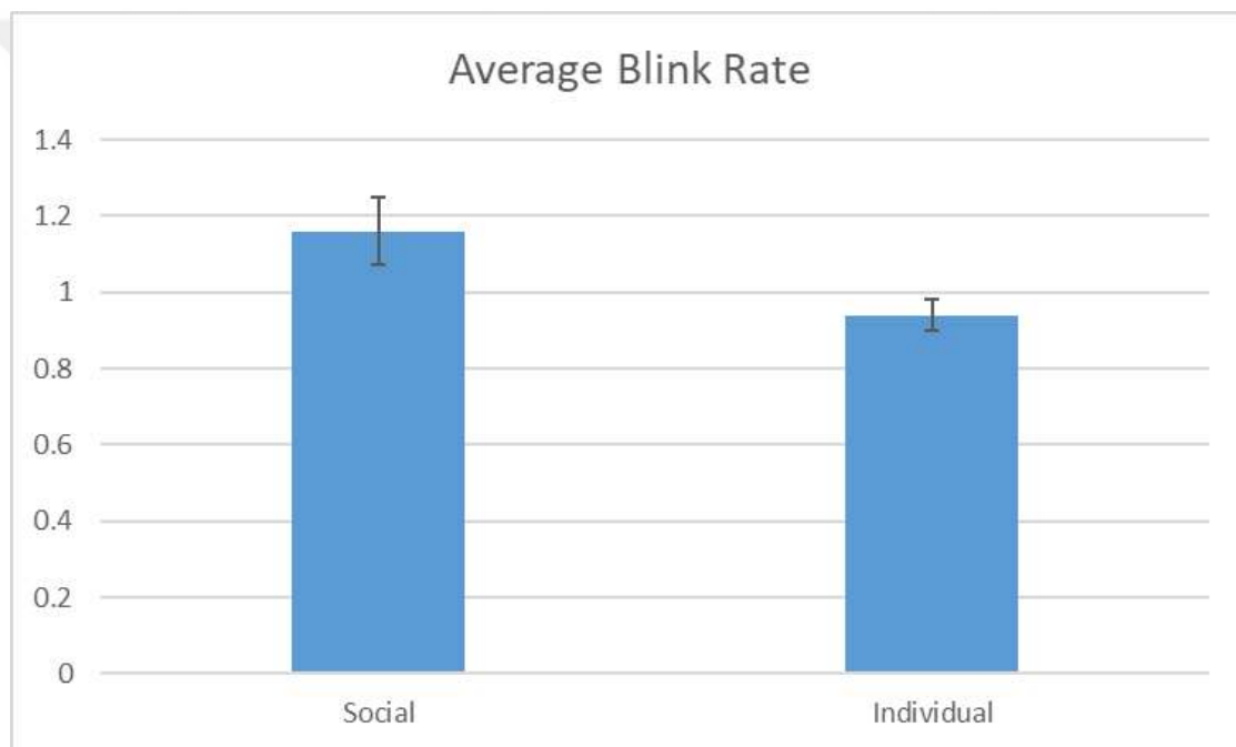
Figure 13: Average Blink Rate for social condition and individual action during 3-back.
