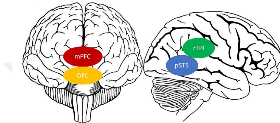
Figure 2: Brain regions associated with Theory of Mind.
