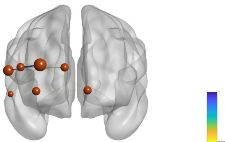
Figure 45: Topography of significant results for the intrabrain comparison of 1- and 2-back in HbR.
