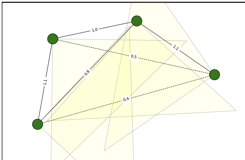
Figure 3.11. Edge weight calculation for an example group formation. The edge pruning tolerance is set at an arbitrary value of 0.6. The dashed edges indicate edges to be removed from graph.
