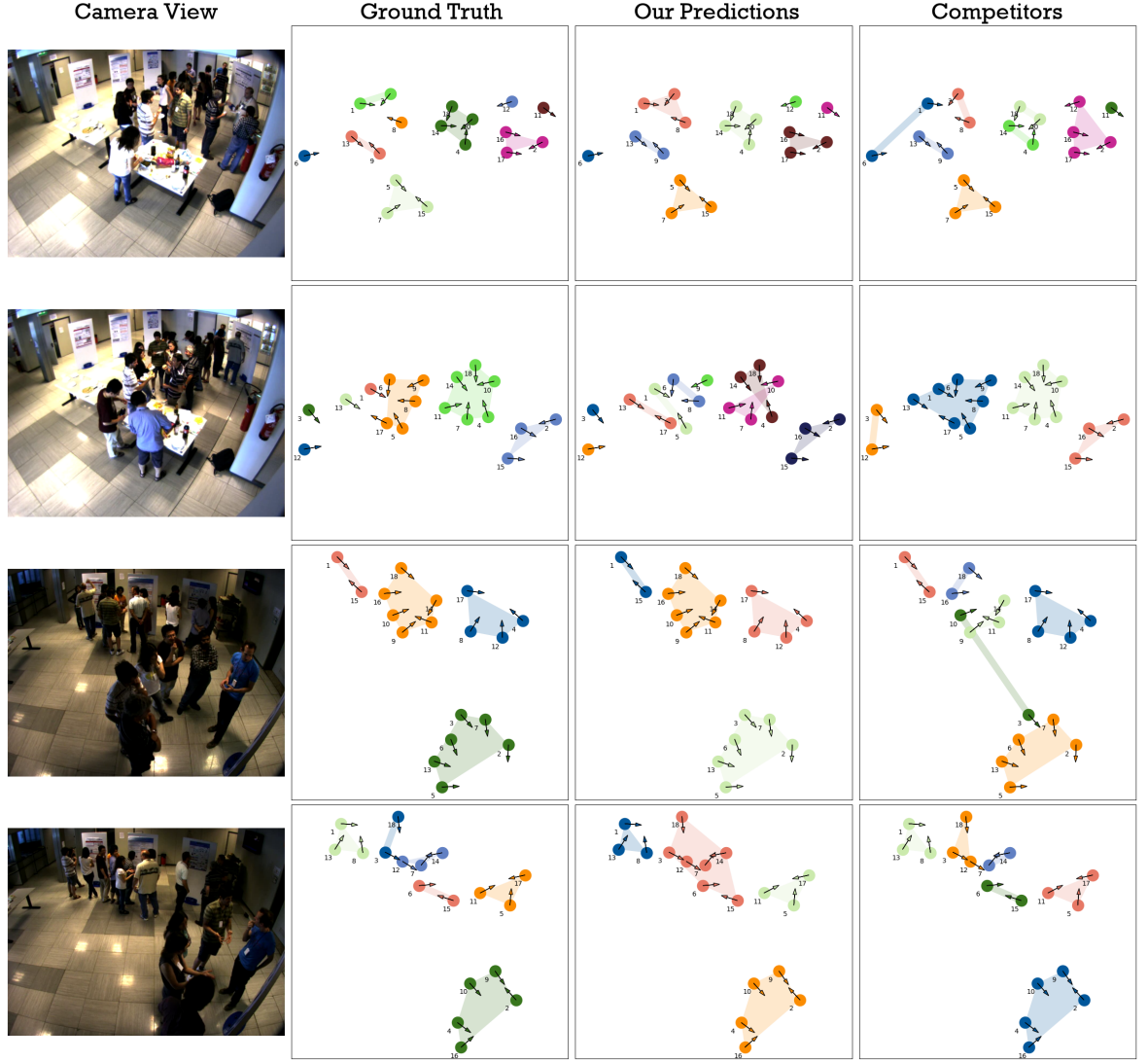
Figure 4.9. Visual group detection results. The first two rows of results are from the SALSA Cocktail Party dataset, and the next two rows are from the SALSA Poster Session. The first column shows the video frame, the second column shows the ground truth, the third column shows the results from our approach, and the last column shows the results from the best competitors, e.g., the GCFF approach for the Cocktail Party and DANTE for the Poster Session dataset.
