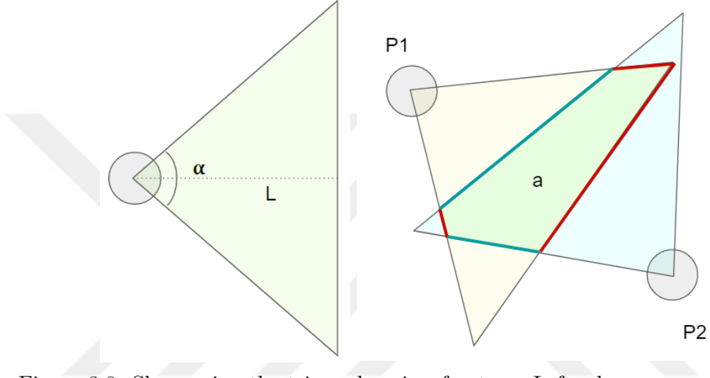
Figure 3.8. Showcasing the triangular view frustum. Left: shows an example view frustum of a single person where L is the length of frustum and \alpha is the frustum angle. Right: shows the intersection of two view frustums. Red and cyan lines represent the edges obtained from Sutherland-Hodgman algorithm with respect to P1 and P2.
