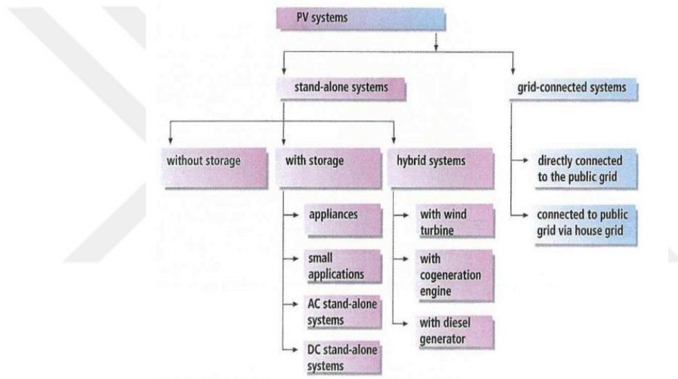
Figure 2.2. Types of PV systems [22].
