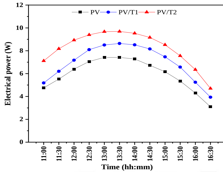
Figure 6.4. Electrical power of modules.
