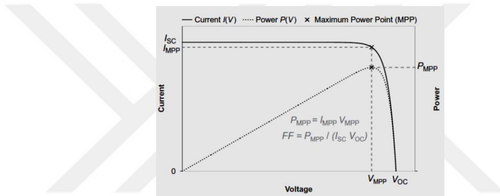
Figure 2.21. I-V and P-V curves [62].
