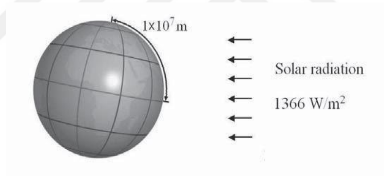
Figure 1.5. The yearly solar energy that reaches earth's surface [14].
